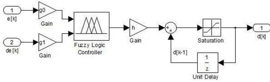
Figure 4.11 Calculation of PWM Duty Value after FLC
