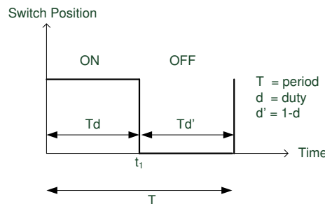
Figure 2.2 Switch Positions
