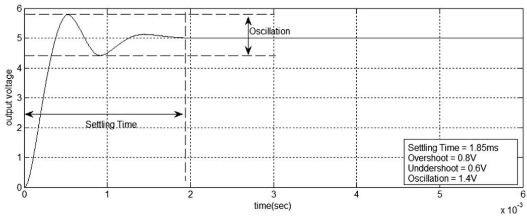
Figure 4.14 Transient Response of Optimized Controller
