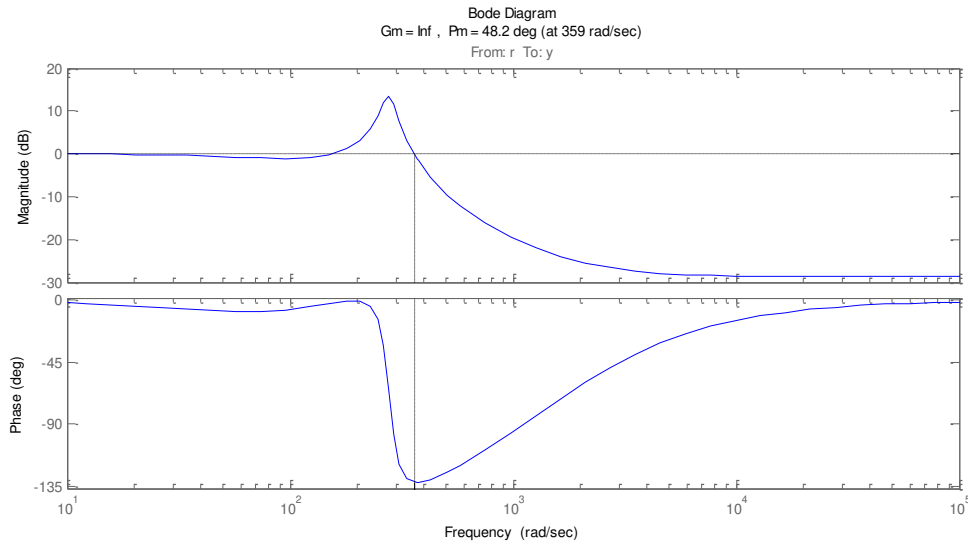
Figure 4.21 Bode Plot of the Closed-loop System with NZ tuned
