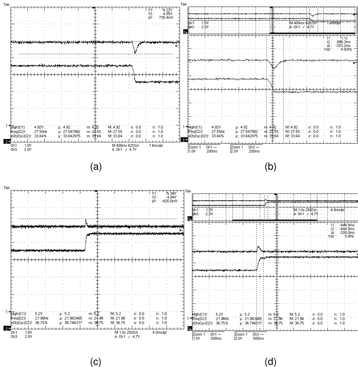
Figure 5.10 Transient Response of the System with FLC under Line Variation between 7.2V and 11V (a) Voltage Change of the System for Line Variation from 9V to 7.2V (b) Recover Time of the System for Line Variation from 9V to 7.2V (c) Voltage Change of the System for Line Variation from 9V to 11V (d) Recover Time of the System for Line Variation from 9V to 11V
