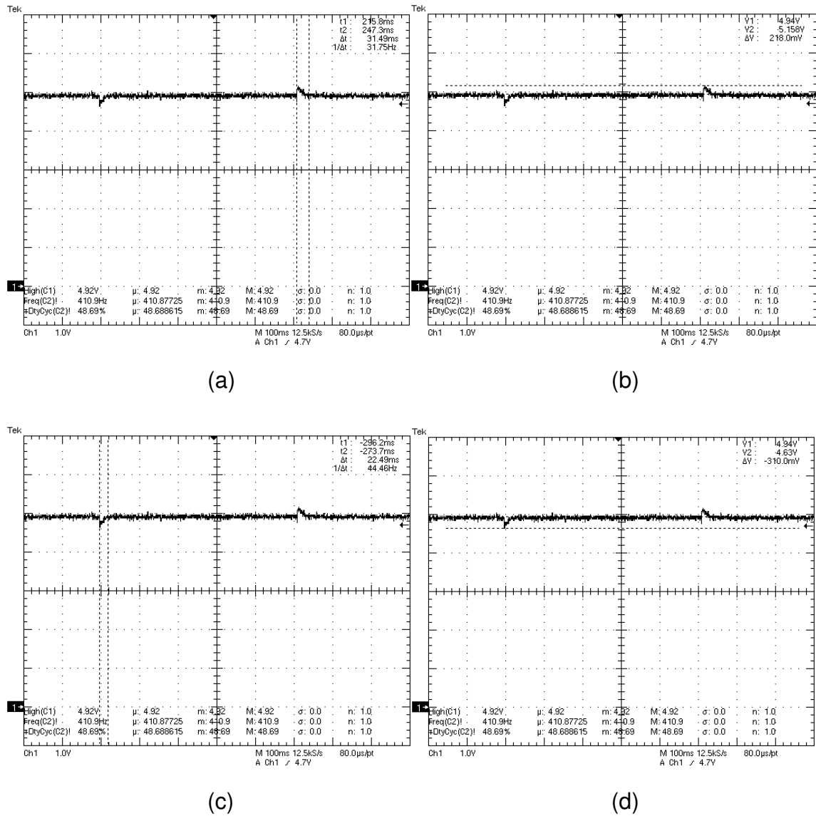
Figure 5.4 Transient Response of the System with SMC under Load Variation between 10Ω and 5Ω (a) Recover Time of the System for Load Variation from 5Ω to 10Ω (b) Voltage Change of the System for Load Variation from 5Ω to 10Ω (c) Recover Time of the System for Load Variation from 10Ω to 5Ω (d) Voltage Change of the System for Load Variation from 10Ω to 5Ω
