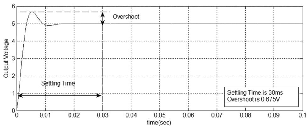
Figure 4.25 Output Voltage of the Synchronous Buck Converter by PSO
