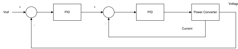
Figure 3.9 Current PID Controller Block Diagram
