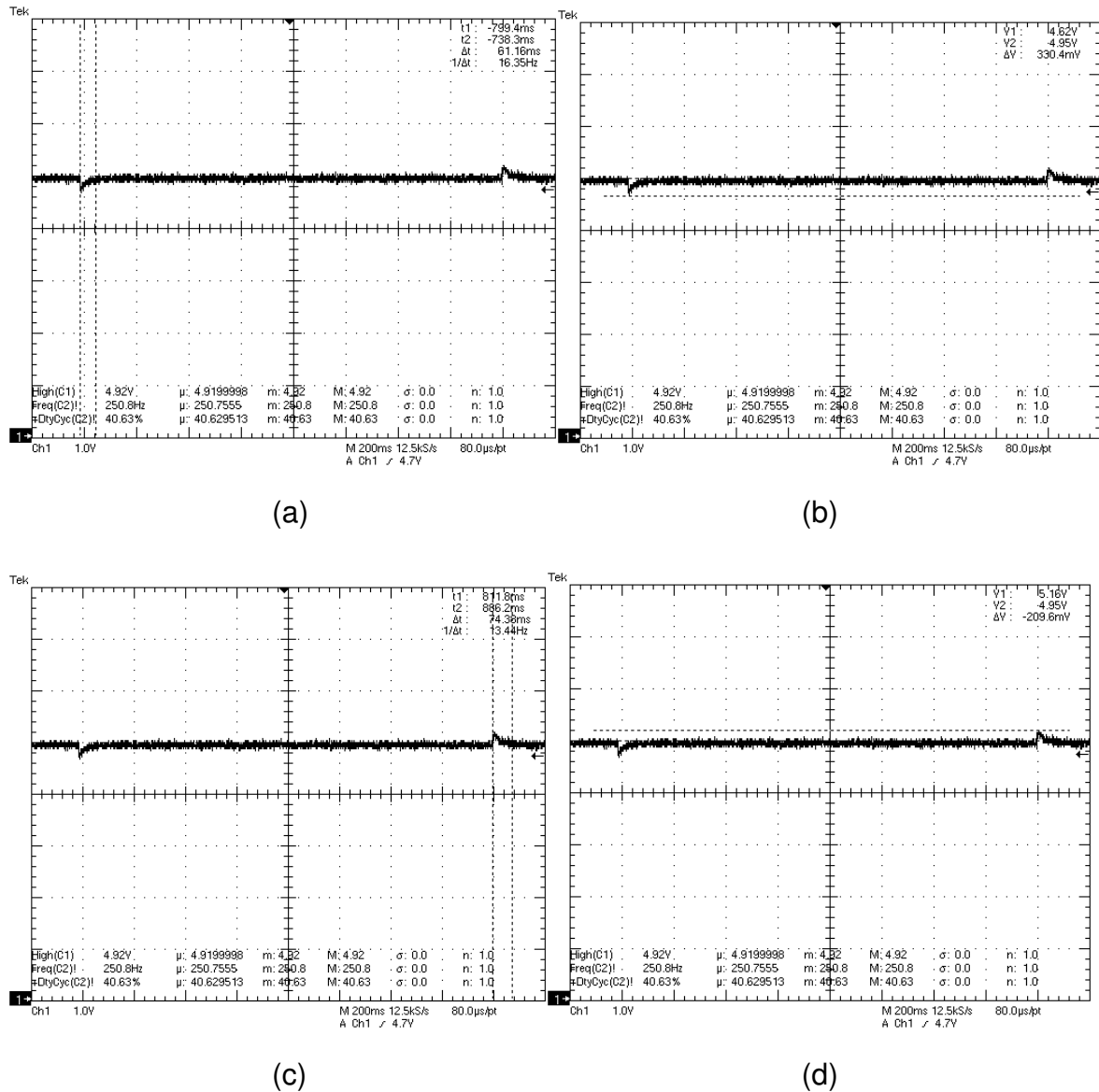
Figure 5.9 Transient Response of the System with FLC under Load Variation between 10Ω and 5Ω (a) Recover Time of the System for Load Variation from 5Ω to 10Ω (b) Voltage Change of the System for Load Variation from 5Ω to 10Ω (c) Recover Time of the System for Load Variation from 10Ω to 5Ω (d) Voltage Change of the System for Load Variation from 10Ω to 5Ω
