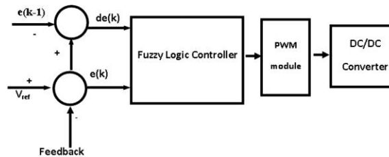
Figure 3.4 General Fuzzy Logic Controller Scheme
