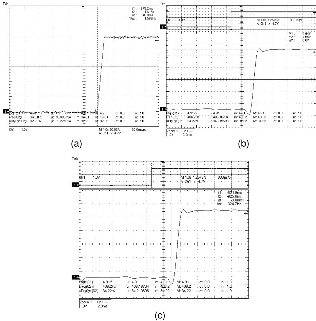
Figure 5.3 Transient Response of the SM Voltage Controller with (a) Initial Duty is Zero (b) Overshoot of the System that has the Initial Duty is equal to Steady State Duty (c) Settling Time of the System given in (b)
