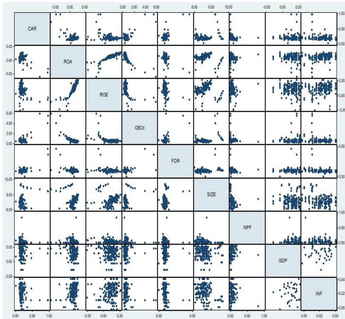
Appendix 2: Graphical Data Point Outlier Detection (Scatter Matrix Plot)
