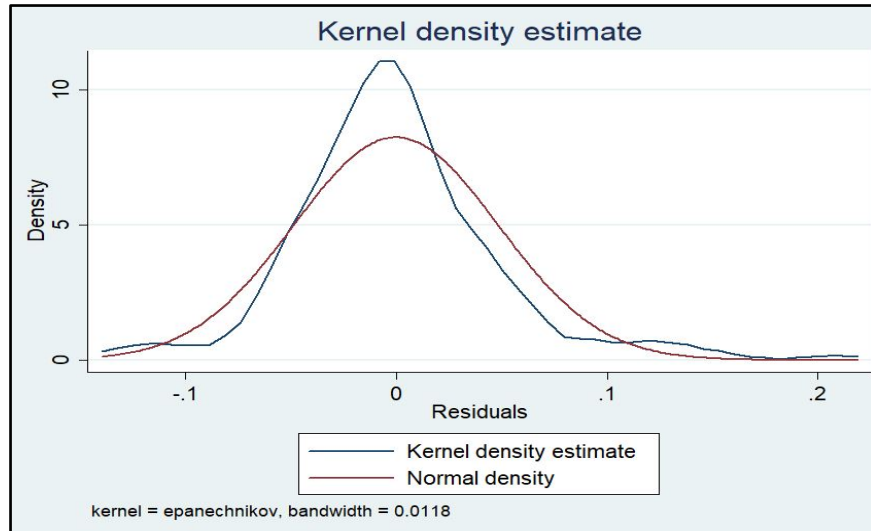
Figure 3: KDensity Graphic Normality Test
