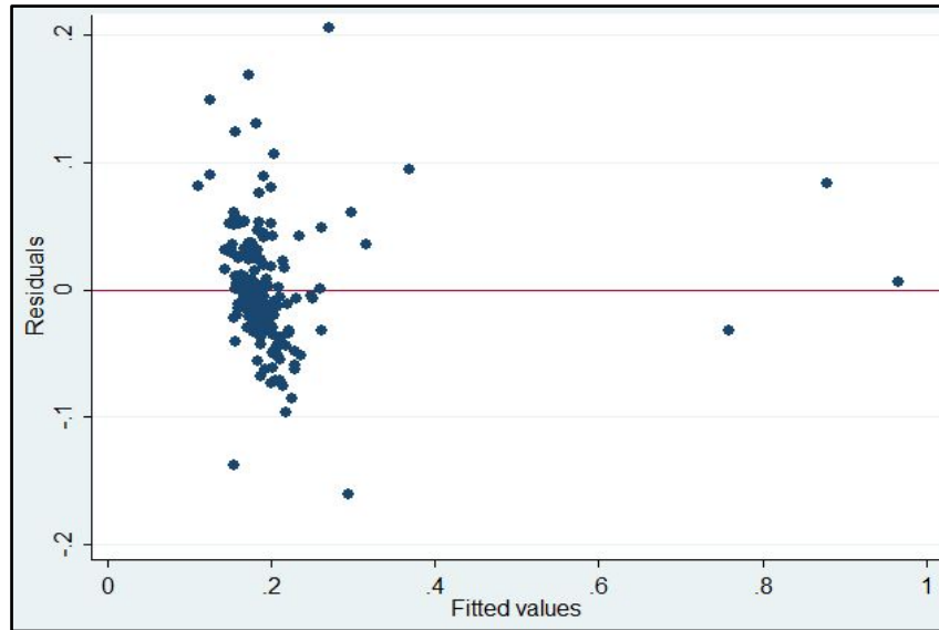
Figure 4: Residual-Versus-Fitted (RVF) Plot
