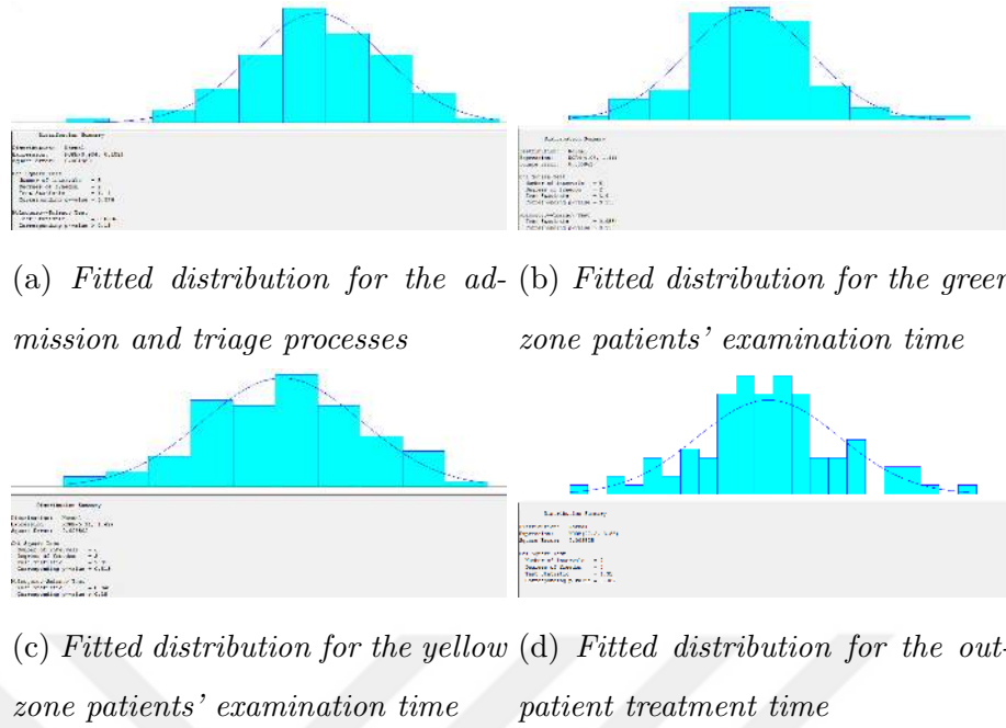
Figure 3.2. Fitted distributions
