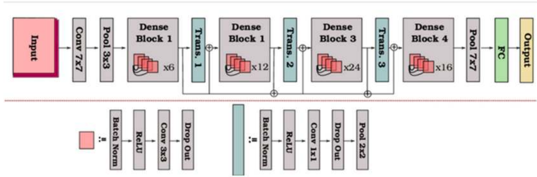
Figure 5.10: DenseNet121 Architecture.
