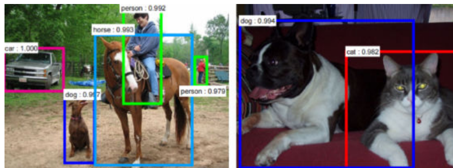
Figure 2.10: Image Segmentation.
