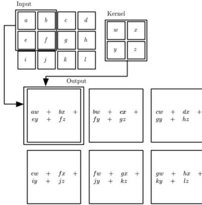
Figure 2.11: 2D convolution.
