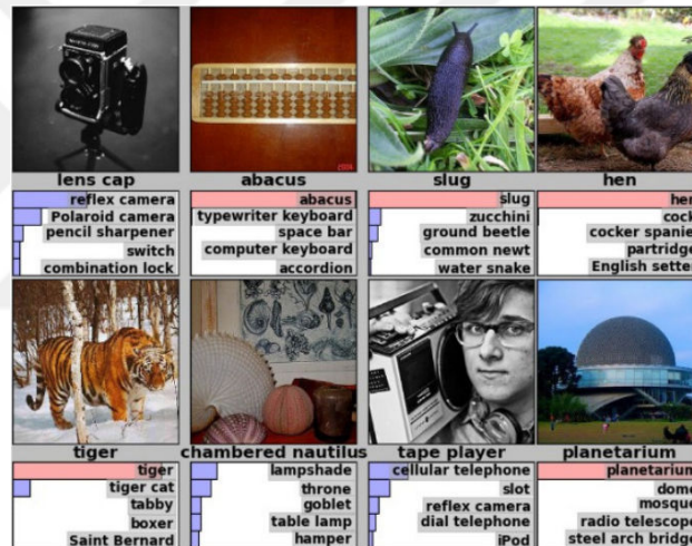
Figure 2.9: Image annotation.
