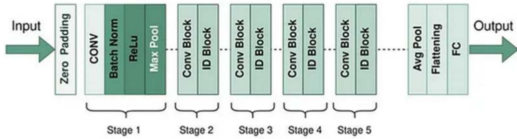
Figure 5.8: ResNet50 Architecture.
