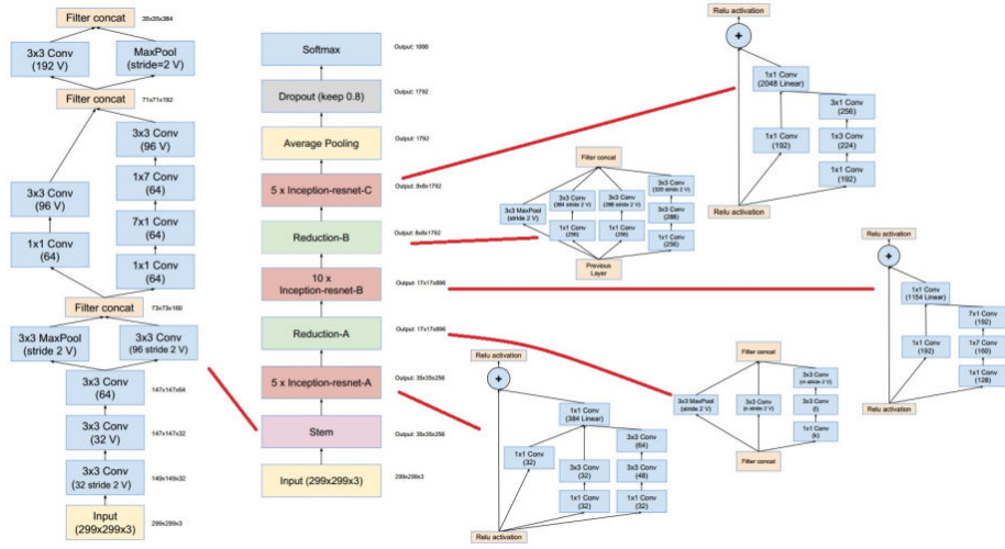
Figure 2.19: Inception-v4, Inception-resnet [81].
