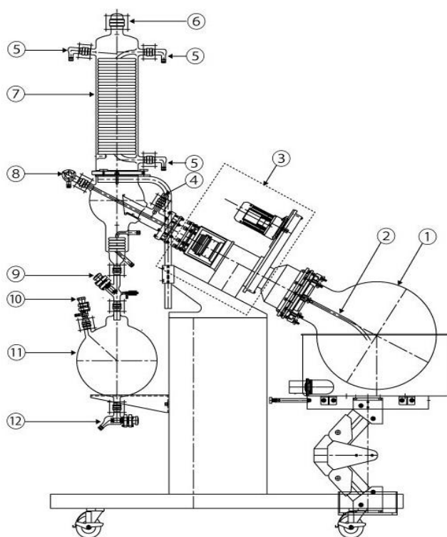
Figure 1.9: Rotary Evaporator
