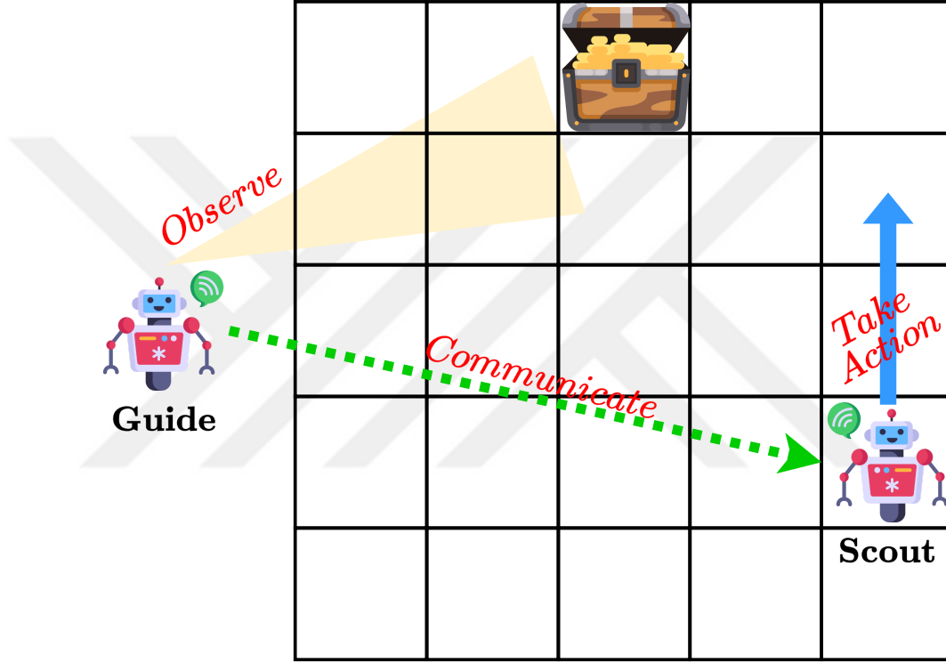
Figure 2.16: Proposed formulation of effectiveness level communication [170] as a guided robot problem in grid world as MARL. The guide has perfect information about the state of environment but it is unable to take any action on the grid world whereas the scout can take actions, i.e., 16 possible movements and their corresponding hand crafted codewords, however cannot observe the environment state at all. Hence, the guide leads the scout to capture the treasure chest by communicating through noisy channel. The authors models both the guide and the scout as 3-layer MLPs and utilize deep reinforcement learning algorithms to train the agents. In particular, the guide is trained to learn a semantic encoding robust against the variations in the channel for the transmission of the action that the scout should take. On the other hand, the scout is trained to learn a semantic decoding technique to accurately recover the transmitted action-to-take.
