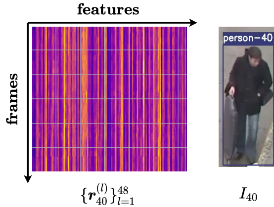
(c) Second and third level attributes of Person-40. The second level includes a set of collected feature vectors across 48 frames with T_{40} = 48 . The third level includes the cropped RGB image I_{40} , although alternative encoded versions of I_{40} can also be used.
