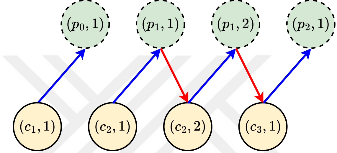
Figure 3.2: Instance level semantic graph \mathcal{D} . Just like class level graph \mathcal{S} , instance level graph \mathcal{D} preserves the directed bipartite graph structure formed by signal components and predicates. As illustrated, there may be more than one instance that belongs to the same class, both for signal components and predicates which are indexed by k . The signal components are drawn with solid yellow circles and depicted as nodes (c_i, k_i) whereas the predicate nodes are drawn with dashed green circles and denoted by (p_j, k_j) . This structure allows us to express both state indicating information for individual instances such as (c_1, 1) \rightarrow (p_0, 1) or (c_3, 1) \rightarrow (p_2, 1) and relation among the individual components and predicates such as (c_2, 1) \rightarrow (p_1, 1) \rightarrow (c_2, 2) or (c_2, 2) \rightarrow (p_1, 2) \rightarrow (c_3, 1) , simultaneously. Note that, since (c_1, 1) component is disconnected from others, it is connected to (p_0, 1) by default.
