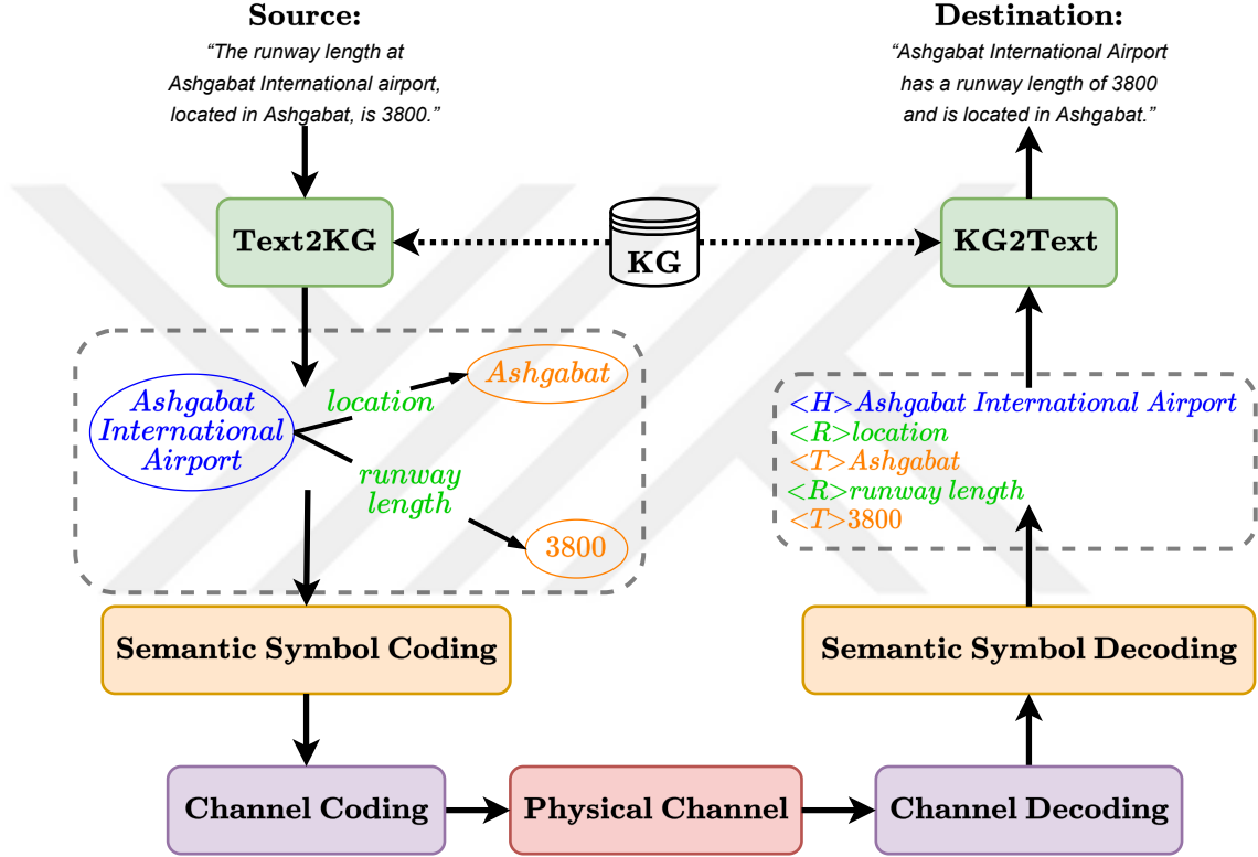
Figure 2.15: Cognitive semantic communication framework for text transmission proposed in [168] leverages knowledge graph as arbitrary semantic modality. The text-to-knowledge graph (Text2KG) module is a simple alignment algorithm which sequentially processes each sentence and constructs a concise knowledge graph consist of triplets ( head, relation, tail ). The Semantic Symbol Coding module is a simple dictionary ( key, value ) that maps each possible triplet to a unique integer and encodes the integers to fixed length bit-sequence. The Semantic Symbol Decoding module is a correction algorithm which traverses the possible triplets in the knowledge graph to find most similar ones observed by the receiver. Finally, the recovered set of triplets are processed by the knowledge graph-to-text (KG2Text) module comprised of a fine-tuned NLP transformer module to output semantically identical text.
