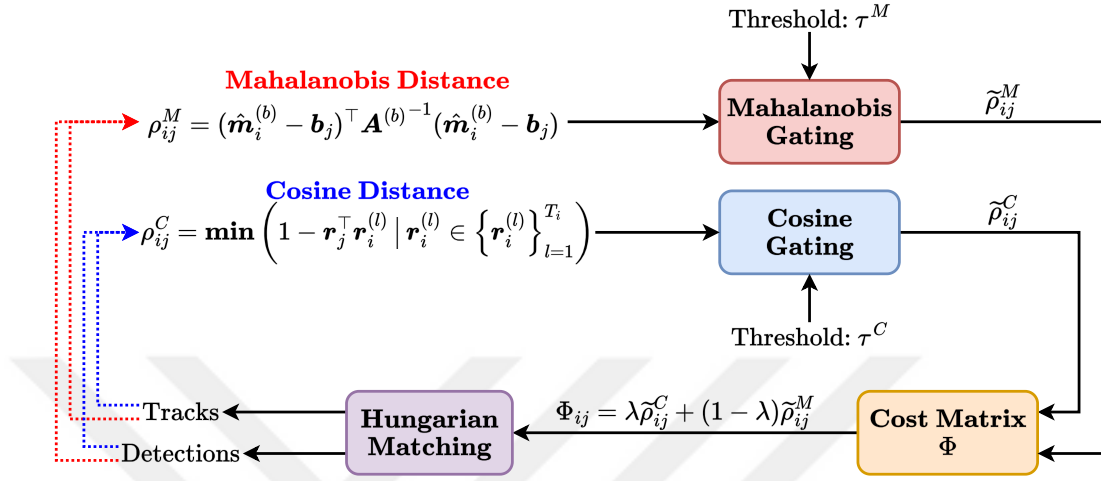
Figure 4.5: First association process of DeepSORT via Matching Cascade. For each track i and detection j pair, two distance metrics are computed, namely, Mahalanobis distance \rho_{ij}^M of bounding box coordinates and cosine distance \rho_{ij}^C of feature vectors. We denote the entries that corresponds to bounding box coordinates of estimates with (b) superscript as in state estimate \hat{\mathbf{m}}_i^{(b)} and covariance matrix \mathbf{A}^{(b)-1} , and use \mathbf{b}_j for bounding box coordinates of detection j . For feature dictionary configuration, we use the smallest cosine distance among all extracted feature vectors in \{\mathbf{r}_i^{(l)}\}_{l=1}^{T_i} of track i . If the computed distance values exceed the predefined gating thresholds \tau^M or \tau^C , we replace them with infinity to prevent unfavourable matching outcomes. The entries of cost matrix consist of convex combination of gated Mahalanobis \tilde{\rho}_{ij}^M and gated cosine \tilde{\rho}_{ij}^C distances. Finally, the resulting cost matrix is used by Hungarian assignment algorithm [200] to match tracks and detections.
