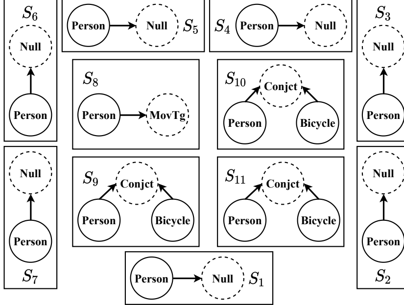
(b) Class-level abstractions are performed on disconnected subgraphs similar to the one in Fig. 4.7c so that we obtain \mathcal{S} = \{S_1, \dots, S_{11}\} . Together with original graph \mathcal{D} and attribute set \mathcal{A} , abstraction \mathcal{S} forms the complete semantic description \mathcal{Y} . Global goal-based filtering is performed using these high-level graphs.
