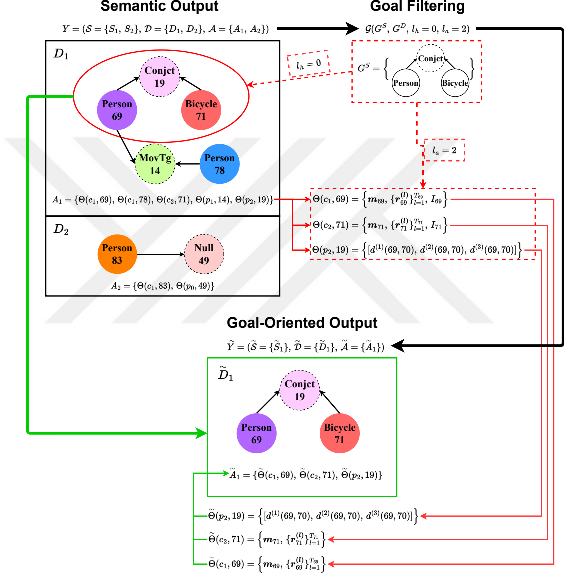
Figure 4.9: A goal-based filtering example. The filtering operation yields goal-oriented semantic description \tilde{Y} . Dashed red lines denote the queries/goals and solid green lines denote the goal-oriented returns. For brevity, we do not visualize class-level graphs S . The goal pattern G^S is searched in S_1 and D_1 to provide \tilde{S}_1 , and \tilde{D}_1 . Graph complexity is chosen as l_h = 0 so that only the exact matchings are returned. The corresponding attributes A_1 are distilled into \tilde{A}_1 according to the given attribute complexity parameter l_a = 2 .
