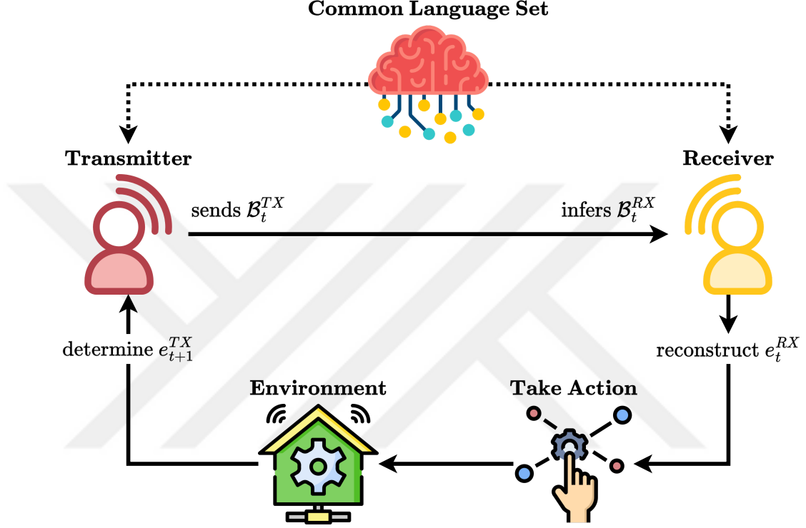
Figure 2.17: Schematic of goal-oriented semantic communications with common language set proposed in [175]. The transmitter observes an event e_t^{TX} at time t as the environment state and describes it with its believes \mathcal{B}_t^{TX} , i.e., with elements from the common language set independent of the data modality. Next, the receiver infers \mathcal{B}_t^{RX} based on \mathcal{B}_t^{TX} and reconstructs the event e_t^{RX} based on the combined believes \mathcal{B}_t = \{\mathcal{B}_t^{TX}, \mathcal{B}_t^{RX}\} . Finally, the receiver takes an action based on the reconstructed event e_t^{RX} and triggers transition of the environment to the next event e_{t+1}^{TX} observed by the transmitter. Since the transmitter and receiver have no information about the usefulness of any descriptor, they gain this knowledge by experiencing rewards while executing various tasks. Particularly, constructed belief sets hierarchically expand at each iteration based on the incurred transmission, inference and task execution costs. Therefore, the problem is formulated as constrained infinite horizon discounted cost Markov decision process. Due to sparseness of rewards and massive number of possible descriptor the authors adopt curriculum learning approach of MARL to solve the formulated constrained optimization problem such that the transmitter learns to choose useful beliefs to describe each event as concise as possible whereas the receiver learns to complete the transmitted description.
