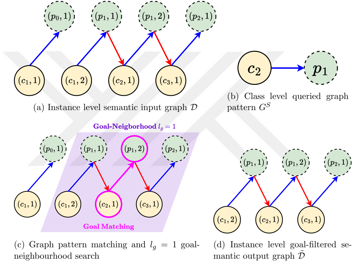
Figure 3.3: An example goal-filtering process with G^S and l_g arguments. (a) The instance level input graph \mathcal{D} contains 3 types of predicates and signal components with varying multiplicity regarding instances. (b) The class level queried graph pattern G^S seeks to gather all the nodes where a c_2 type component instance is connected to p_1 type predicate instance. (c) The input \mathcal{D} contains the queried graph pattern G^S which denoted in magenta. The specified neighbourhood complexity is l_g = 1 retrieves the other signal component and predicate nodes within 1-hop distance with respect to predicates. (d) The instance level output graph \tilde{\mathcal{D}} has lesser complexity than the input graph \mathcal{D} , since the isolated (c_1, 1) component and the associated null predicate (p_0, 1) instances are goal-filtered.
