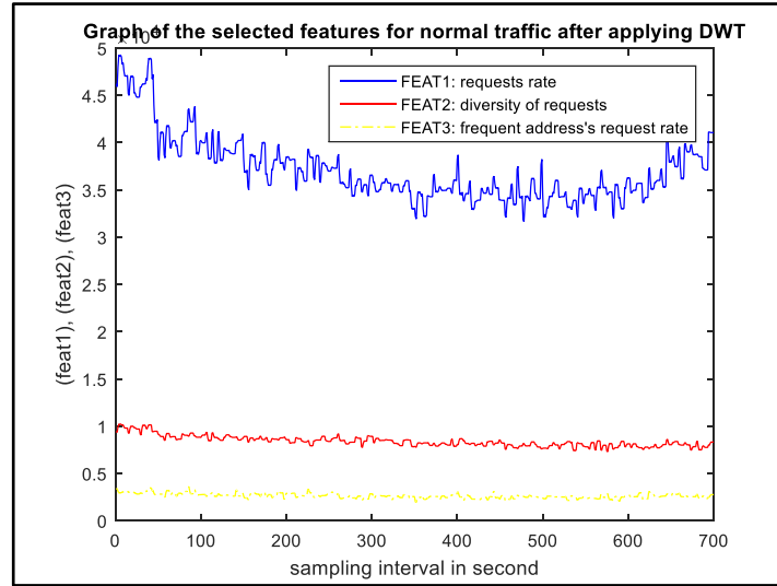
Figure 4.15. The DWT-based new generated features representing the normal traffic
