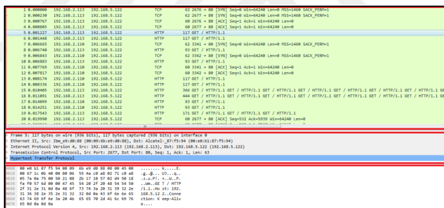
Figure 4.1. Network traces with their packet payload captured during the 15 th of June auditing activity.
