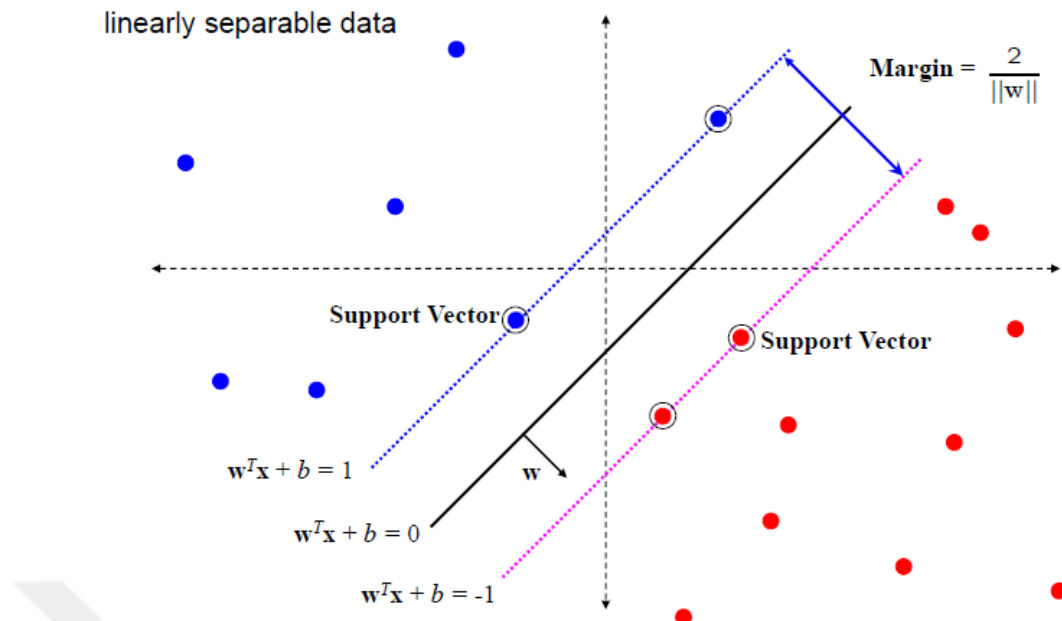
Figure 3.3. Linear hyperplane that maximizes the margins between binary classes (49)
