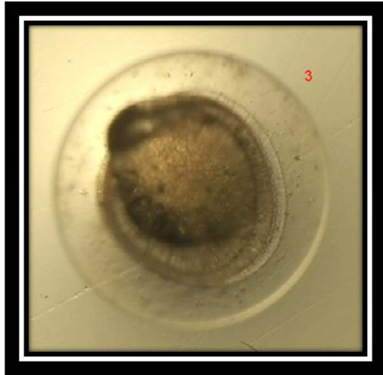
Congeridae sp.
