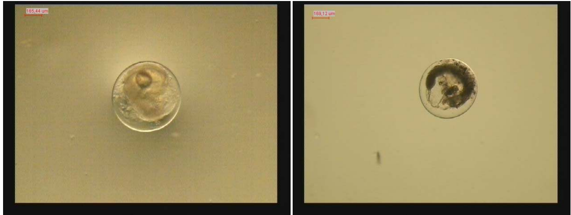
Bothidae sp.
