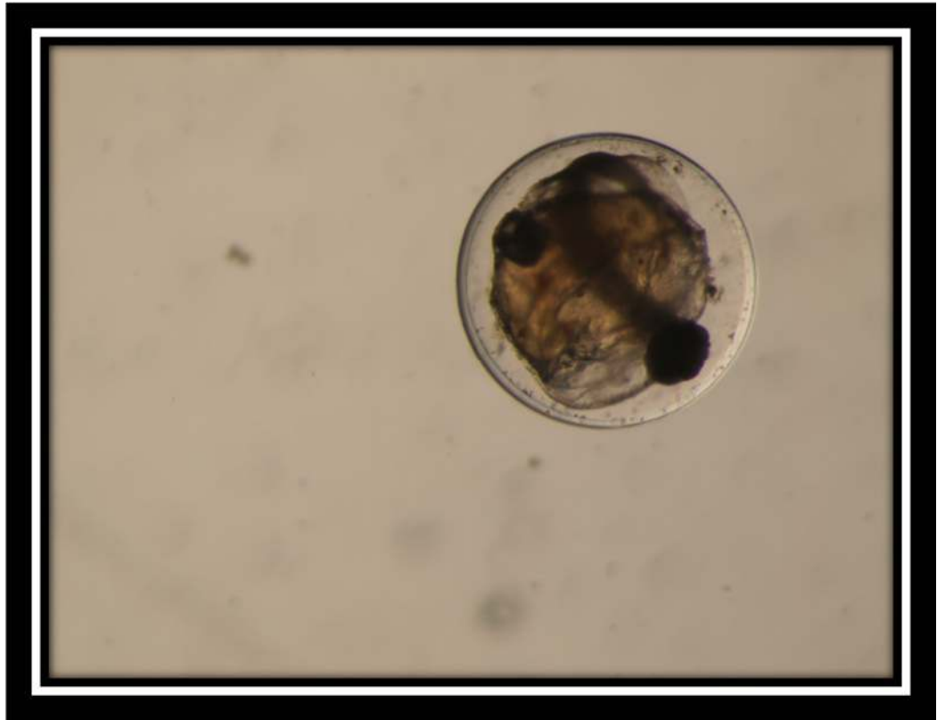
Argyropelecus hemigymnus
