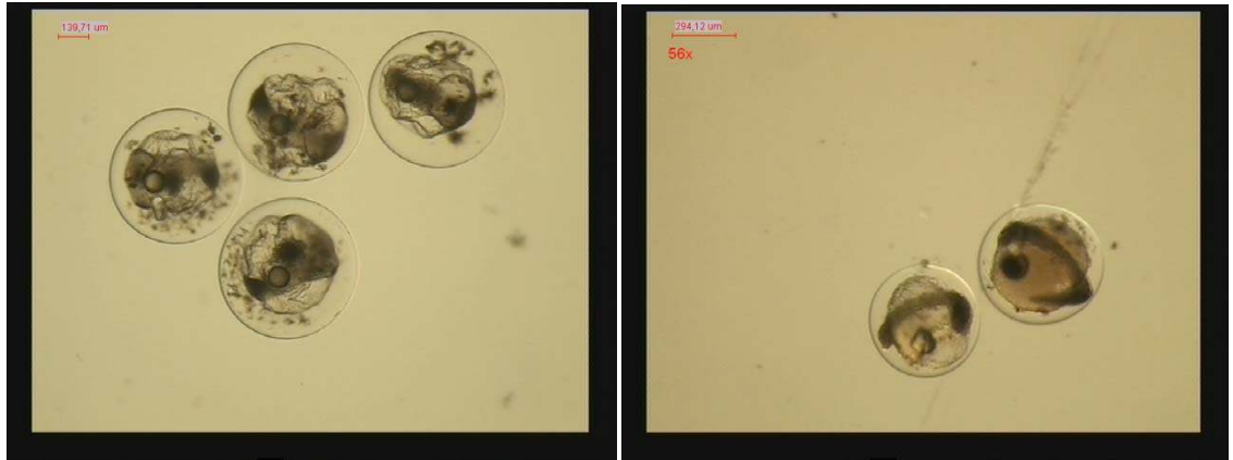
Labridae sp.
