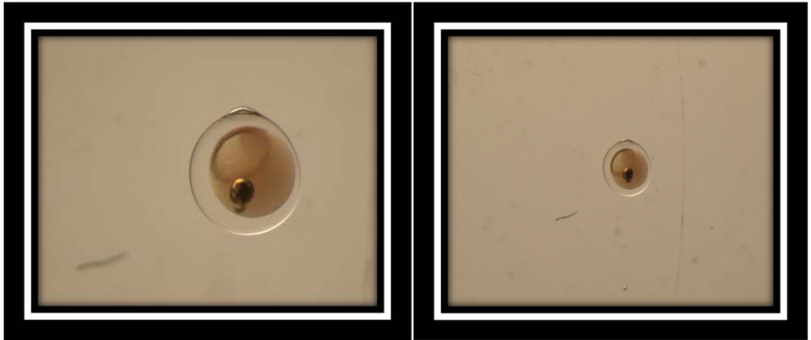
Centracanthidae sp.
