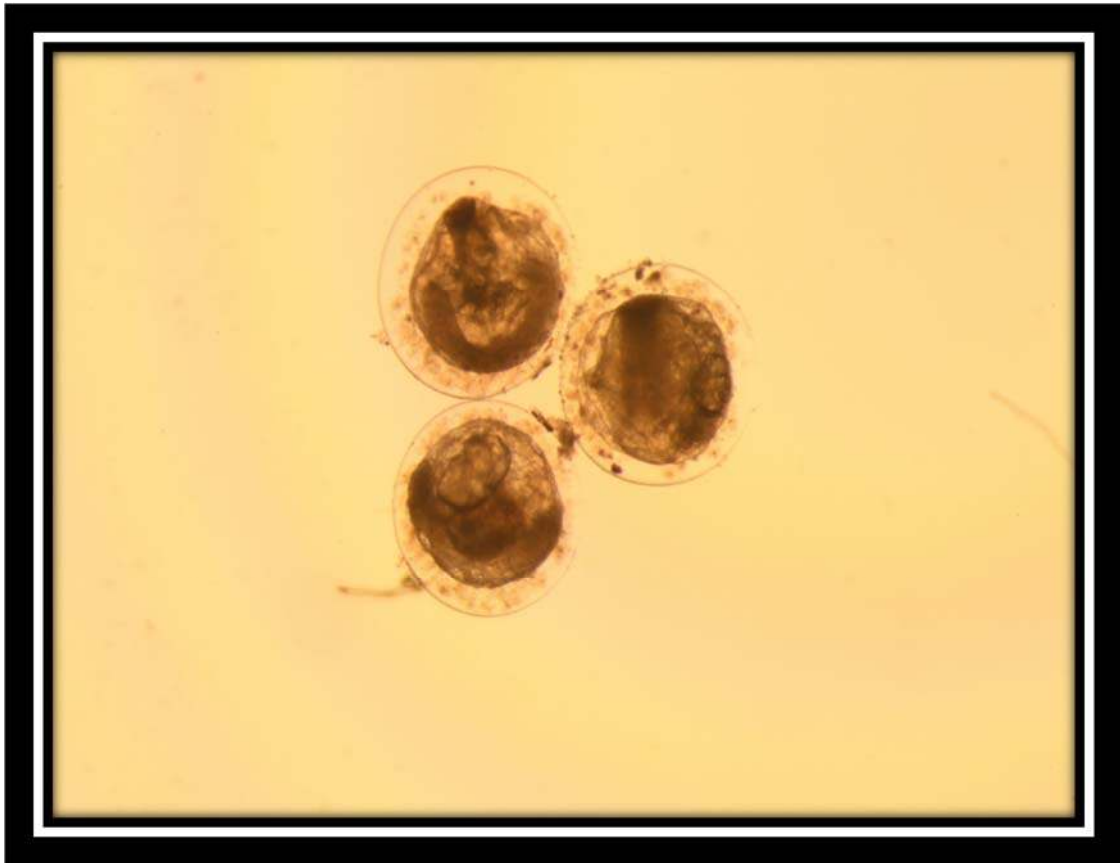
Upeneus sp.
