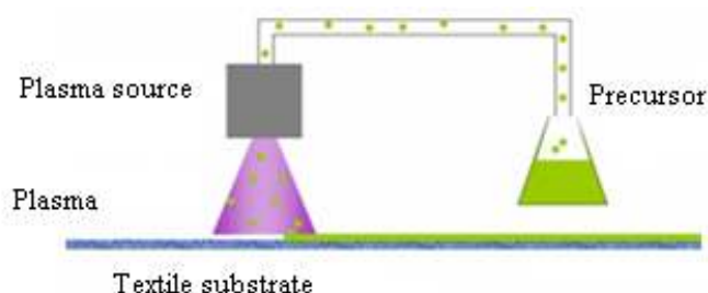
Figure 3.2. Plasma treatment [41]
