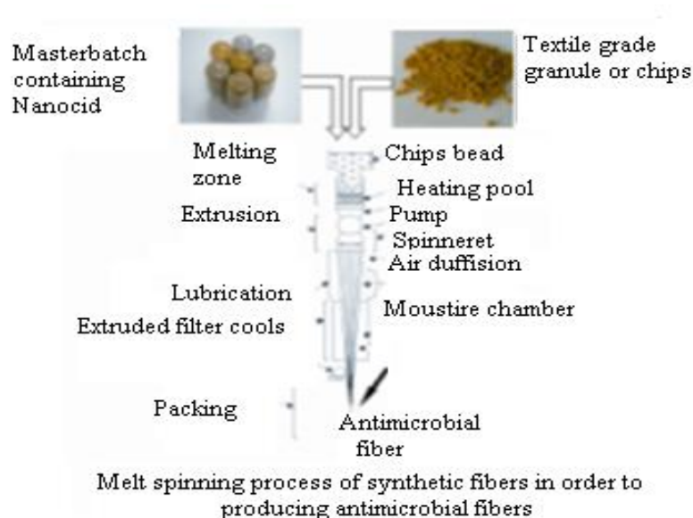
Figure 3.7. Spinning process [49]
