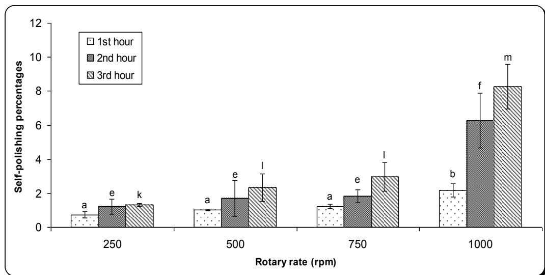
Figure 3.5 Effect of rotary rate on the self-polishing percentage of fibre reinforced lanolin based material which contains %1 fiber 1 (w/w) at 40 °C.
