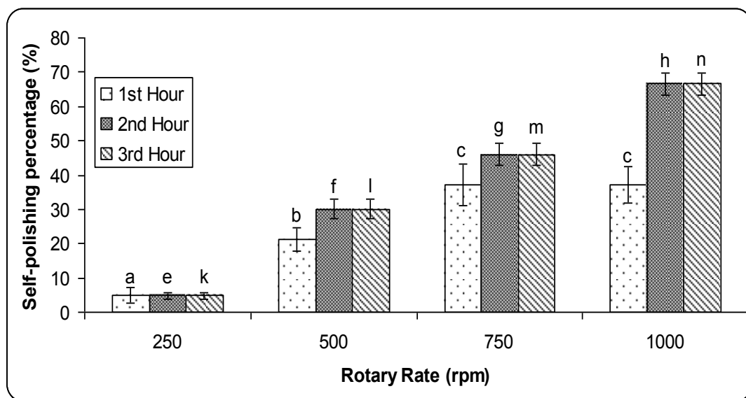
Figure 3.12 Effect of rotary rate on the self-polishing percentage of fibre reinforced lanolin based material which contains 5% Fiber 2 (w/w) at 50 °C.
