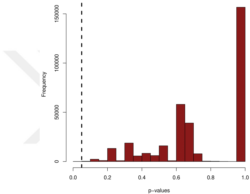
Figure 4.6: Histogram of P -values. The dashed line shows P less than 0.05. The P -value distribution is not continuous because of our limited sample size and the test being rank-based.
