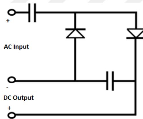
Figure 2.8 Villard Cascade Circuit
