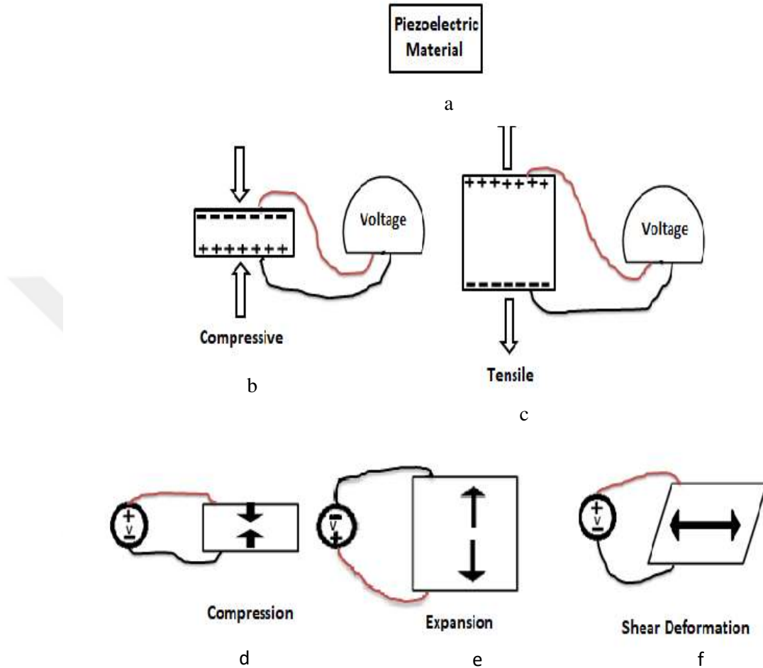
Figure 1.4. Behavior of piezoelectric material
