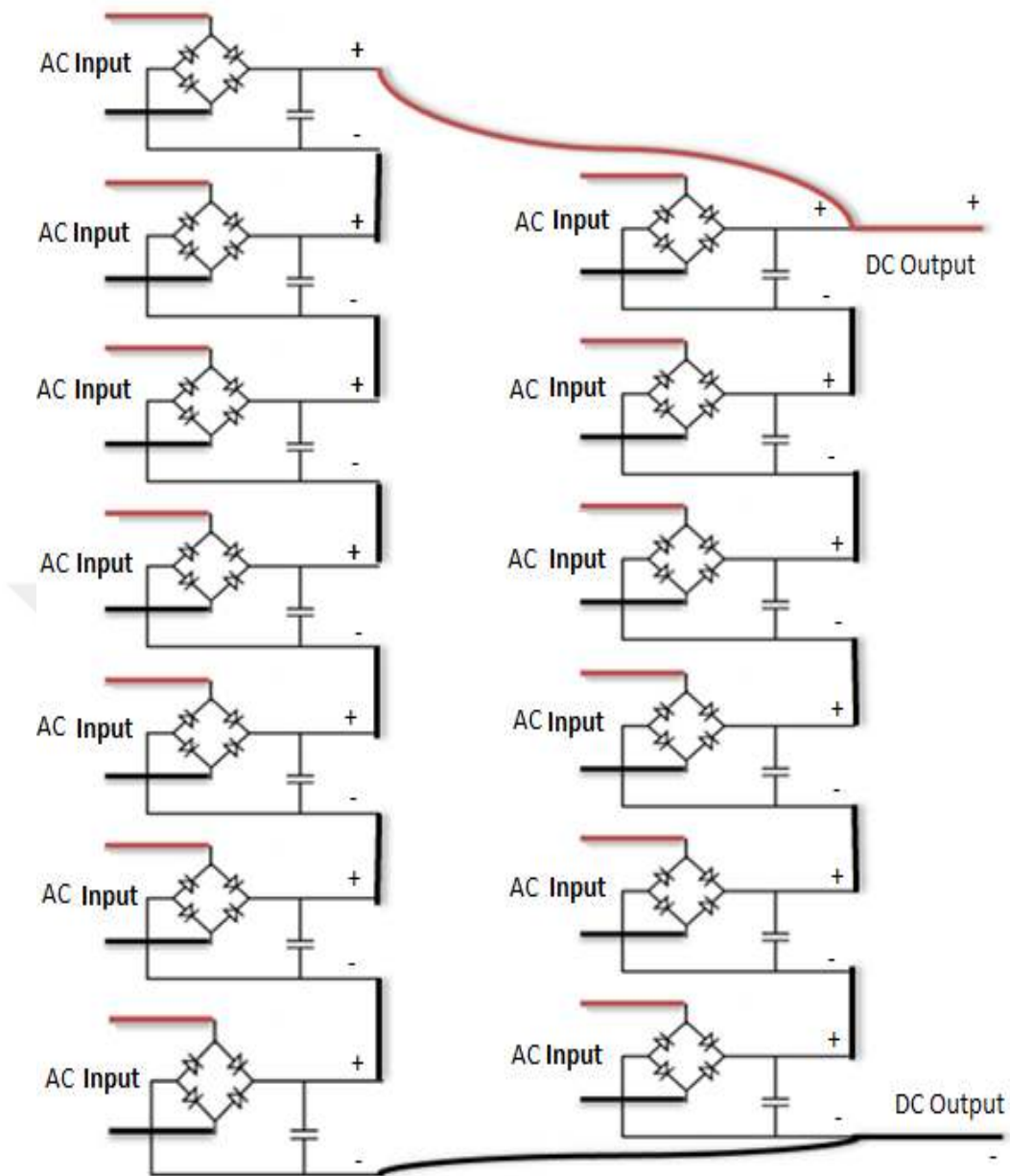
Figure 2.26. Parallel and serial connection of piezodisc outputs
