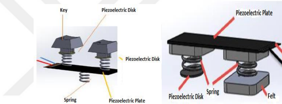
Figure 1.6 Keyboard design with piezoelectric materials (Şenyürek and Demetgül, 2015)
