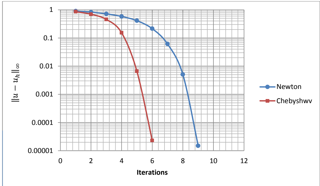
Figure 4.4: Comparison of the Convergency between (NM) and CM) Using 5-Point Scheme with h=1/16 .
