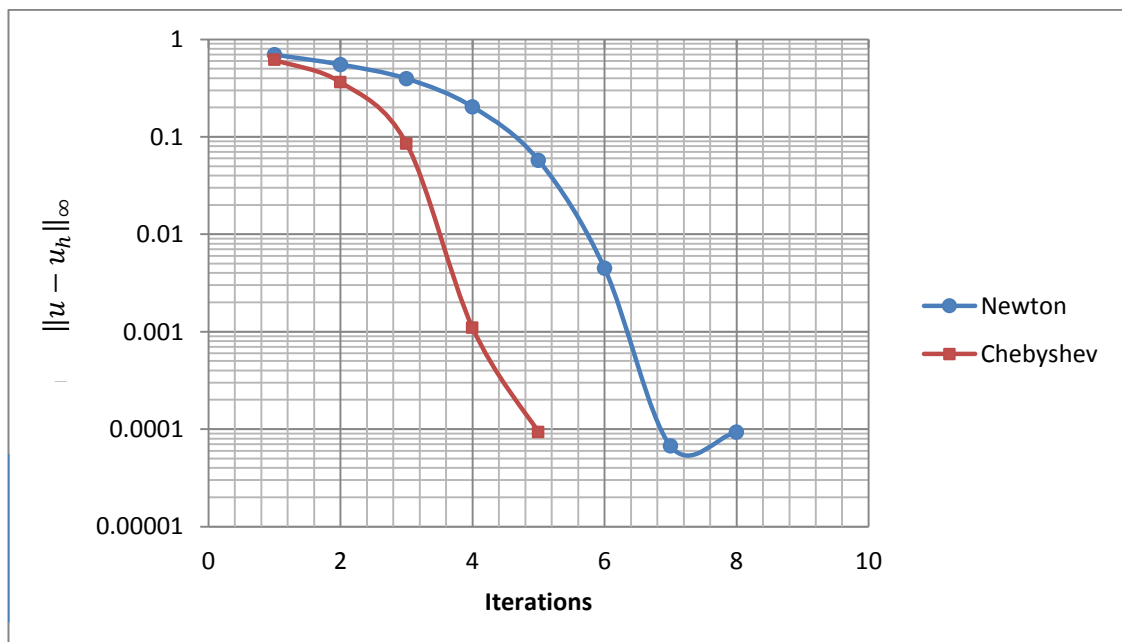
Figure 4.3: Convergence Comparison of (NM) and (CM) Using 5-Point Scheme with h=1/8 .
