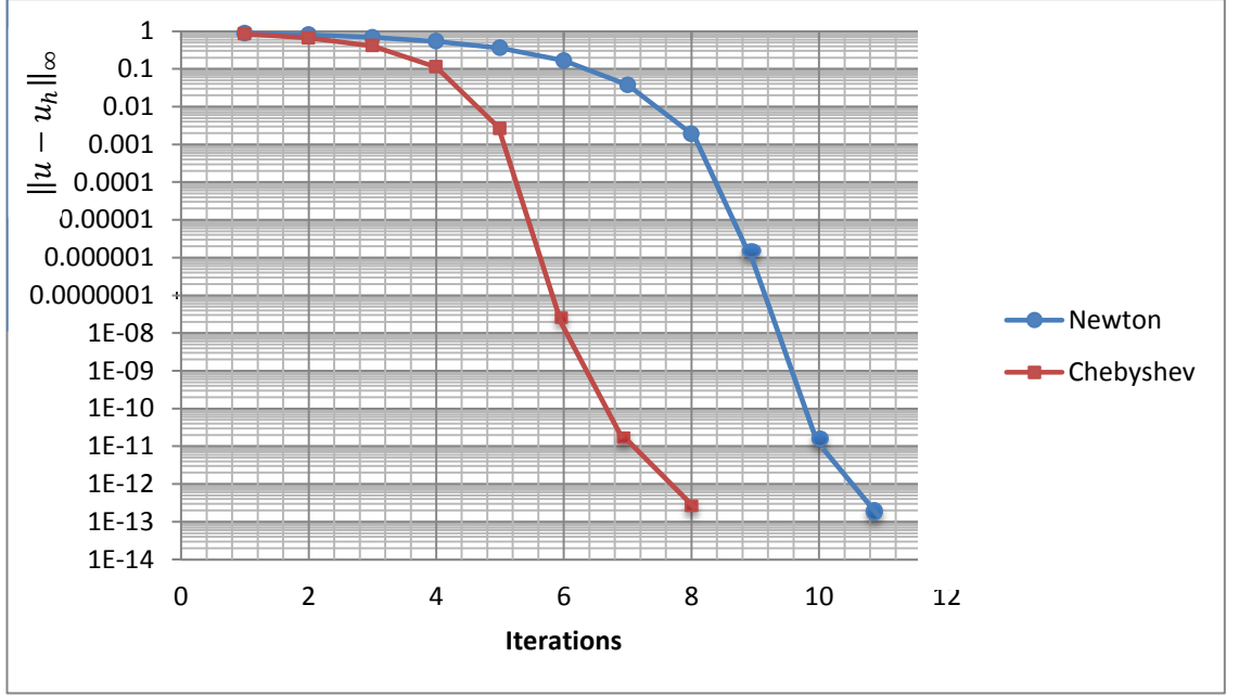
Figure 4.7: Convergence comparison of (NM) and (CM) Using 9-Point Scheme with h=1/16 .
