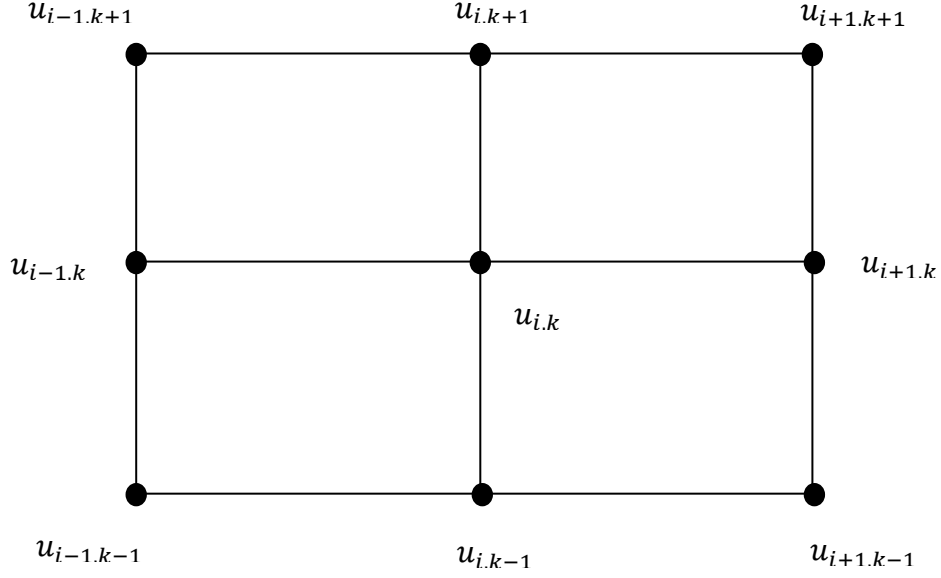
Figure 3.2: 9-Point Stencil.
