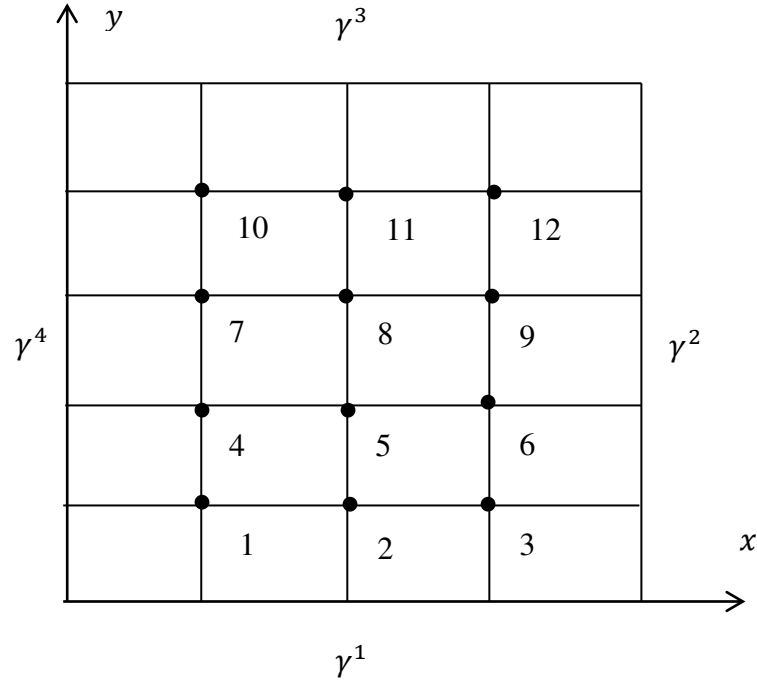
Figure 3.3: Lexicographical Ordering, for the case n_1 = 4 and n_2 = 5 .
