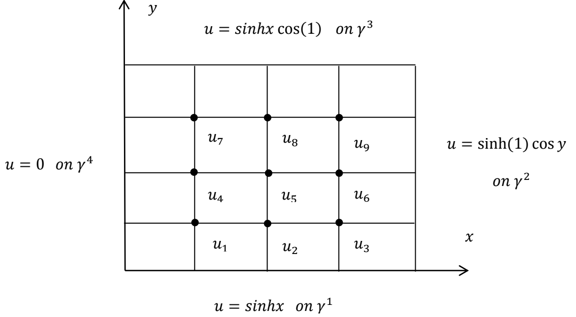
Figure 4.1: The Model Problem and Representation of Inner Grids for h=1/4 .
