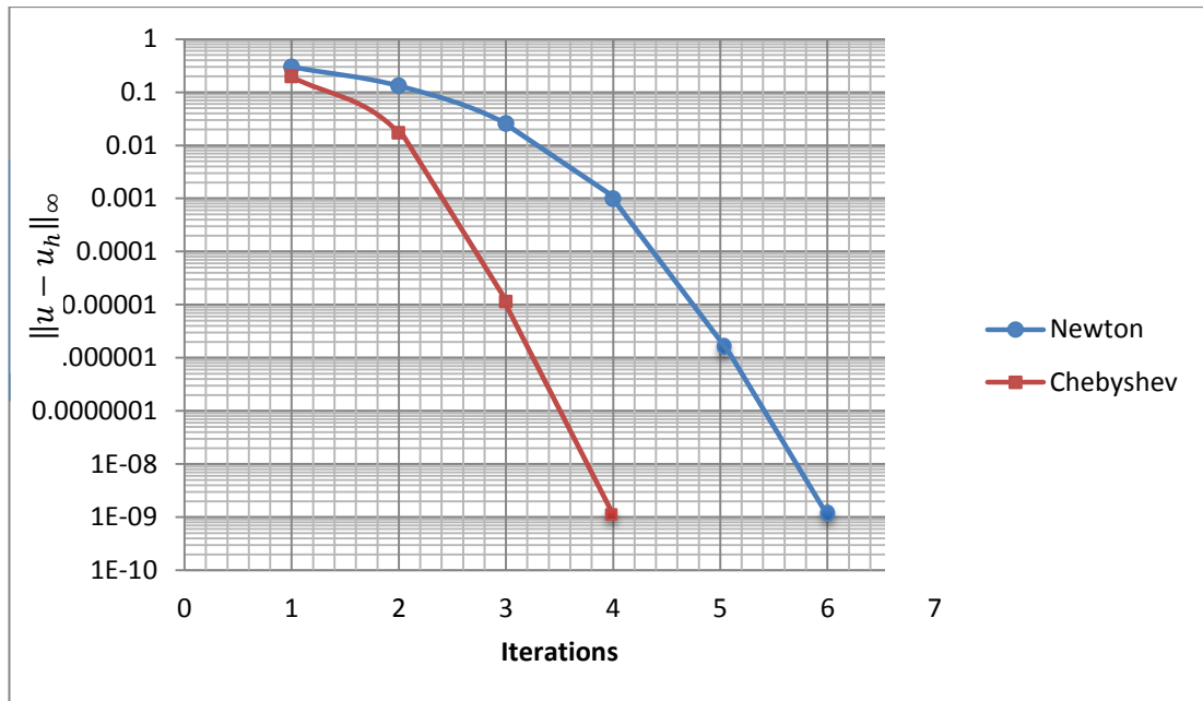
Figure 4.5: Convergence Comparison of (NM) and (CM) Using 9-Point Scheme with h=1/4 .
