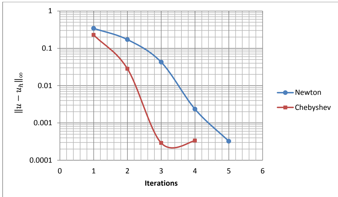
Figure 4.2: Comparison of the Convergence of (NM) and (CM) Using 5-Point Scheme for h=1/4 .
