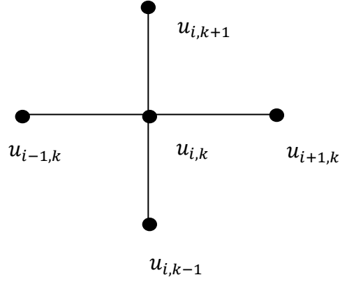
Figure 3.1: 5-Point Stencil.
