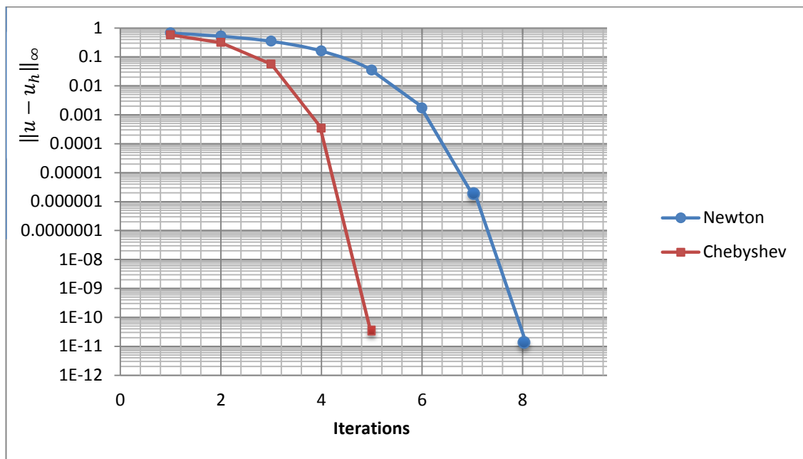
Figure 4.6: Convergence comparison of (NM) and (CM) Using 9-Point Scheme with h=1/8 .
