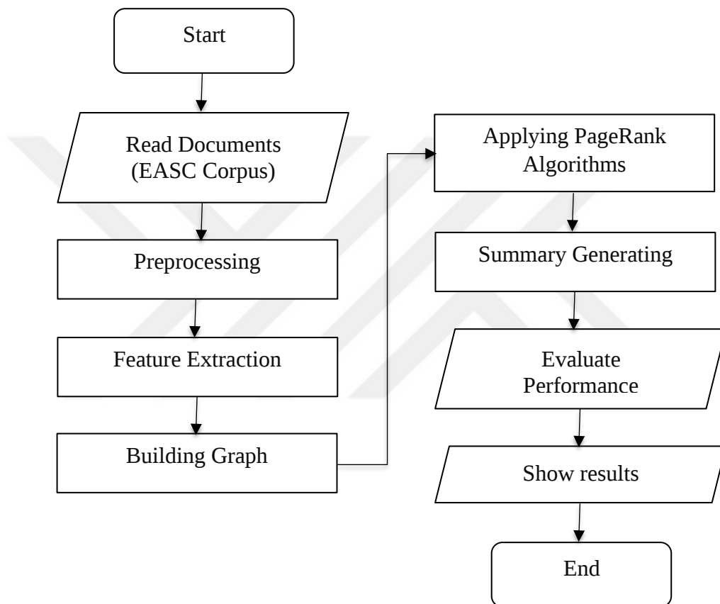
Figure 5.1. The flow chart of the GEATS approach
