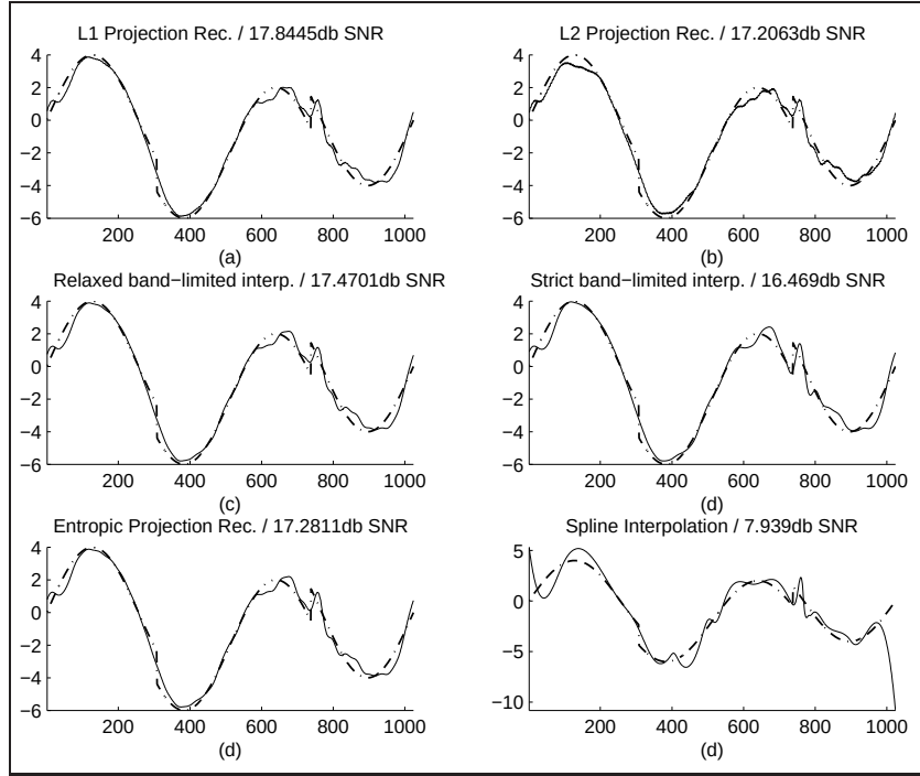
Figure 4.2: (i) 32 point irregularly sampled version of the Heavisine function and the original noisy signal ( \sigma = 0.5 ). (ii) The 1024 point interpolated versions of the function given at (i) using different interpolation methods.
