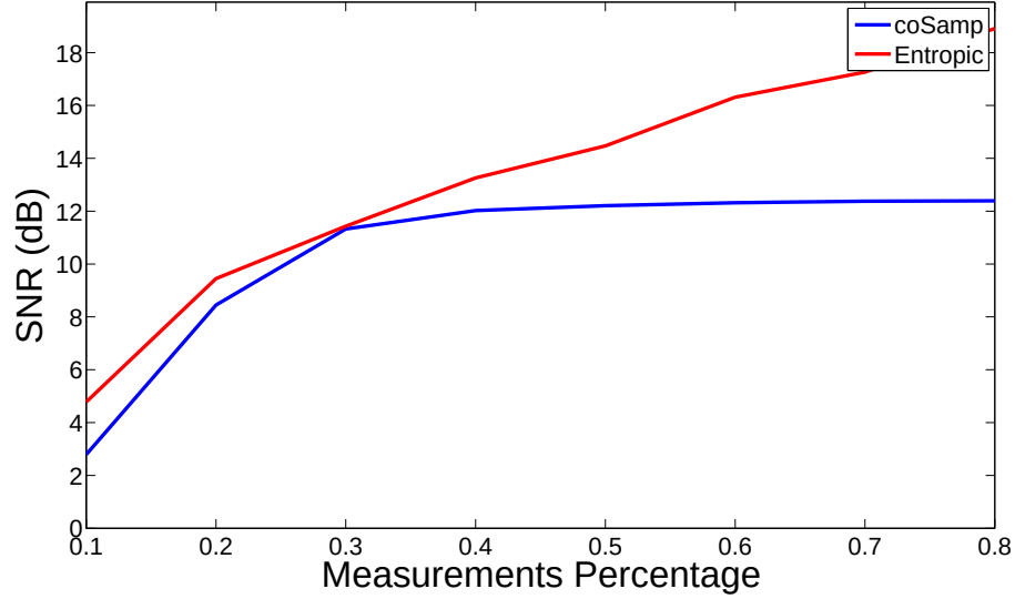
Figure 4.20: The reconstruction error for a hisine signal with N = 256 samples.
