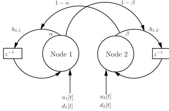
(a) ATC diffusion adaptation scheme
