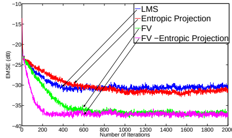
Figure 6.9: EMSE comparison between LMS and Entropic projection based adaptation schemes in Algorithm 1. Node topology shown in Fig. 6.7 (b) under \varepsilon -contaminated Gaussian, is used in the experiment. The noise parameters are given in Tables 6.1 and 6.3
