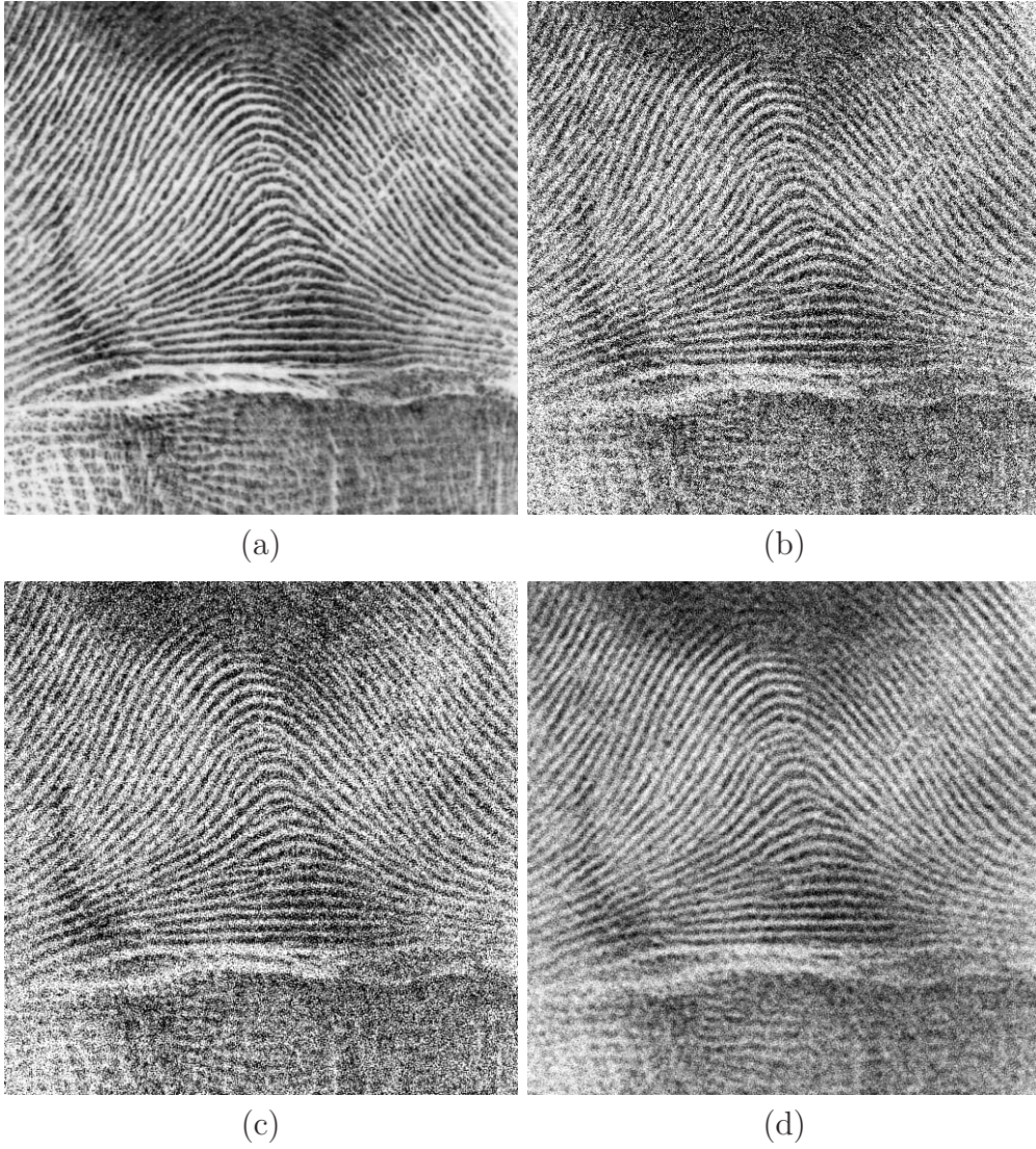
Figure 5.5: (a) Original fingerprint image, (b) fingerprint image with AWGN (SNR = 4.9 dB). (c) Image restored using the TV constraint (SNR=7.45dB). (d) Image restored using the proposed algorithm using C_2 , C_4 and C_5 (SNR=12.75 dB)
