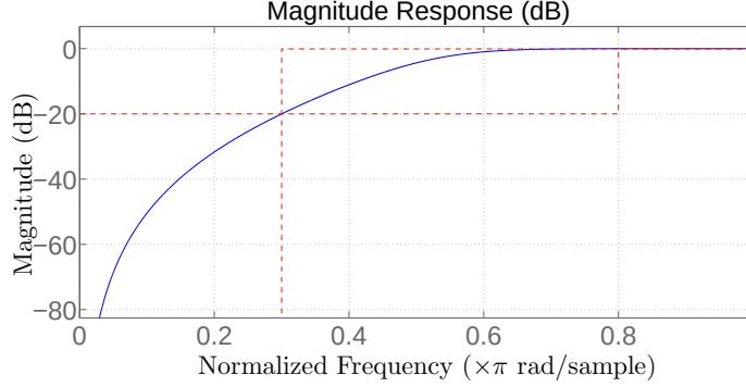
Figure 3.2: An example high pass filter with exponentially decaying transition band.
