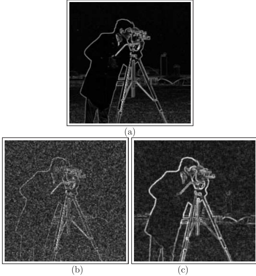
Figure 5.1: TV images of (a) original, (b) noisy, and (c) low-pass filtered noisy Cameraman images. All images are rescaled in [0, 1] interval.
