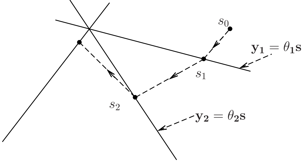
Figure 4.13: Geometric interpretation of the entropic projection method: Sparse representation \mathbf{s}_i corresponding to decision functions at each iteration are updated so as to satisfy the hyperplane equations defined by the measurements y_i and the measurement vector \theta_i . Lines in the figure represent hyperplanes in \mathbb{R}^N . Sparse representation vector s_i converges to the intersection of the hyperplanes. Notice that D-projections are not orthogonal projections.
