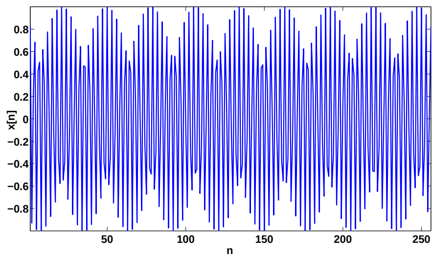
Figure 4.16: Hisine signal with N = 256 samples
