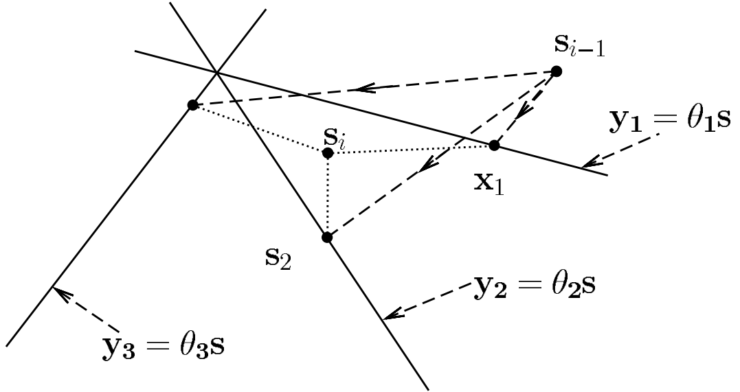
Figure 4.14: Geometric interpretation of the block iterative entropic projection method: Sparse representation s_i corresponding to decision functions at each iteration are updated by taking individual projections onto the hyperplanes defined by the lines in the figure and then combining these projections. Sparse representation vector s_i converges to the intersection of the hyperplanes. Notice that D-projections are not orthogonal projections.
