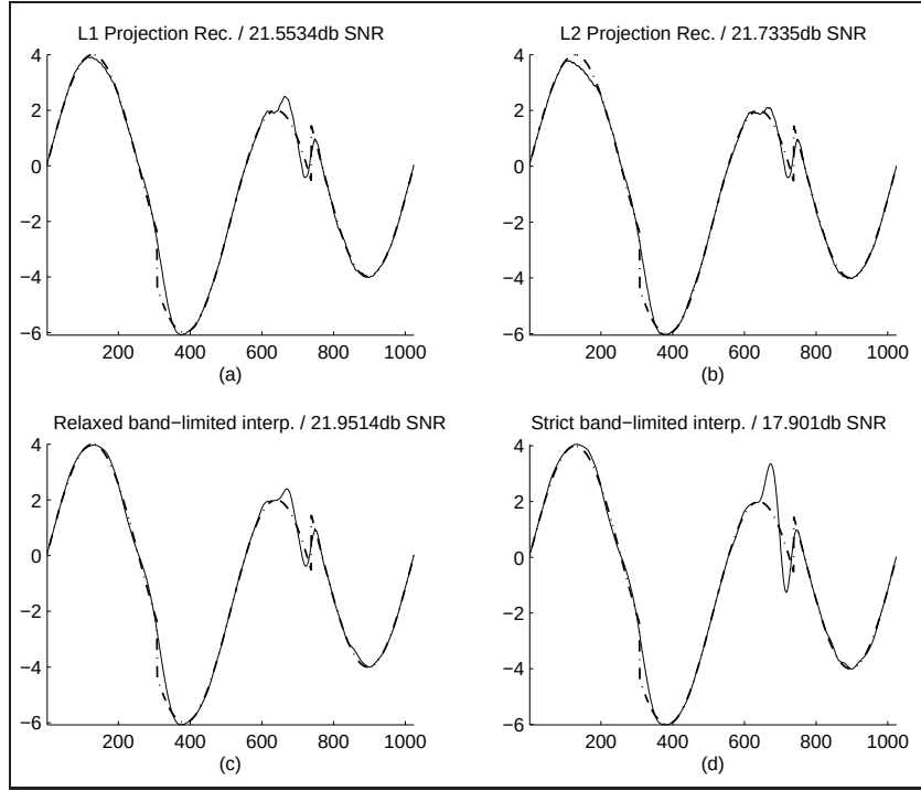
Figure 4.3: (i) 32 point irregularly sampled version of the Heavisine function and the original noiseless signal. (ii) The 1024 point interpolated versions of the function given at (i) using different interpolation methods.
