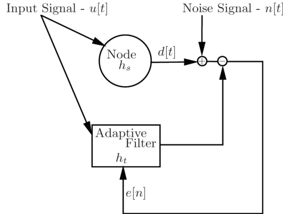
Figure 6.1: Adaptive filtering algorithm for the estimation of the impulse response of a single node.
