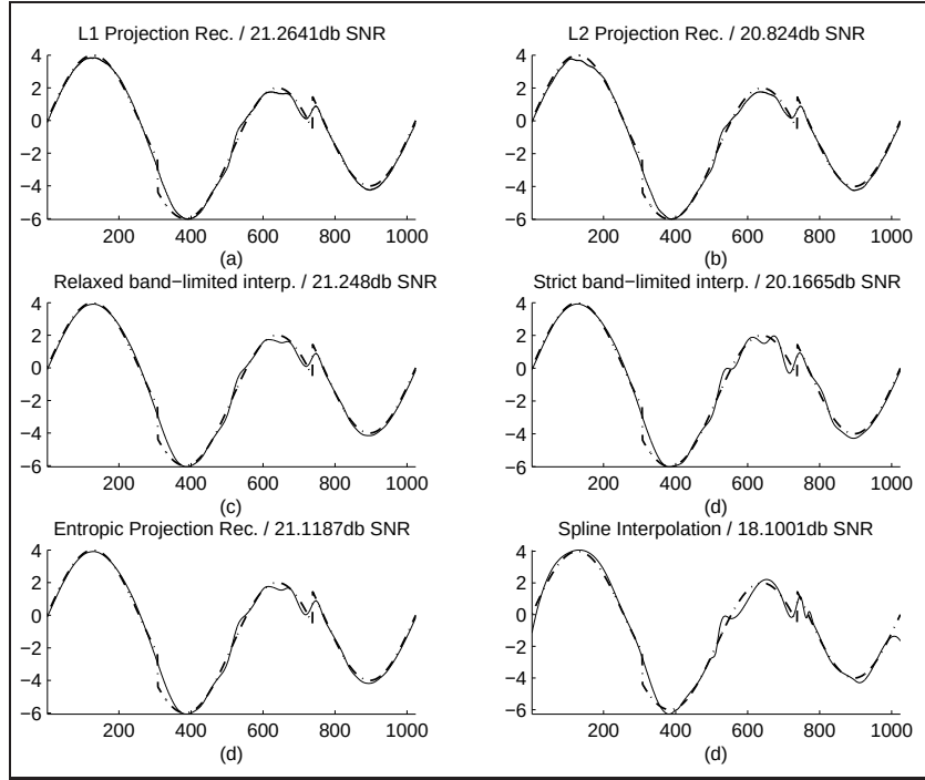
Figure 4.1: (i) 32 point irregularly sampled version of the Heavisine function and the original noisy signal ( \sigma = 0.2 ). (ii) The 1024 point interpolated versions of the function given at (i) using different interpolation methods.
