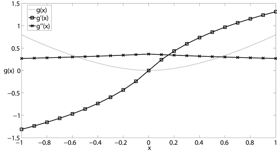
Figure A.1: The plot of the entropic cost function, its first, and second derivatives.
