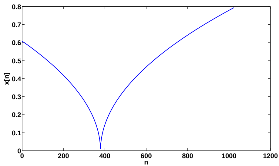
Figure 4.15: The cusp signal with N = 1024 samples
