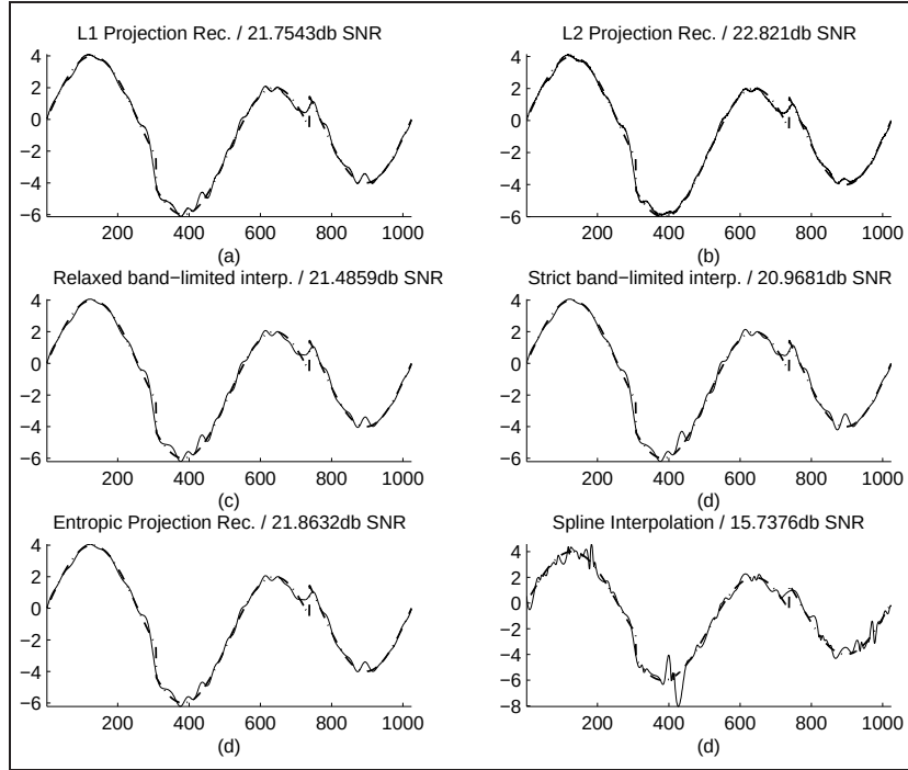
Figure 4.5: (i) 128 point irregularly sampled version of the Heavisine function and the original noisy signal ( \sigma = 0.2 ). (ii) The 1024 point interpolated versions of the function given at (i) using different interpolation methods.
