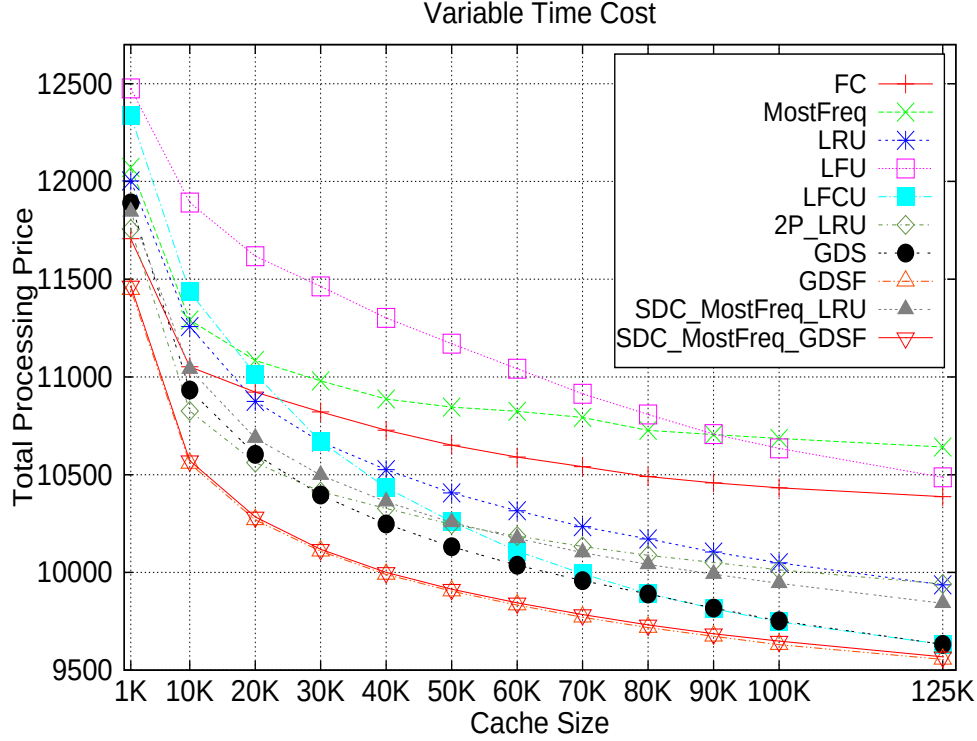
Figure 5.2: Financial cost evaluation of caching policies assuming variable query processing time costs.
