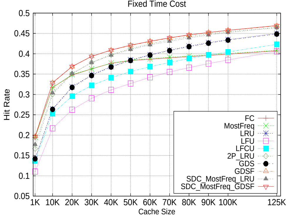
Figure 5.5: Hit rates of caching policies assuming fixed query processing time costs.
