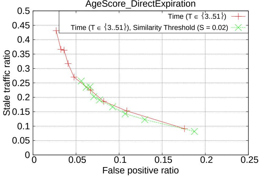
Figure 4.2: Stale traffic and false positive ratios for AgeScore_DirectExpiration Algorithm.
