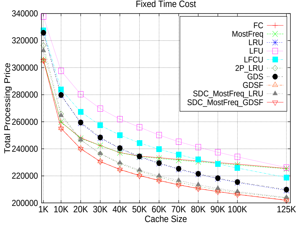
Figure 5.4: Financial cost evaluation of caching policies assuming fixed query processing time costs.
