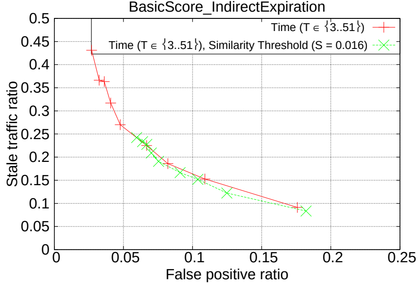
Figure 4.3: Stale traffic and false positive ratios for BasicScore_IndirectExpiration Algorithm.
