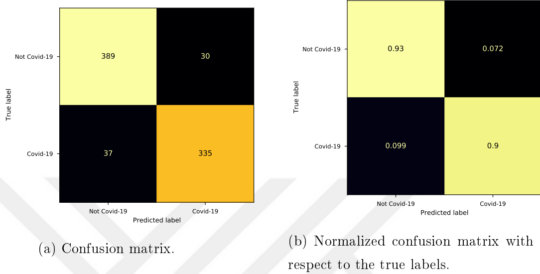
Figure 3.18: The binary classification performance results of the artificial intelligence-based hybrid clinical decision support technique on the test set, where the two classes are COVID-19 and Not COVID-19.
