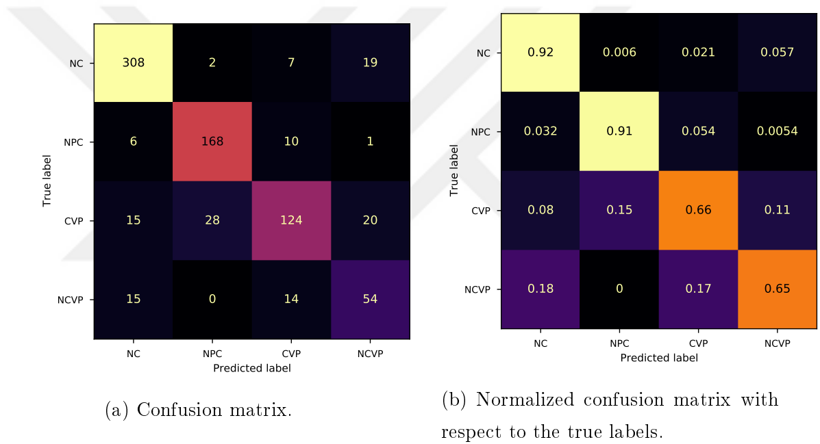
Figure 3.17: The multi-class classification performance results of the artificial intelligence-based hybrid clinical decision support technique on the test set, where the four classes are COVID-19 pneumonia (CVP), non-pneumonia COVID-19 (NPC), non-COVID-19 pneumonia (NCVP), and not COVID-19 (NC).
