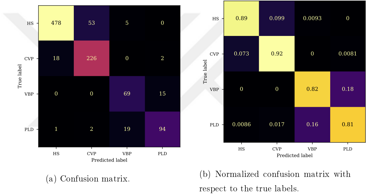
Figure 3.14: Multi-class classification performance results of the BCDU-Net and 3D-convolutional neural network classifier on the test set, where the four classes are COVID-19 pneumonia (CVP), other viral and bacterial pneumonias (VBP), parenchymal lung diseases (PLD), and healthy subjects (HS).
