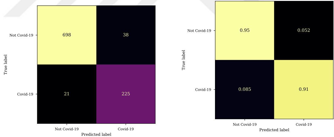
(b) Normalized confusion matrix with respect to the true labels.
