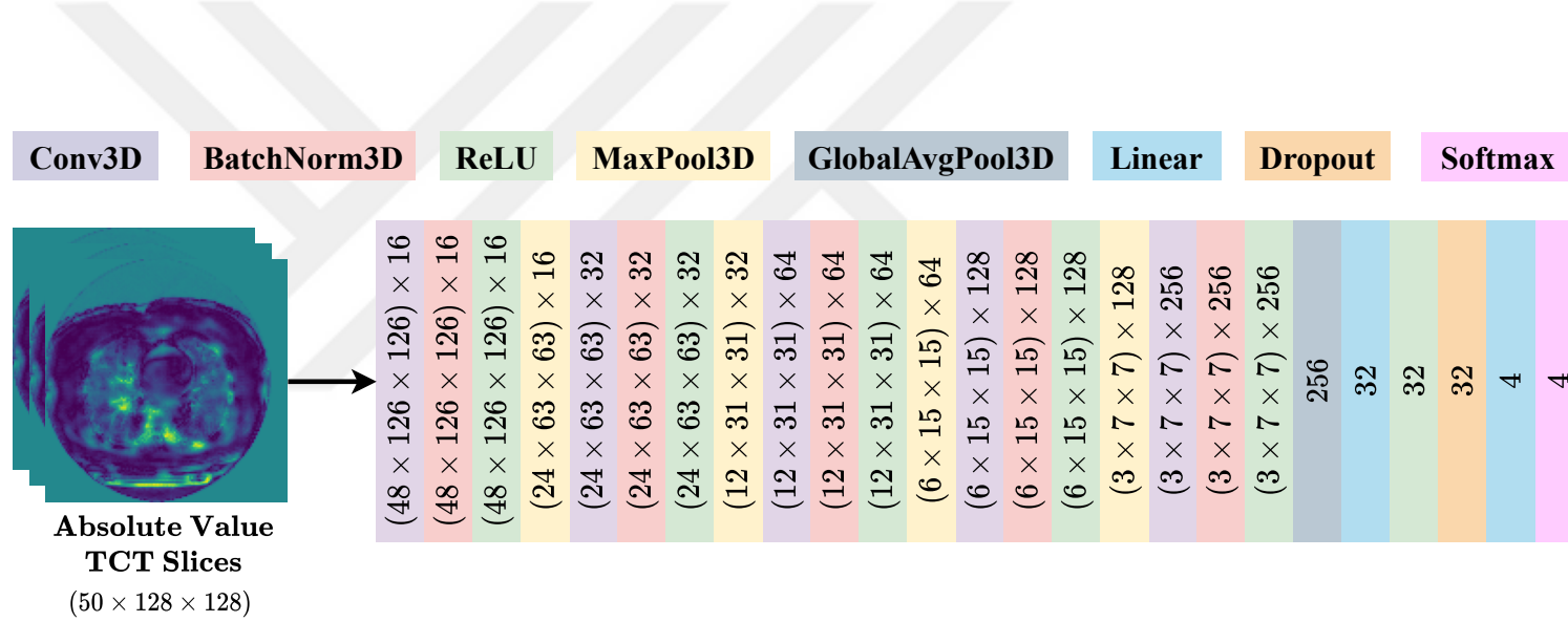
Figure 3.8: The proposed 3D-convolutional neural network classifier that performs multi-class classification for COVID-19 diagnosis using thorax computed tomography images in the AUFM-CoV database. The numbers outside the parentheses in the 3D-convolutional neural network classifier represent the number of channels. The classifier successfully differentiates COVID-19 pneumonia (CVP) from other viral and bacterial pneumonias (VBP), parenchymal lung diseases (PLD), and healthy subjects (HS), where the first three have very similar radiological findings.
