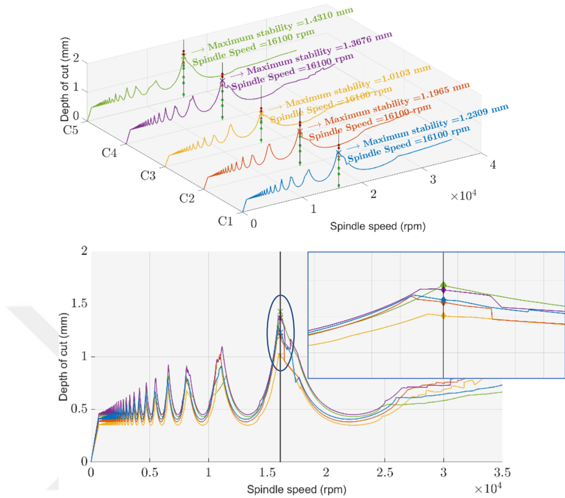
Figure 4-2: Consideration of configuration & dependent stability predictions & shifts in maximum stability at 16100 rpm
