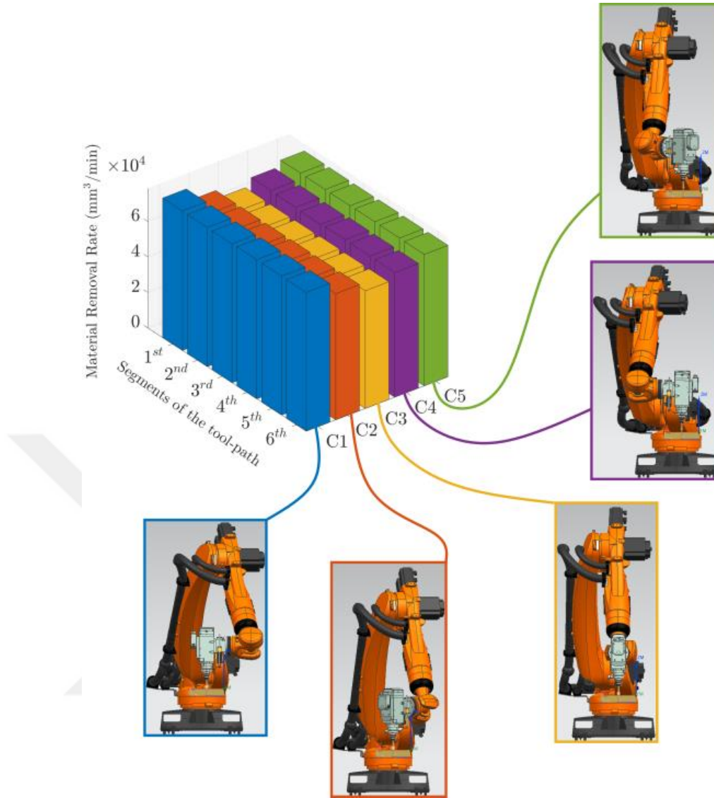
Figure 4-6: Material Removal comparison in Y direction
