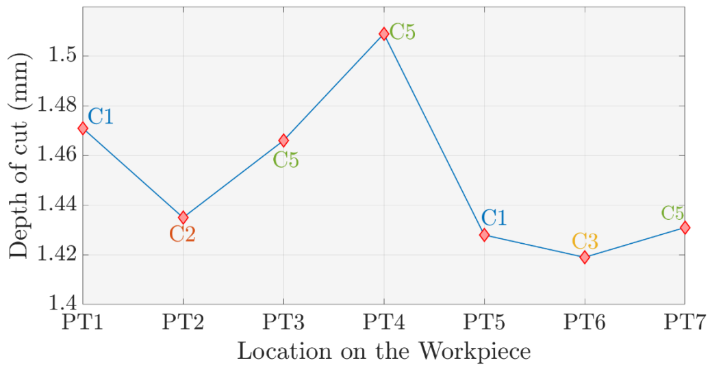
Figure 4-7: Configuration identification based on maximum stability in X direction Maximum depth of cuts is sorted into 1.471 mm, 1.435 mm, 1.466 mm, 1.509 mm, 1.428 mm, 1.419 mm and 1.431 mm, respectively. Limiter depth of cut for constant depth cutting operation is identified as 1.419 mm which corresponds to location at PT6. In this configuration structure, three different reductions and a huge increment observed among
