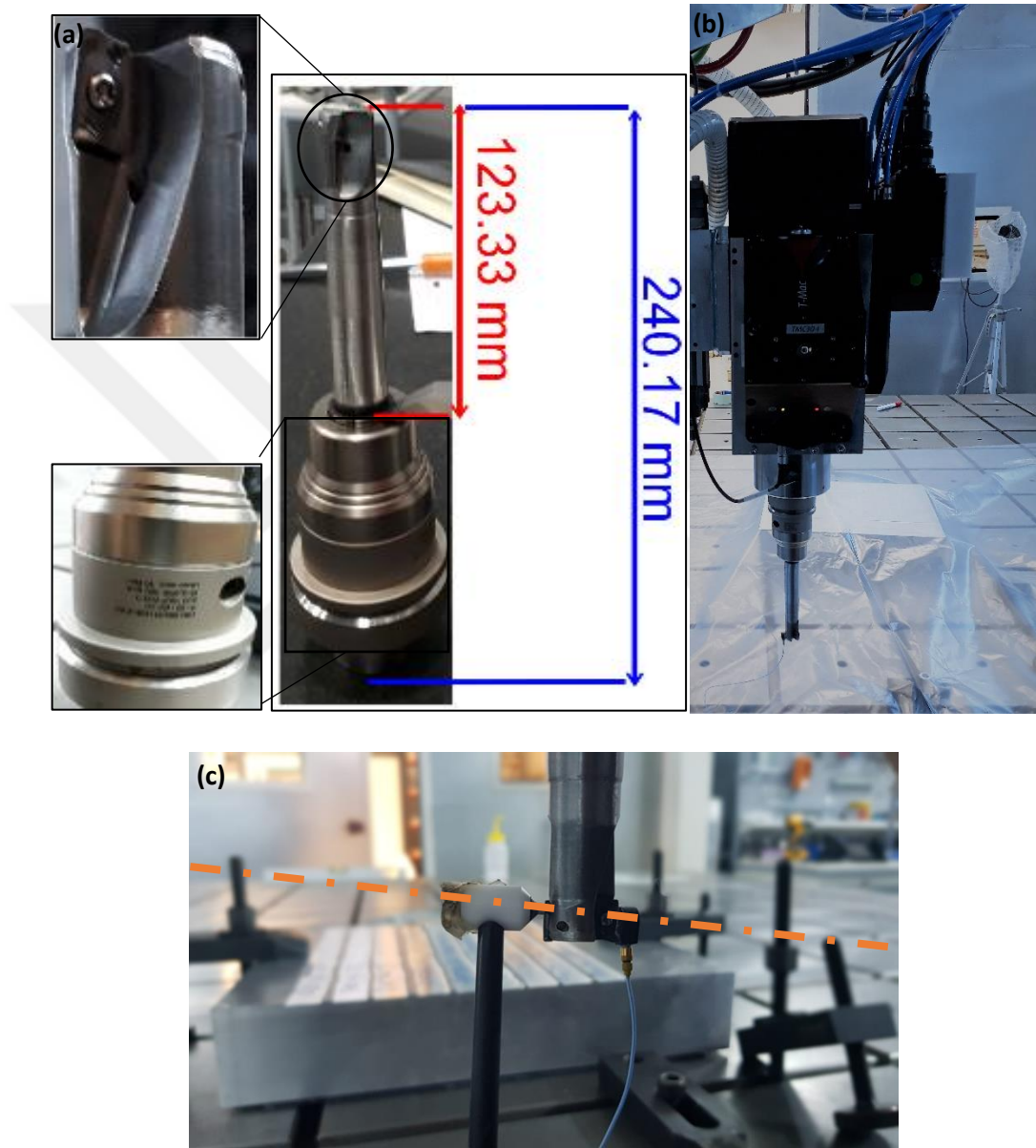
Figure 3-8: (a)Indexable milling tool with inserts and length properties, (b) milling tool, accelerometer and spindle representation (c) alignment of the accelerometer and mini-modal hammer position
