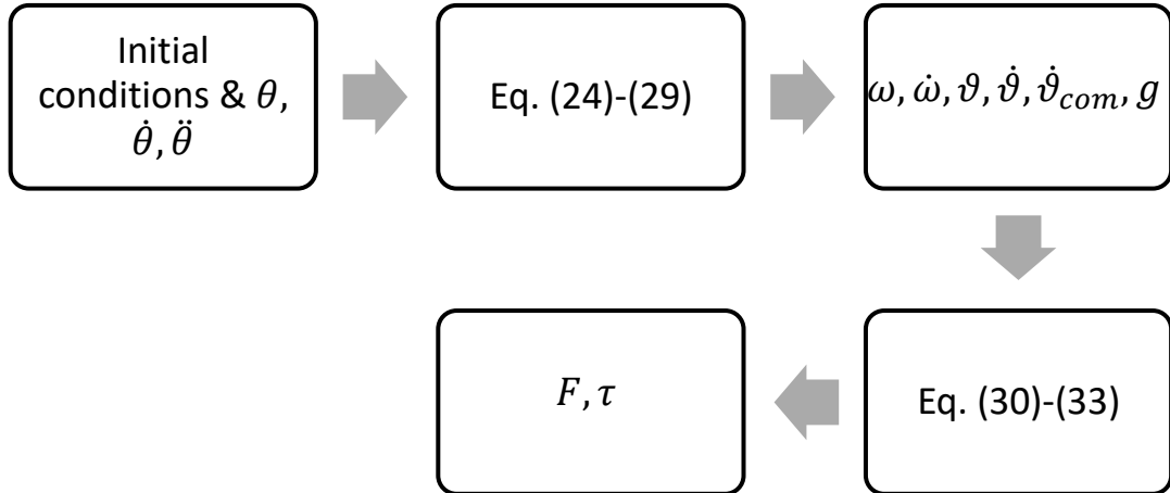
Figure 2-6:Computational mechanism of the Recursive Newton-Euler formulation
