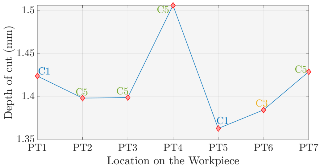
Figure 4-9: Configuration identification based on maximum stability along the tool path at 16100 rpm
