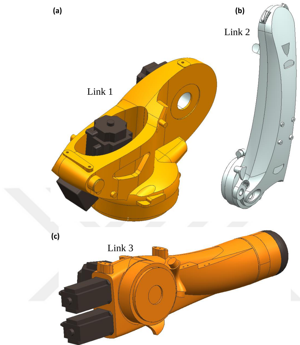
Figure D-8: Link representation and dynamic parameters from CAD data -NX ® (a) Link 1, (b) Link 2, (c) Link 3
