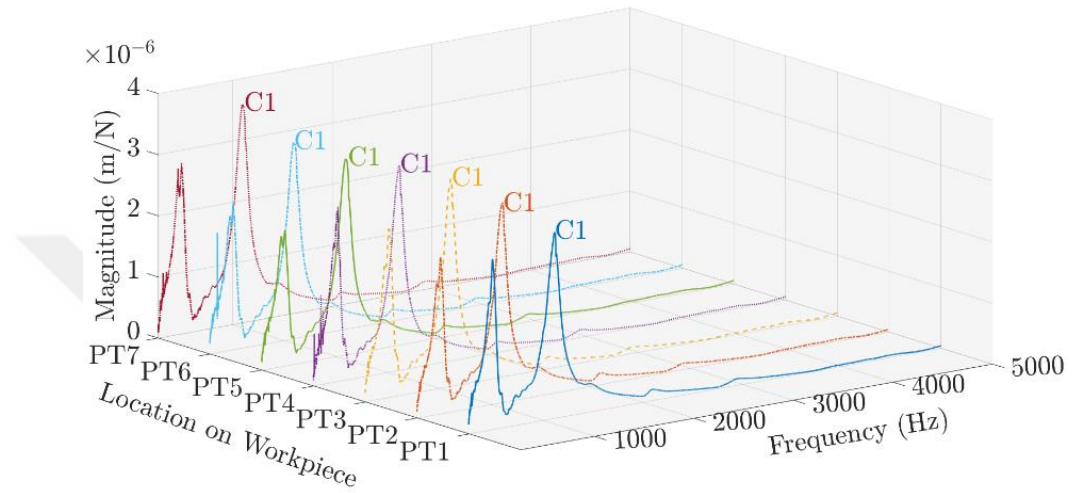
Figure 3-12: Representative positional dependency and accompanying tool mode shifts Two significant modes are observed contributed by tool and tool holder around 500 Hz and 1100 Hz. The variation of tool modes in terms of natural frequency and magnitude are shown in Figure 3-13.
