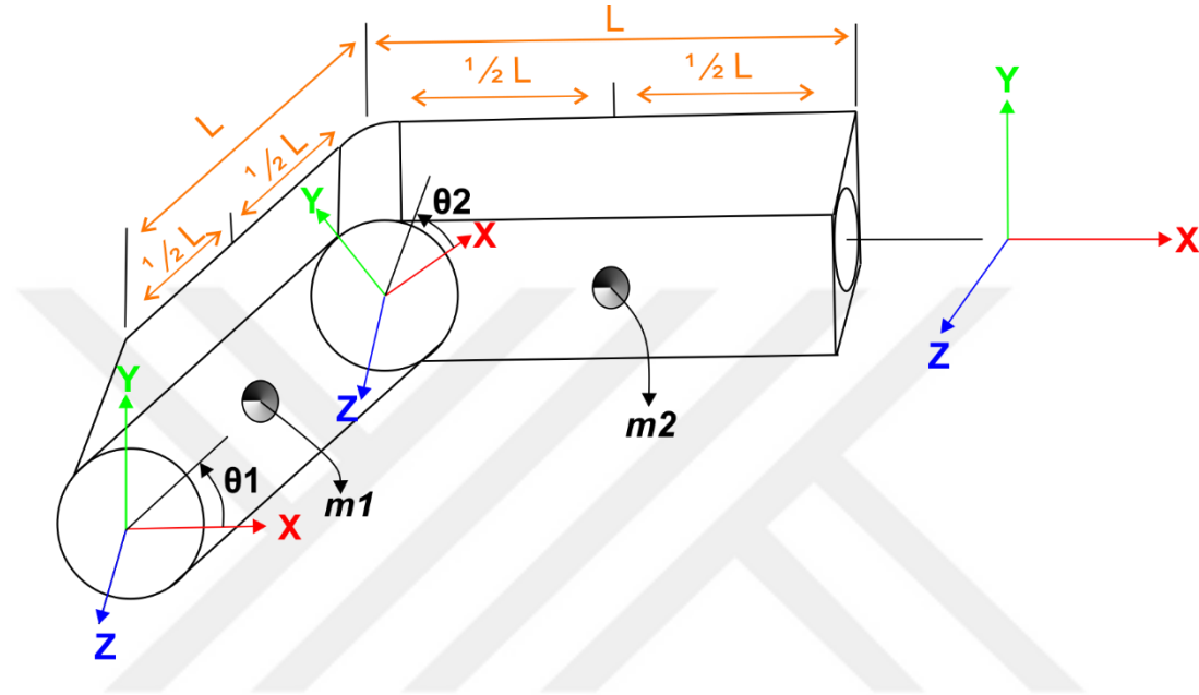
Figure 2-8: Simplified 2 DOF robot structure representation
