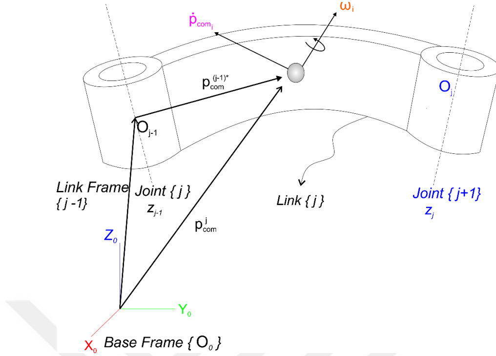
Figure 2-7: Representation of link j by geometrical and physical relations for Lagrangian approach
