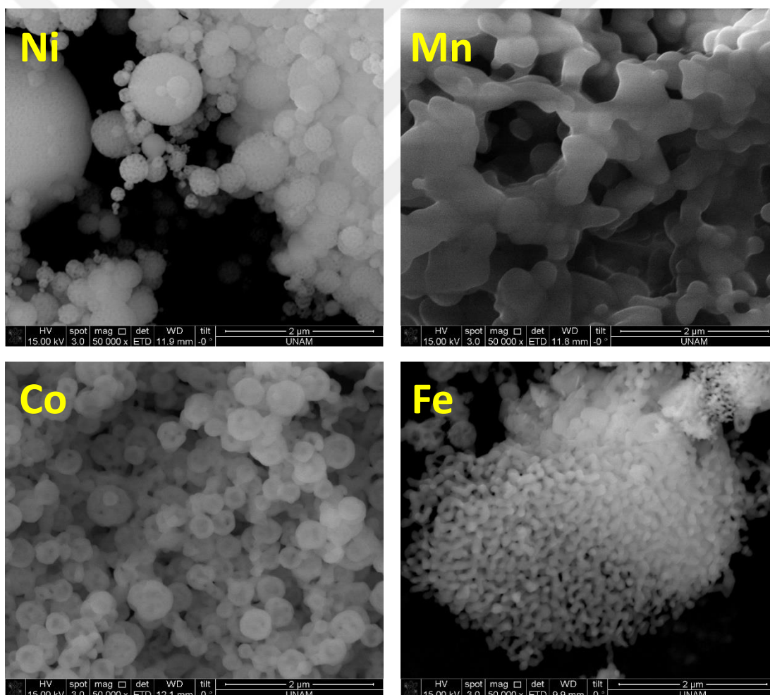
Figure 3.70. SEM images of LMP at 500 °C with scale bar 2 \mu\text{m}
