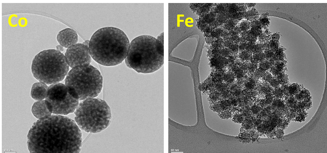
Figure 3.69. TEM images of LMP at 300 °C with scale bar 0.1 \mu\text{m} and 50 nm respectively.
