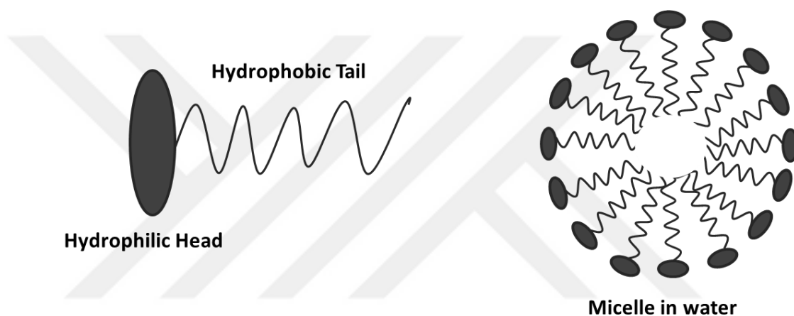
Figure 1.4. Schematic representation of surfactant and a cross-section of a micelle structure in water.
