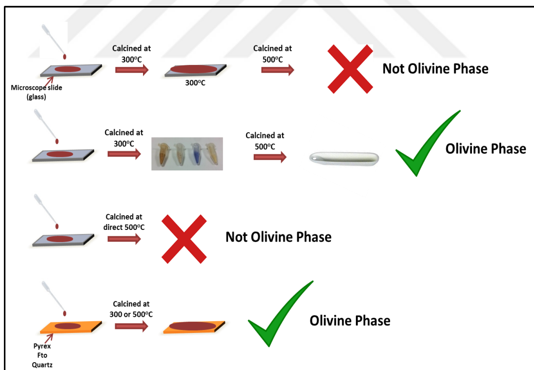
Figure 3.73. Schematic representation of new methodology for calcination steps.
