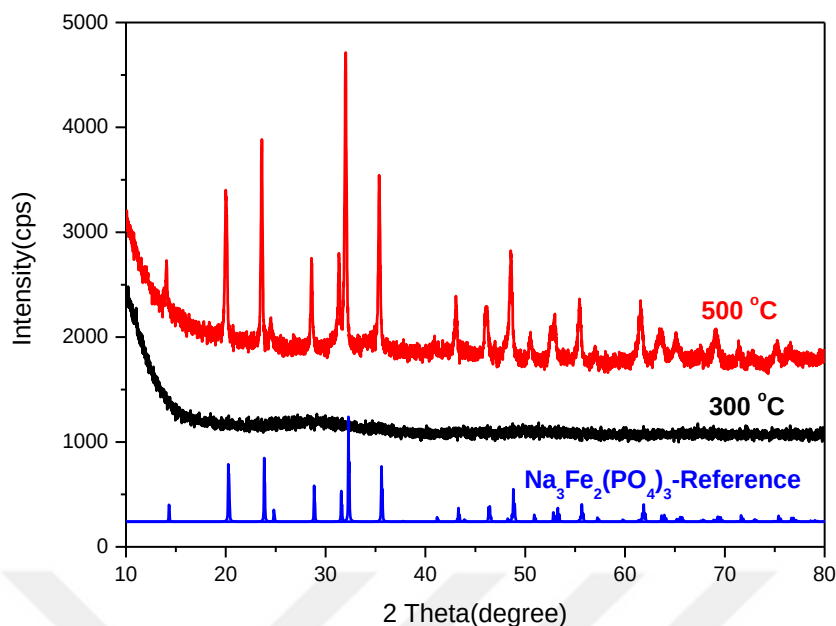
Figure 3.61. High angle XRD patterns of LFeP-60:40:60 sample at 300 and 500 °C and Na 3 Fe 2 (PO 4 ) 3 with PDF-card no 00-045-0319.
