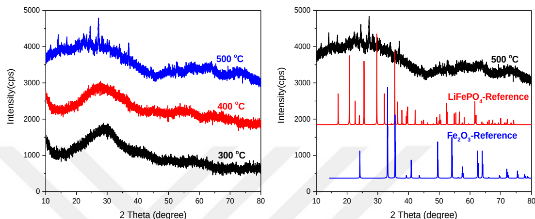
Figure 3.55. XRD patterns of LFeP-90 with \text{NO}_3^- salts (left) at different temperature, (right) at 500 °C and \text{LiFePO}_4 reference with PDF-card no 00-040-1499, and \text{Fe}_2\text{O}_3 reference with PDF-card no 00-033-0664.
