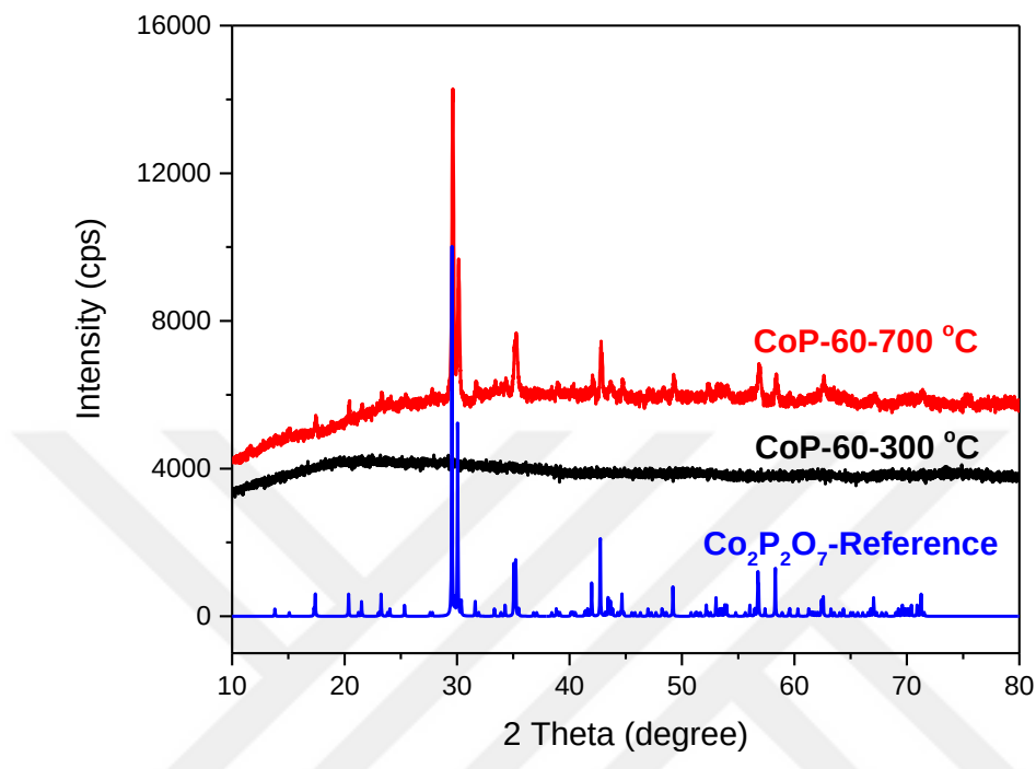
Figure 4.4. High angle XRD pattern of CoPP-60 at 300 and 700 °C and Co 2 P 2 O 7 reference with PDF card no 00-049-1091.
