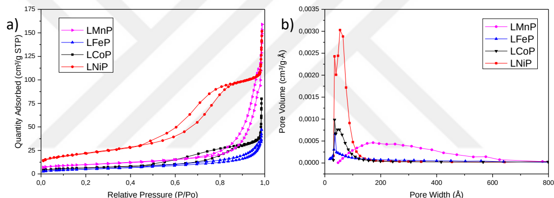
Figure 3.71. a) Linear isotherm plot and b) BJH pore size distribution of LMP for 300 °C.
