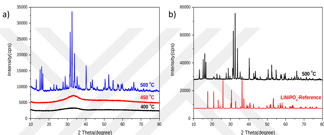
Figure 3.39. High angle XRD patterns of LNiP-90 a) at 400, 450, and 500 °C and b) 500 °C and \text{LiNiPO}_4 reference with PDF-card no 00-032-0578.
