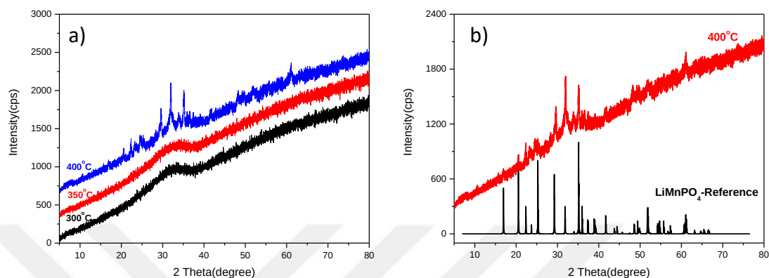
Figure 3.19. High angle XRD patterns of LMnP-90 a) at 300, 350, and 400 °C and b) at 400 °C and \text{LiMnPO}_4 reference PDF-card no 00-033-0804.
