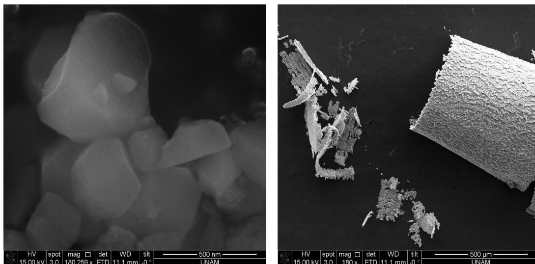
Figure 3.28. SEM images of LCoP-90 at room temperature.
