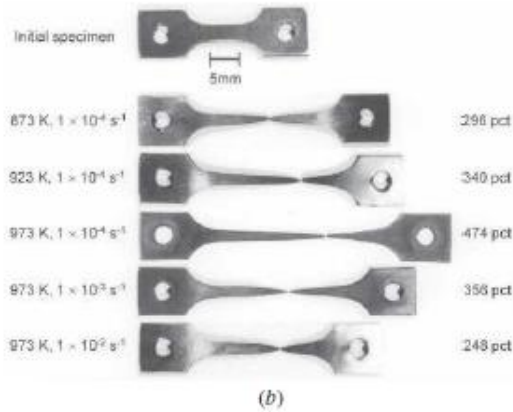
Figure 2.27 (a) True stress-strain curves of UFG Ti-6Al-4V (b) specimens tested at various conditions [98]
