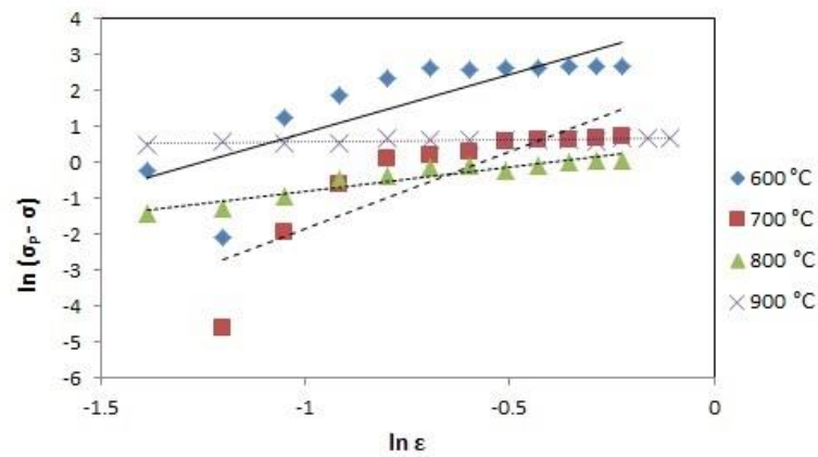
Figure 5.6 Relationship between \ln(\sigma_p - \sigma) and \ln(\epsilon) at various temperatures and at a strain rate of 0.001s^{-1}
