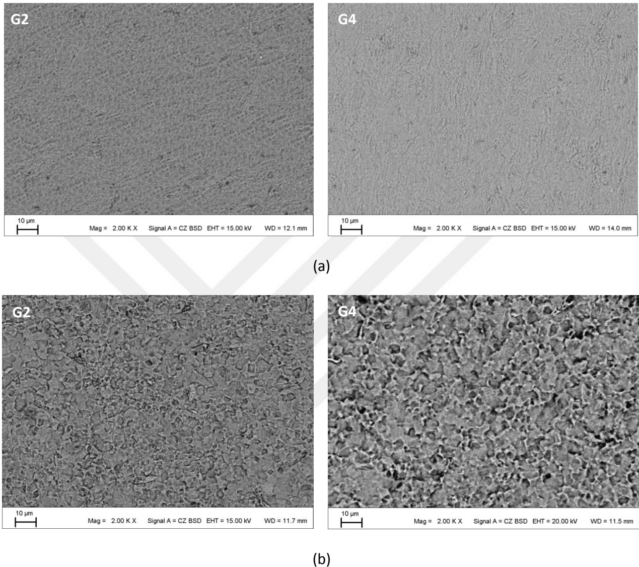
Figure 6.3 SEM images of grade 2 and 4 CP Ti on the flow plane after (a) 8 passes ECAE (b) 8 passes ECAE followed by heat treatment at 873K (600°C) for 3 minutes
