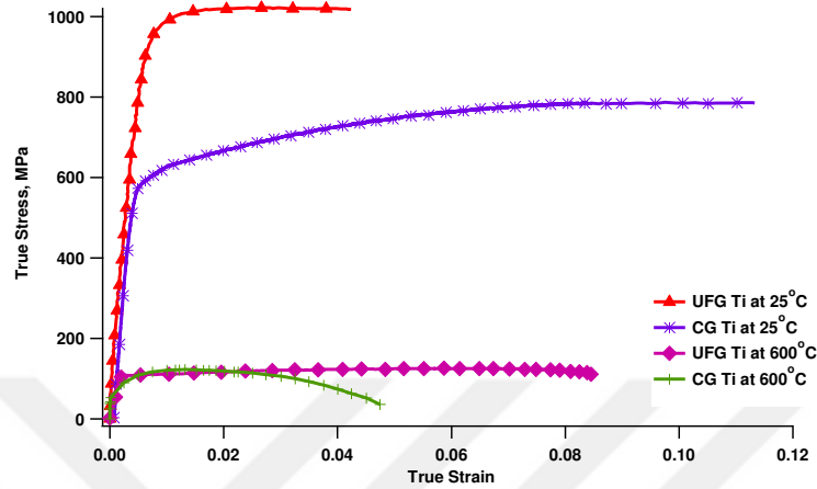
Figure 9.1 True stress–true strain response of CG and UFG Ti with strain rates of 0.01\text{s}^{-1} at 25^{\circ}\text{C} and at 600^{\circ}\text{C}
