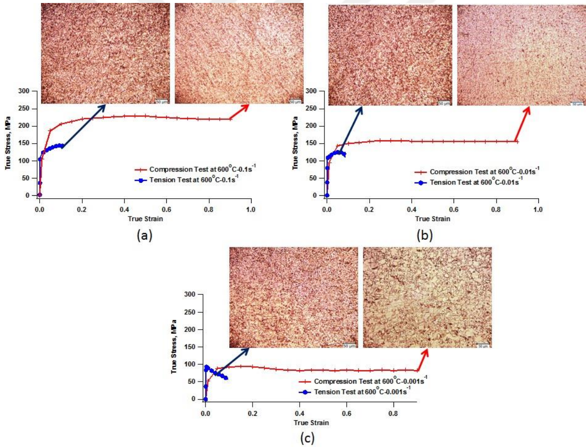
Figure 7.9 Tensile and compressive flow stresses with their corresponding microstructural features of severely deformed grade 4 titanium at 600°C and at strain rate of (a) 0.1\text{s}^{-1} (b) 0.01\text{s}^{-1} and (c) 0.001\text{s}^{-1}
