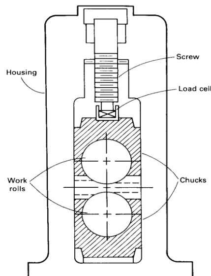
Figure 2.3 Conventional rolling mill stand [43]
