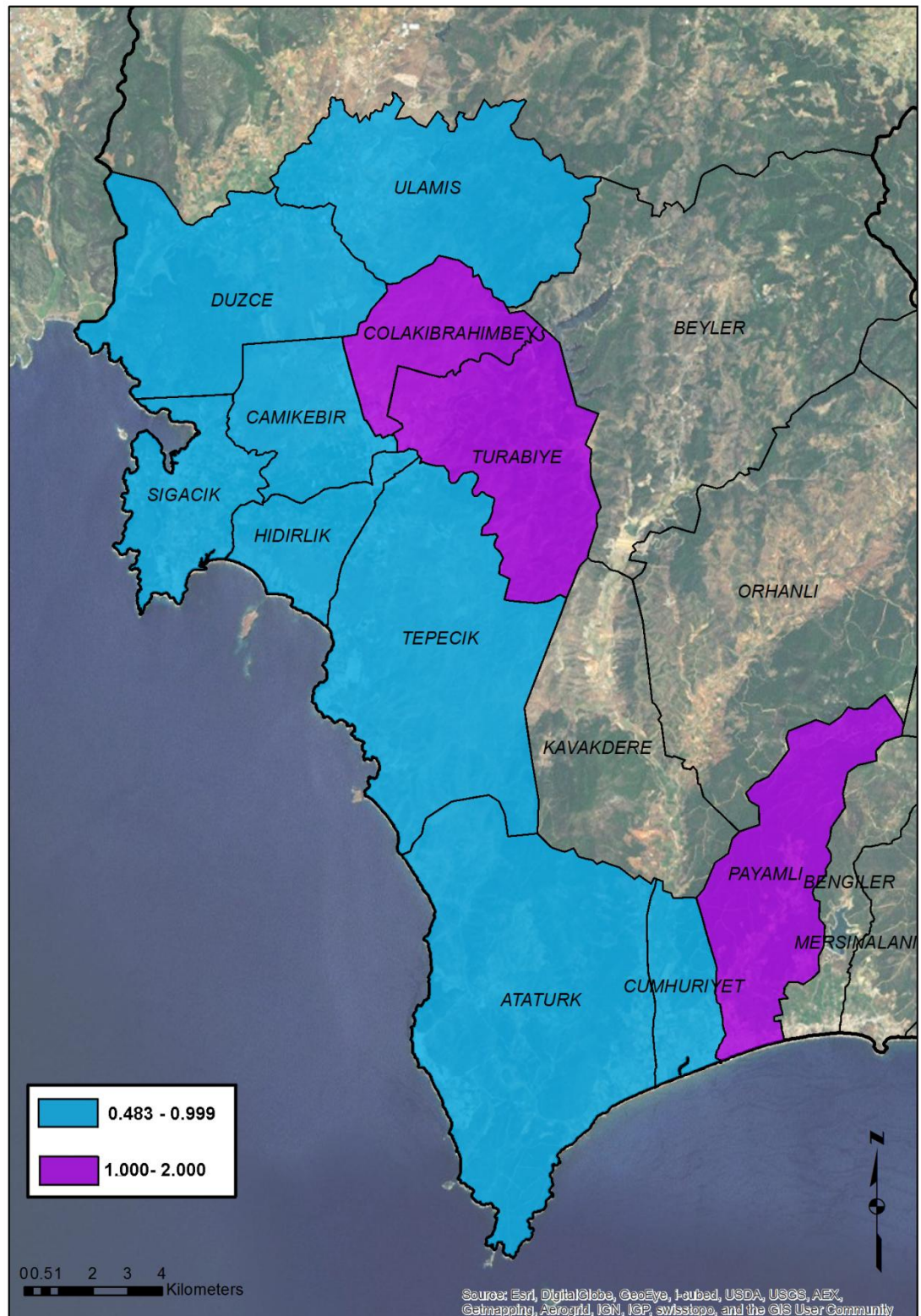
Figure 4.13 R-statistic values of euclidean distances method.
