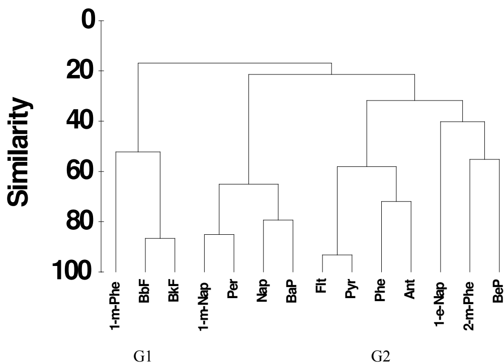
Figure 5.10 Hierarchical dendrogram for PAHs in Mullus barbatus from İzmir Bay
