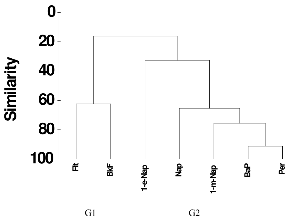
Figure 5.11 Hierarchical dendrogram for PAHs in Diplodus annularis from İzmir Bay
