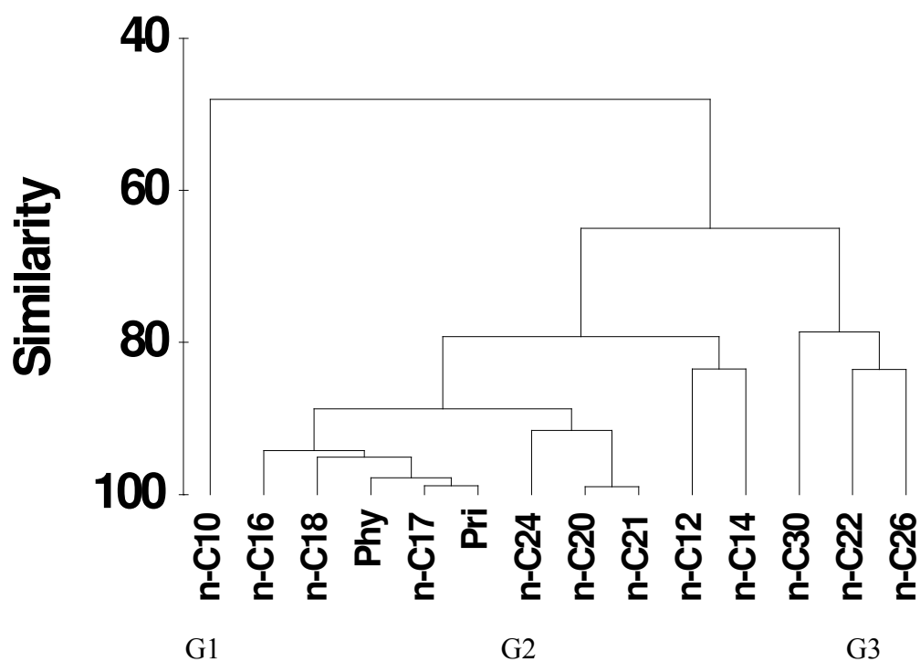
Figure 5.9 Hierarchical dendrogram for aliphatic hydrocarbons in Diplodus annularis from İzmir Bay
