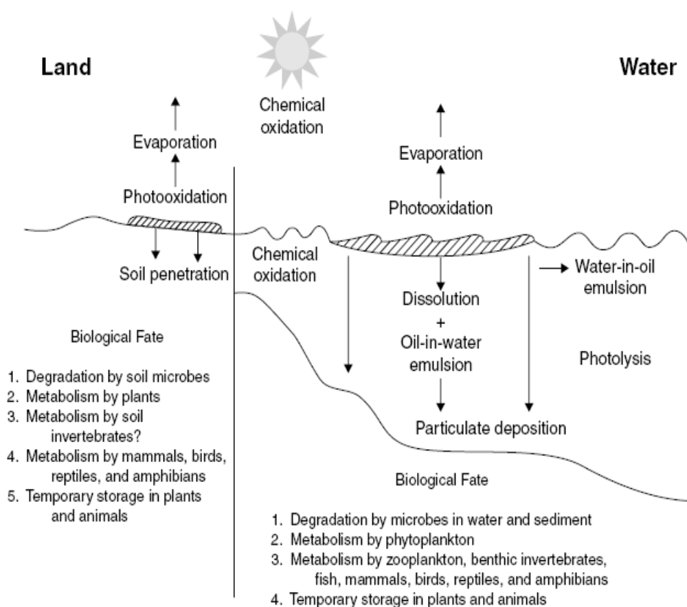
Figure 2.2 Chemical and biological fate of petroleum and PAHs in water and on land (Albers, 2003)
