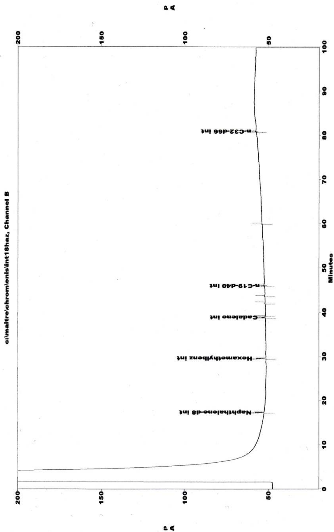
Figure 4.5 Chromatogram for internal standards
