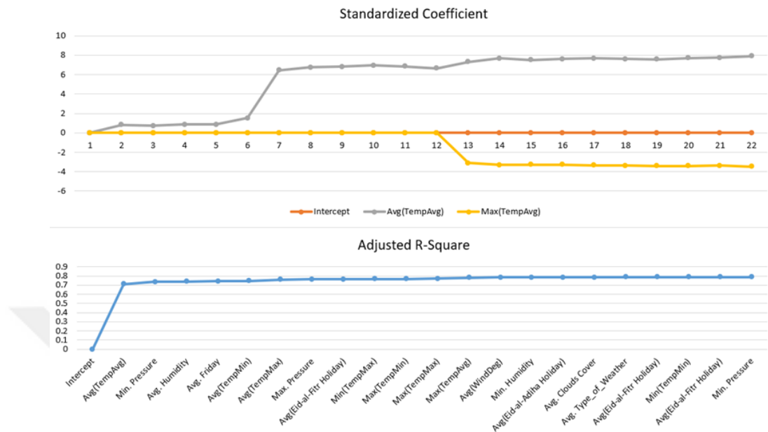
Figure 2.11. Fit Criteria for Load in Stepwise method
