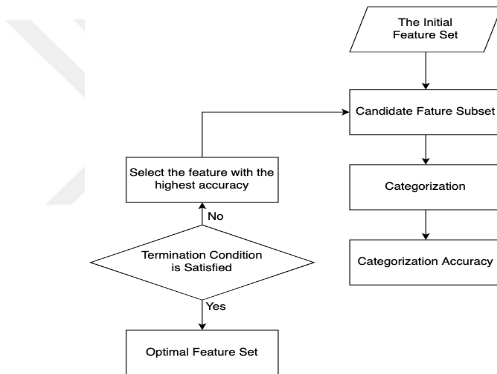
Figure 2.1. Forward selection diagram
