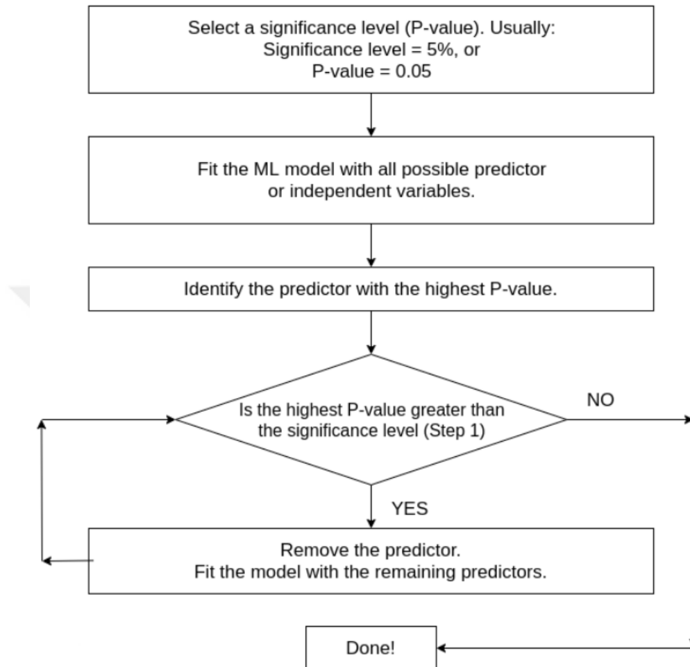
Figure 2.5. Backward elimination diagram
