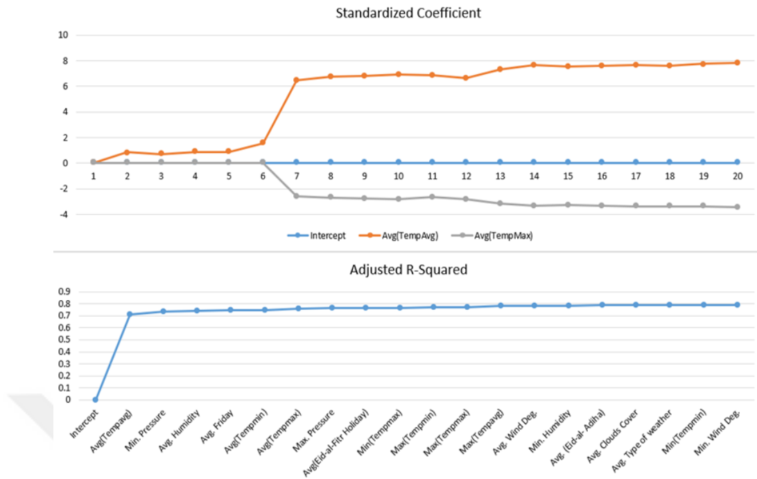
Figure 2.3. Coefficient Progression for Load
