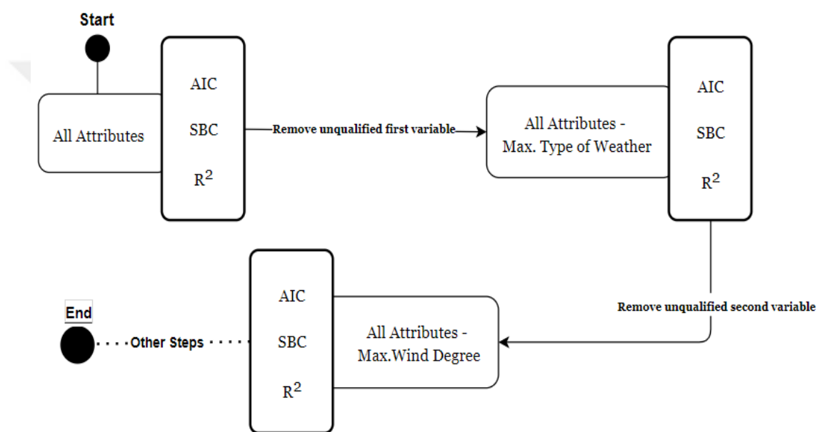
Figure 2.6. Three steps of Backward elimination diagram
