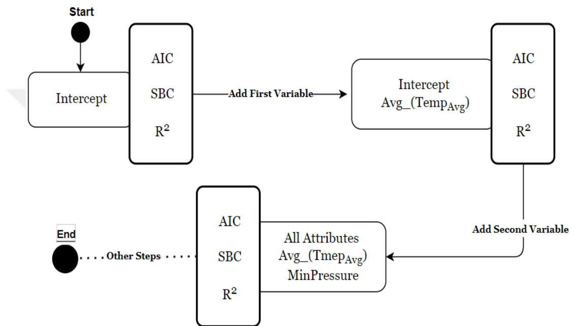
Figure 2.10. Three steps of Stepwise selection method diagram
