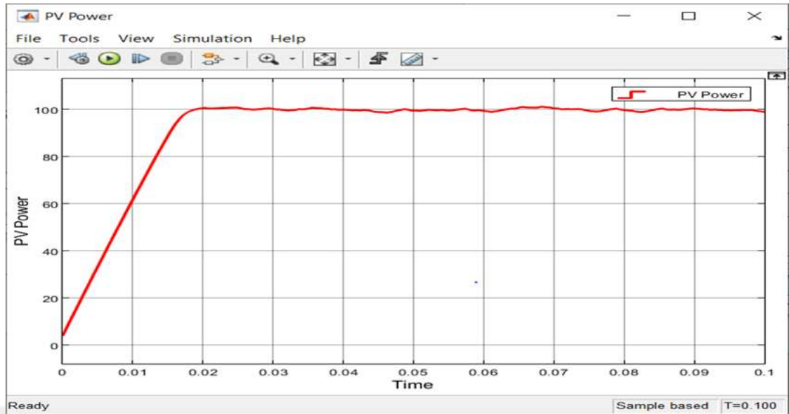
Figure 5.2 PV power with PI controller
