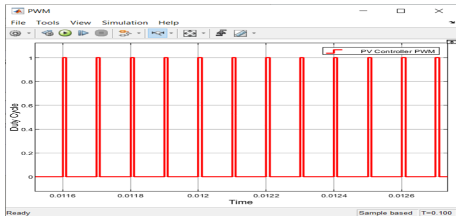
Figure 5.5 PV converter PWM signal
