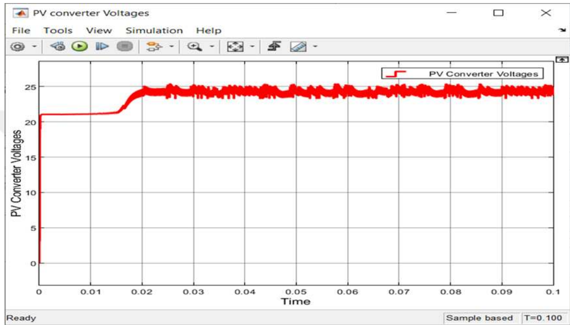
Figure 5.6 PV converter voltages with PI controlled MPPT
