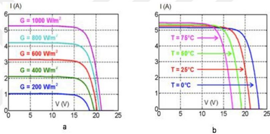
Figure 3.9 The influence of temperature fluctuations on I-V curves and the impact of changes in solar radiation (Guo et al. 2011)
