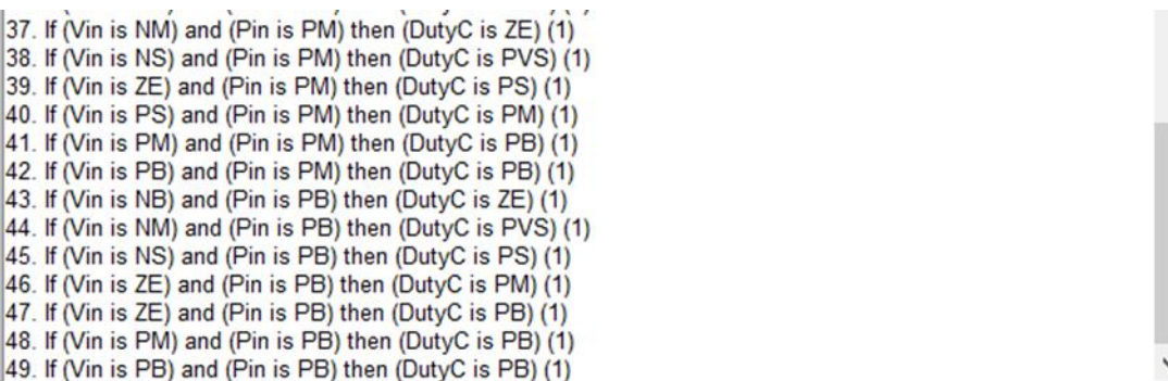
Figure 4.17 Assign the rules of the FLC unit
