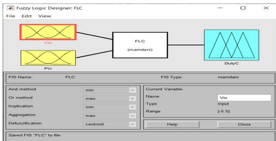
Figure 4.13 I/O of FLC window
