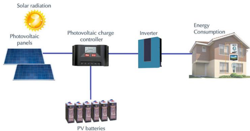
Figure 1.3 Isolated photovoltaic system applications
