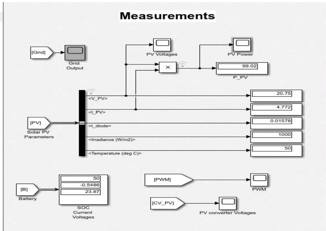
Figure 5.1 Measurements with PI controller results
