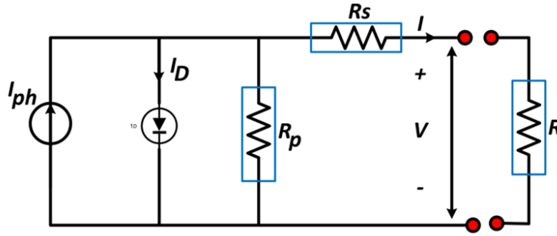
Figure 3.11 Photocell styled diode circuit
