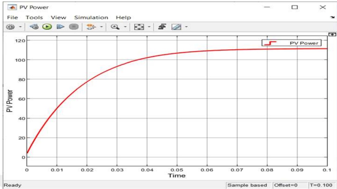
Figure 5.13 Maximum power achieved with ANFIS
