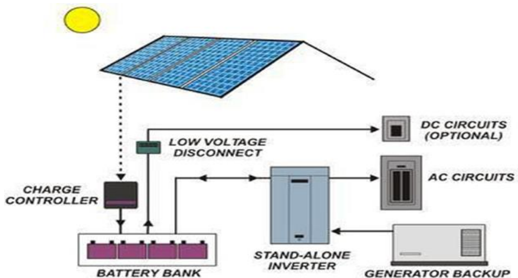
Figure 3.14 Standalone PV system (Diab et al. 2012)
