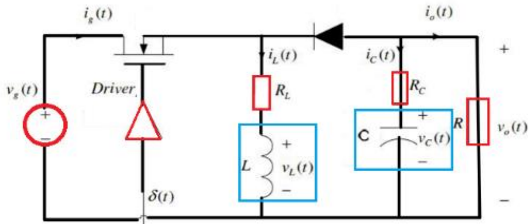
Figure 3.19 A circuit for buck-boost conversion
