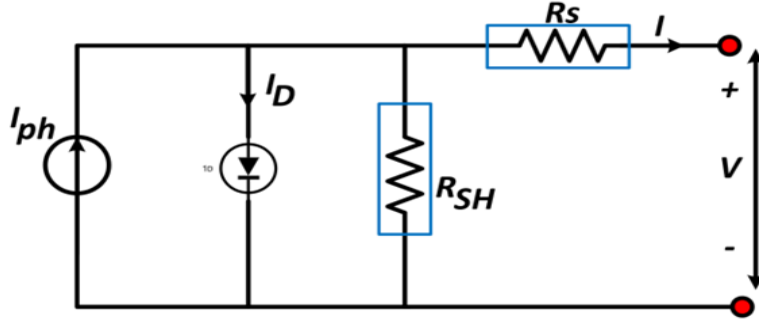
Figure 3.6 Single solar cell module
