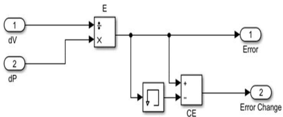
Figure 4.9 Error generating block diagram
