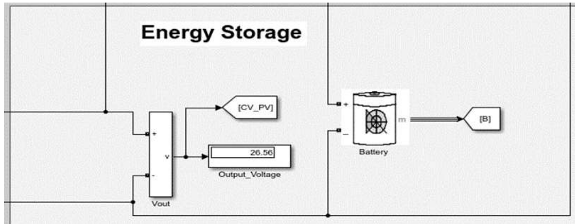
Figure 4.3 Energy storage unit for the simulation system
