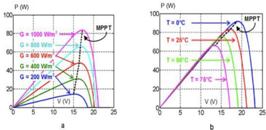
Figure 3.10 a) The impact of changing solar radiation on PV curves, and b) how temperature variations affect PV curves (Guo et al. 2011)
