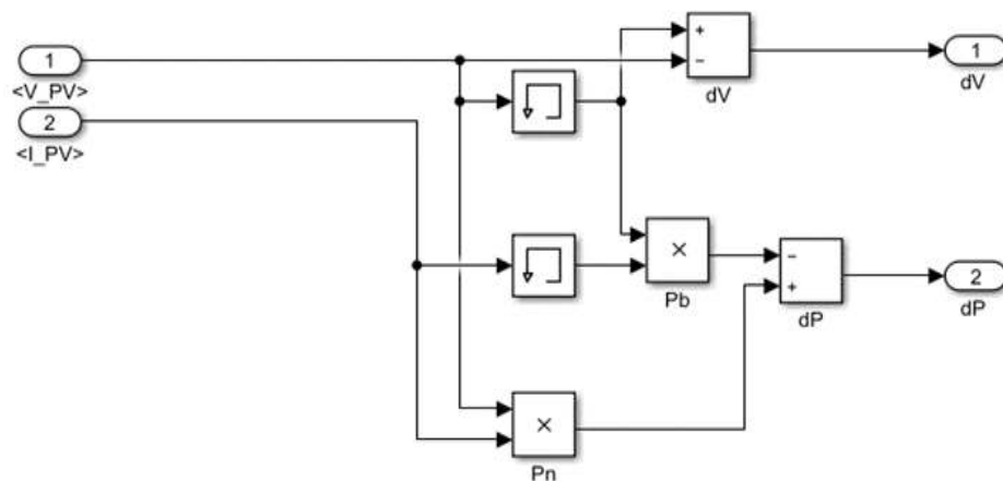
Figure 4.8 Differential change in power and voltage block diagram.
