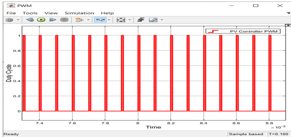
Figure 5.10 PWM with fuzzy controlled MPPT
