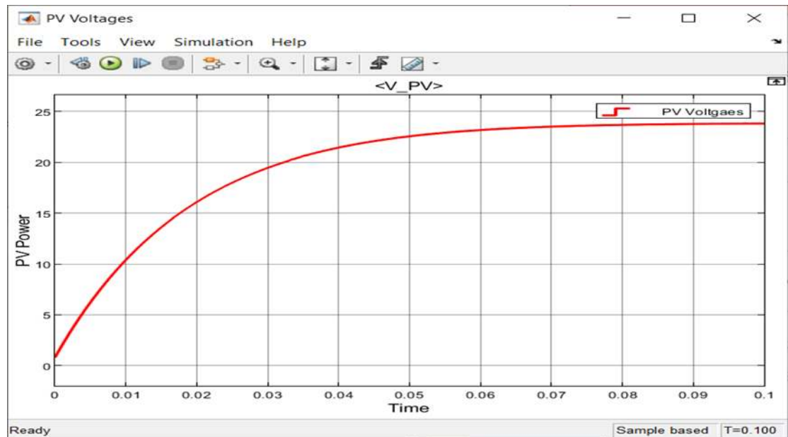
Figure 5.14 Controlled voltage of PV system
