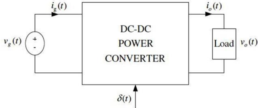
Figure 3.16 DC-DC converter structure (Himanshu and Tripathi 2012)
