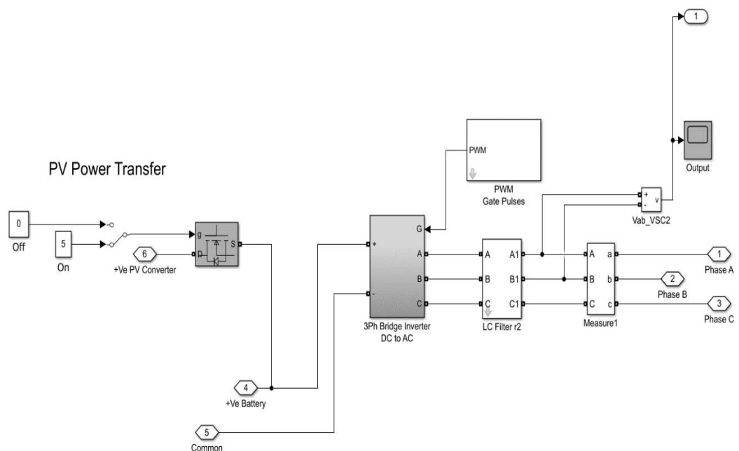
Figure 4.4 Microgrid block daigram
