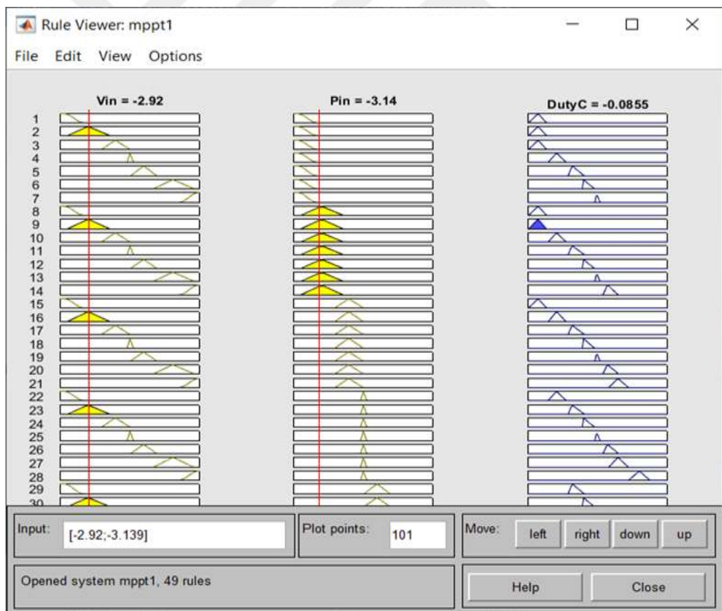
Figure 4.20 Viewer rules for FLC output monitoring
