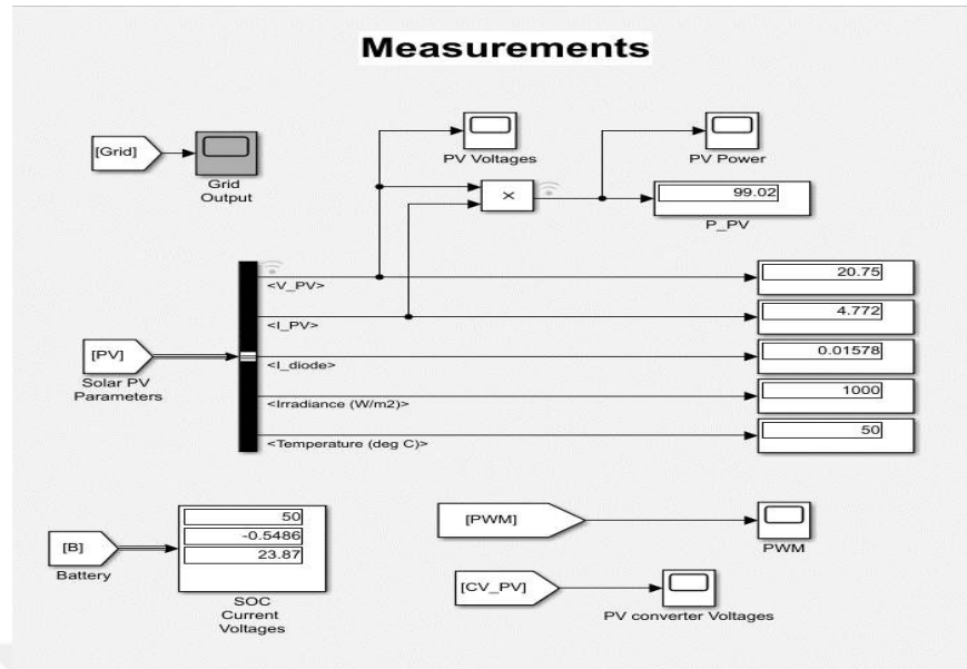
Figure 4.6 Monitoring section part in the simulation software
