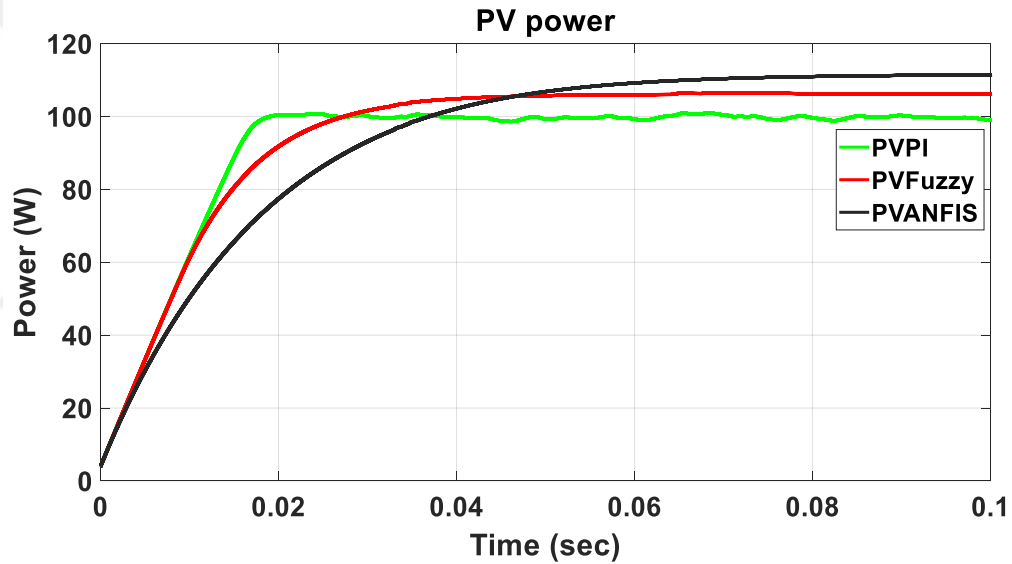
Figure 5.17 The comparison among three MPPT algorithms (PI, Fuzzy and ANFIS)
