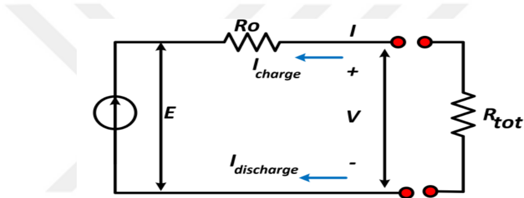
Figure 3.20 Schematic diagram of a battery
