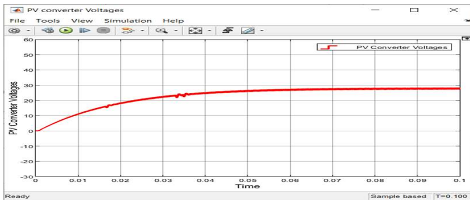
Figure 5.16 PV controller voltages with ANFIS controlled MPPT
