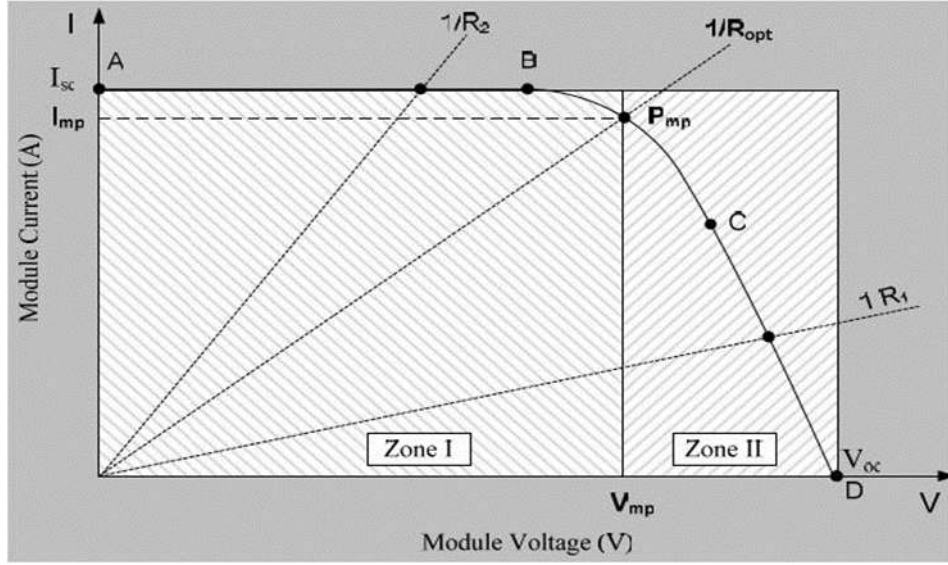
Figure 3.18 Monitoring the PV module's maximum power point (Erickson et al. 2001)
