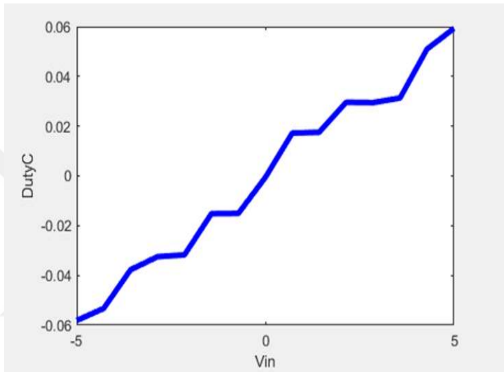
Figure 4.18 V_{in} and duty cycle
