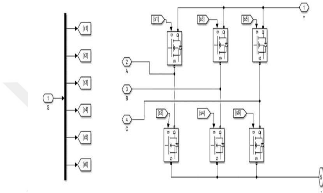
Figure 4.5 Three-phase inverter unit for the simulation system
