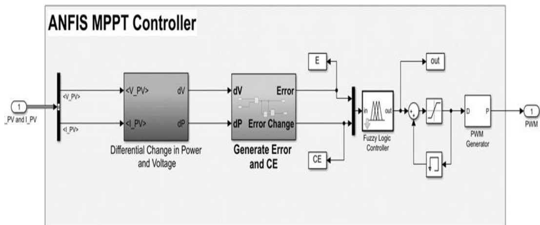
Figure 4.11 ANFIS controller system block diagram
