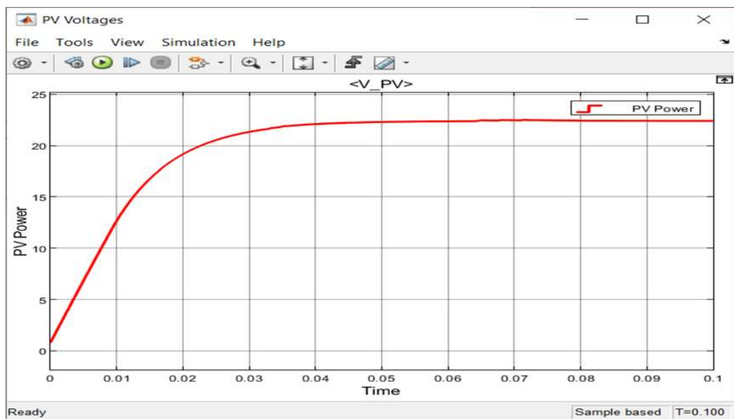
Figure 5.9 PV voltages with fuzzy control MPPT
