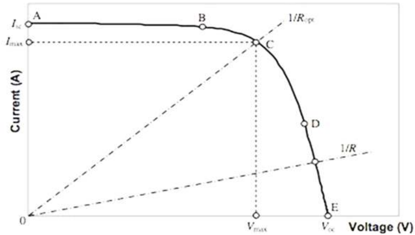
Figure 3.7 Representative voltage curve for photovoltaic cells (Lorenzo 1994)
