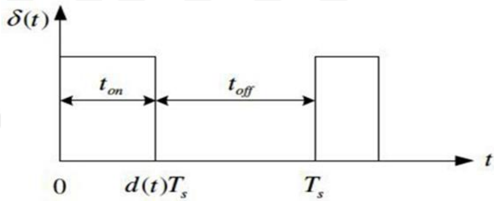
Figure 3.17 Transistor control signal (Erickson et al. 2001)
