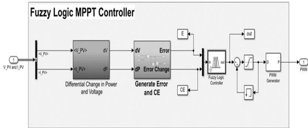
Figure 4.10 Fuzzy logic controller system block diagram
