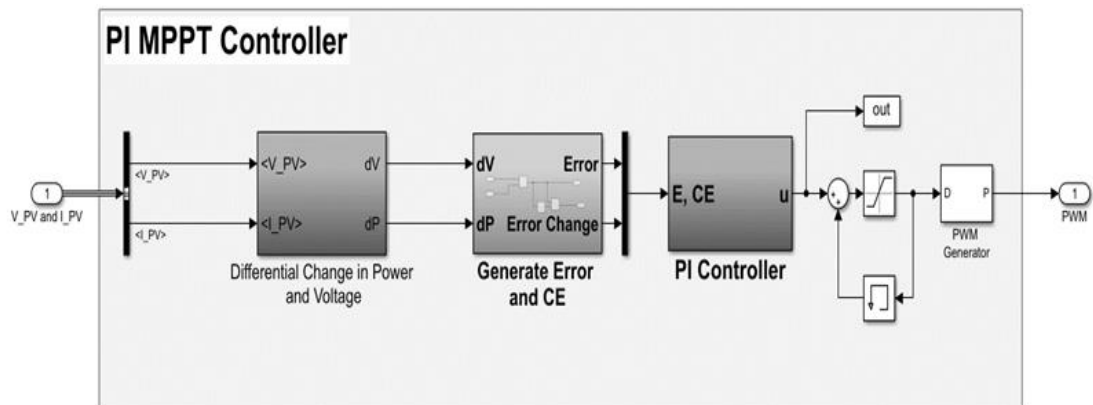
Figure 4.7 PI controller section
