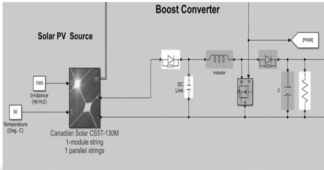
Figure 4.2 Solar PV source and boost converter
