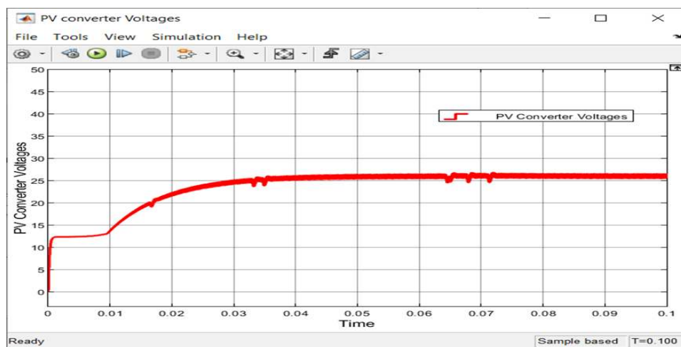
Figure 5.11 Converter voltages
