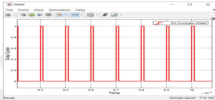
Figure 5.15 PWM duty cycle for ANFIS controller MPPT
