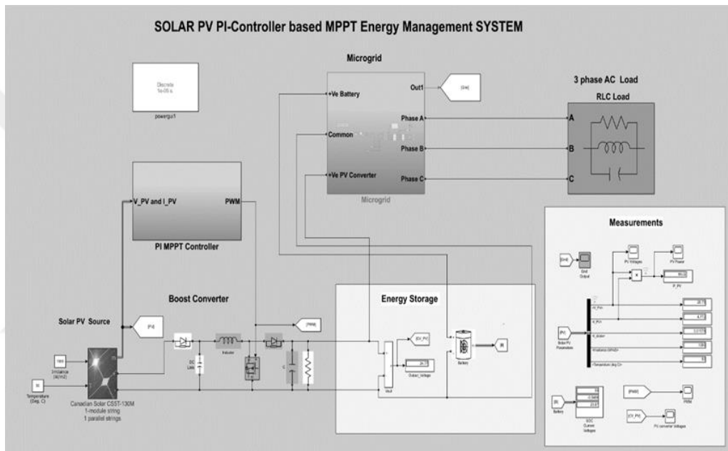
Figure 4.1 Complete simulink model design solar PV based on MPPT
