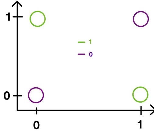
Figure 4.1: Binary XOR is a logical operator where the output of XOR operation is True if the inputs are different and the output is False if the inputs are identical. The phase space of XOR operator can be shown as above where there is no line that can separate the two output classes of XOR on the 2D space.
