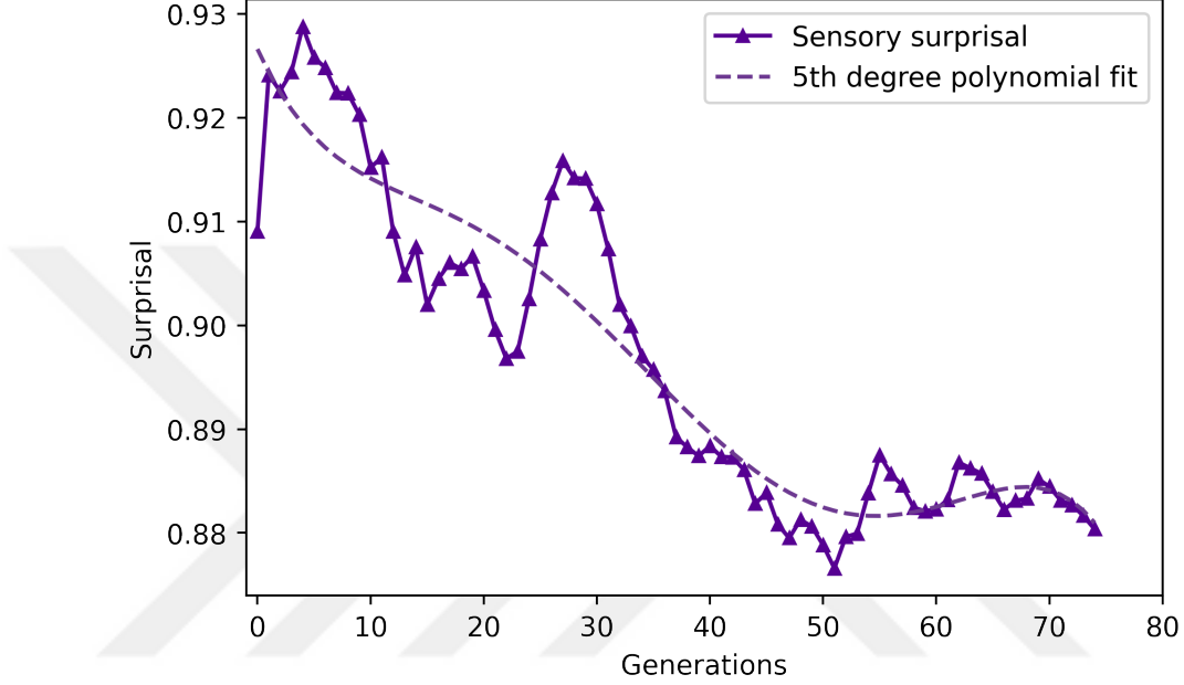
Figure 4.12: The average sensory surprisal of the agents decreases through generations. A 5th degree polynomial is fit to the original plot so that the decreasing is obvious. The fluctuation around the 28th generation is due to the discovery of the new behaviour.
