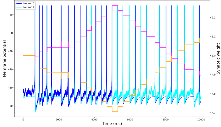
Figure 3.4: As the figure shows, the synaptic weight from Neuron 1 to Neuron 2 increases in the first half of the simulation due to the causal structure of the firings. However, on the second half the synaptic weight starts to decrease as the injected currents change. Of course the synaptic weight of the second synapse from Neuron 2 and Neuron 1 is affected by STDP as well, decreasing in the first half and increasing in the second. The Neuron1's potential is shown in Blue, and Neuron 2's potential in Cyan while the weight of the synapse from Neuron 1 to Neuron 2 is shown in Magenta and the other weight is shown in Orange.
