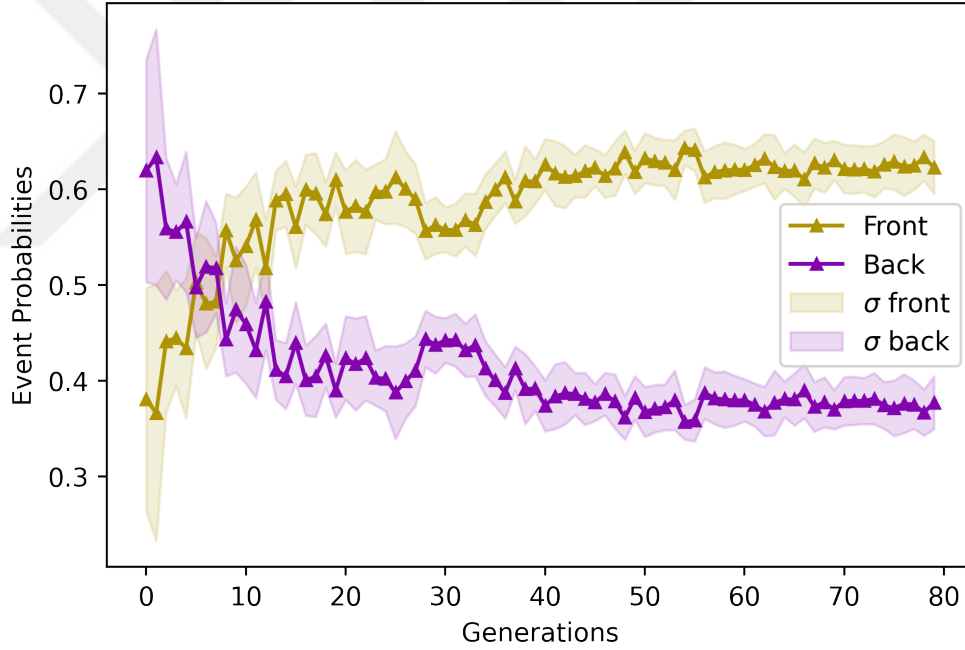
Figure 4.11: The agents learn to take the food in front of them after a while. Although a couple of fluctuations appear when the agents discover a new strategy, the decreasing regime continues.
