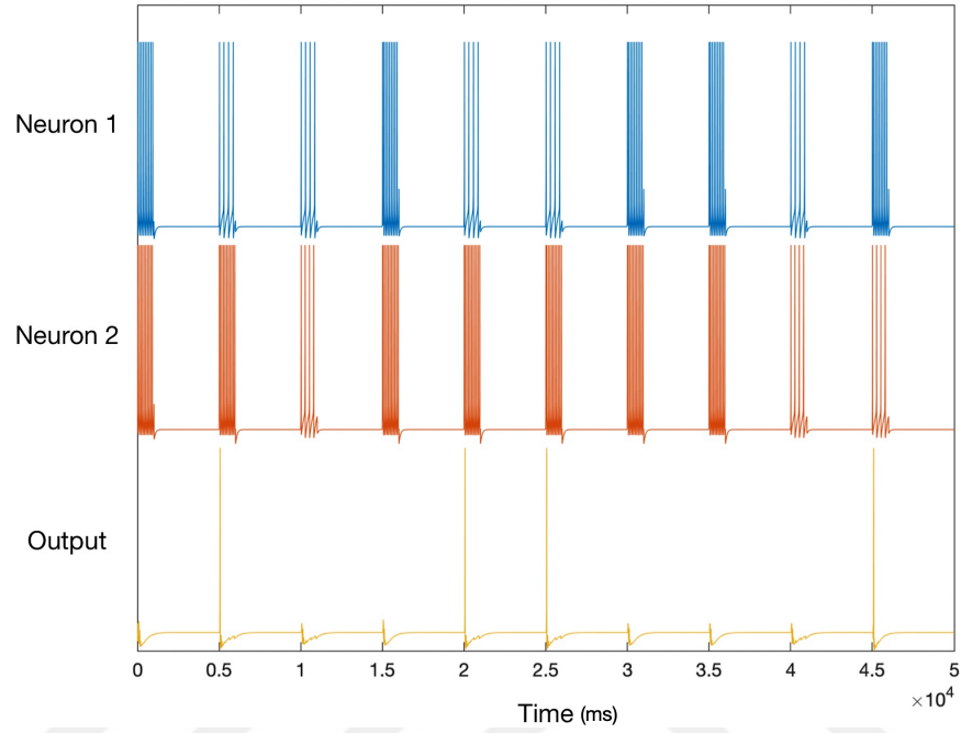
Figure 4.3: The neurons are stimulated with randomly chosen inputs from \{0, 1\} and the result is read from the third neuron. Whenever the inputs are different, the output neuron fires and stays silent when the inputs are the same.
