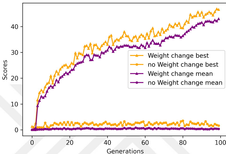
Figure 4.15: Direct external dopamine injection results. The agents with STDP learn the task where agents with no STDP show no improvement from the start.
