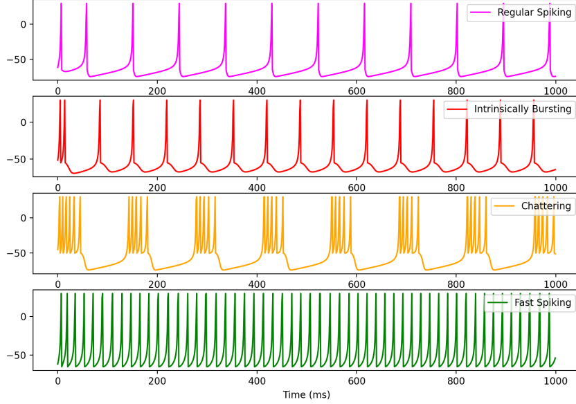
Figure 3.2: Here we show Regular Spiking (RS), Intrinsically Bursting (IB), Chattering (CH) and Fast Spiking (FS) neurons' response to constant I = 10 mA current for 1000 ms.
