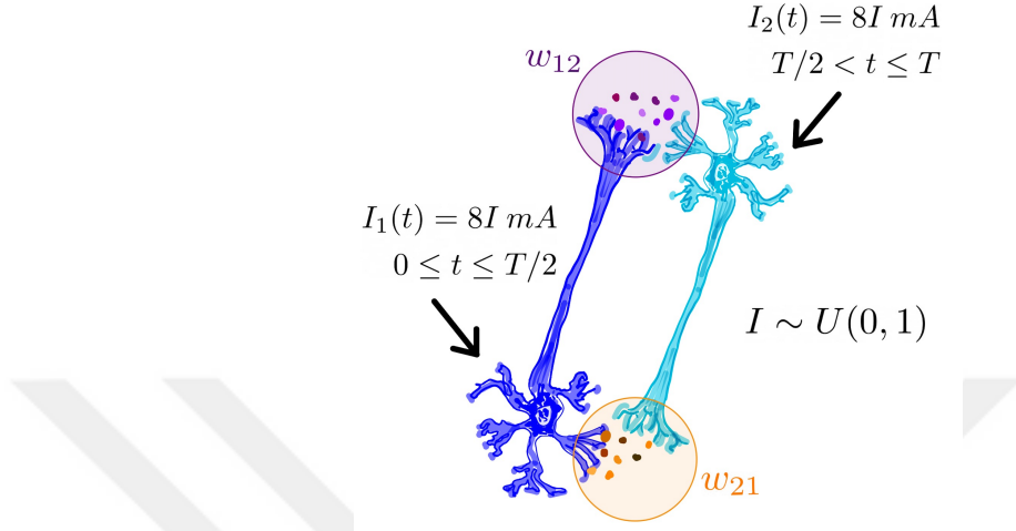
Figure 3.3: Two neurons as a loop is shown, the first one is blue and the second one is cyan. For the first half of the simulation, the first neuron is stimulated with a current I_1(t) = 8I \text{ mA} and the second neuron receives no injected current. On the second half of the simulation only the second neuron is stimulated with an injected current of I_2(t) = 8I \text{ mA} where I is sampled from the uniform distribution U(0, 1) . The weights of the synapses from the first to the second neuron and from the second to the first neuron are w_{12} and w_{21} respectively.
