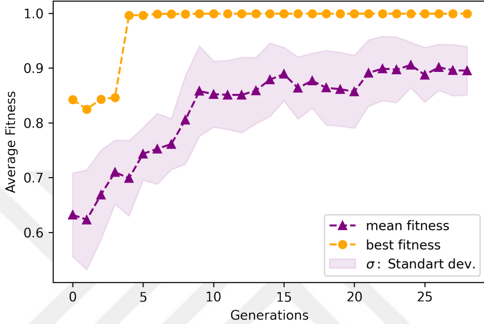
Figure 4.7: NEAT reaches 0.99 in the pole balancing problem within 15 generations.
