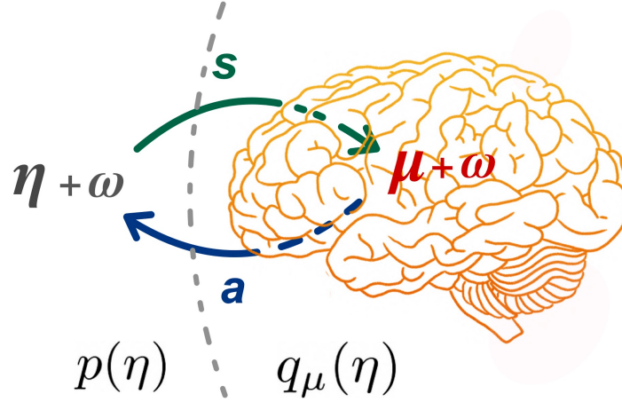
Figure 3.6: Showing the Markov Blanket of a brain where \mu are internal states with random fluctuations \omega only affecting the active states a , \eta are the external states with random fluctuations \omega only influencing the sensory states s , q_\mu(\eta) are internal beliefs about the external states and p(\eta) is the true density of external states.
