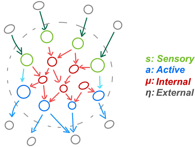
Figure 3.5: A Markov Blanket of a thing contained in the grey dotted line. The sensory ( s ) and active states ( a ) are highlighted with green and blue colours while internal states ( \mu ) are shown in red and external states ( \eta ) are in grey.
