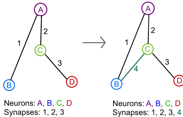
Figure 3.10: A new connection is added between neurons B and C and changed the genome accordingly.
