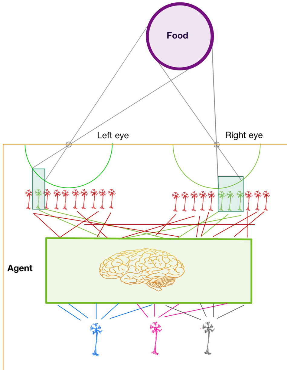
Figure 4.8: Architecture of the agents used in food chasing game with visual sensory units. The food's projection falls into the retinal cells and stimulates the respective fields. The stimulation causes firing of some neurons (green) more than the others (red). The sensory firings then stimulate the internal network, which will be determined by NEAT, and the output is given with three motor neurons shown in Blue, Magenta and Gray.
