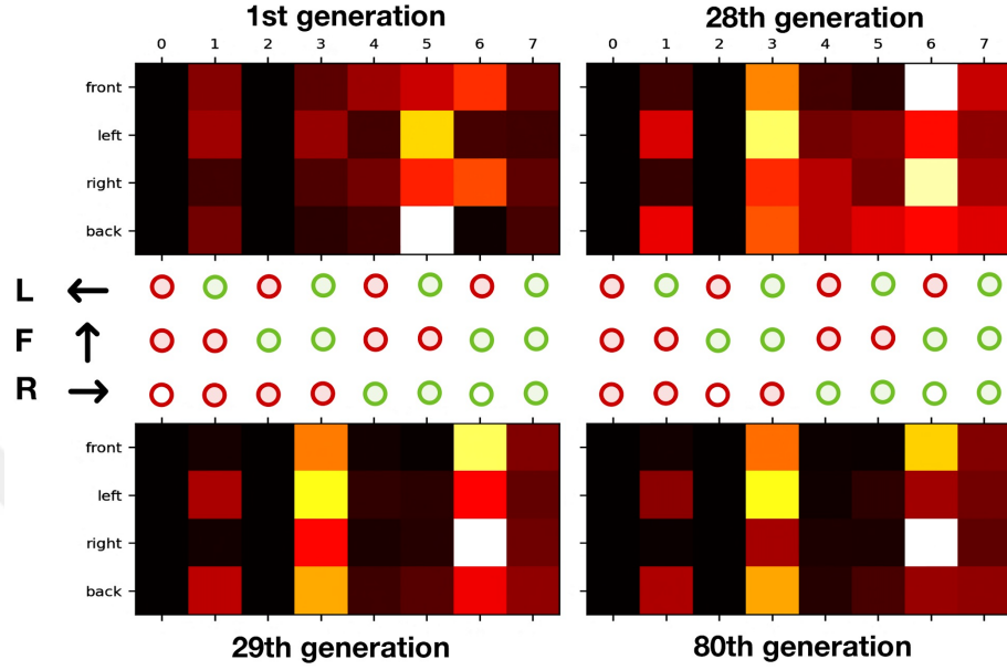
Figure 4.10: Behavioural maps of 1st, 28th, 29th and 80th generation as 4x8 matrices. Each row represents the situations where the food falls with respect to the agent while each column represents the response given by the agent as a motor activity. The eight responses are binary coded configurations each of which has three components: left, forward and right motor neurons' firings. Each cell represents a probability where the rows are normalized, i. e. sum of any row is equal to 1. The red and green circles represent whether left (L), right (R) and/or Forward (F) neurons fired when encountered with the situation on y axis. The cells are hot color coded, black is the lowest and white is the highest. Notice that the agents prefer to fire left and right when the food is on the back at 1st generation but this behaviour is almost totally abolished when we look at the 29th generation.
