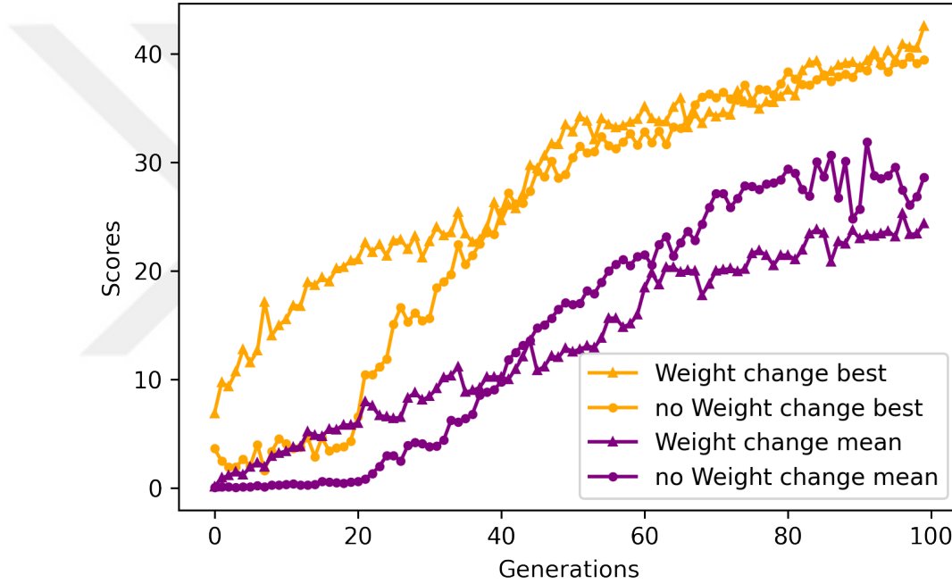
Figure 4.14: Simulation results of two populations, the first contains agents without STDP and the second with STDP. Both of the populations solve the matrix chase problem where the agents are supposed to catch the correct pill out of two pills. The first population is given with Circles and the second class is in Triangles.
