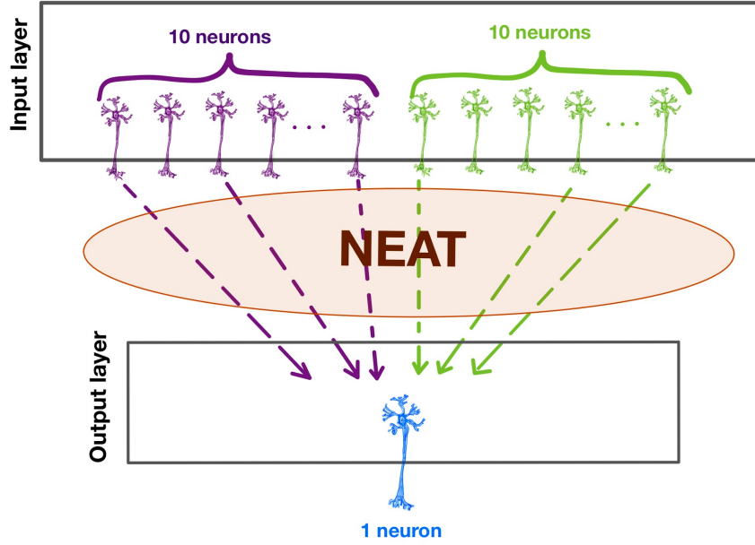
Figure 4.2: The design of an SNN initialized with random connections from input layer to output layer. The purple colored neurons represent the first input while the green ones represent the second input. There are only 21 neurons present at first. The hidden internal parts of the network is determined with NEAT.
