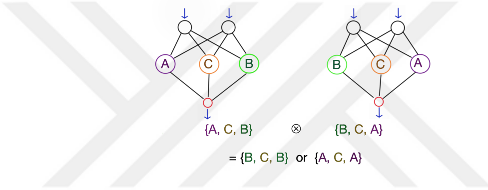
Figure 3.7: An example of competing conventions. Two networks work the same but their internal order is different, so when cross-over (shown with \otimes ) is applied the possible offsprings lose a third of the information.
