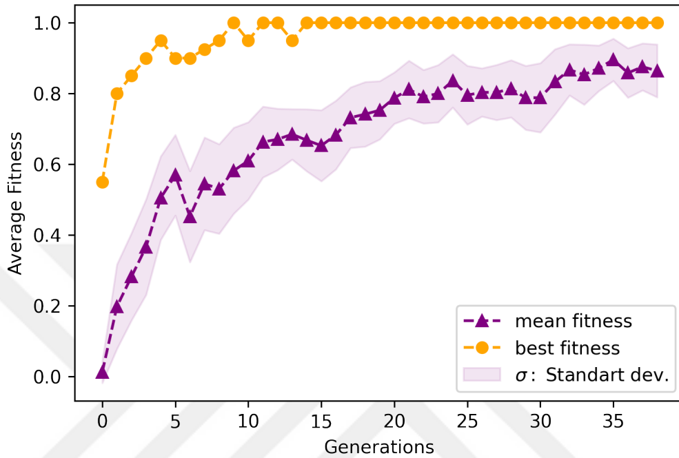
Figure 4.4: NEAT algorithm solves XOR problem within 15 generations. The figure shows the mean score of agents in each generation in purple and the best agent’s score in orange. The purple shade is the standard deviation of agents’ scores.
