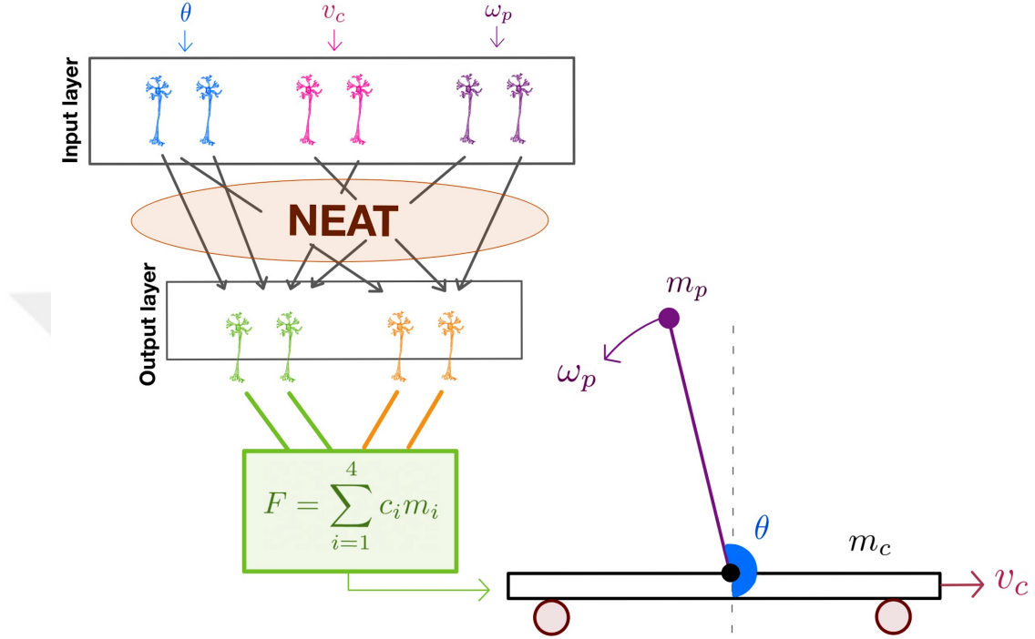
Figure 4.6: Initial architecture of the pole balancing network and the respective inputs and outputs taken from the cart pole system. Three main inputs are the deviation of the pole ( \theta ), velocity of the cart ( v_c ) and the angular velocity of the pole ( \omega_p ). Only output is the force that will be applied to the cart.
