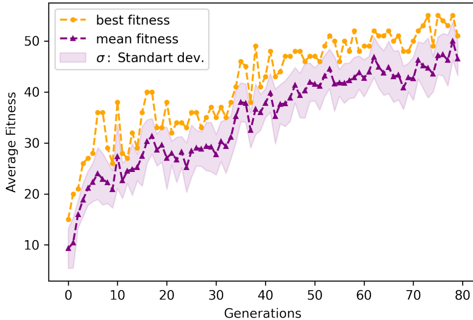
Figure 4.9: The average fitnesses of the agents increase in a consistent way. Fitness of an agent is the number of foods the agent consumes within its lifetime.
