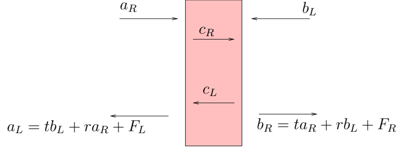
Figure 5.1: Absorbing dielectric slab
