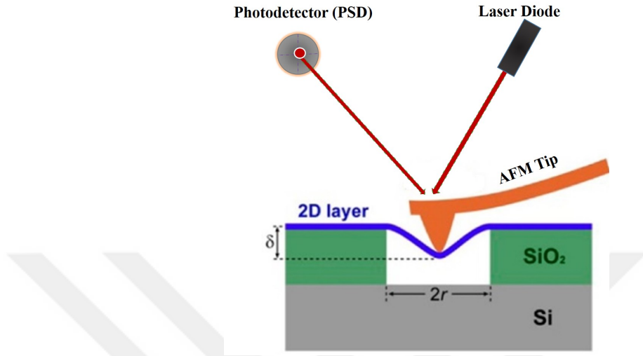
Figure 2.13: AFM nanoindentation block diagram Reproduced and Copyright ACS (2014) [75]
