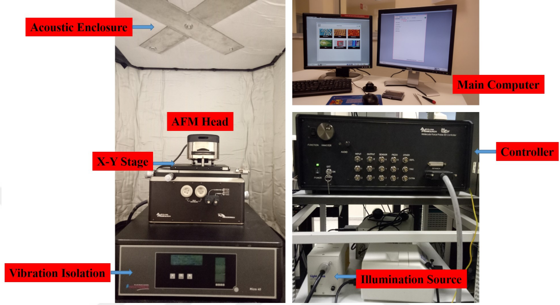
Figure 3.1: Asylum AFM setup at UNAM
