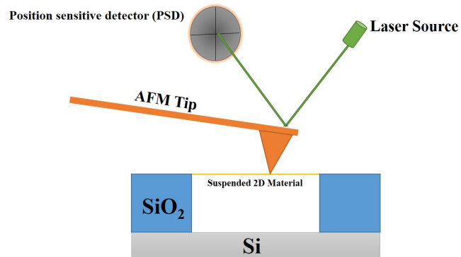
Figure 2.10: AFM based nanoindentation schematic
