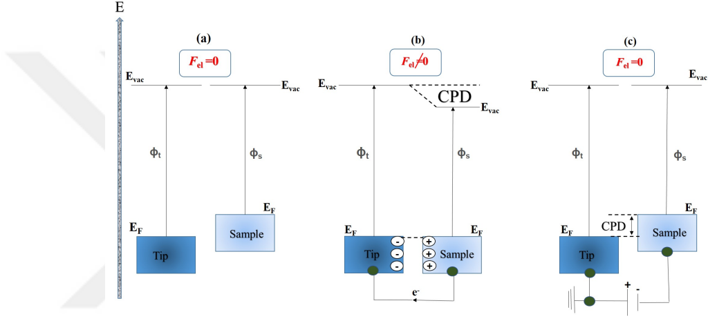
Figure 2.2: Mechanism of KPFM. (a) two metals having different values of work functions come into contact (b) Fermi level alignments (electron flow from less work function metal to higher until CPD generates because of build in electric field) (c) external potential needed to nullify CPD (re-alignment of Fermi levels)
