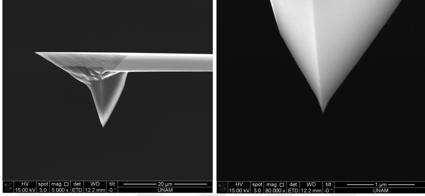
Figure 3.10: High resolution SEM images of nanoindentation probes
