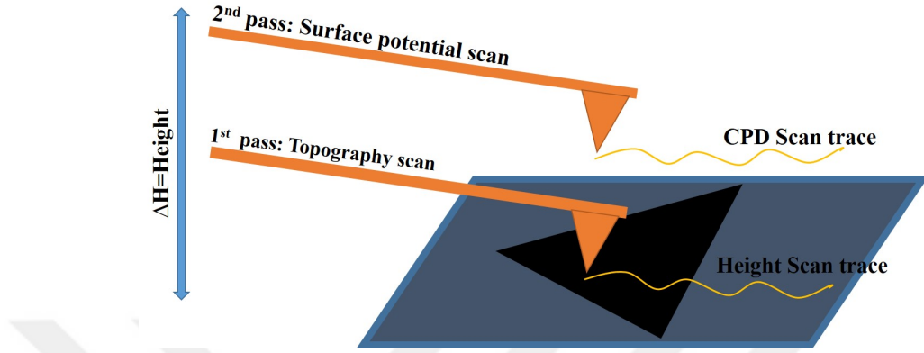
Figure 3.4: Sketch map for KPFM scanning process
