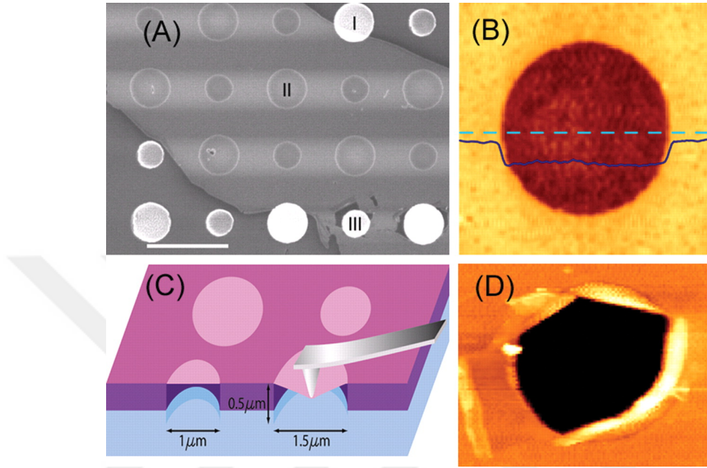
Figure 2.8: (A) SEM image of suspended graphene over holes (B) Non-contact mode topographical image of graphene flake over hole (C) Schematic setup for nanoindentation (D) Fractured topographical image after maximum indentation Copyright (2008) Science [8]
