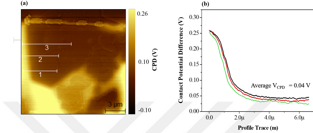
Figure 4.7: (a) CPD map of V_2O_3 flake (b) CPD profiles from previous different region in image
