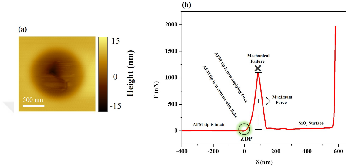
Figure 4.14: (a) AFM image of 2H-TaS 2 flake after fracture in center (b) F-D curve steps explanation
