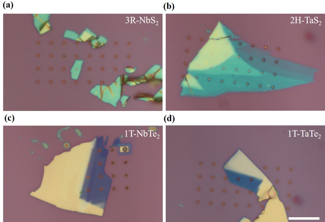
Figure 4.1: Optical microscope images (a) 3R-NbS 2 (b) 2H-TaS 2 (c) 1T-NbTe 2 (d) 1T-TaTe 2 crystals transferred over FIB drilled holes using viscoelastic stamp technique
