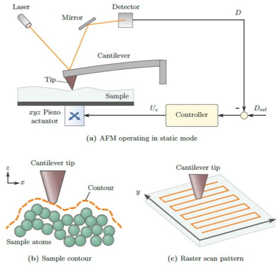
Figure 1.3: (a) AFM Static mode working principle (b) tip follows contour path (c) tip scans sample in raster pattern
