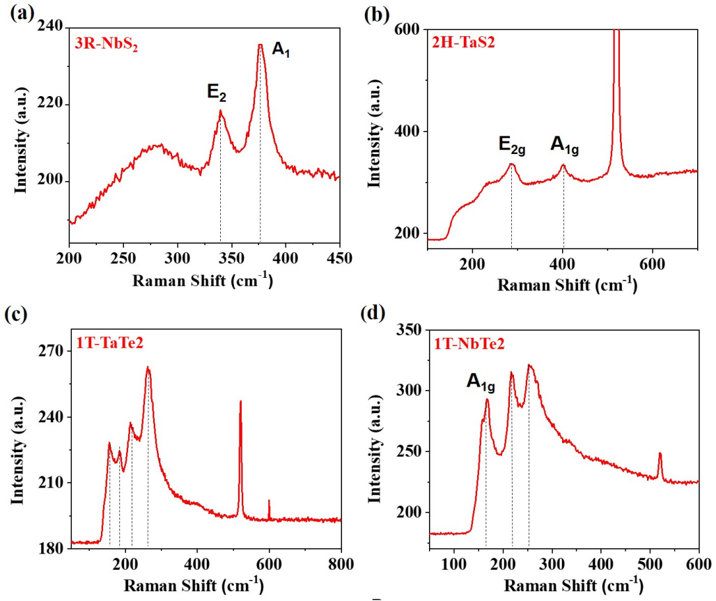
Figure 4.3: Raman profiles of metallic (a) 3R-NbS 2 (b) 2H-TaS 2 (c) 1T-TaTe 2 (d) 1T-NbTe 2 ultrathin flakes
