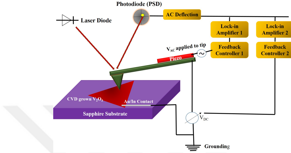
Figure 3.3: Schematic of Asylum KPFM setup
