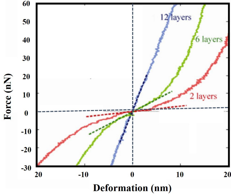
Figure 2.12: FD Curves for mica showing non-linear behave for 2-6 layer while 12 layers showing linear trend under applied load
