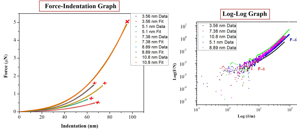
Figure 4.11: (a) Force versus indentation of 2H-TaS 2 sheets with fitting (red crosses show breaking point of sheets that gives breaking stress) (b) log graph showing liner and cubic region at lower and higher loads respectively
