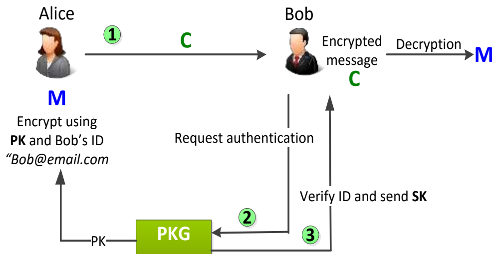
Figure 1: ID-Based Encryption
