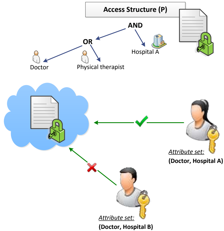
Figure 3: CP-ABE
