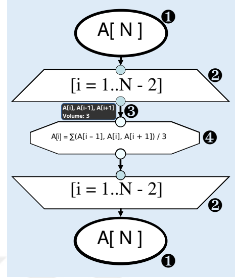
(b) Generated SDFG IR (simplified)
