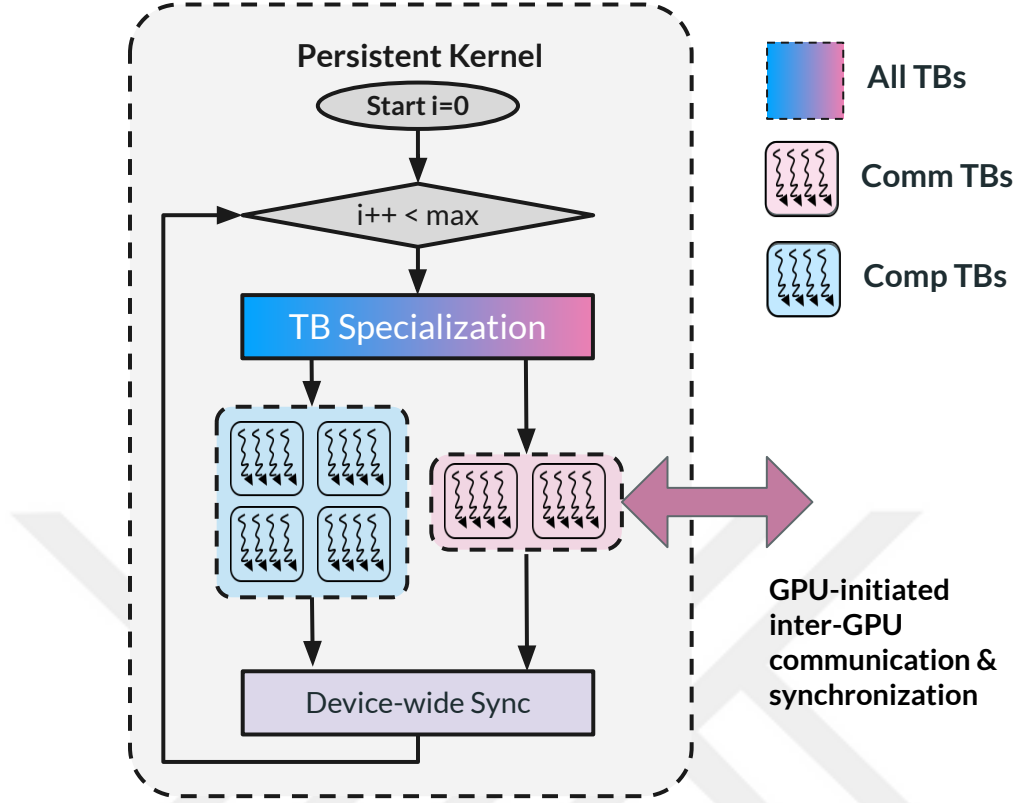
Figure 3.1: CPU-free execution model leverages persistent kernels, thread-block (TB) specialization, GPU-initiated data transfers, and device-side synchronization. Comm: Communication, Comp: Computation.
