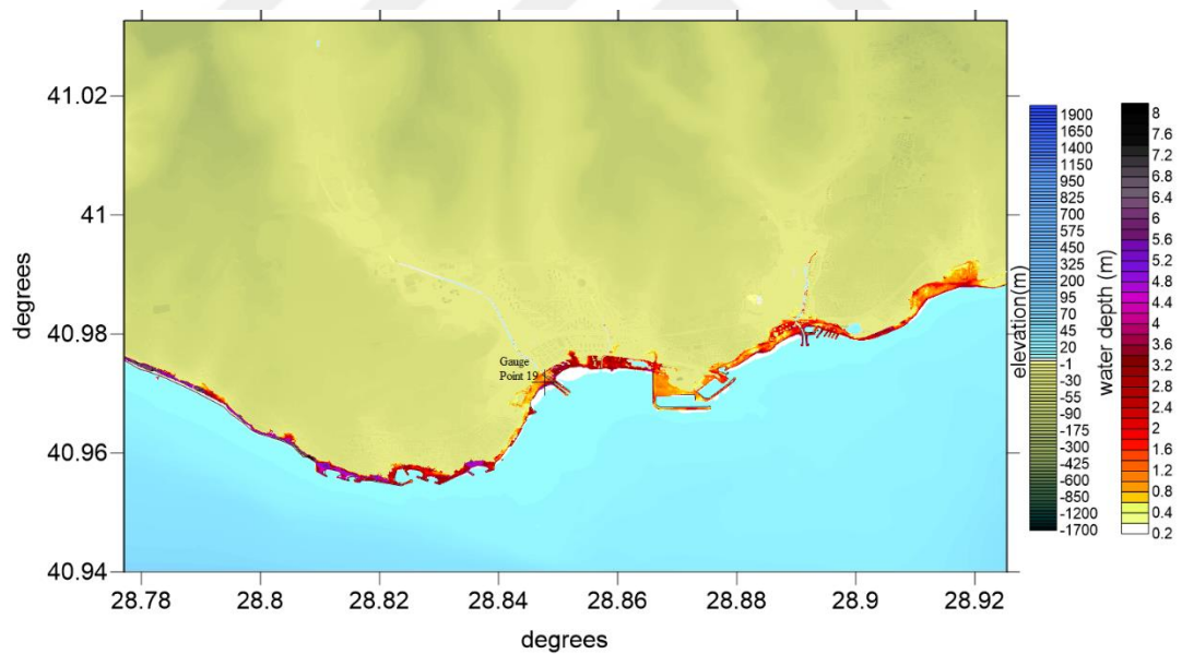
Figure 4-19 Location of Gauge 19 on Maximum Flow Depth Map
