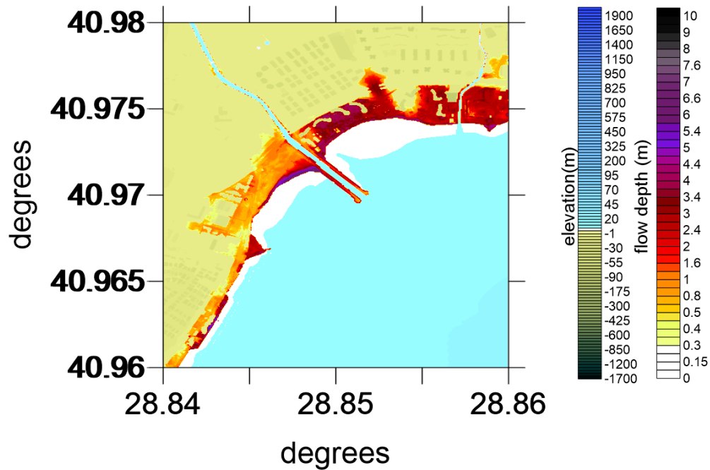
Figure 4-20 Flow depth distribution for LSBC sourced Tsunami focused on the Ayamama River Mouth
