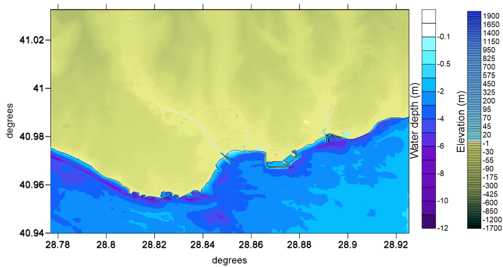
Figure 4-11 Minimum Eta Map of LSBC Sourced Model
