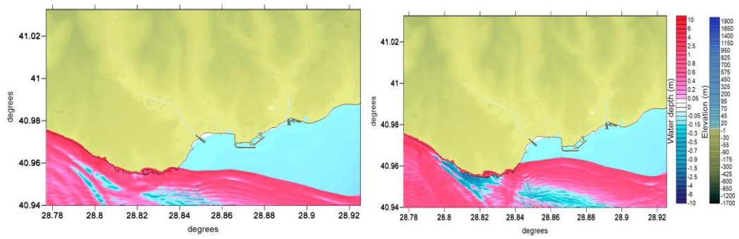
Figure 4-13 Tsunami propagation at 2-3 minutes
