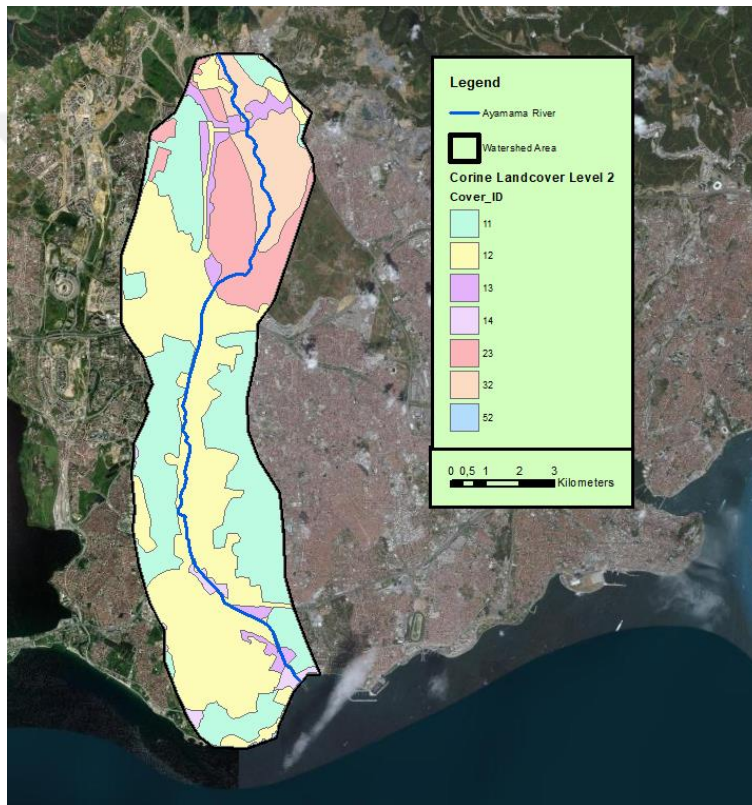
Figure 3-6 Level 2 Corine Landcovers in Ayamama Watershed
