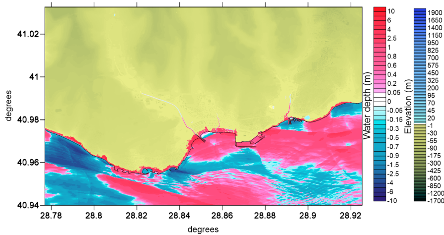
Figure 4-17 Tsunami propagation at 10 minutes
