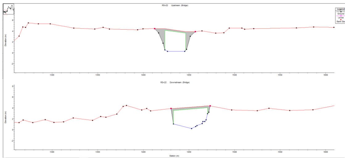
Figure 3-13 Bridge at the station 22 meters
