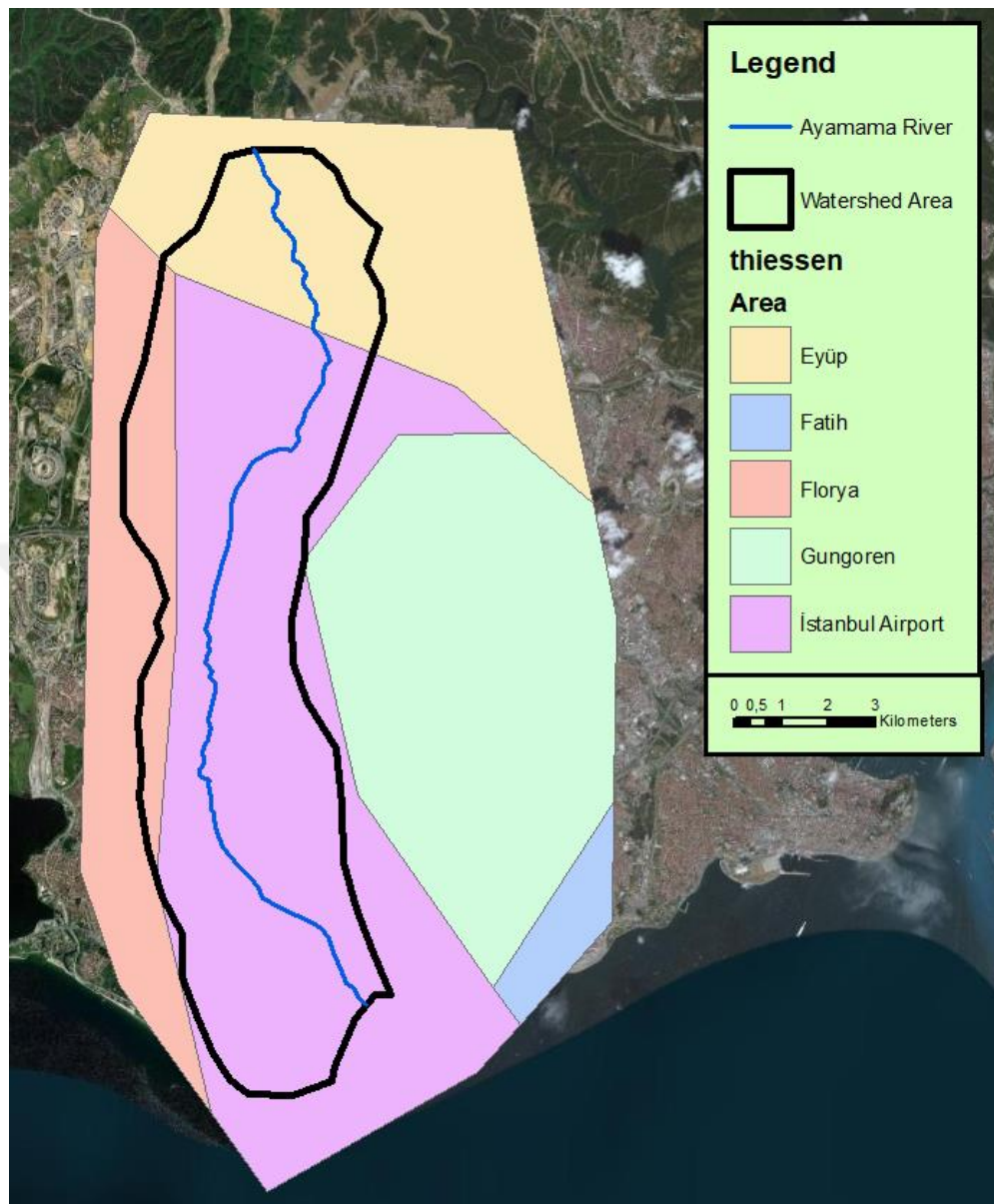
Figure 3-5 Thiessen Area of 5 stations
