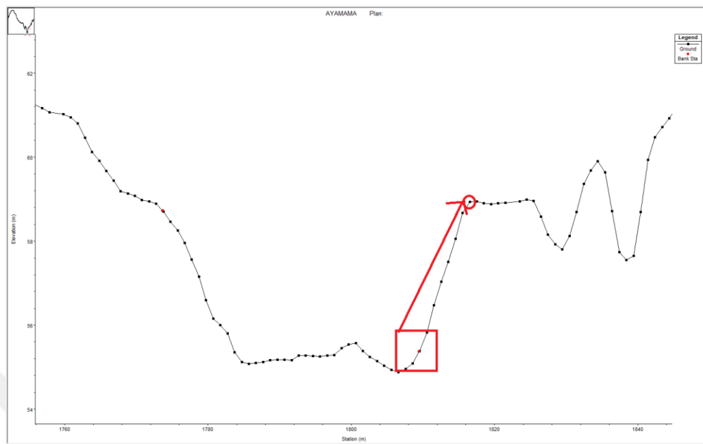
Figure 3-11 Correction of bank point
