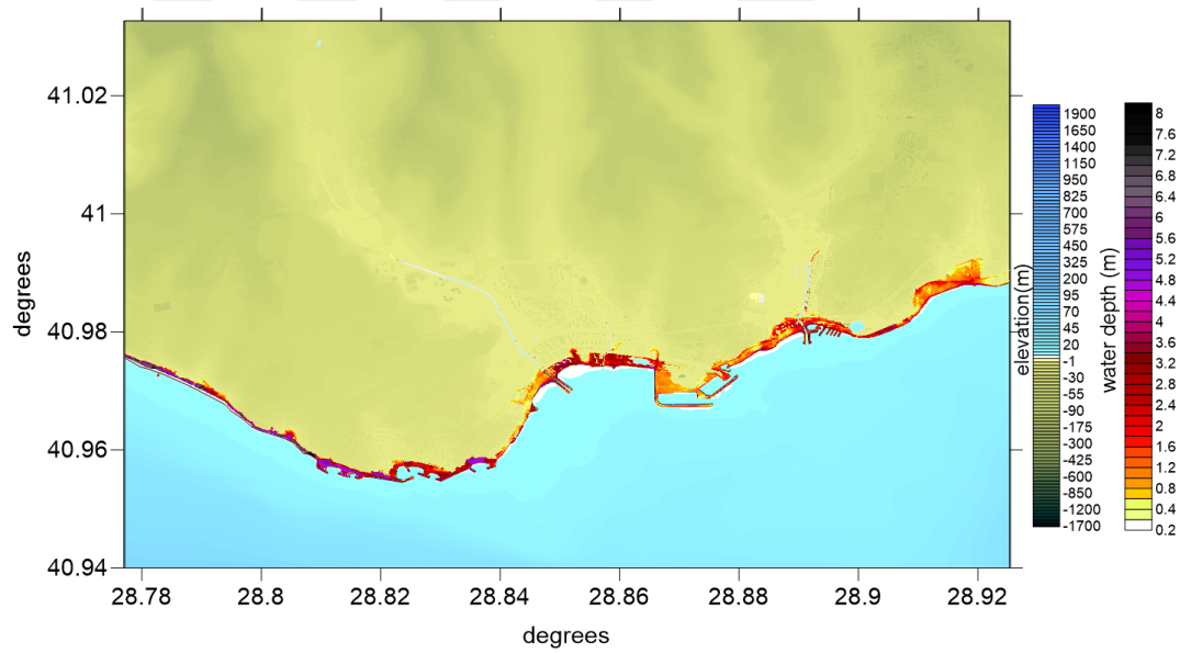
Figure 4-10 Maximum Flow Depth Map of LSBC Sourced Model
