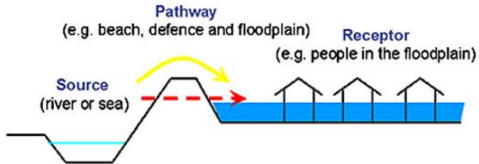
Figure 2-3 1D SPRC model for Coastal Flooding (Narayan et al., 2011)
