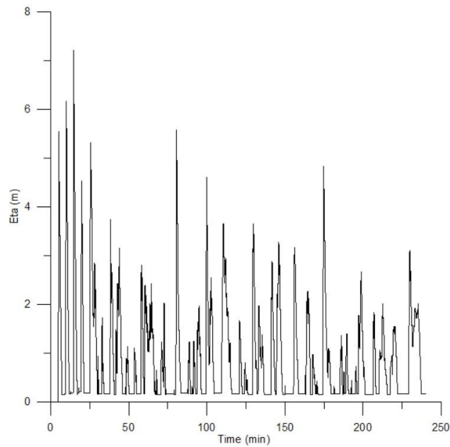
Figure 4-18 Time History of Gauge Point 19
