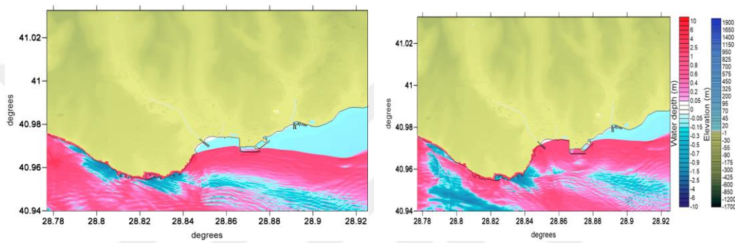
Figure 4-14 Tsunami propagation at 4-5 minutes
