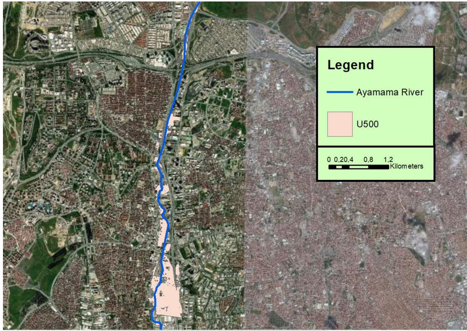
Figure 4-3 Flood inundation with 500 year return period flow in the Ayamama River (Center)
