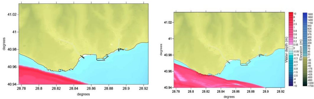
Figure 4-12 Tsunami propagation at 0-1 minutes
