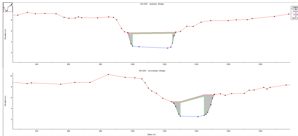
Figure 3-16 Bridge at the station 3250 meters
