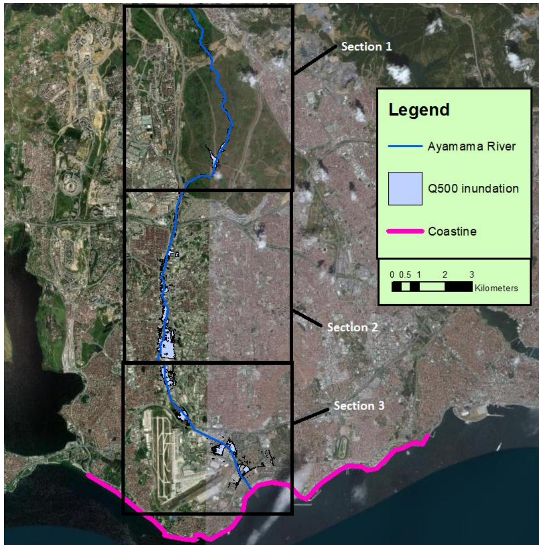
Figure 4-1 Three sections of inundation maps for 500 year return period
