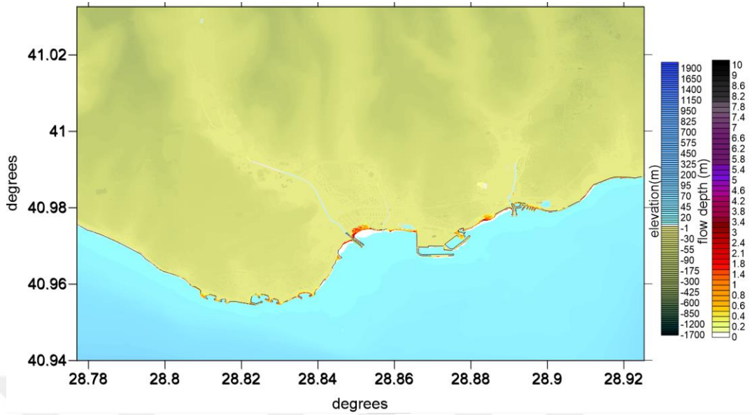
Figure 4-9 Maximum Flow Depth Map of PIN Sourced Model
