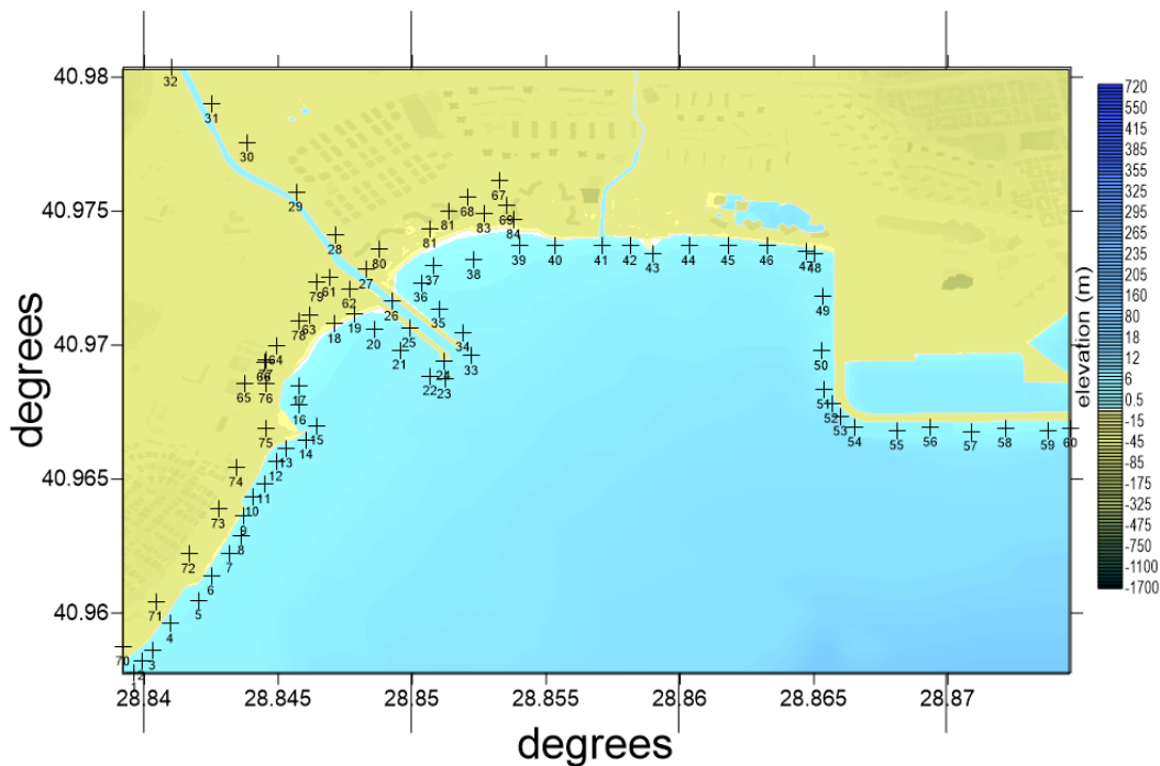
Figure 3-31 Gauges on the Study Area
