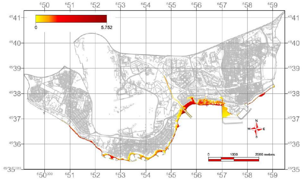
Figure 2-1 Inundation map for Bakırköy Coasts for YAN sourced Tsunami (Tüfekçi, 2016)
