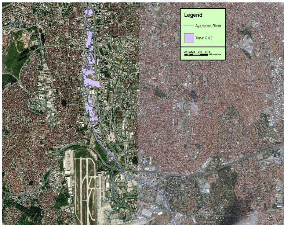
Figure 4-7 Flood inundation at 6:00
