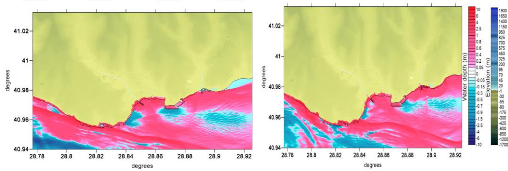
Figure 4-15 Tsunami propagation at 6-7 minutes
