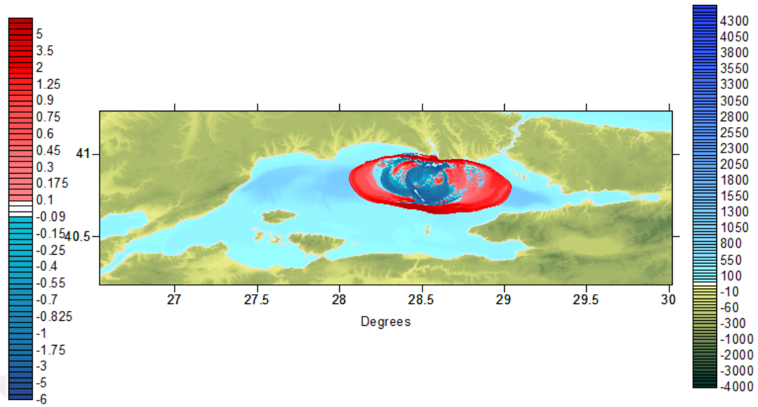
Figure 3-30 Tsunami Source LSBC
