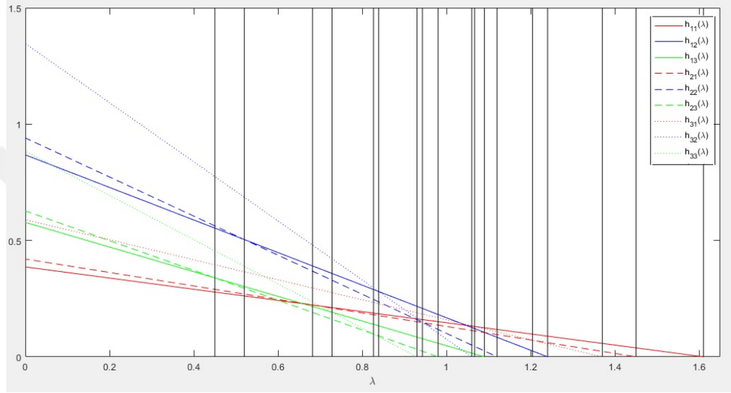
Figure 4.1: h_{ik} lines
