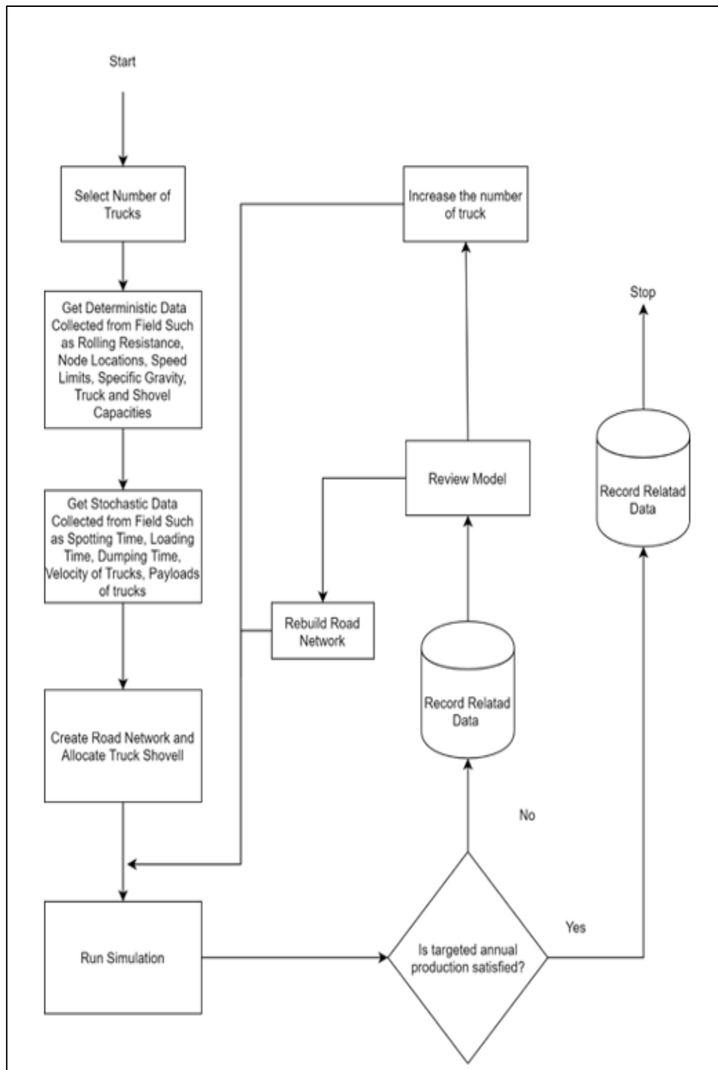
Figure 3.4 Dispatch Algorithm
