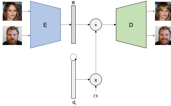
(c) Our approach, where we learn an end-to-end trainable pipeline with latent directions that are learned in training time.
