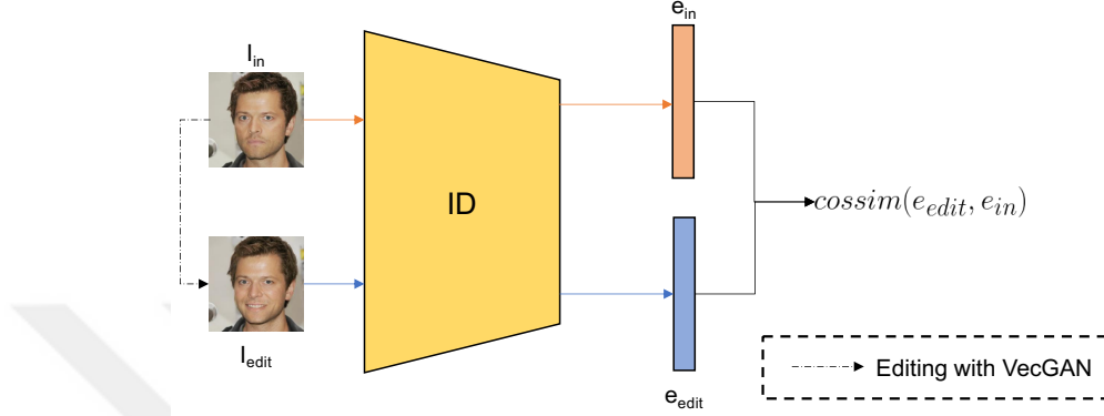
Figure 4.3: Identity Preservation (ID) metric calculation for smile addition task. After editing the input with a negative smile attribute with smile addition edit, we feed both the generated image I_{edit} and input image I_{in} to the CurricularFace model. Then by using the embeddings outputted from the input image e_{in} and the generated image e_{edit} , we report the cosine similarity between them as the ID score.
