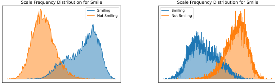
(a) Histogram \alpha_s values for smile tag of VecGAN base
