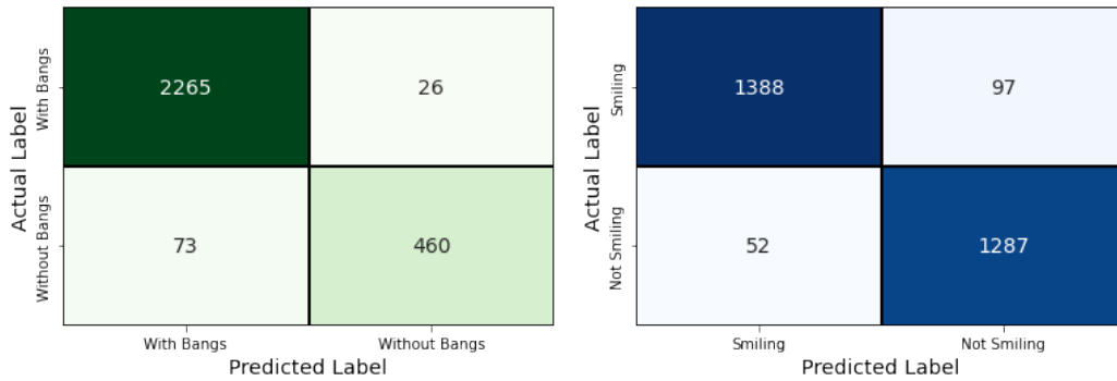
Figure B.1: Confusion matrices for the classifiers used in evaluation Setting II.
