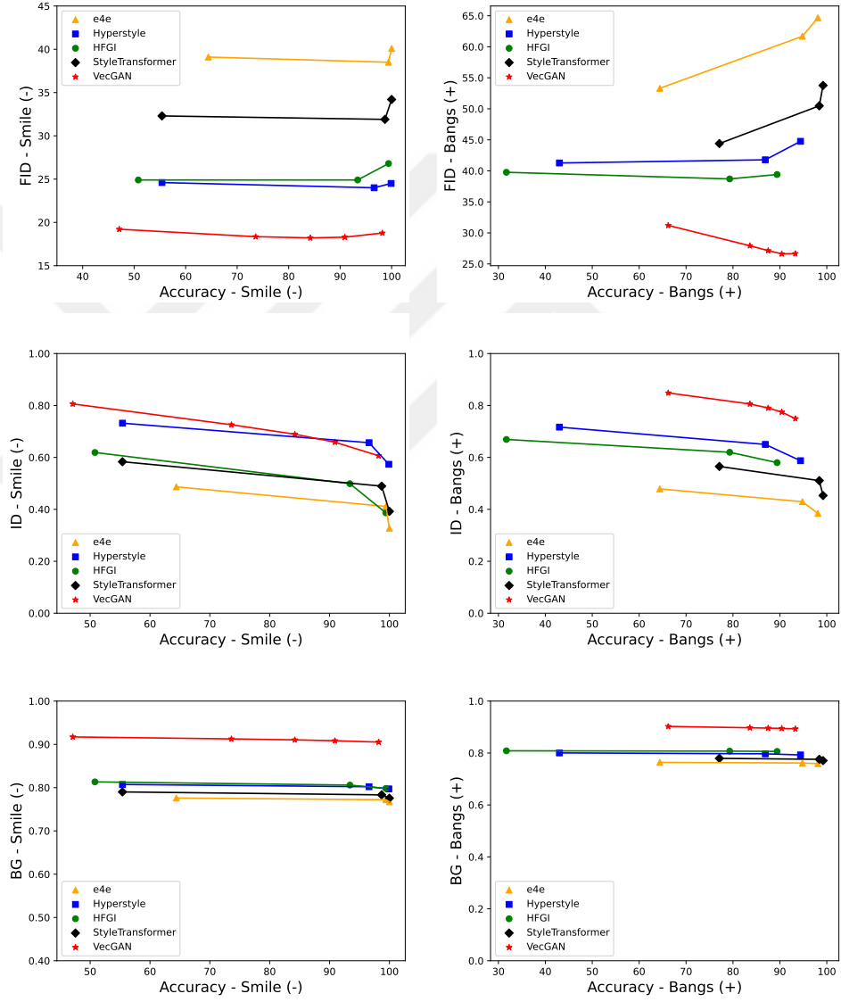
Figure 4.10: Plots of FID, ID, and BG metrics as we change the intensity of the attributes. For each intensity, we measure the attribute accuracy in the x-axis. The first column plots present results for smile removal (global attribute), and the second column presents them for bangs addition (local attribute).
