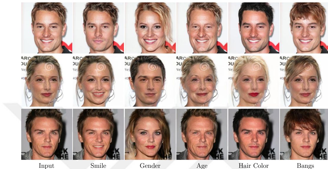
Figure 1.1: VecGAN image translation results. The first column shows the source images, and the other columns show the result of editing a specific attribute. Each edited image has a semantic value opposite to the input image with respect to the target attribute. Only for the hair color semantic, we translate the image to one of three semantics, black, blonde, and brown hair, where we illustrate black hair and blonde hair edits above.
