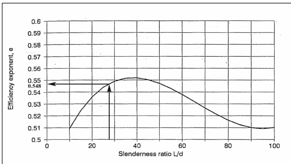
Figure B1 Efficiency exponent for pile group stiffness (after Randolph, 1994)
