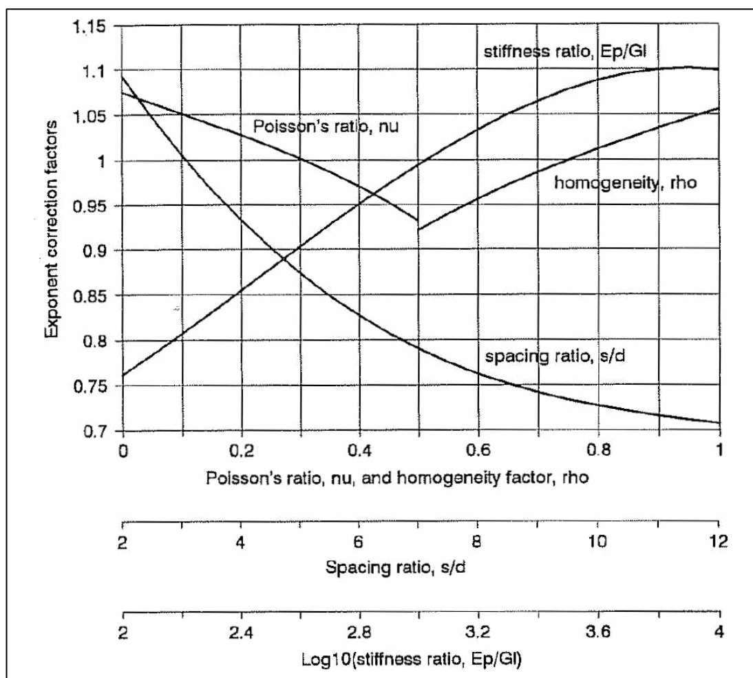
Figure 2.39 Exponent correction factors (Randolph, 1994)
