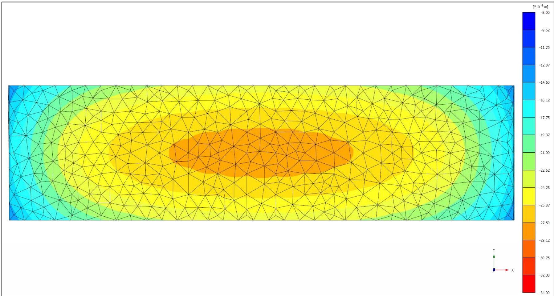
Figure 4.12 Settlement contours for first (distributed load) model at z = -5.3 plane (Units are mm)
