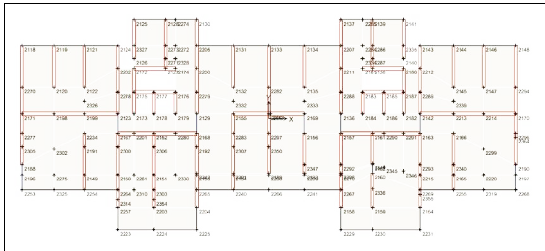
Figure 4.5 Plan view of ETABS model for single structural block
