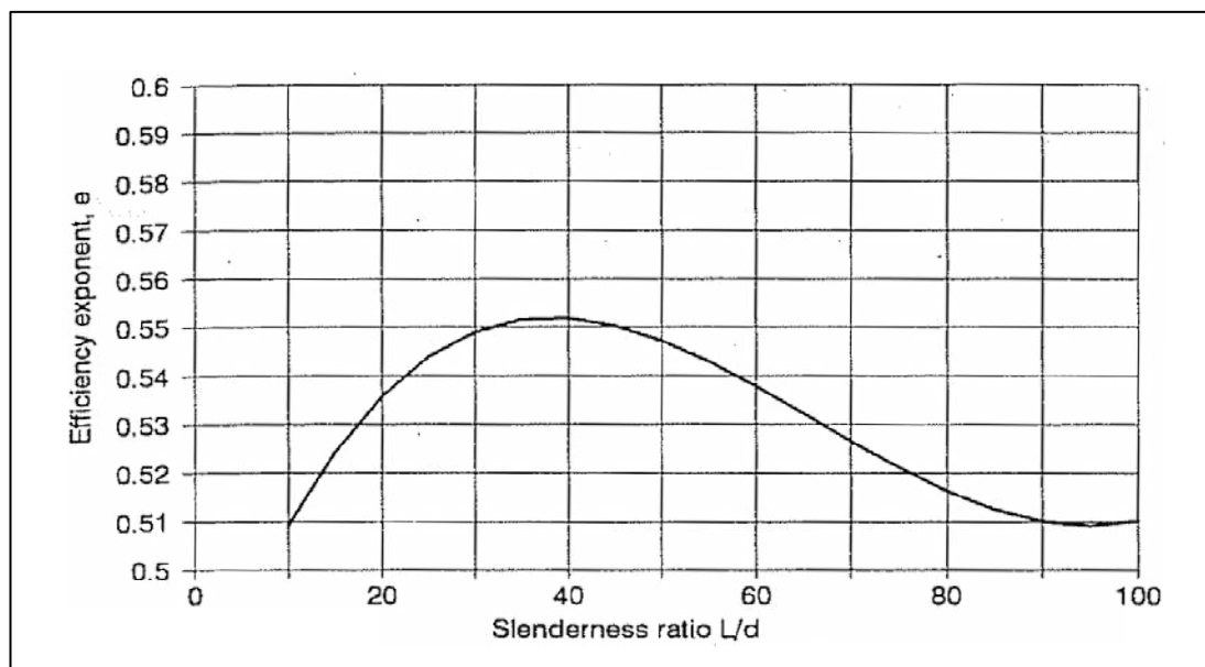
Figure 2.38 Efficiency exponent for pile group stiffness (Randolph, 1994)
