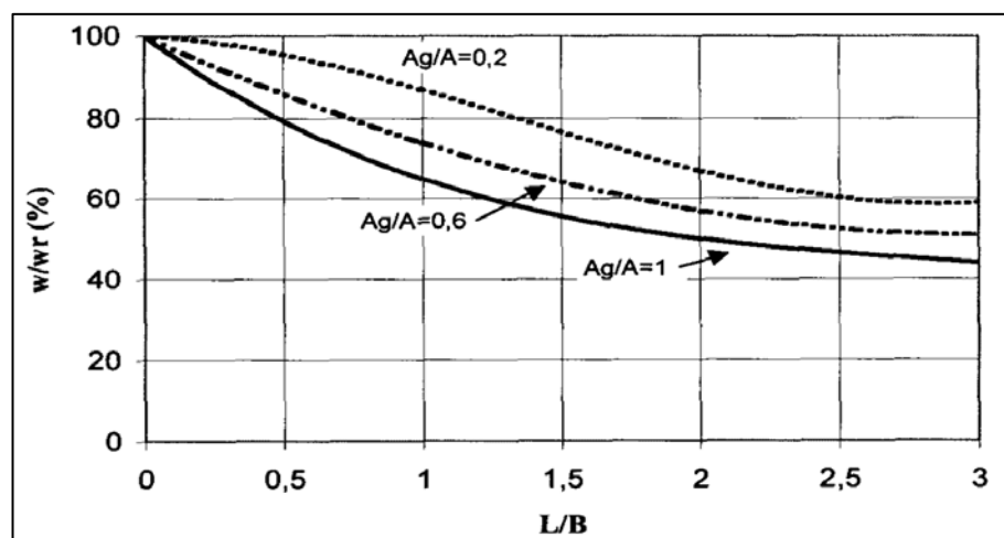
Figure 2.12 Average settlement reduction for “small piled rafts” (De Sanctis et al., 2002)
