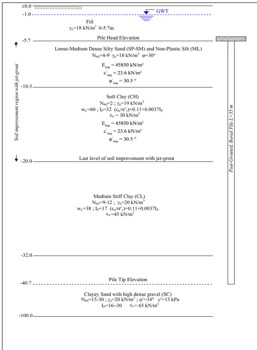
Figure 4.7 Idealized soil profile (with improved soil parameters)
