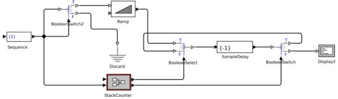
Figure 3.4: A data flow diagram representing a stack [23]
