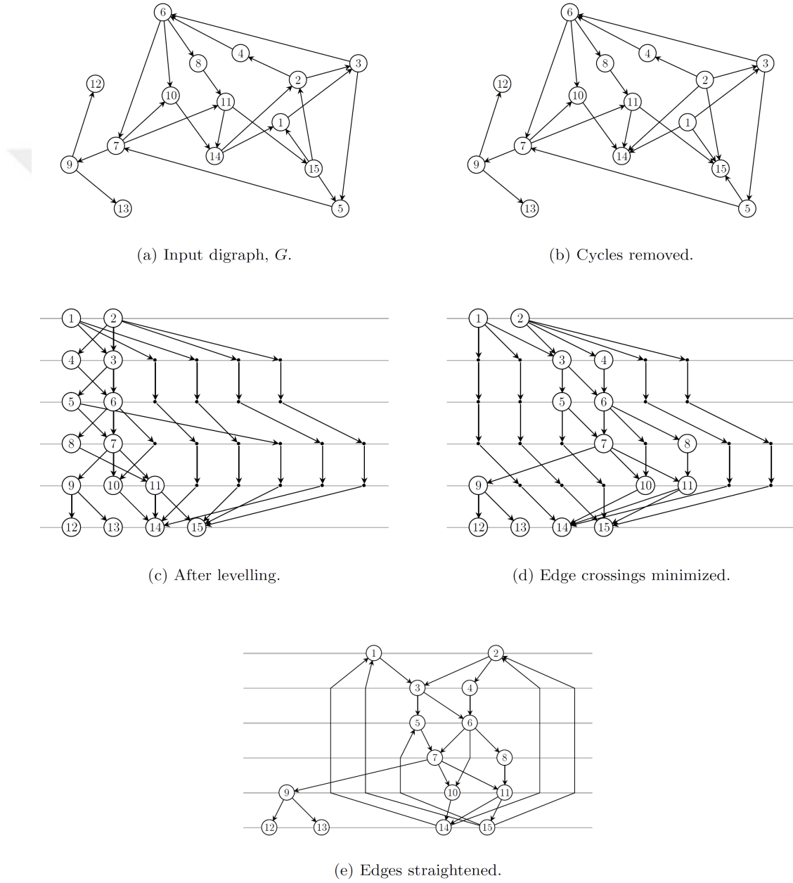
Figure 2.6: A directed graph drawn according to the Sugiyama framework [18] with polyline edge routing
