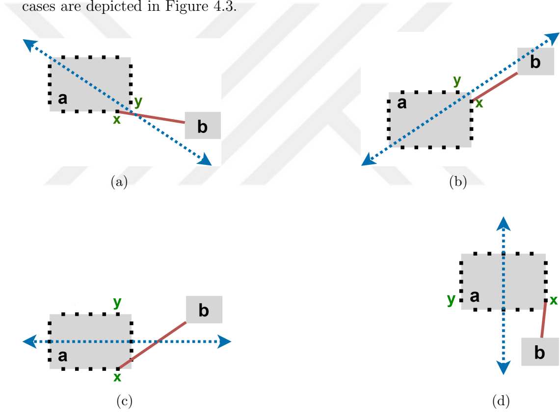
Figure 4.3: Four different cases of edge end shifting are presented. The blue dashed line indicates the other edge end's position requirement for edge end shifting. The edge end at port x can shift to port y in (a) and (c), but (b) and (d) fail the location requirement and should not be allowed to do so.
