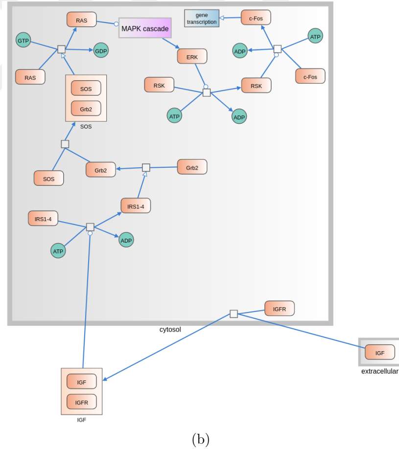
Figure A.4: An SBGN PD map illustrating insulin-like growth factor (IGF) signaling is laid out with CoSE (a) and CoSEP (b) using Fixed Sided and Fixed Position constraints. Respective metrics (CoSE - CoSEP): ratio of properly oriented edge ends: 48.27% - 100%, number of edge-edge crossings: 10 - 0, running time 38.7ms - 96.44ms
