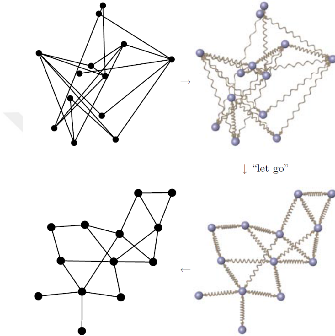
Figure 2.4: A physical analogy of the force-directed algorithms [13]
