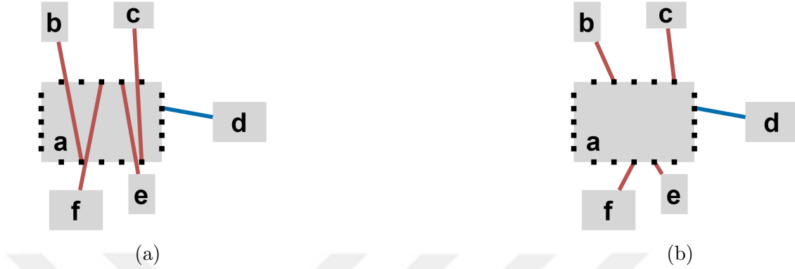
Figure 4.4: An example, where the rotational force of node a does not exceed the threshold in (a). Performing a 180^\circ rotation on node a , however, creates a more stable system (b)
