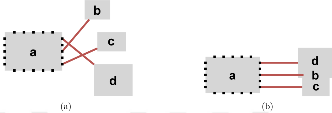
Figure 4.6: An example where a node a is connected to nodes b , c and d via Fixed position port constrained edges. Since repulsion and spring forces are stronger than polishing forces, the edge crossing in (a) will not be removed. The proposed heuristic resolves these edge crossings by placing the degree one nodes ( b , c and d ) directly to their ideal location (b). The node overlaps are eliminated in the later iterations through repulsion.
