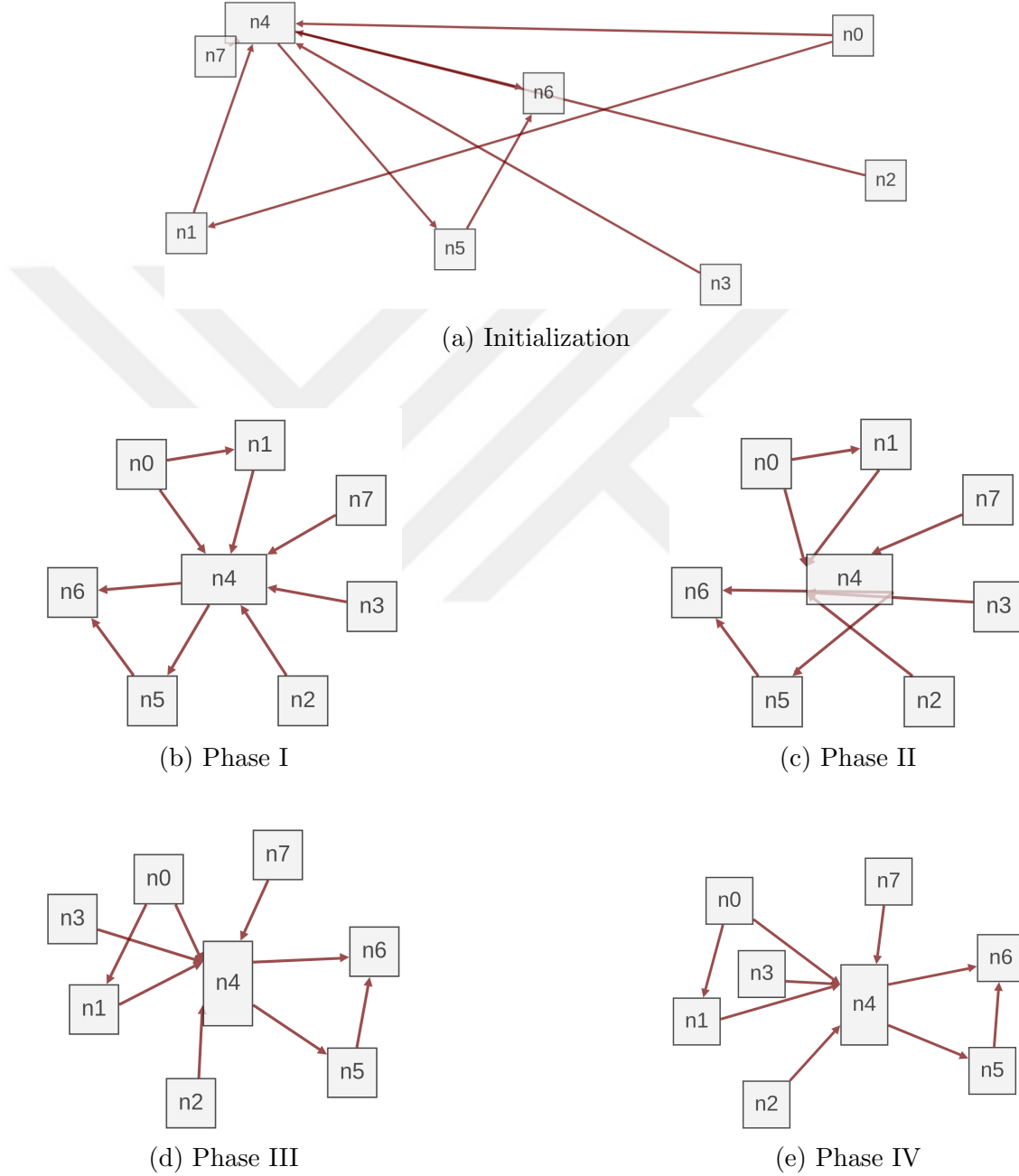
Figure 4.8: A simple graph is laid out using CoSEP algorithm while demonstrating the different phases of the algorithm. Nodes n0, n1, n2 and n3 have Fixed Sided port constraints connecting them to left of node n4 . Similarly, nodes n5 and n6 are connecting to node n4 from the right side. Whereas, node n7 should connect to node n4 from top or bottom
