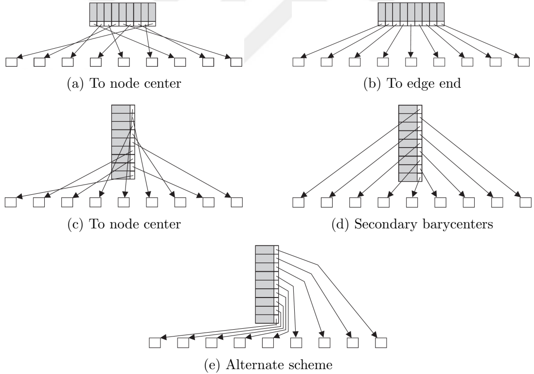
Figure 3.2: Different strategies for assigning barycenters [21]
