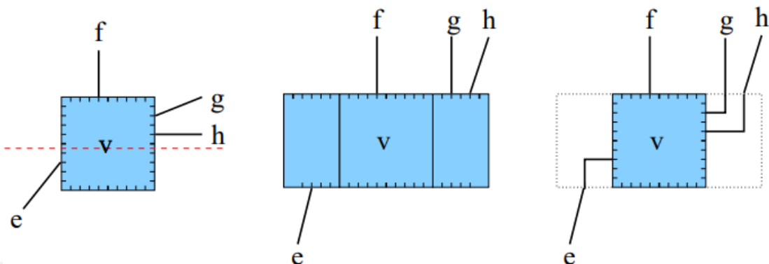
Figure 3.5: An example of Siebenhaller’s technique of rerouting right and left side ports to top or bottom [24]
