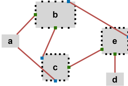
Figure 5.1: Nodes a, b, c, d , and e are connected to each other via port constrained edges. Among the nine port constrained edge ends, five of them (connected to green ports) are considered properly oriented whereas the rest are improper (blue). Thus, the ratio in this layout is %55.56.
