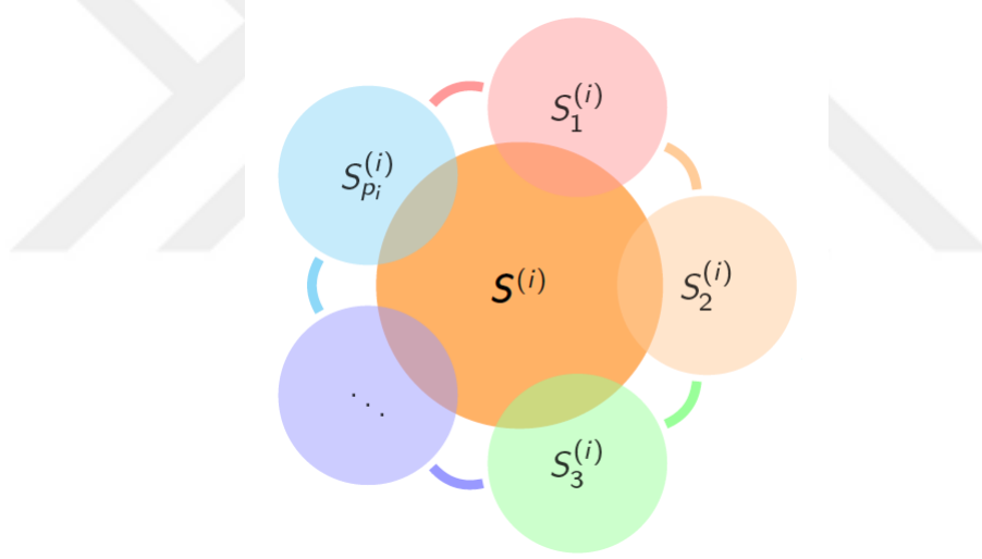
Figure 1.3: Dependency of aggregate claim rvs for a single risk cluster
