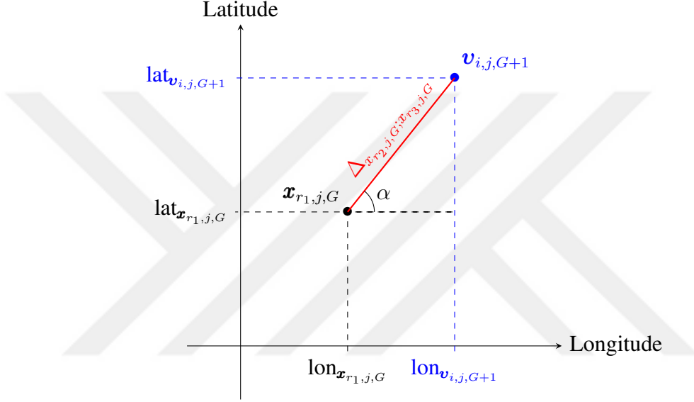
Figure 6.1: Mutation of \mathbf{v}_{i,j,G+1} for the target matrix \mathbf{X}_{i,G}
