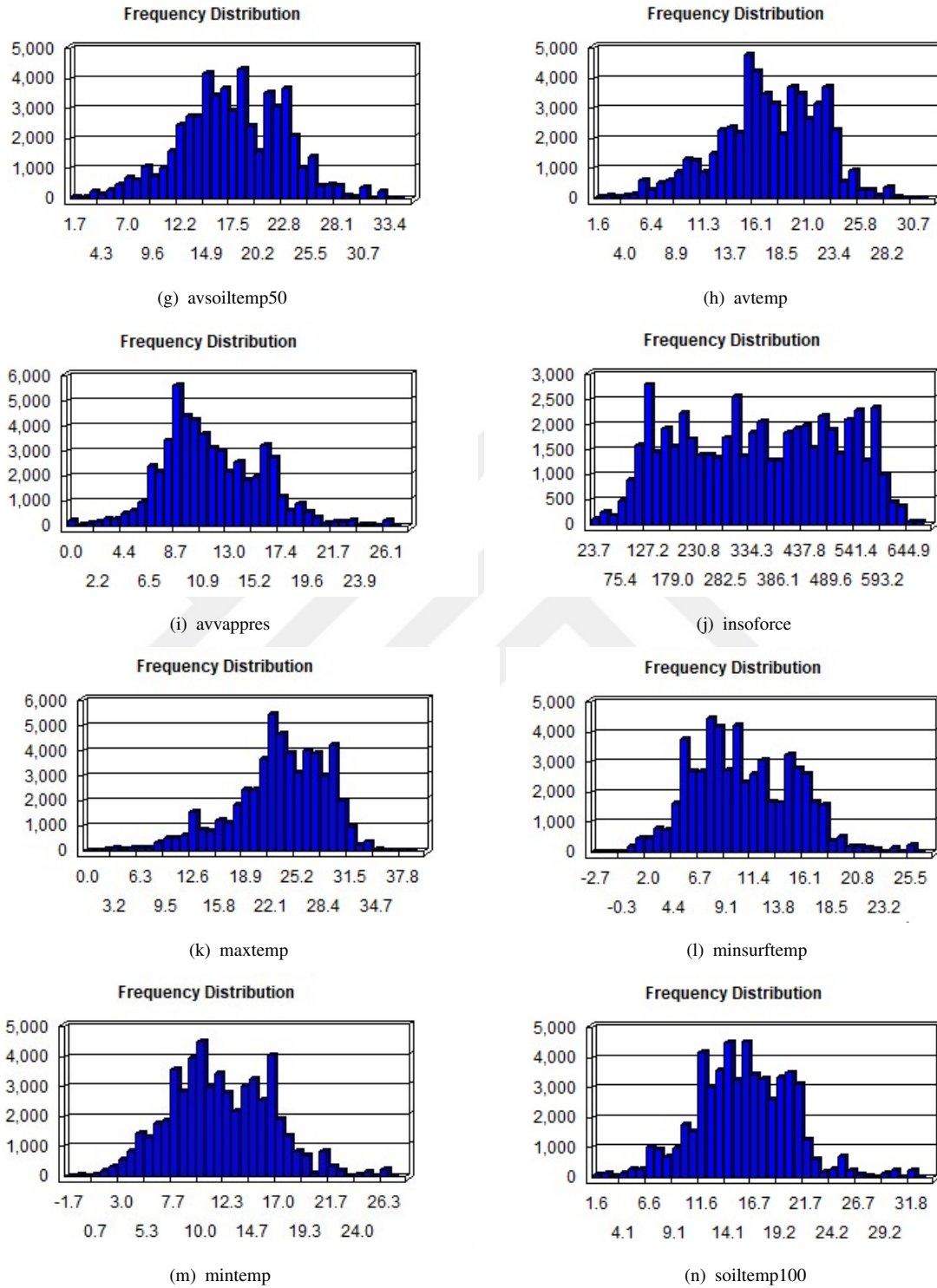
Figure A.2: The histograms of the estimated meteorological values: (g)-(n)
