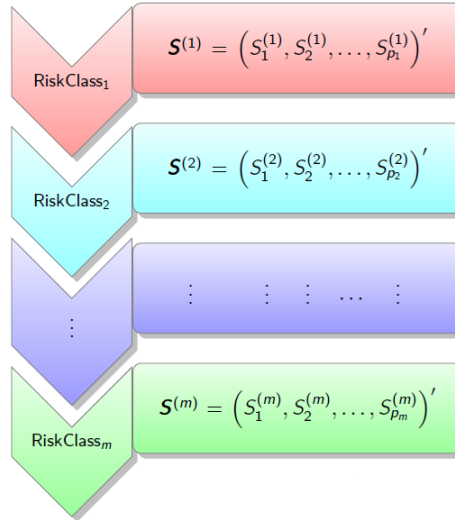
Figure 1.2: Prioritization of aggregate claim r.vectors of risk clusters
