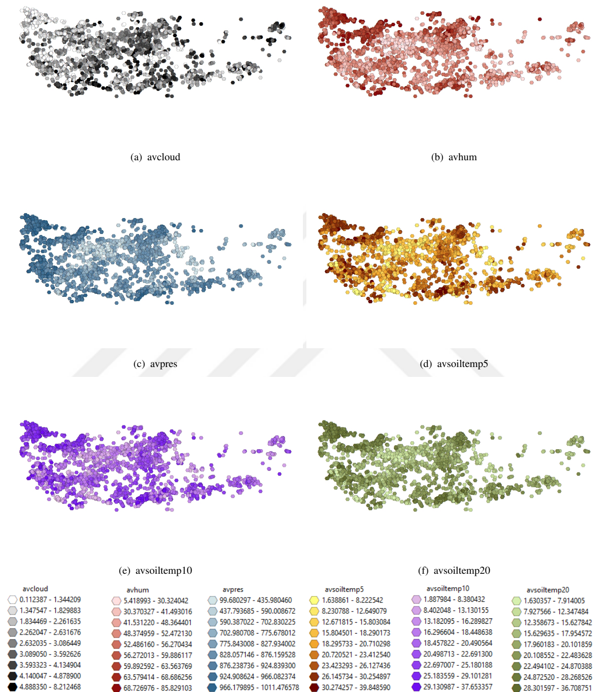
Figure 6.4: Choropleth maps for the estimated meteorological values related to the reported agricultural claims using IDW reduction technique: (a)-(f)
