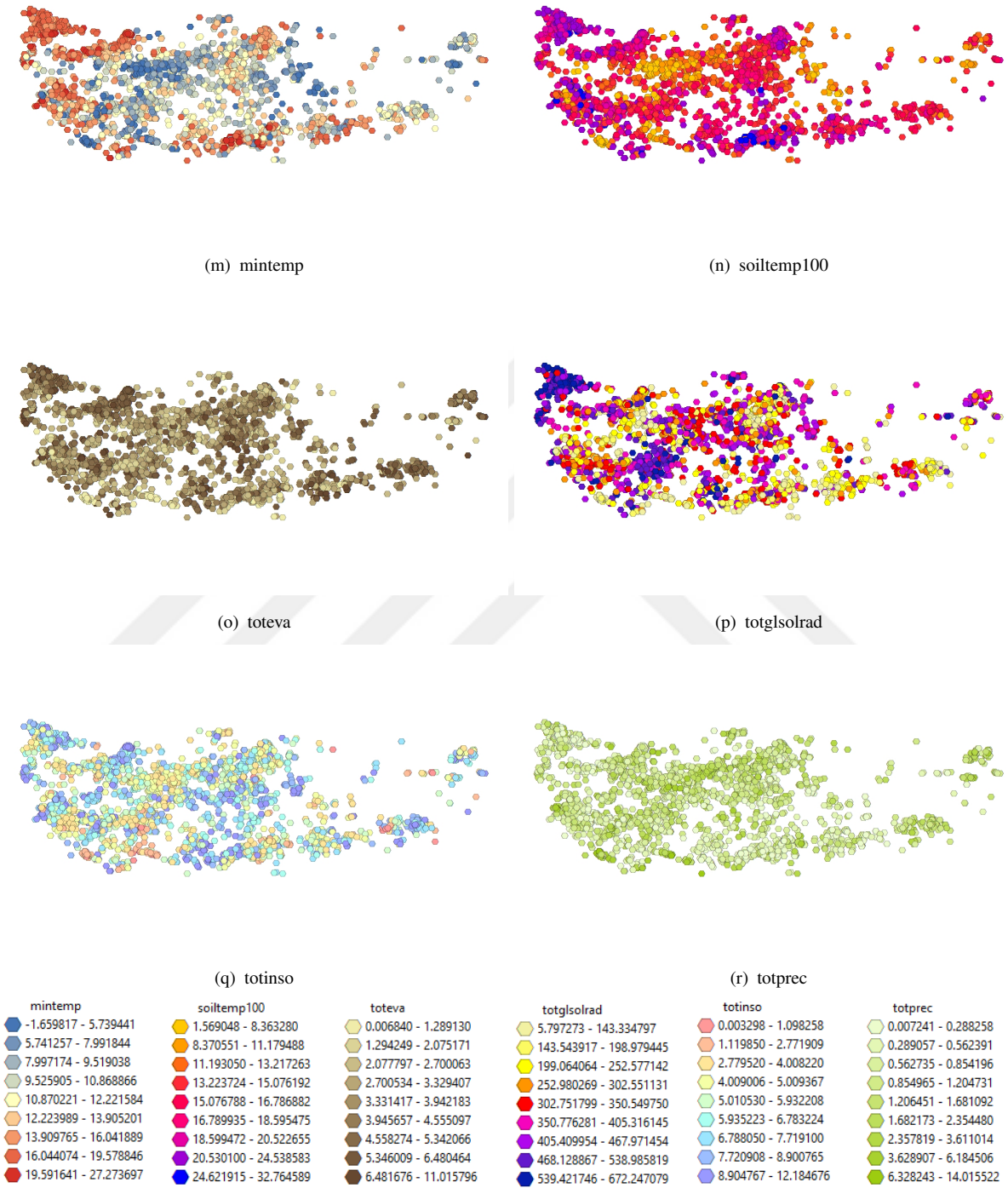
Figure 6.6: Choropleth maps for the estimated meteorological values related to the reported agricultural claims using IDW reduction technique: (m)-(r)
