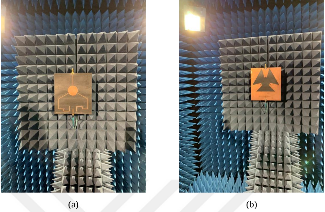
Figure 5.11: The gain measurement environment of the UWB IBFD antenna (a) front-view (b) back-view
