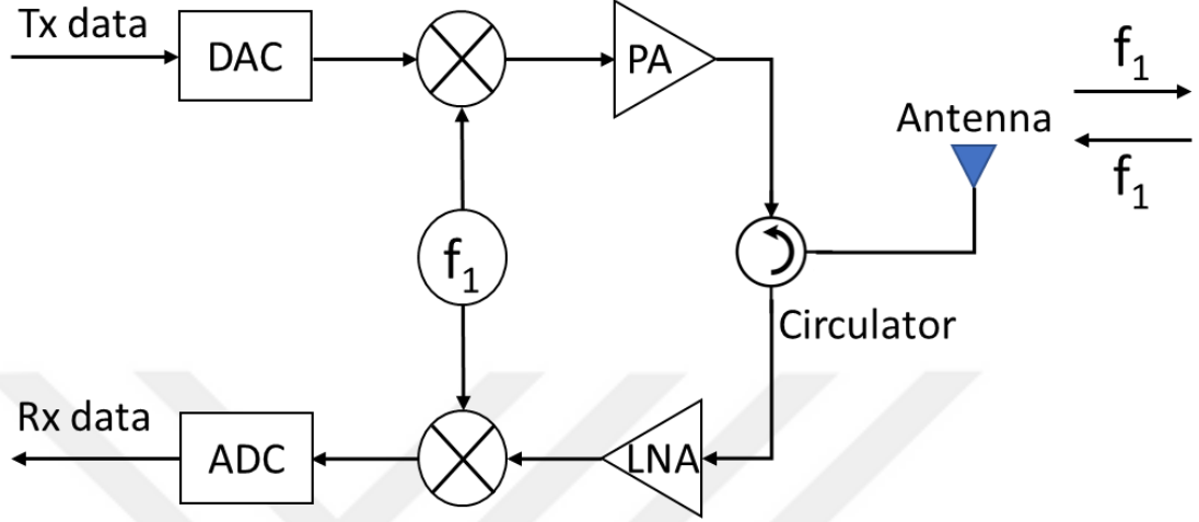
Figure 2.4: Block diagram of full duplex transceiver by using three-port routing device
