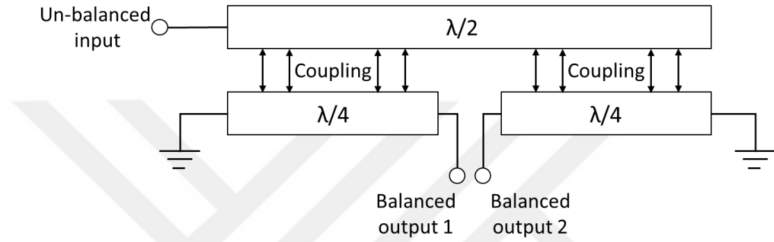
Figure 3.1: Operating principles of Marchand coupler
