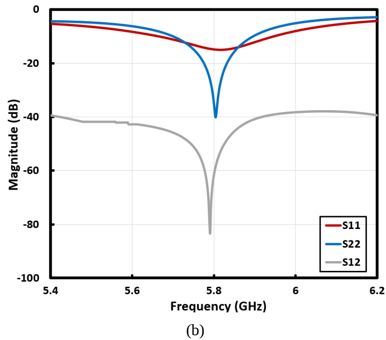
Figure 3.9: 5.8 GHz IBFD differential fed microstrip patch antenna array (a) HFSS design (b) Simulation results of S-parameters
