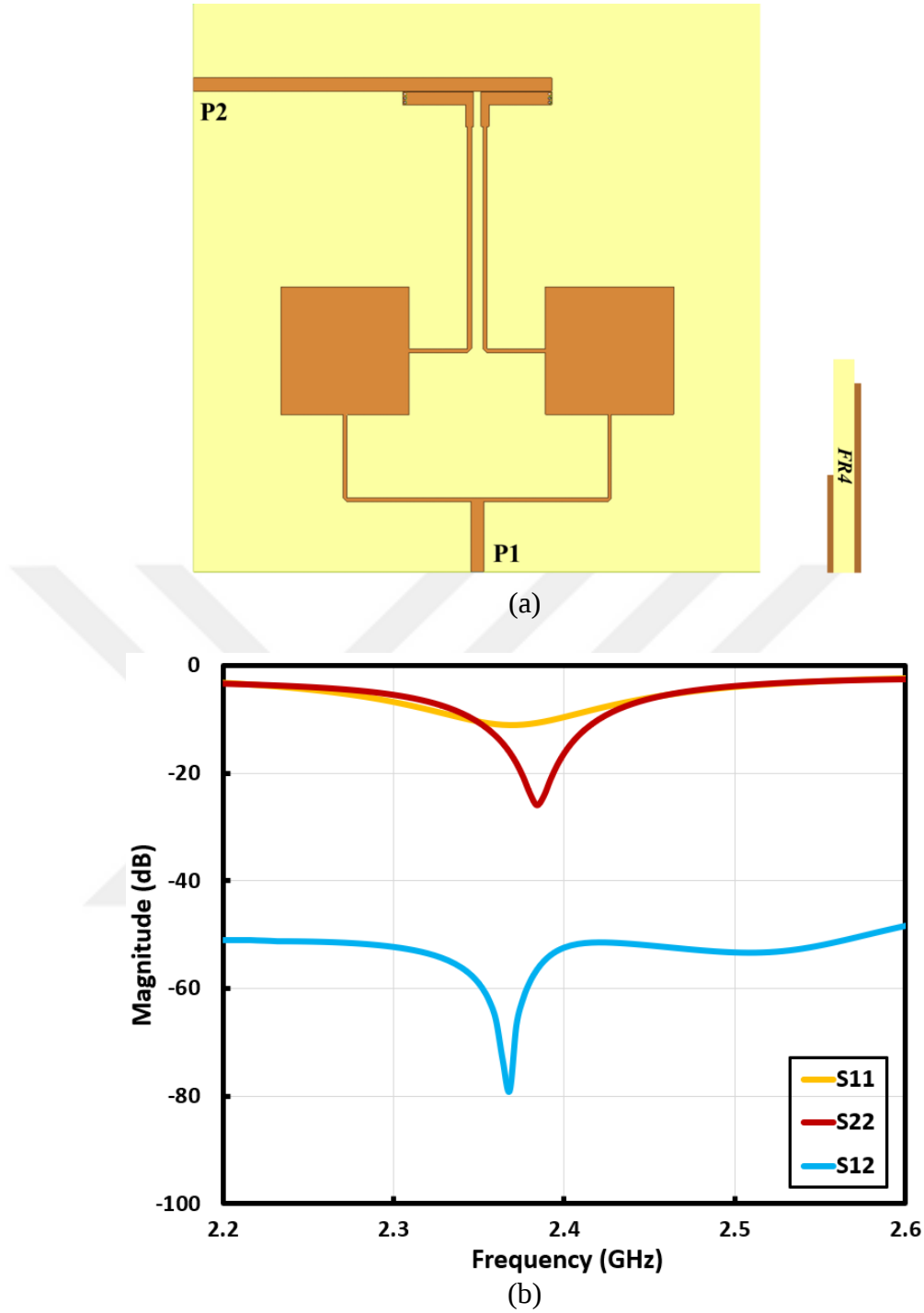
Figure 3.6: 2.4 GHz IBFD differential fed microstrip patch antenna array (a) HFSS design (b) S-parameters simulation results
