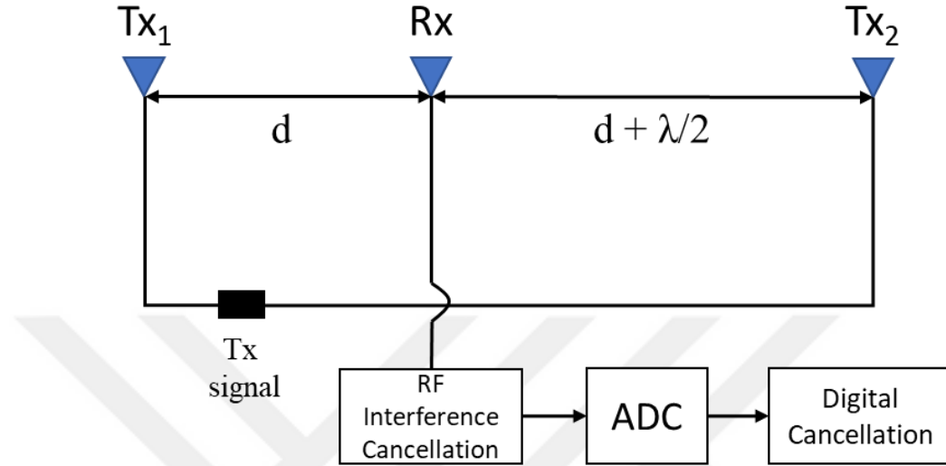
Figure 2.5: Block diagram of Multiple antenna SI cancellation
