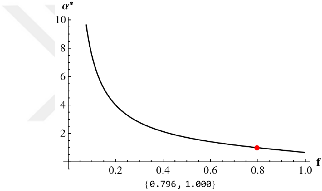
Figure 3: The change in \alpha^* with respect to f .
