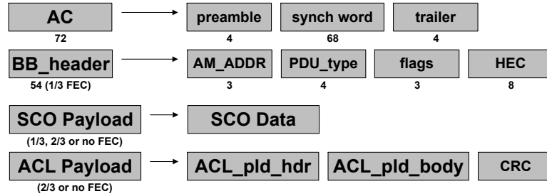
Figure 2.5: Baseband packet fields
