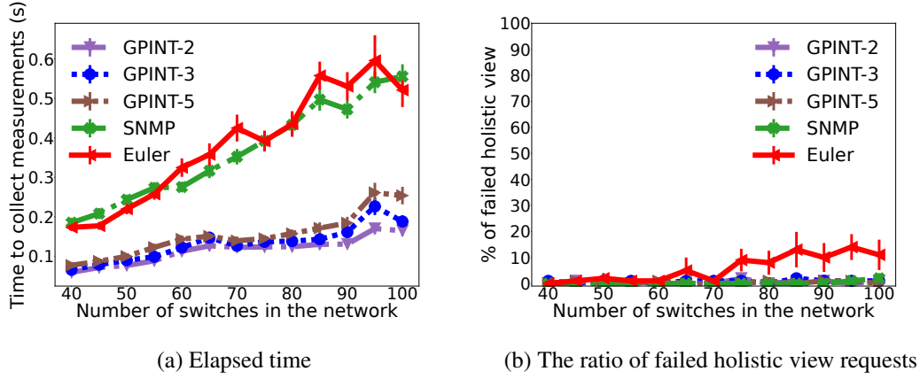
Figure 7.13: Obtained results without recovery mode on low load as |V| increases.
