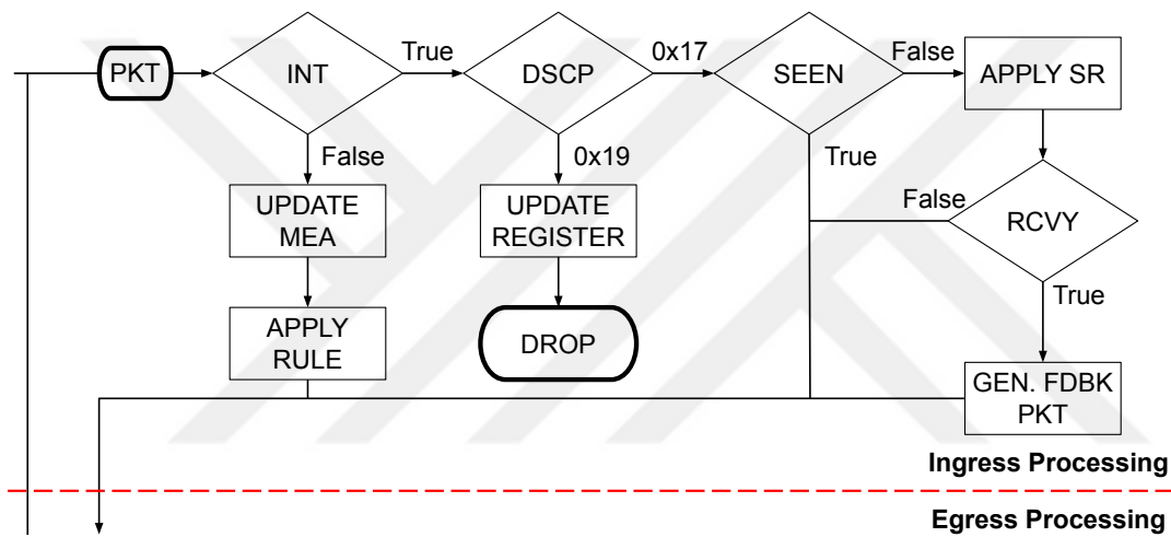
Figure 3.4: The flowchart of the ingress pipeline.
