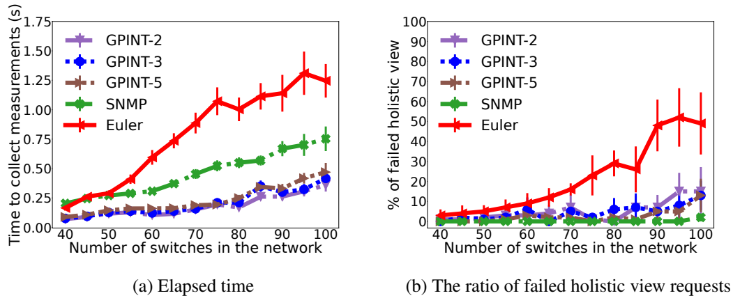
Figure 7.14: Obtained results without recovery mode on medium load as |V| increases.
