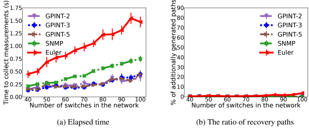
Figure 7.19: Obtained results when recovery mode enabled on low load as |V| increases.
