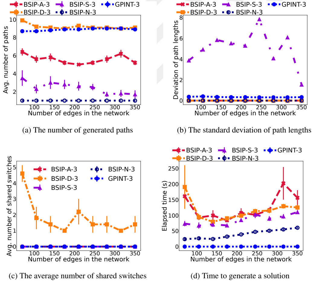
Figure 7.5: Numerical results of experiments where we increase |E| and set |V| = 35 on Watts-Strogatz graphs.
