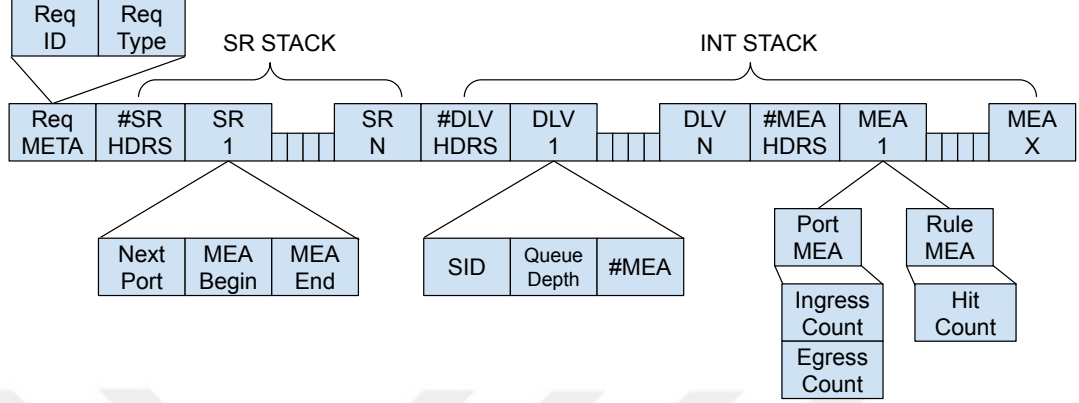
Figure 3.2: The packet layout used in this work.
