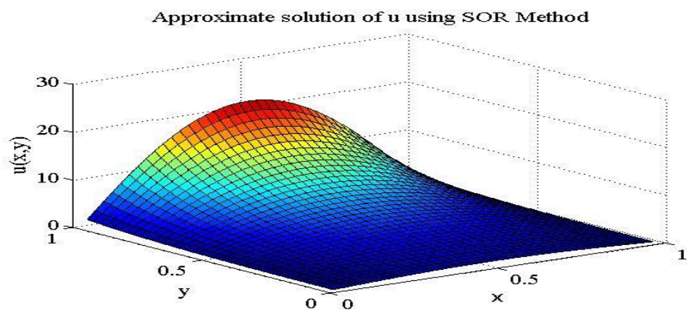
Figure 4.4: Exact and approximate solution of u using Jacobi, Gauss-Seidel and SOR methods with h = 1/40 for problem 2
