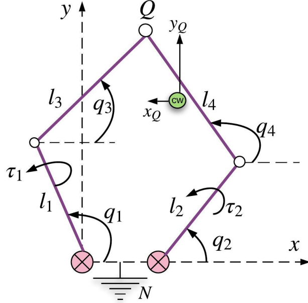
FIGURE 5.19: schematic representation of the planar manipulator
