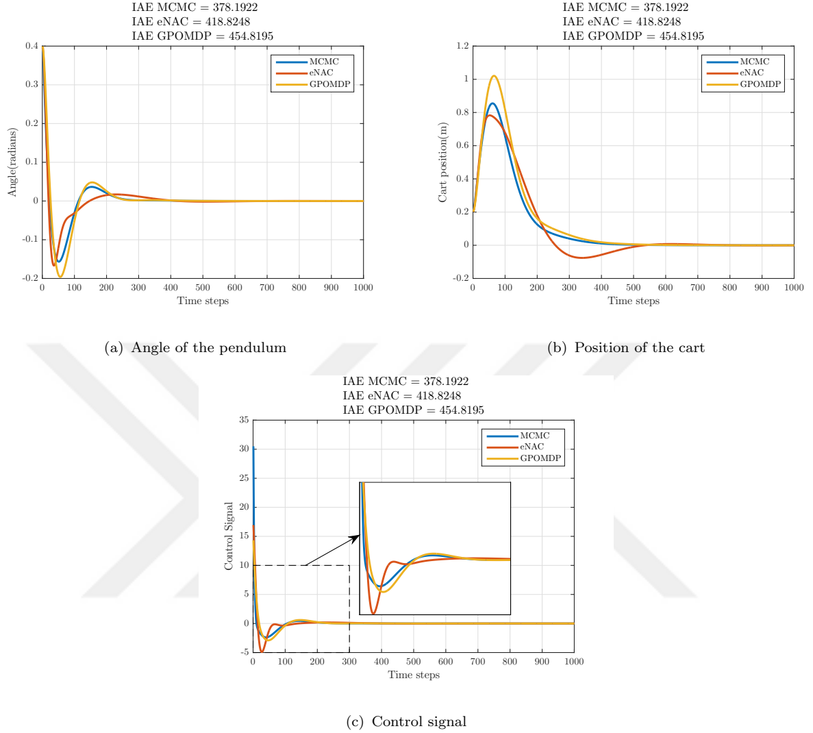
FIGURE 5.13: A sample time response for stabilization of the Cart-Pole - Quadratic reward
