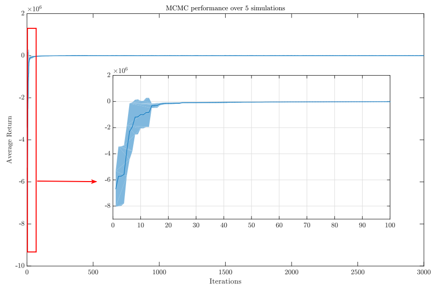
FIGURE 5.20: MCMC average return for 2-D manipulator.
