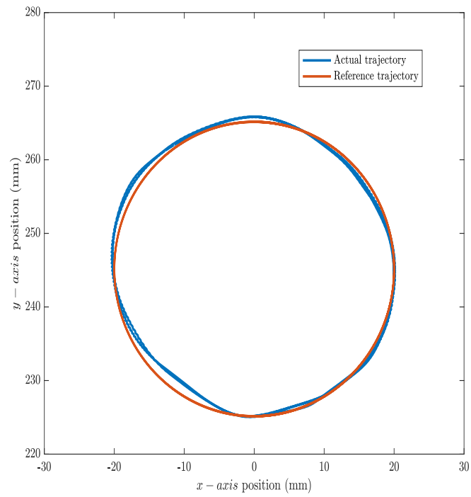
FIGURE 6.6: Desired reference and actual trajectory.
