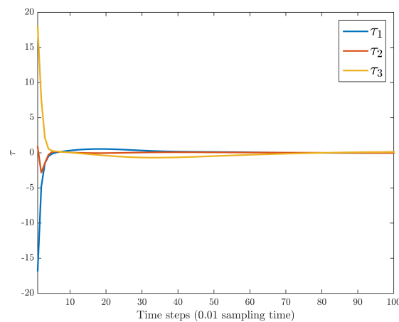
FIGURE 5.35: Time responses for the torque profiles of the adaptive MCMC for Ballbot system.
