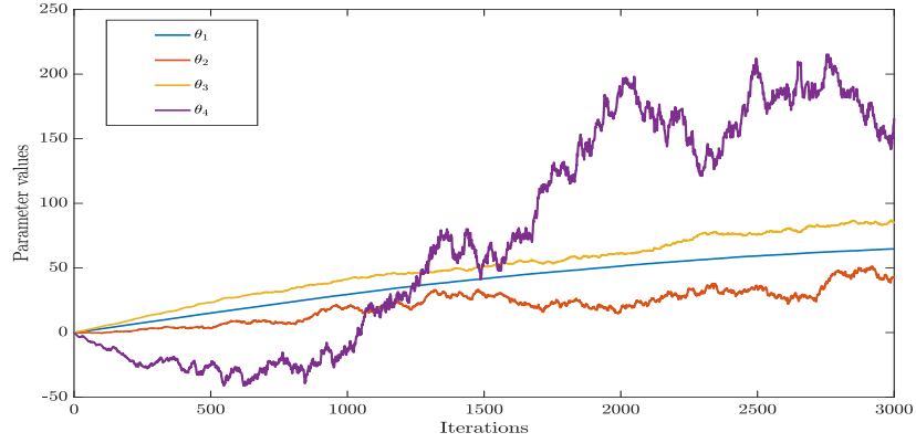
FIGURE 5.23: Trace plots for eNAC, 2-D manipulator
