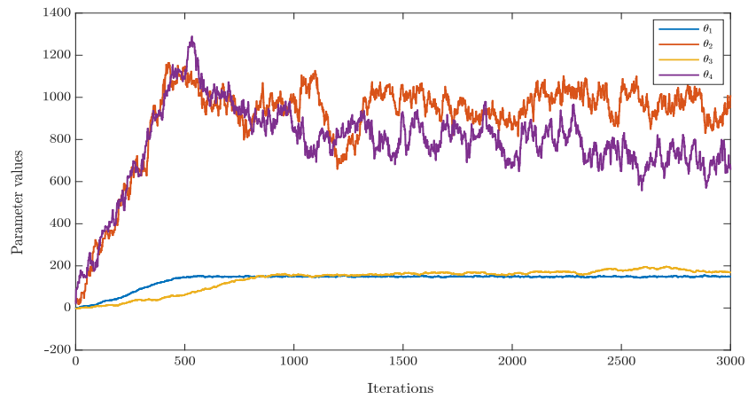
FIGURE 5.22: Trace plots for MCMC, 2-D manipulator
