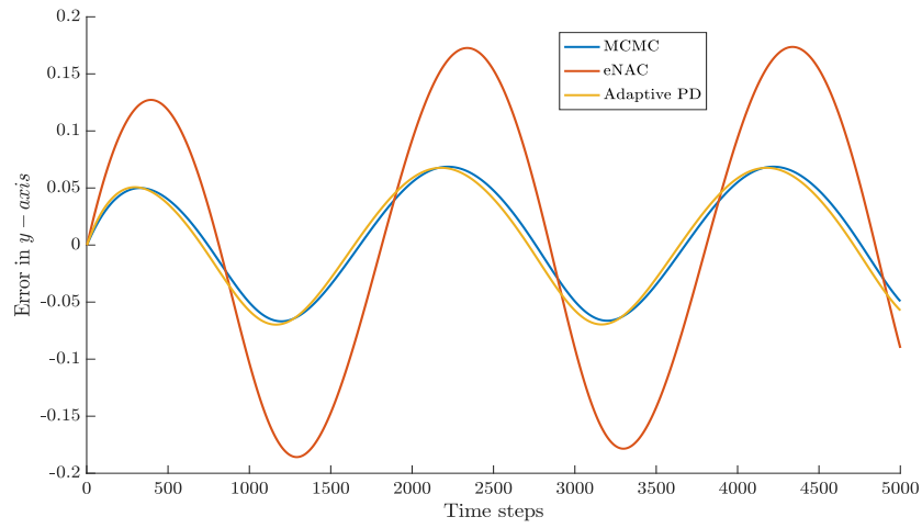
FIGURE 5.27: Error trajectory in the y -axis.
