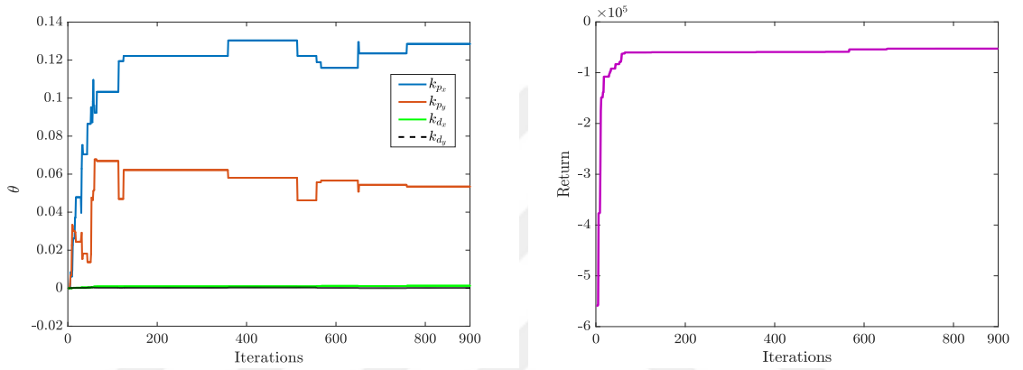
FIGURE 6.3: Trace plots and average return for physical setup of robotic manipulator: Left: Trace plots. Right: Total return
