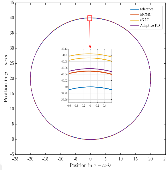
FIGURE 5.28: Circular reference and actual trajectory.
