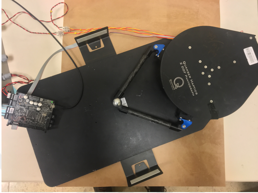
FIGURE 6.1: Physical setup for the two link manipulator.
