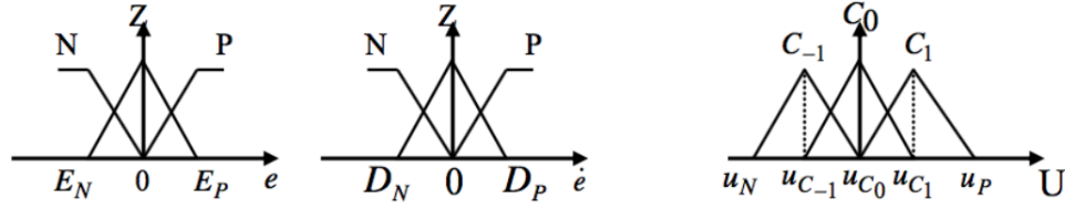
FIGURE 5.1: FLC Membership functions for the input-output.
