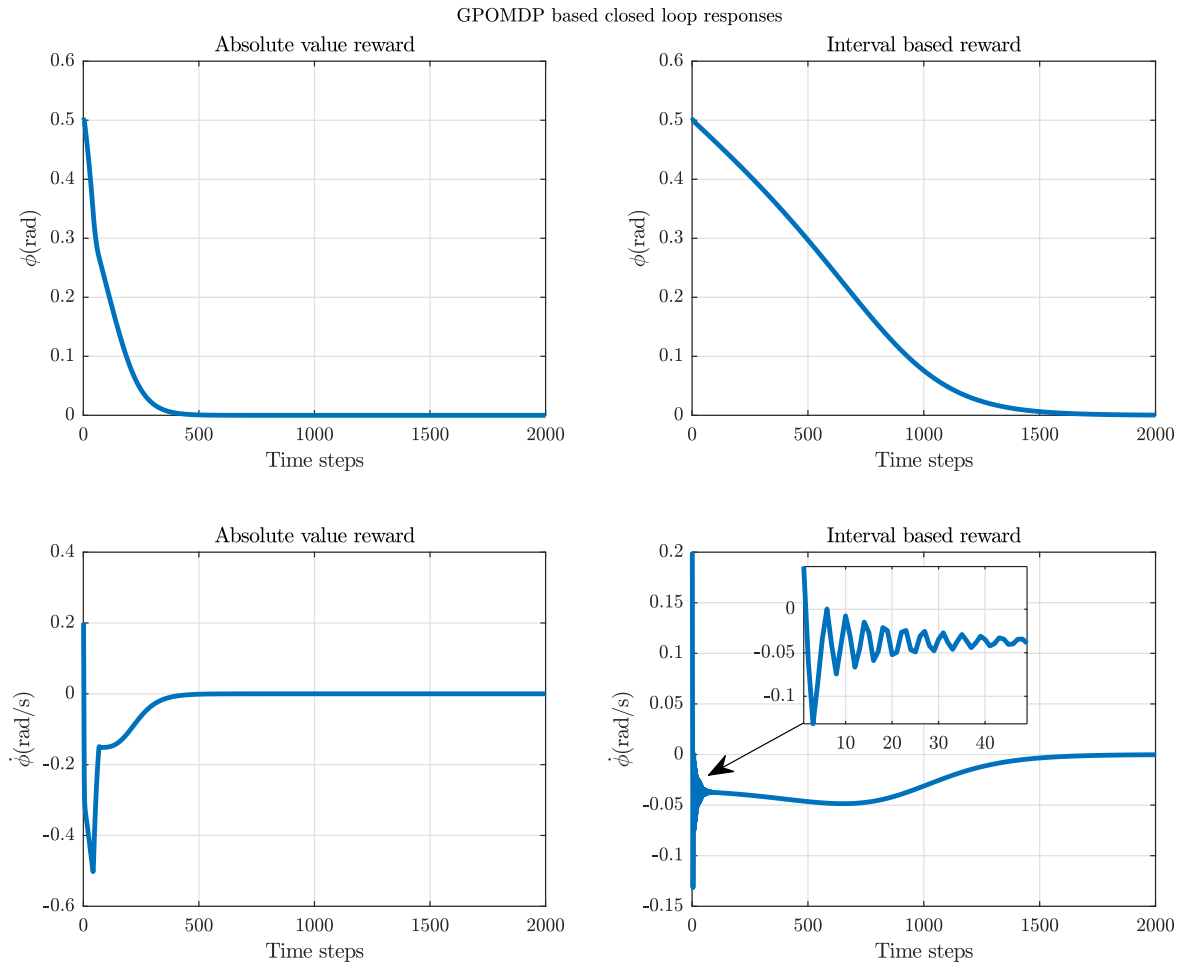
FIGURE 5.4: Closed loop responses for GPOMDP algorithm.
