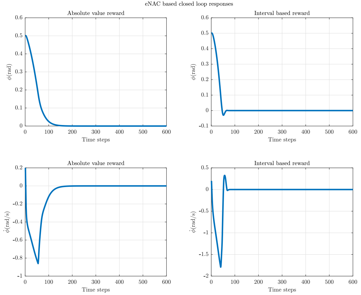
FIGURE 5.3: Closed loop responses for eNAC algorithm.
