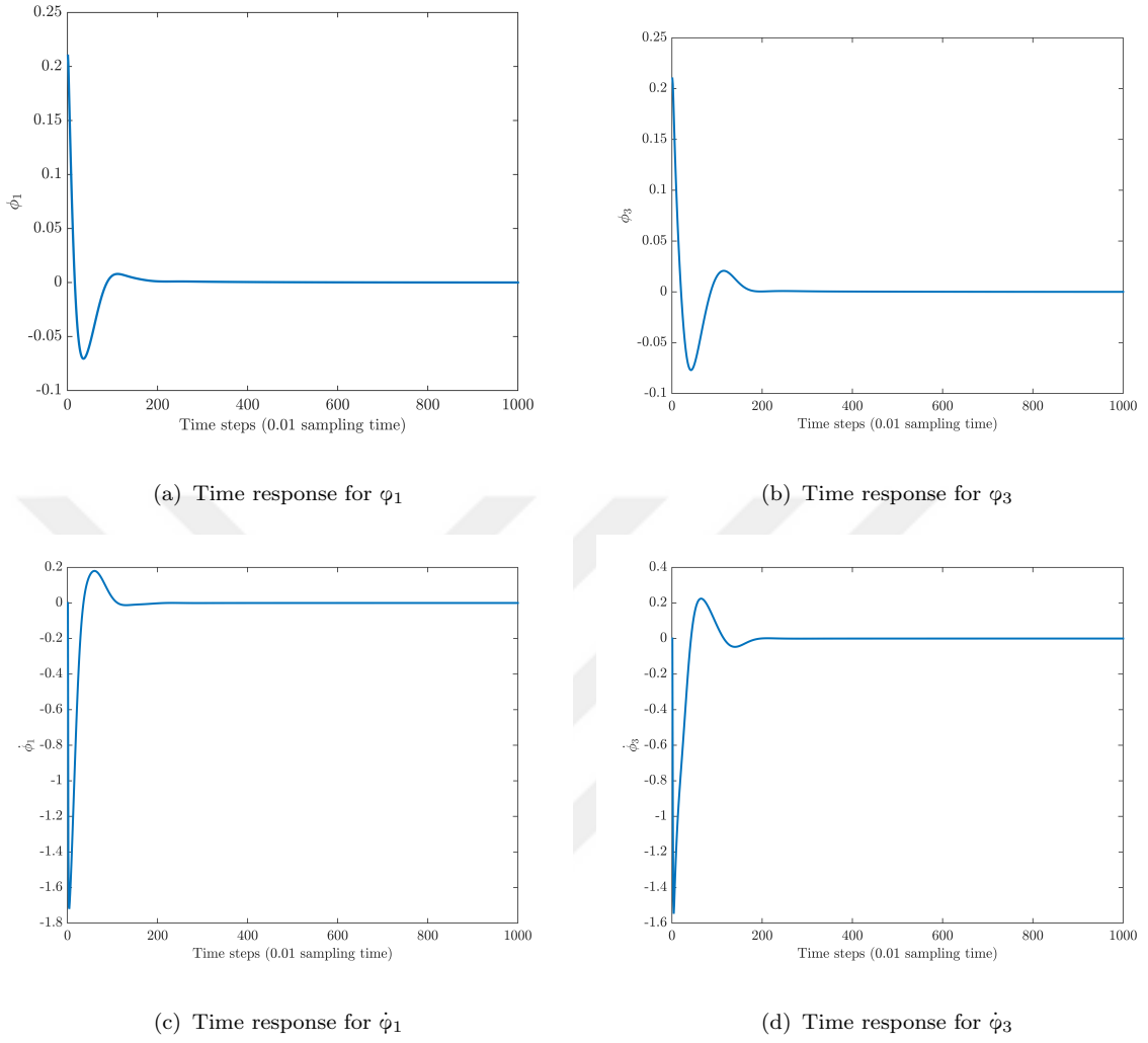
FIGURE 5.36: Time responses of the adaptive MCMC for Ballbot system.
