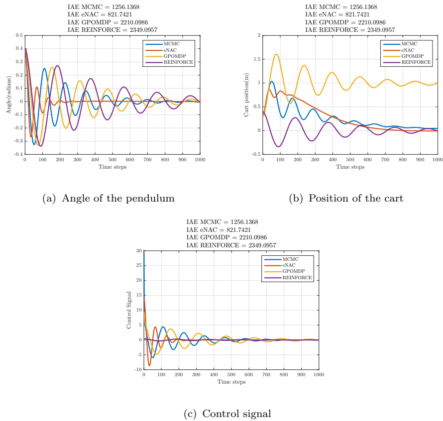
FIGURE 5.9: A sample time response for stabilization of the Cart-Pole - Interval based reward
