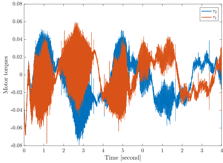
FIGURE 6.5: Torque profiles generated by motors.
