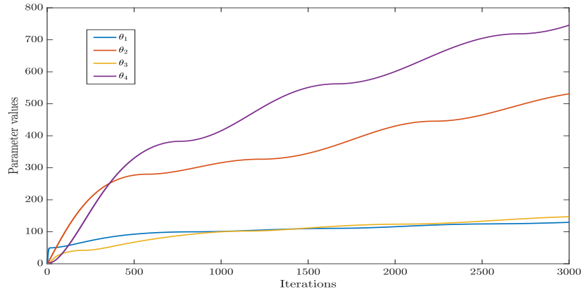
FIGURE 5.24: Trace plots for adaptive PD, 2-D manipulator
