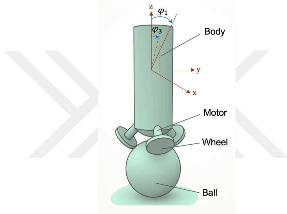
FIGURE 5.29: Model of a Ballbot system.
