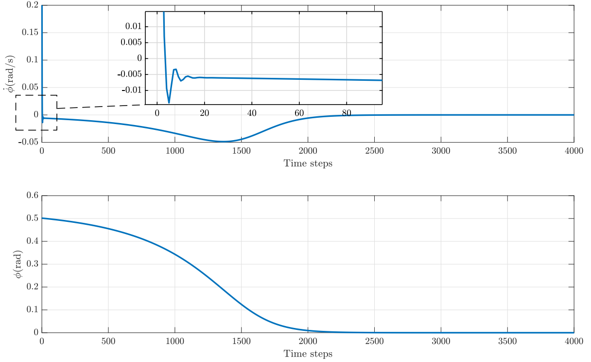
FIGURE 5.5: Closed loop responses for REINFORCE algorithm.
