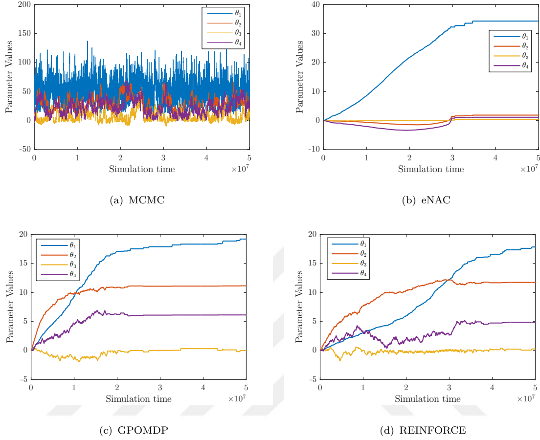
FIGURE 5.6: Trace plots for MCMC and gradient based algorithms - Interval based reward
