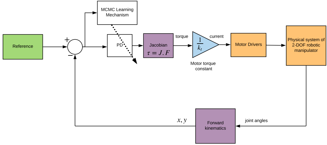
FIGURE 6.2: Learning paradigm for the trajectory control of the 2-DoF manipulator.
