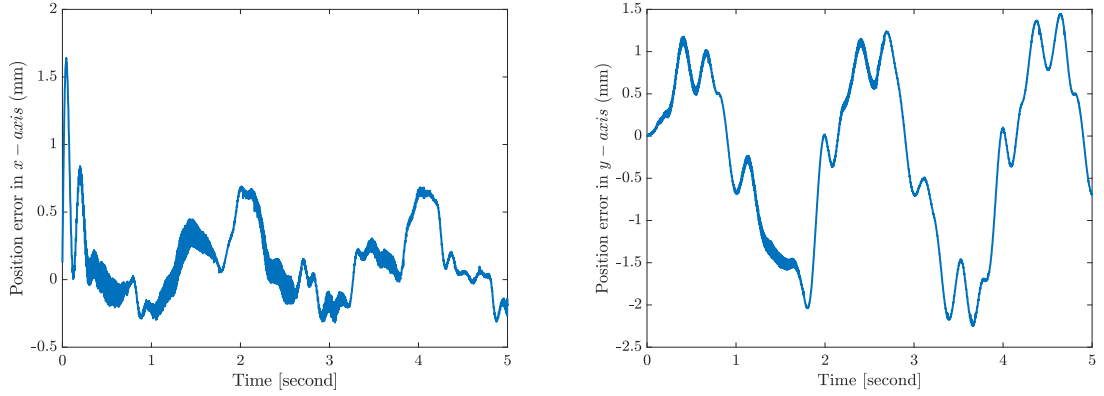
FIGURE 6.4: Position error for physical setup of robotic manipulator: Left : error in x -axis. Right : error in y -axis.
