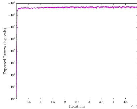
FIGURE 5.34: Expected return of the adaptive MCMC for Ballbot system.
