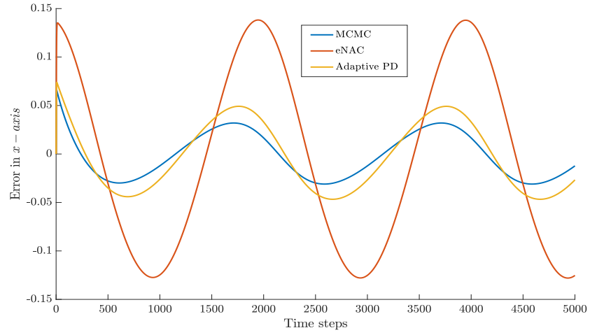
FIGURE 5.26: Error trajectory in the x -axis.
