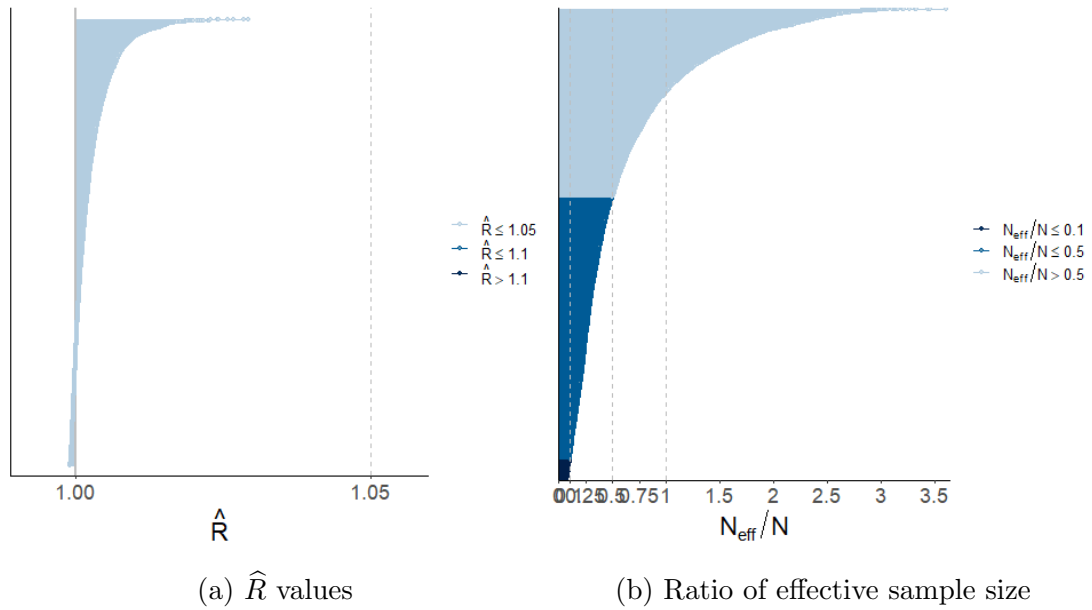
Figure 6.12: Chain diagnostics
