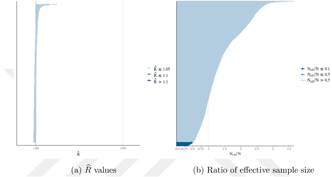
Figure 7.22: Chain diagnostics
