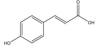
p-Kumarik asit
