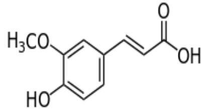
Ferulic acid
