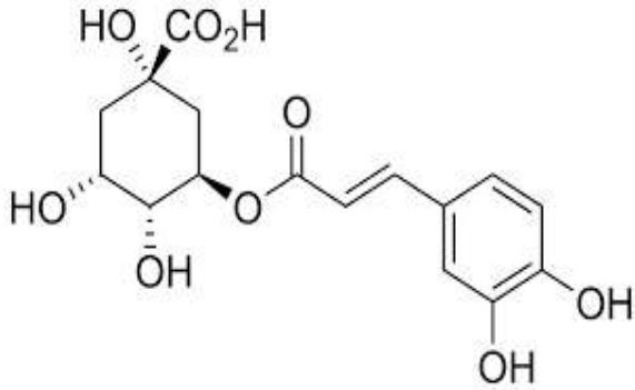
Chlorogenic acid
