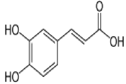
Coumaric acid
