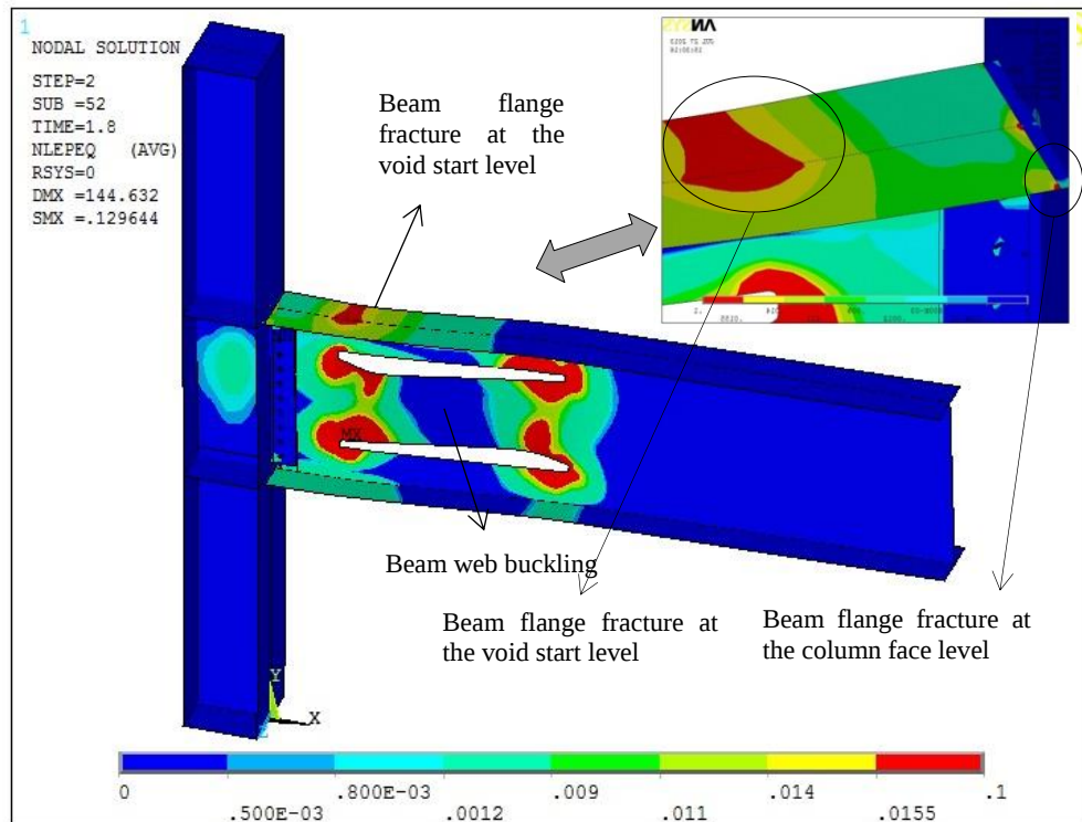
Figure 39: PEEQ distribution for modified specimen SAC7 with single voids at four percent total rotation
