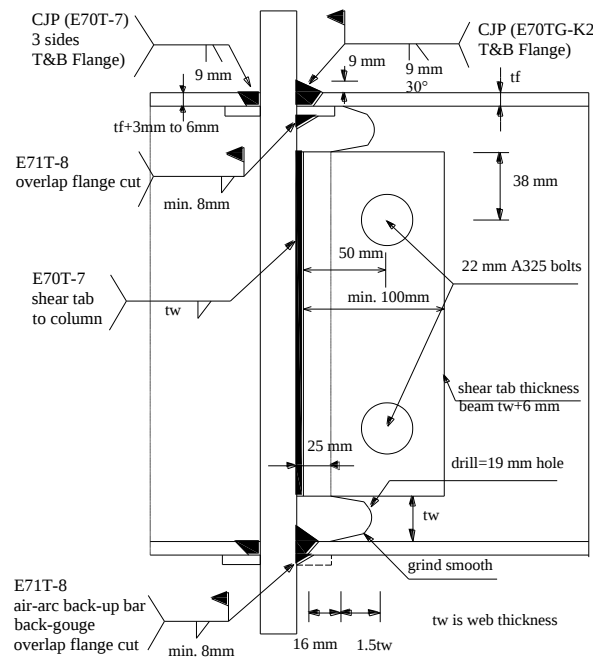
Figure 7: SAC post-Northridge connection (Lee et al., 2000)
