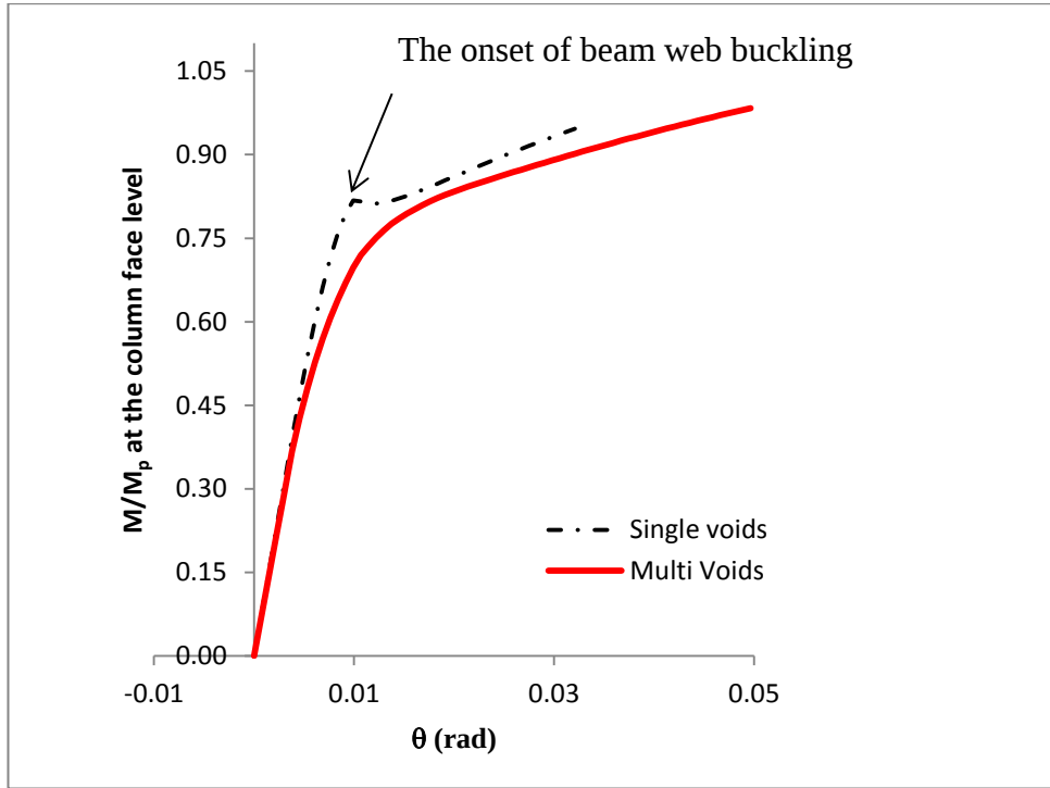
Figure 41: Normalize moment-rotation curves of modified specimens SAC7 with single and multi-longitudinal voids
