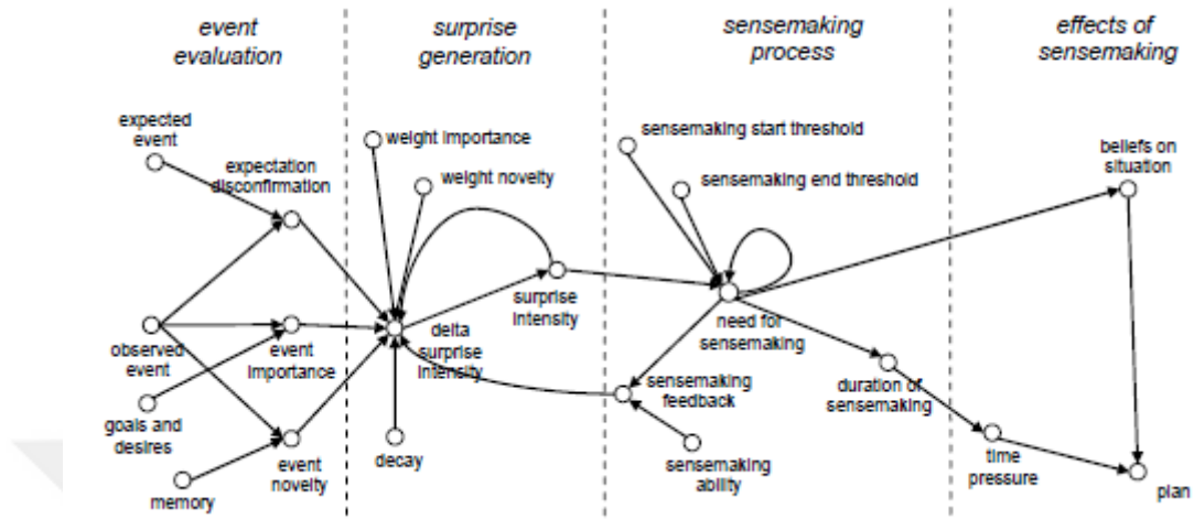
Figure 5: Computational Model of Surprise proposed by Merk. [2]
