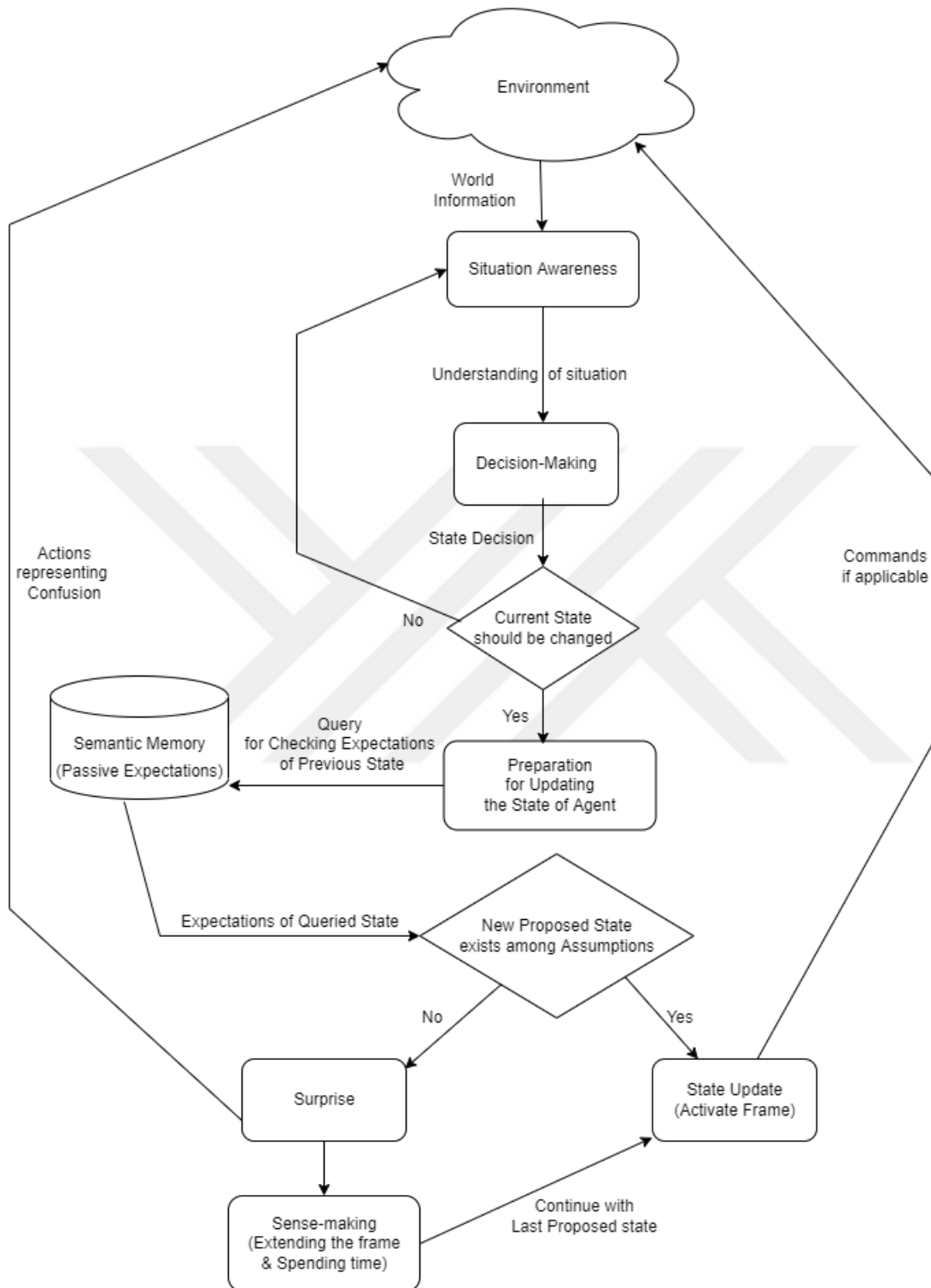
Figure 7: The flow chart diagram of the proposed model
