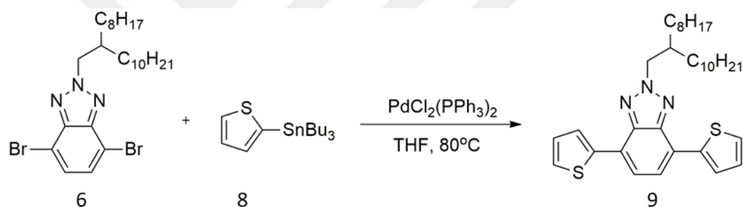
Figure 2.6. Synthesis of compound 9
