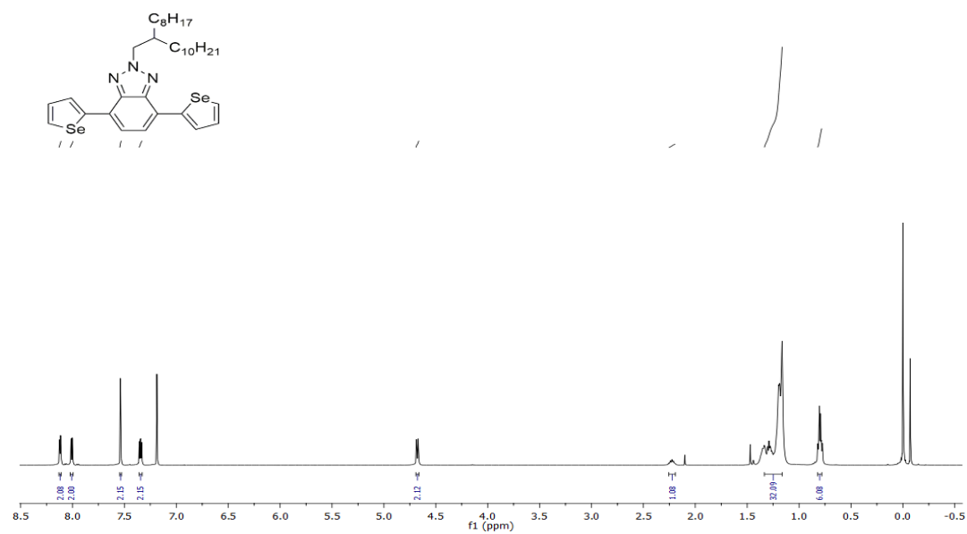
Figure A.7. ^1H NMR result of 13
