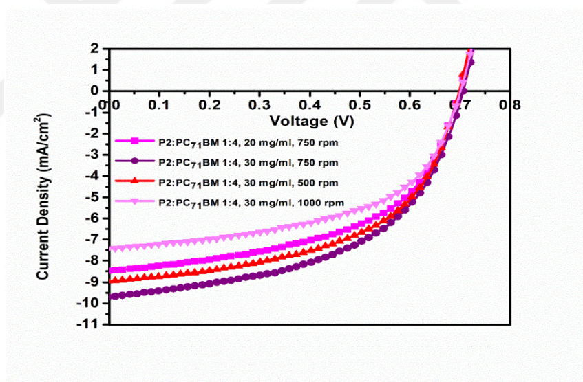
Figure 3.10. J–V curve of PSCs based on P2:PC 71 BM with different spin coating rates
