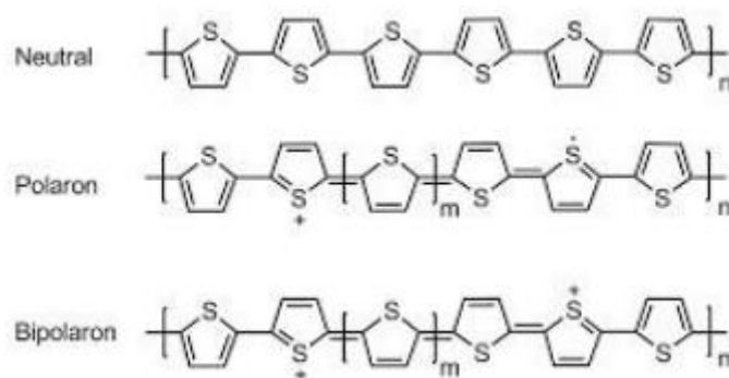
Figure 1.3. The neutral state, polaron and bipolaron state of polythiophene
