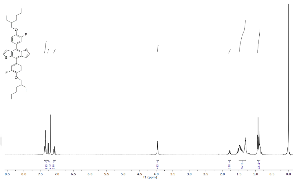
Figure A.13. 1 H NMR result of Compound 18
