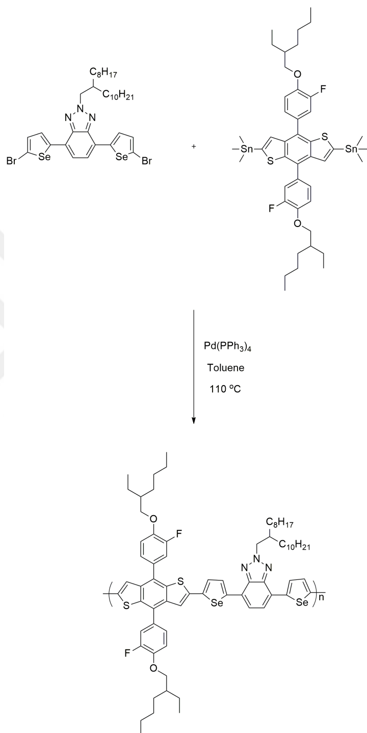
Figure 2.15. Synthesis of P2
