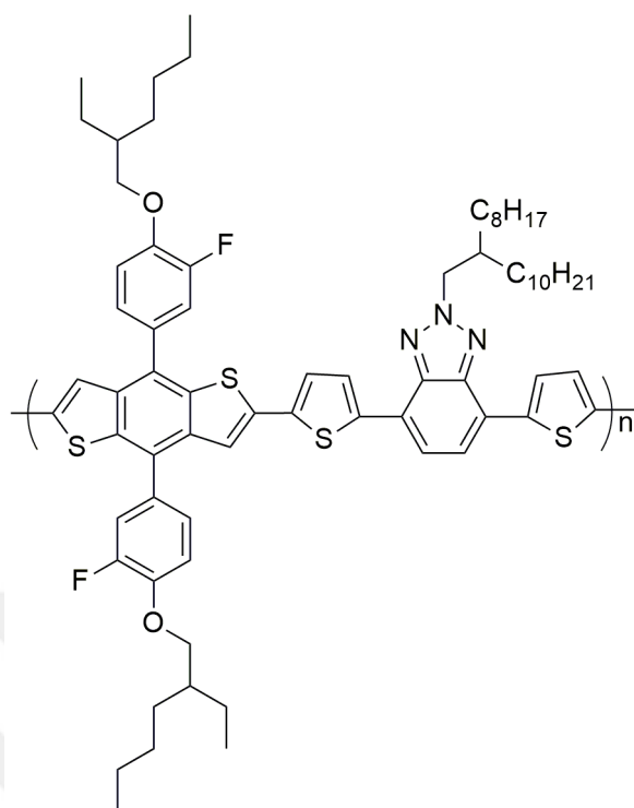
Figure 1.15. The molecular structure of thiophene containing P1
