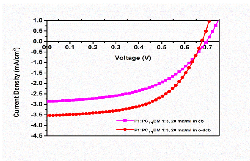
Figure 3.7. J–V curve of PSCs based on P1:PC 71 BM with different solvents
