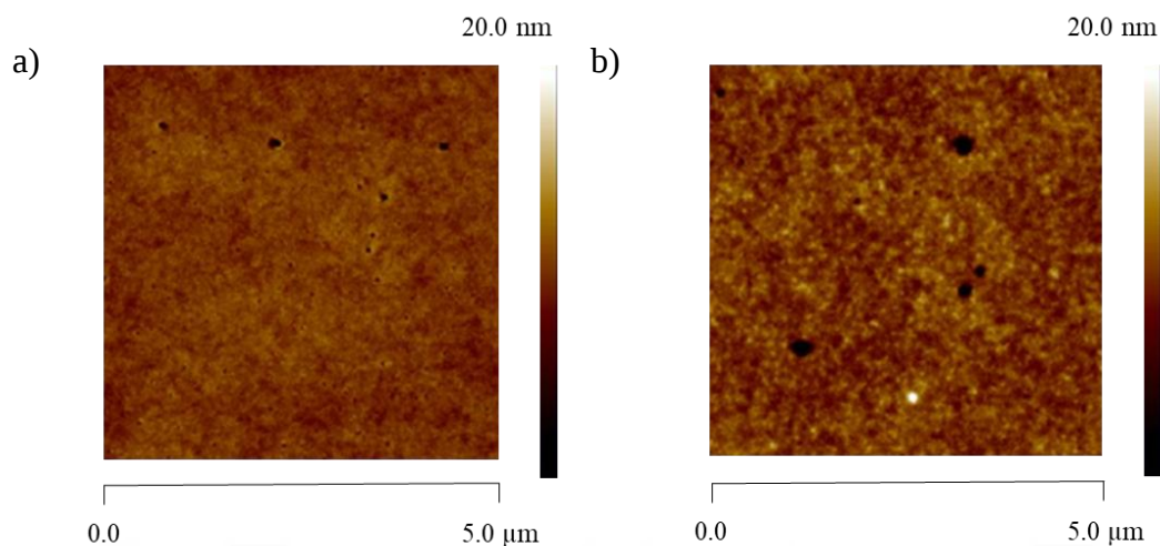
Figure 3.12. AFM images of a) P1:PC 71 BM (1:3, w/w) with 25 mg/mL blend concentration b) P2:PC 71 BM (1:4, w/w) with 30 mg/mL blend concentration
