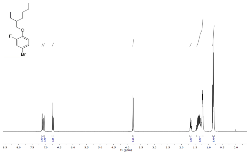
Figure A.11. 1 H NMR result of Compound 16
