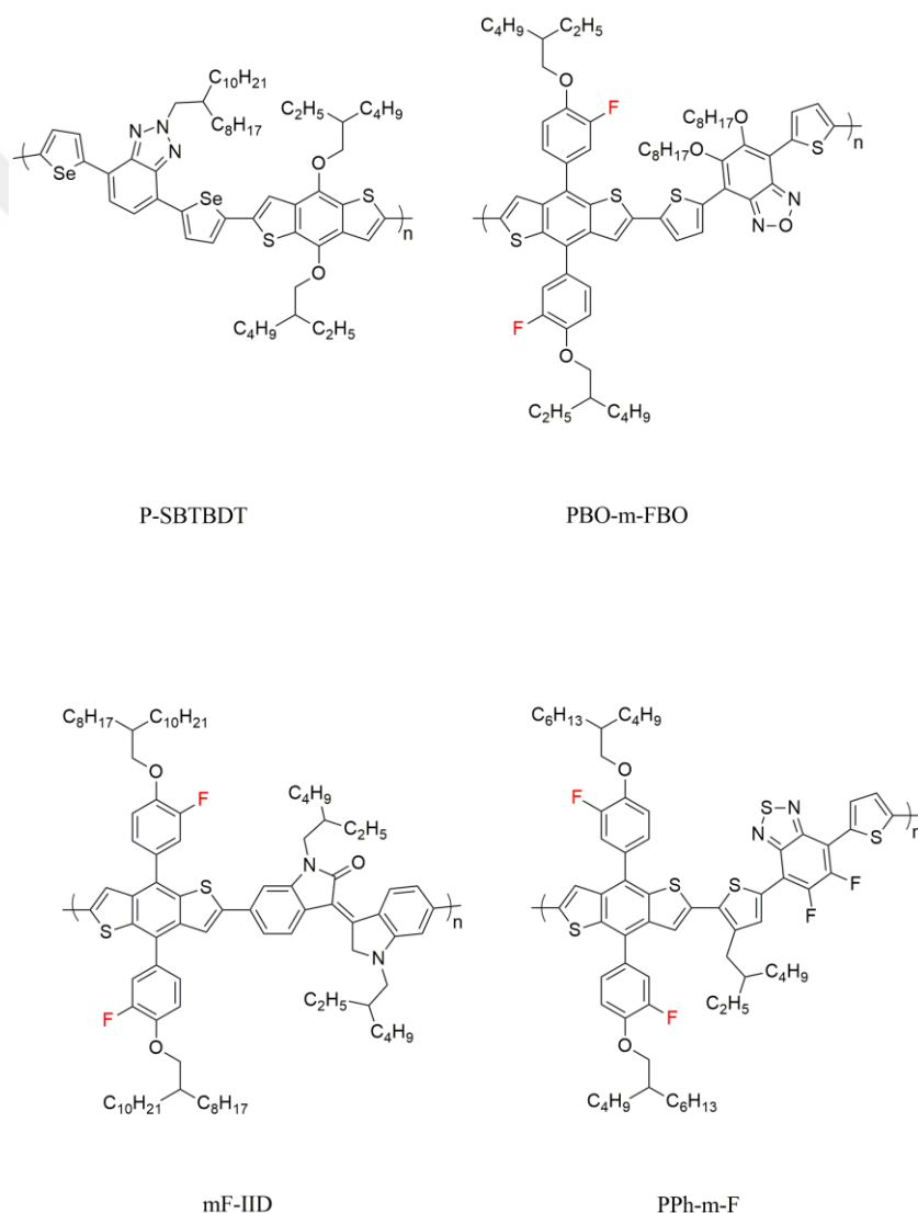
Figure 1.14. Molecular structures of BDT based P-SBTBDT, PBO-m-FBO, mF-IID and PPh-m-F
