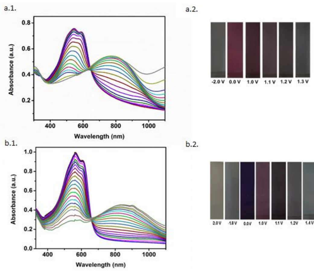
Figure 3.2 UV-Vis-NIR absorption spectra of a.1) P1 and b.1) P2 in 0.1 M TBAPF 6 / ACN electrolyte solution and the colors of a.2) P1 and b.2) P2 in the neutral, reduced and oxidized forms
