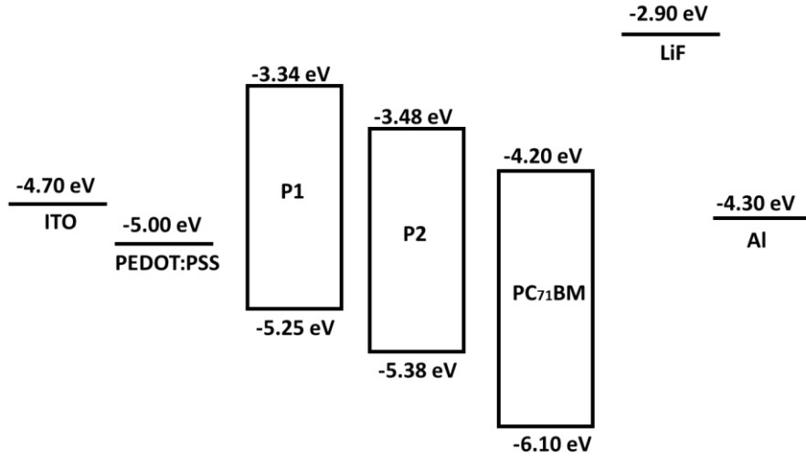
Figure 3.6. The energy levels of P1 and P2 used in bulk heterojunction device architecture
