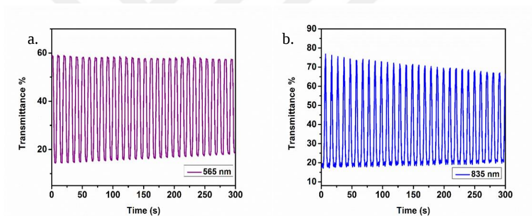
Figure 3.5. Percent transmittance changes of P2 at a) 565 nm b) 835 nm
