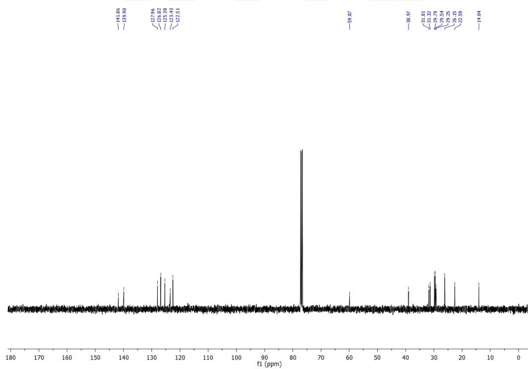
Figure A.4. 13 C NMR result of Compound 9
