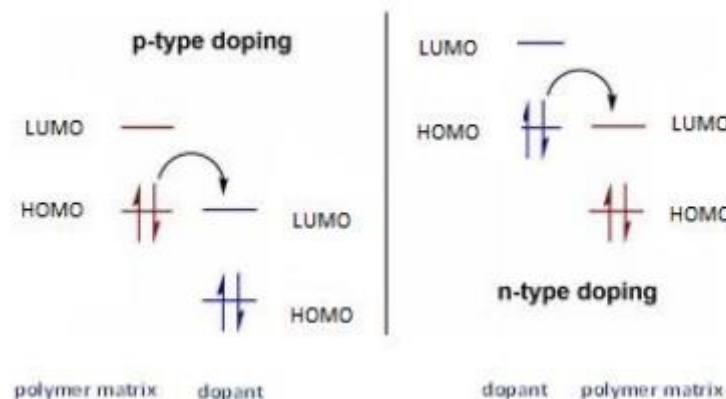
Figure 1.2. Scheme of p-doping and n-doping processes
