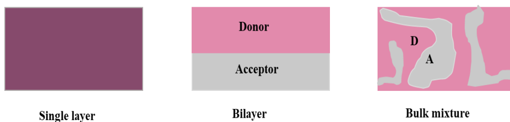
Figure 1.9. Representation of active layer of single layer, bilayer and BHJ organic photovoltaic devices
