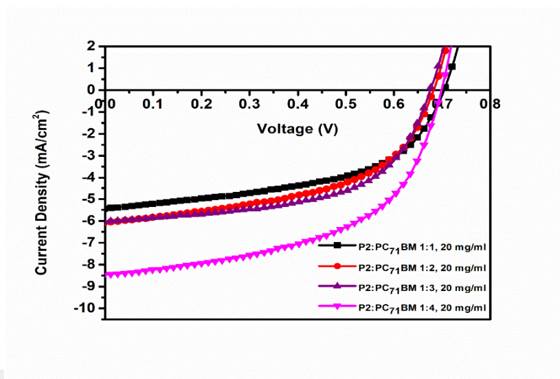
Figure 3.9. J–V curve of PSCs based on P2:PC 71 BM with different D/A ratios
