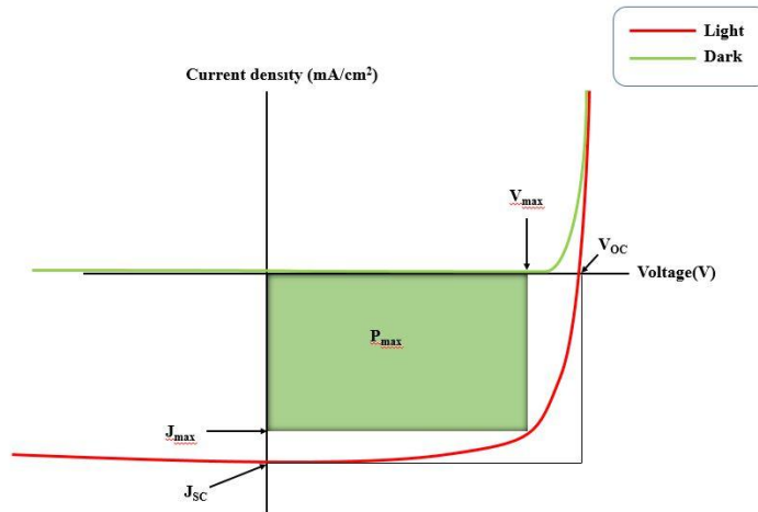
Figure 1.12. Current density (J)-voltage (V) curve under dark and light
