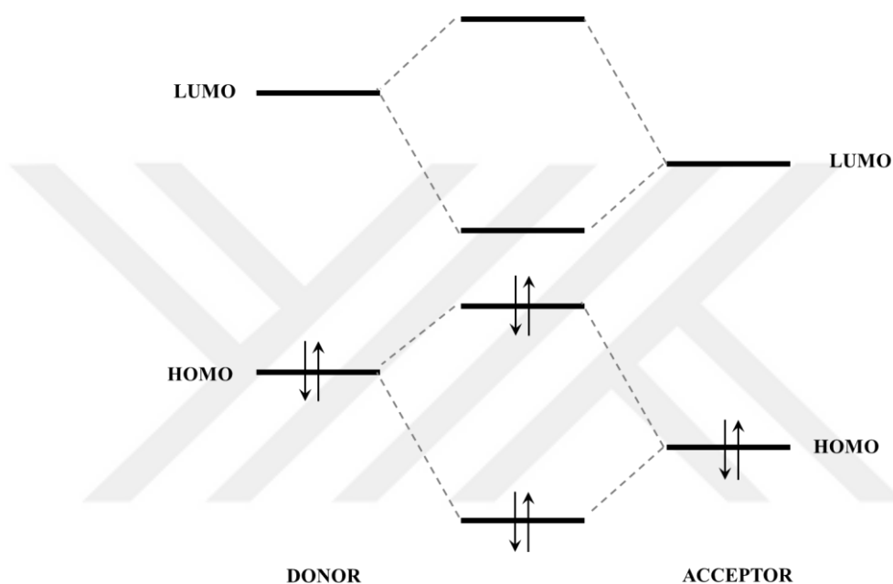
Figure 1.5. Creation of new molecular orbital energy diagram in D-A approach
