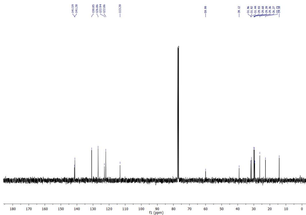
Figure A.6. 13 C NMR result of Compound 10
