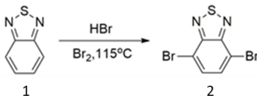
Figure 2.1. Synthesis of compound 2
