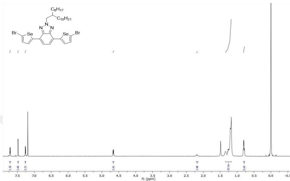
Figure A.9. 1 H NMR result of Compound 14
