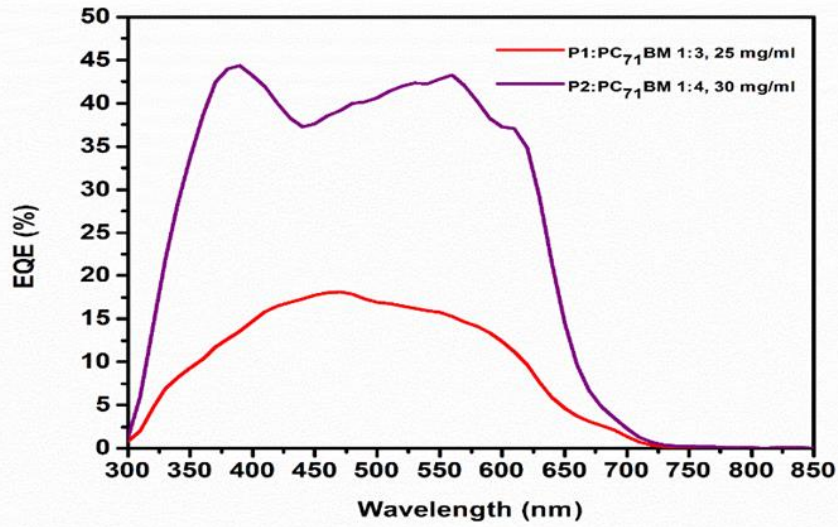
Figure 3.11. External quantum efficiency curves for best performance photovoltaics of P1 and P2
