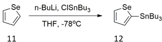
Figure 2.8. Synthesis of compound 12
