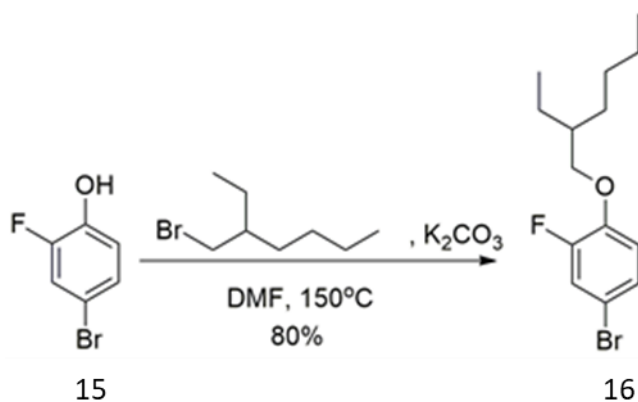
Figure 2.11. Synthesis of compound 15
