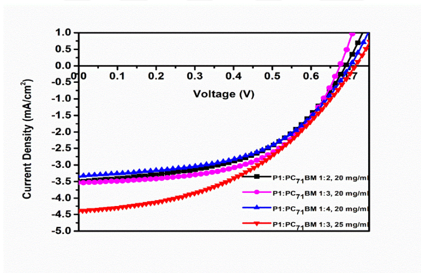
Figure 3.8. J–V curves that summarize photovoltaic performance of P1
