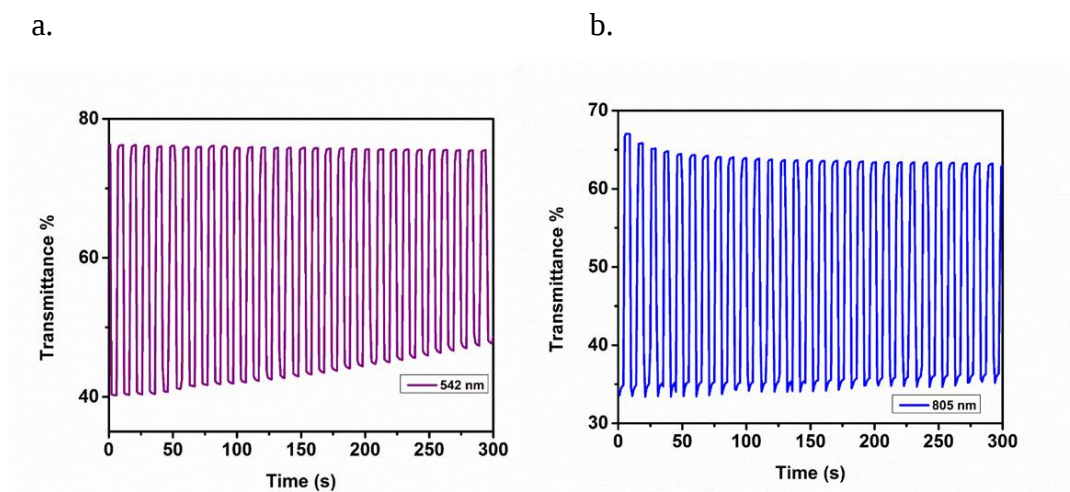
Figure 3.4. Percent transmittance changes of P1 at a) 542 nm b) 805 nm
