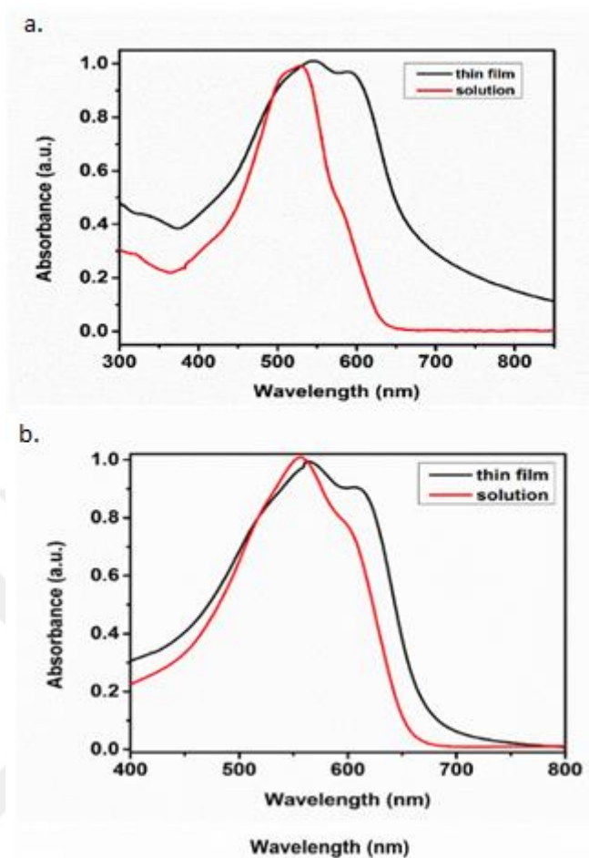
Figure 3.3. UV-Vis spectra of a) P1 and b) P2 in a chloroform solution and in the thin-film state
