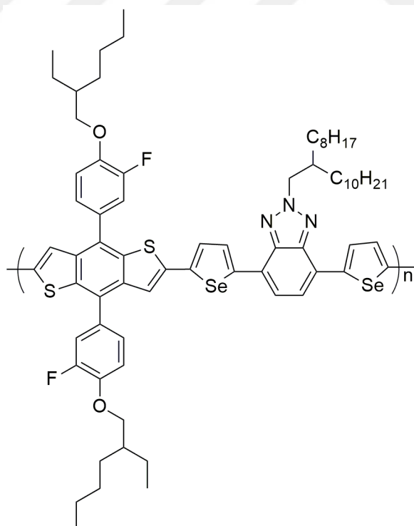
Figure 1.16. The molecular structure of selenophene containing P2
