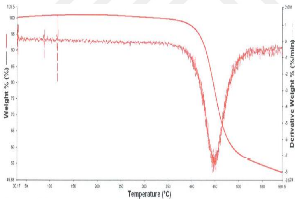
Figure B.2. TGA Curve of P1
