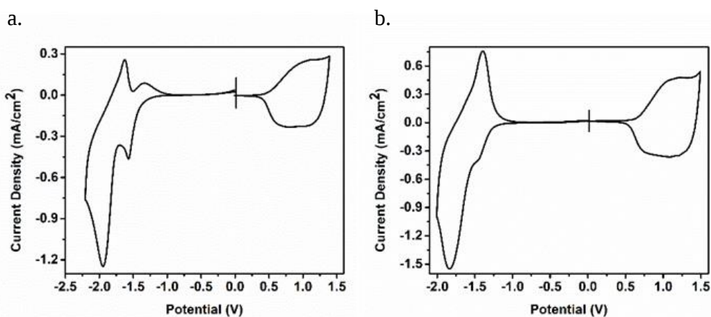
Figure 3.1. Cyclic voltammograms of polymers a) P1 b) P2 in 0.1 M TBAPF 6 /ACN electrolyte solution at a scan rate 100 mV/s
