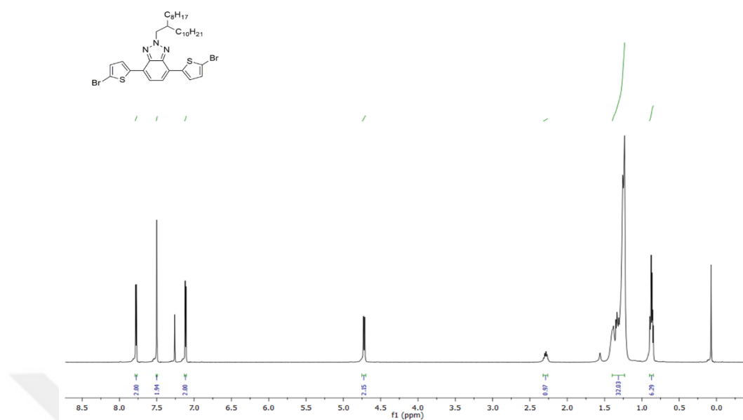
Figure A.5. 1 H NMR result of Compound 10
