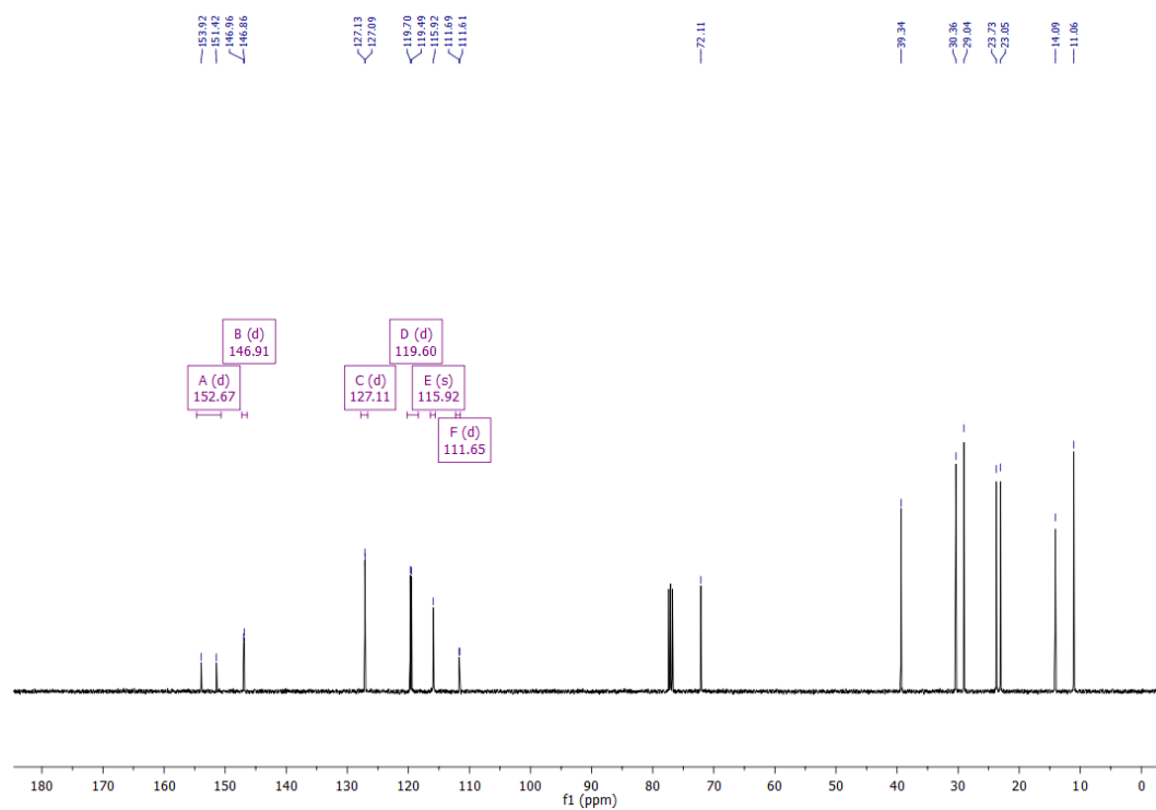
Figure A.12. 13 C NMR result of Compound 16
