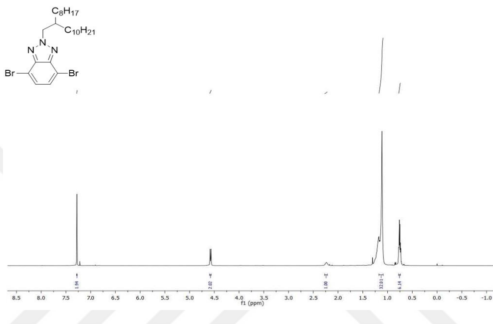
Figure A.1. 1 H NMR result of Compound 6
