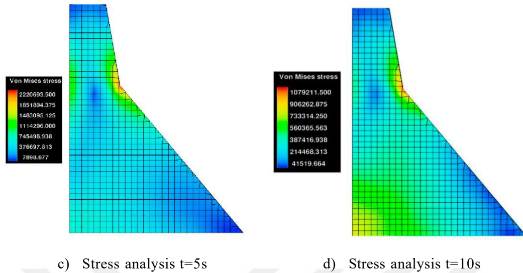
Figure 5.4. Stress analysis on Koyna dam's body
