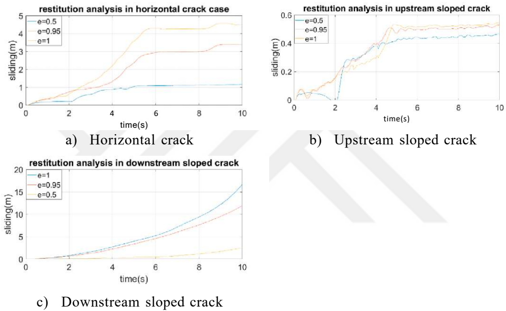
Figure 4.3. The effect of restitution coefficient on top block sliding
