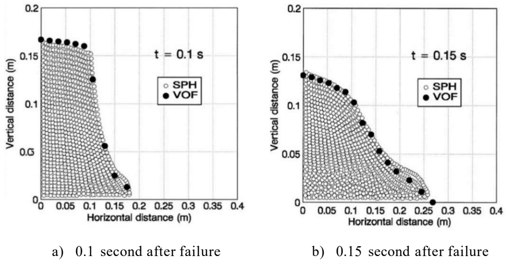
Figure 2.4. Comparison of SPH and VOF results in sudden dam break case reprinted from Shao & Lo, (2003). P. 794
