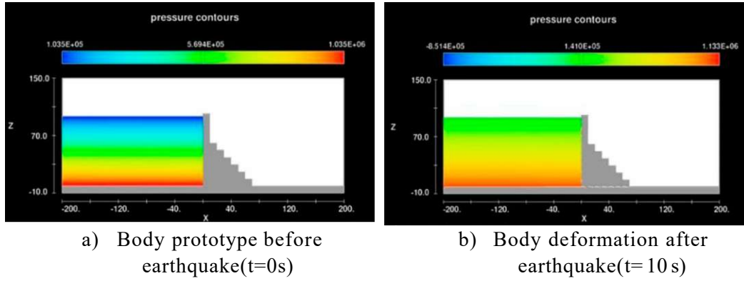
Figure 5.8. Failure of Koyna dam in the earthquake time
