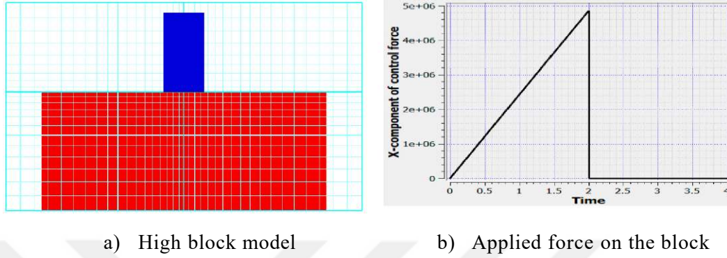
Figure 4.12. High block model
