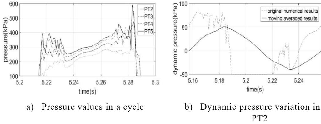
Figure 3.8. Detailed analysis of pressure distribution
