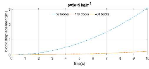
d) p=5e+5 \text{ kg/m}^3
