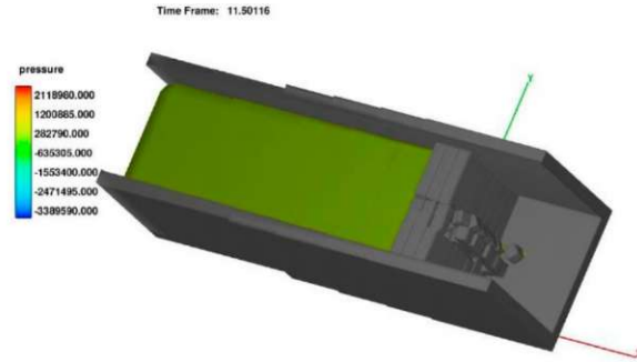
h) t=11.5s (3D view)
