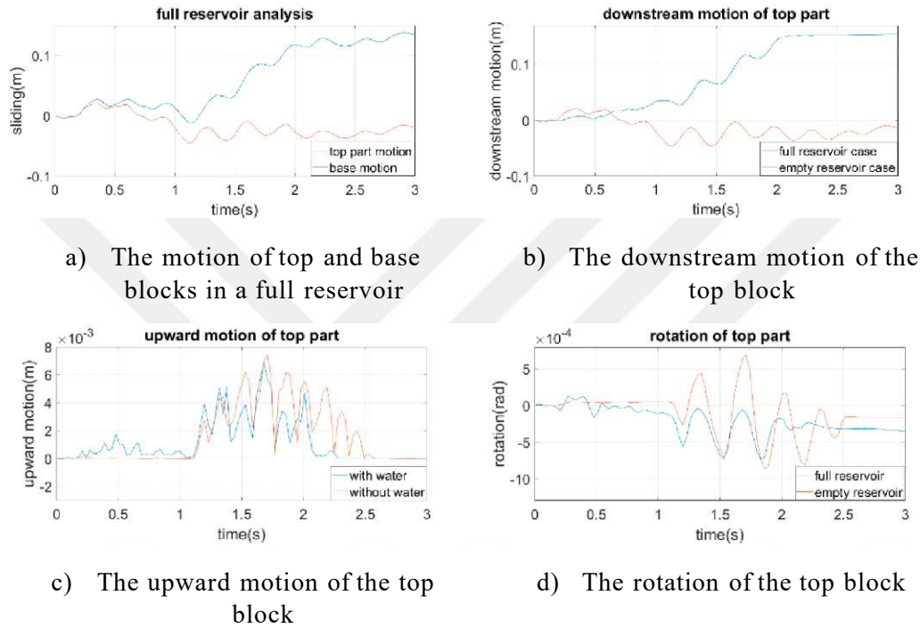
Figure 4.20. Full reservoir analysis compared to empty reservoir case
