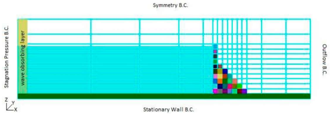
Figure 5.3. Utilized mesh planes and boundary conditions in CFD model
