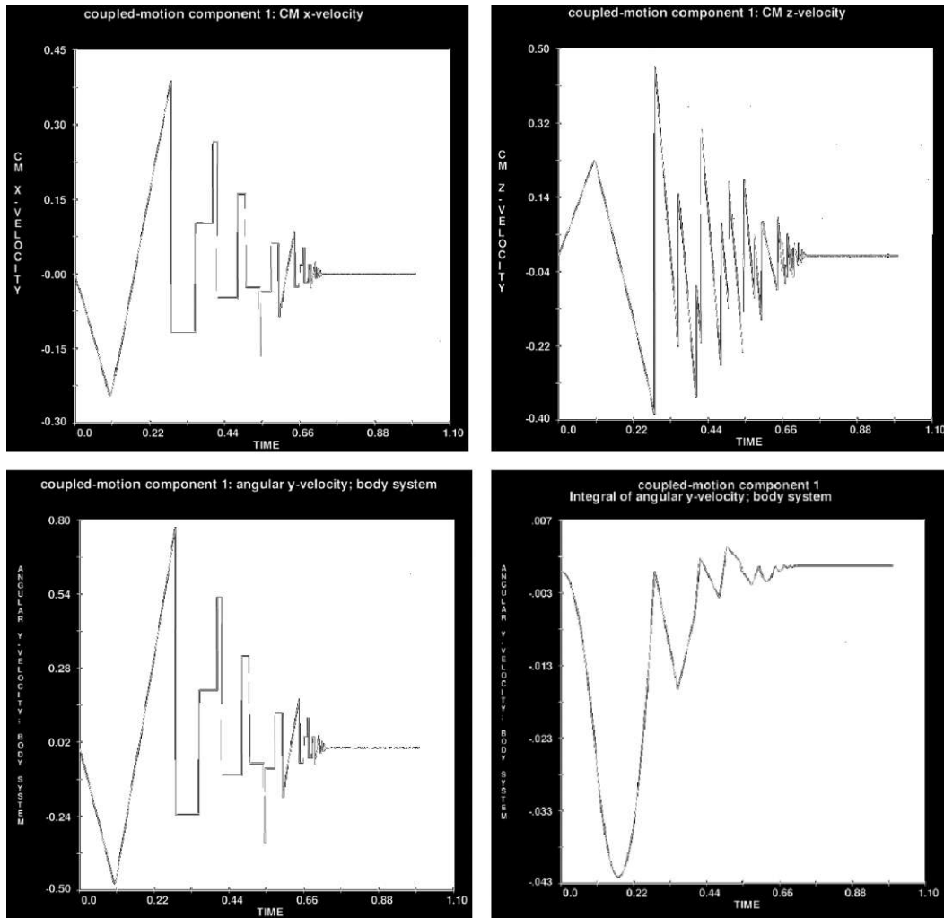
Figure B.2. The motions of the top block due to applied force on its movable base
