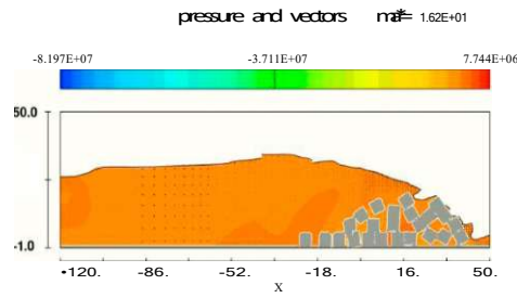
c) Sudden failure (t=20s)
