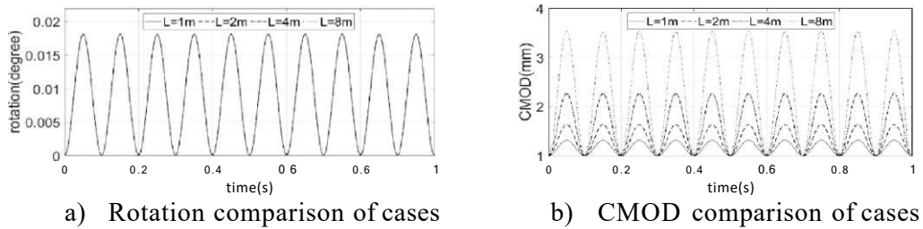
Figure 3.24. Constant angular velocity- crack size effects
