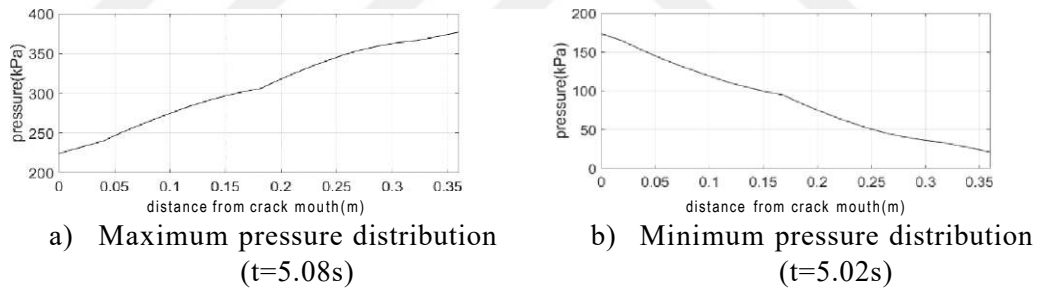
Figure 5.2. Pressure distribution inside of the crack
