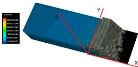
a) t=1s (sudden failure)
