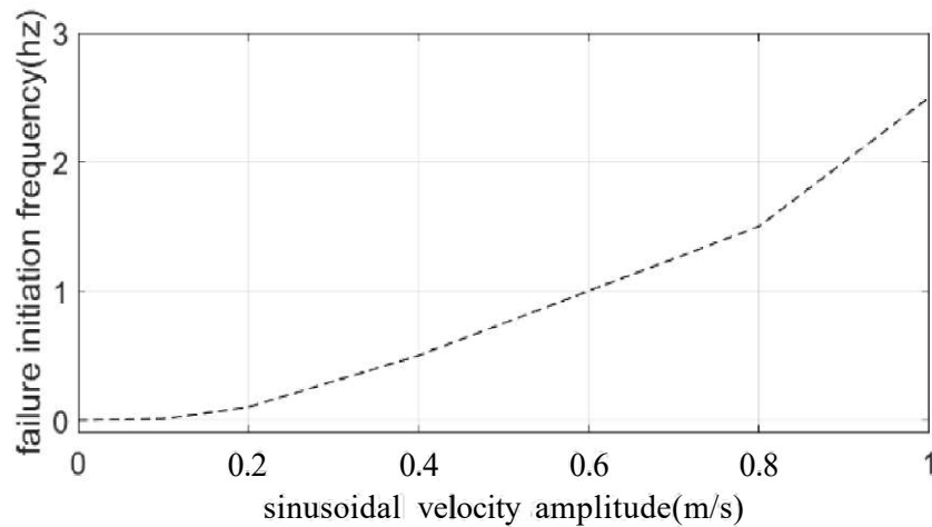
a) The critical frequency of failure vs. velocity amplitude
