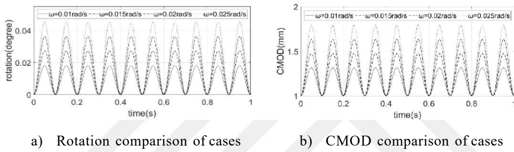
Figure 3.22. Constant crack length- CMOD effects
