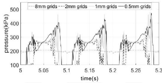
c) Grid size analysis in PT3
