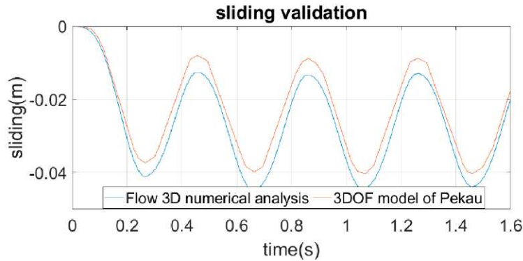
Figure 4.11. Square block sliding motion validation
