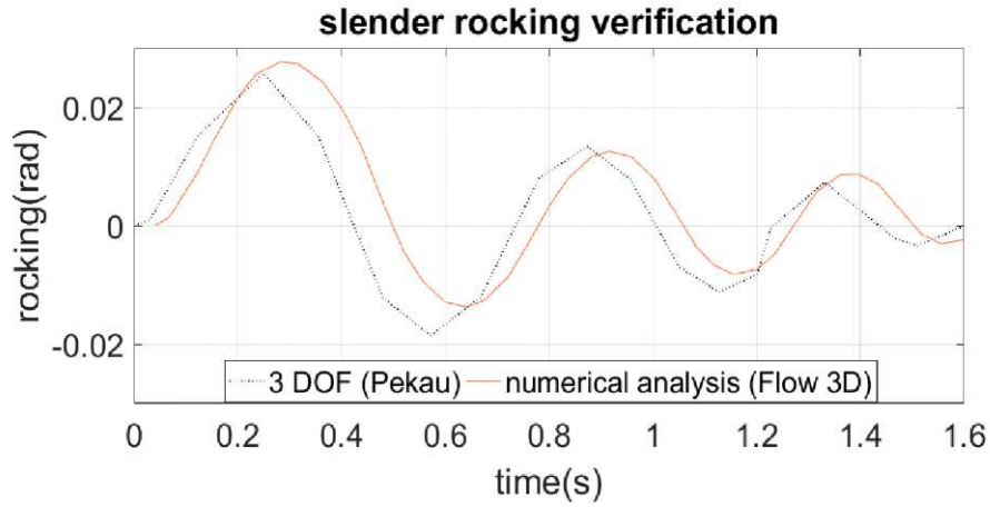
Figure 4.17. . Rocking validation of slender bar
