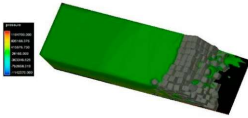
c) t=3s (sudden failure)
