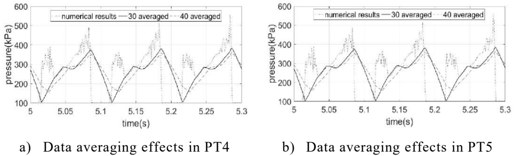
Figure 3.9. Moving average filtering of points PT4 and PT5
