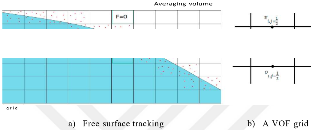
Figure 2.2. VOF technique
