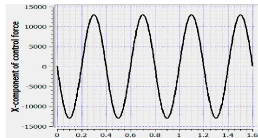
b) Applied force on the low block
