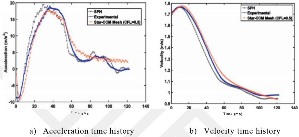
Figure 2.6. Comparison of RANS and SPH methods with the experimental study reprinted from Sasson et al., (2016). P. 127
