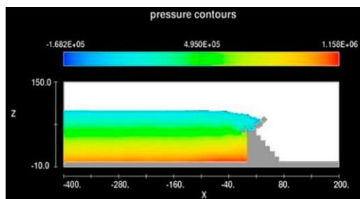
a) Gradual failure (t=45s)
