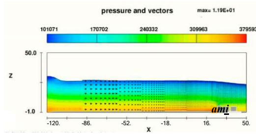
l) Semi-gradual failure (t=500s)
