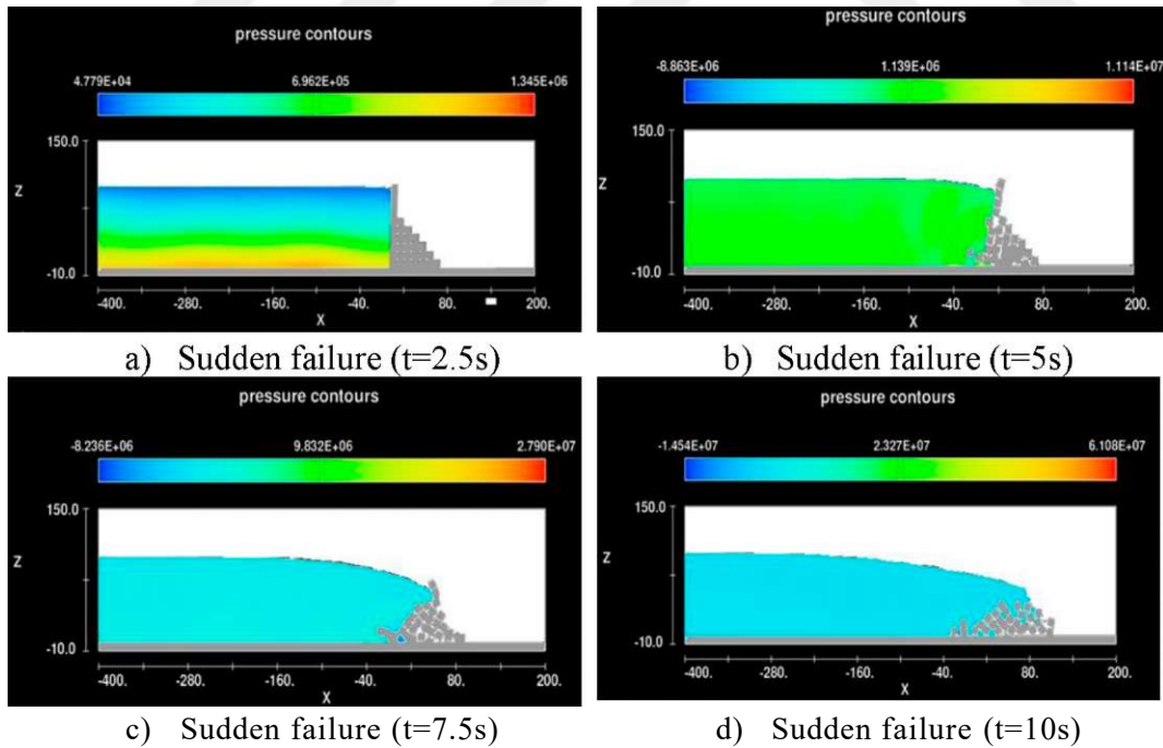
Figure 5.9. Failure of hypothetical plaster dam
