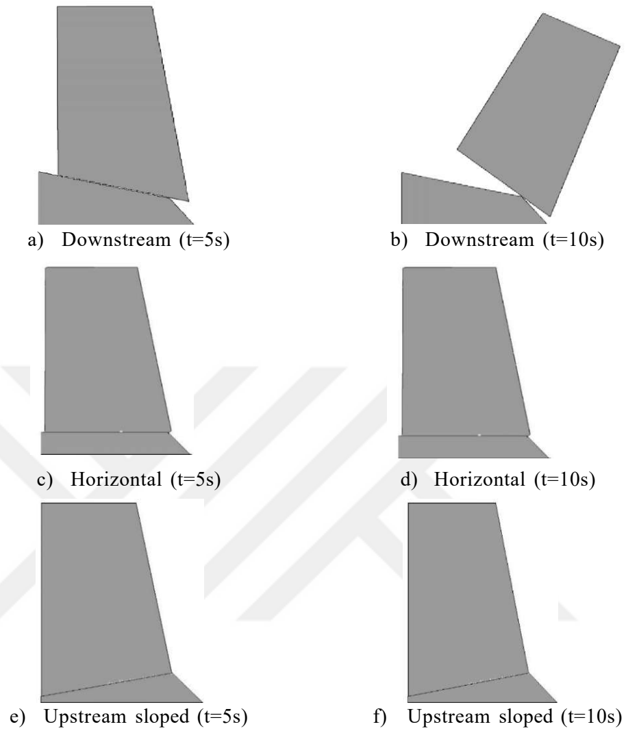
Figure 4.8. Displacement comparison of three cases of cracks
