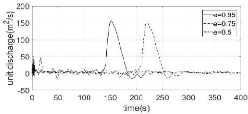
c) Upstream sloped crack case
