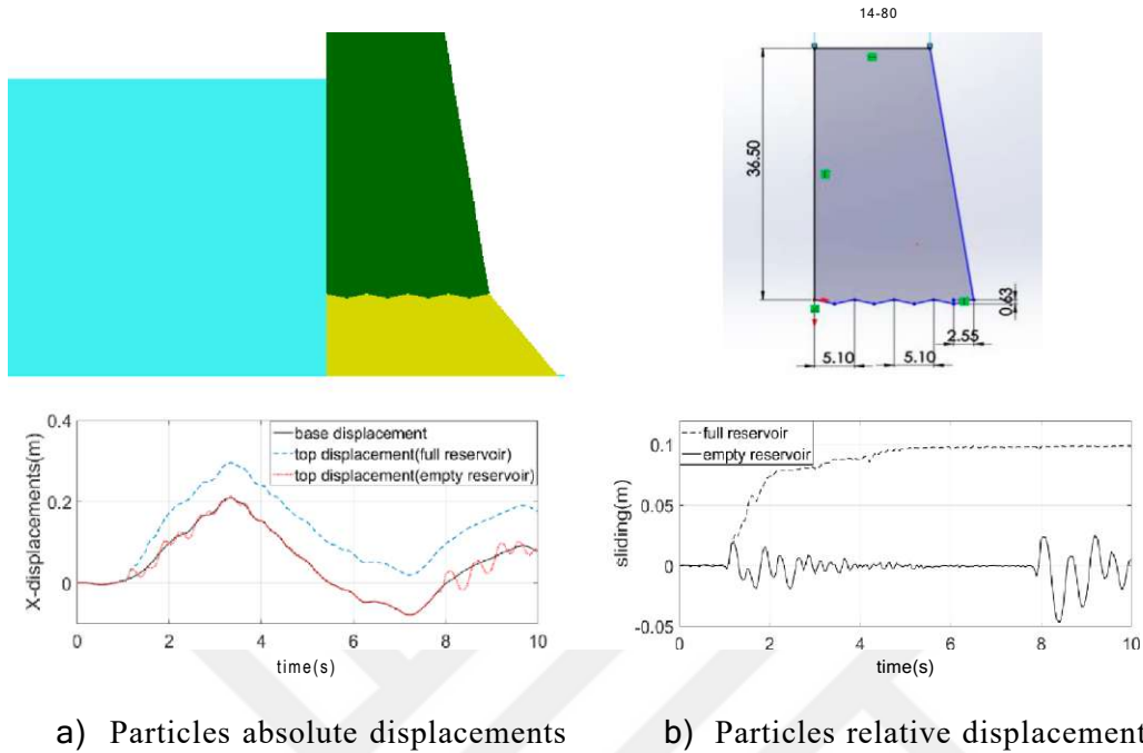
Figure C.4. Four-step case motion in full and empty reservoir conditions
