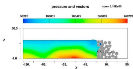
a) Sudden failure (t=10s)
