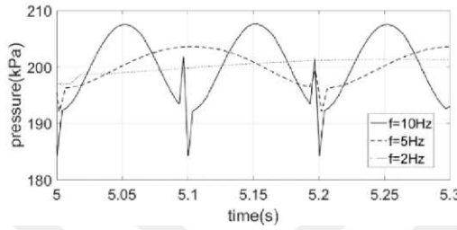
c) Pressure variation with time in PT3
