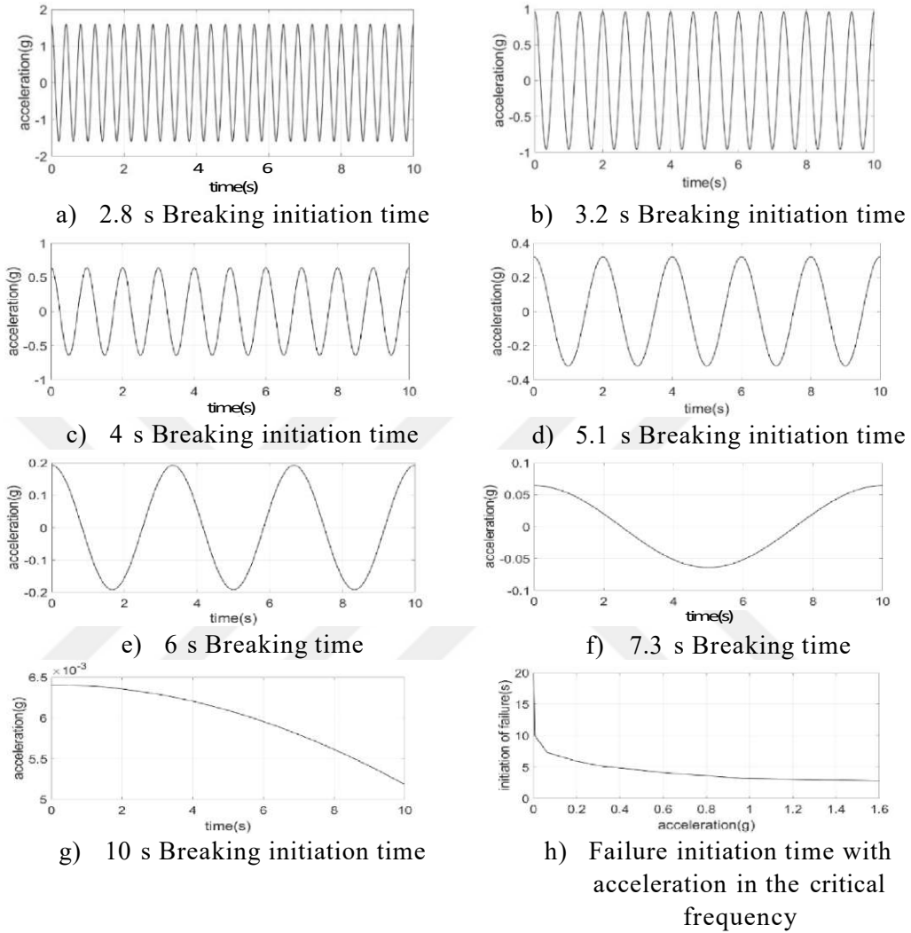
Figure 5.13. Failure analysis using acceleration concept
