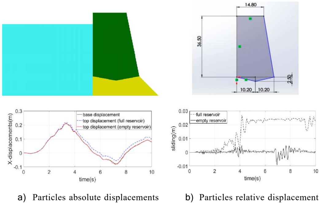
Figure C.1. One-step case motion in full and empty reservoir conditions
