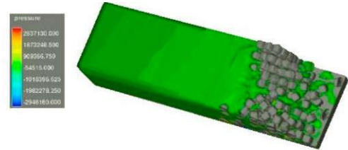
l) t = 16s (semi-gradual failure)
