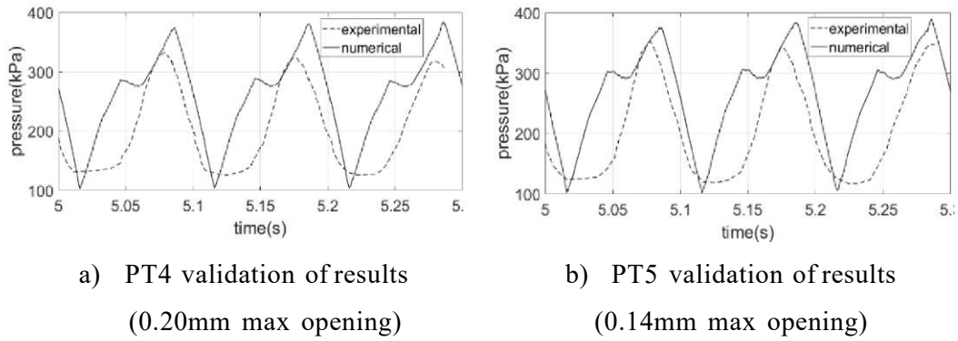
Figure 3.11. Verification of results with experimental data for PT4 and PT5
