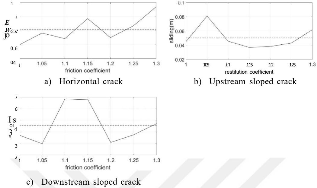
Figure 4.7. Final displacement vs. friction coefficient
