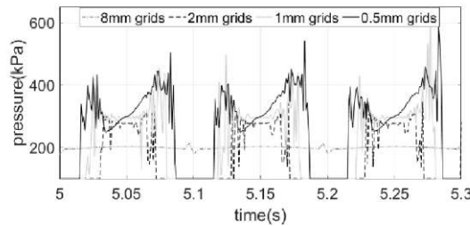
e) Grid size analysis in PT5
