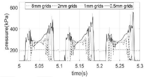
d) Grid size analysis in PT4
