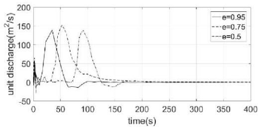
a) Horizontal crack case
