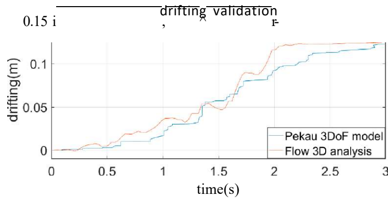
b) Drifting validation
