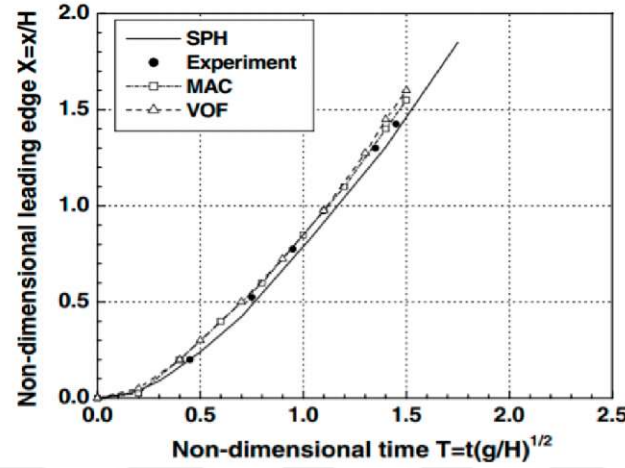
Figure 2.5. Verification of VOF, MAC, and SPH results with reprinted from Shao & Lo, (2003). P. 794
