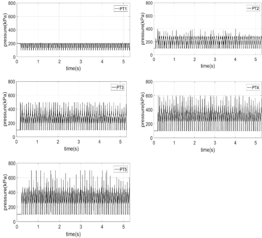
Figure 3.7. Pressure variation with time in 5.3 seconds
