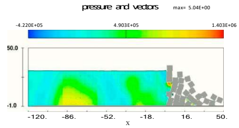
d) Semi-gradual failure (t=20s)
