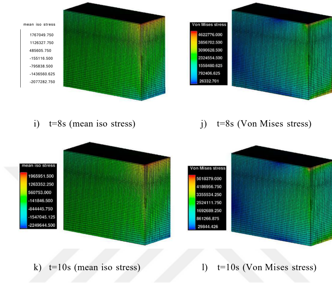
Figure 5.24. Stress analysis on the dam's body
