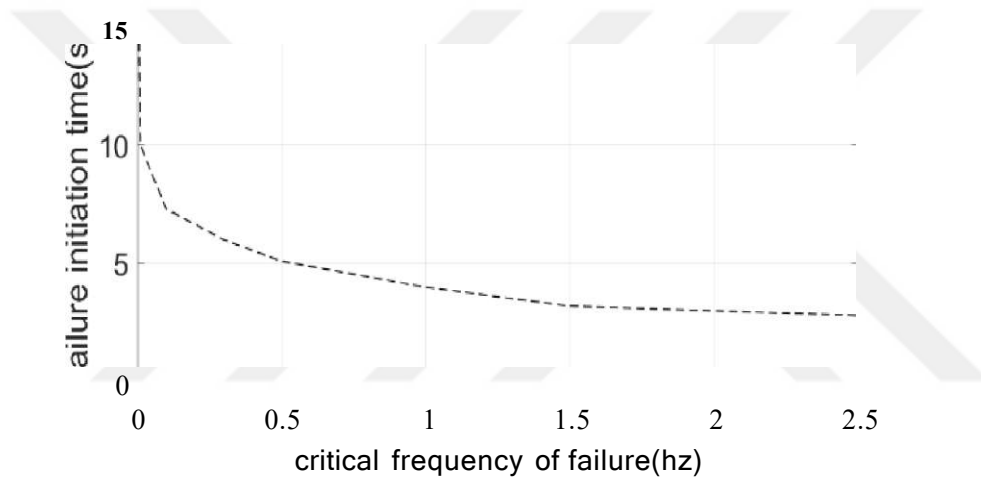
c) Critical failure time vs. critical frequency
