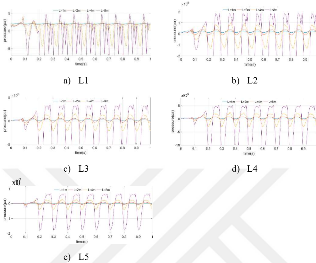
Figure 3.25. Crack size effects on pressure distribution in the cracked area
