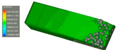
p) t = 20s (semi-gradual failure)
