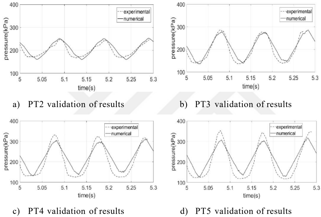
Figure 3.10. Verification of results with experimental data for PT2, PT3, PT4, and PT5 locations
