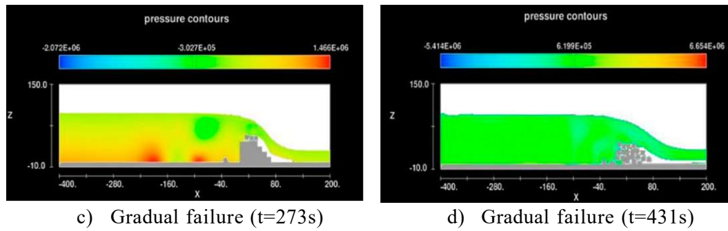
Figure 5.15. Gradual failure of Koyna dam
