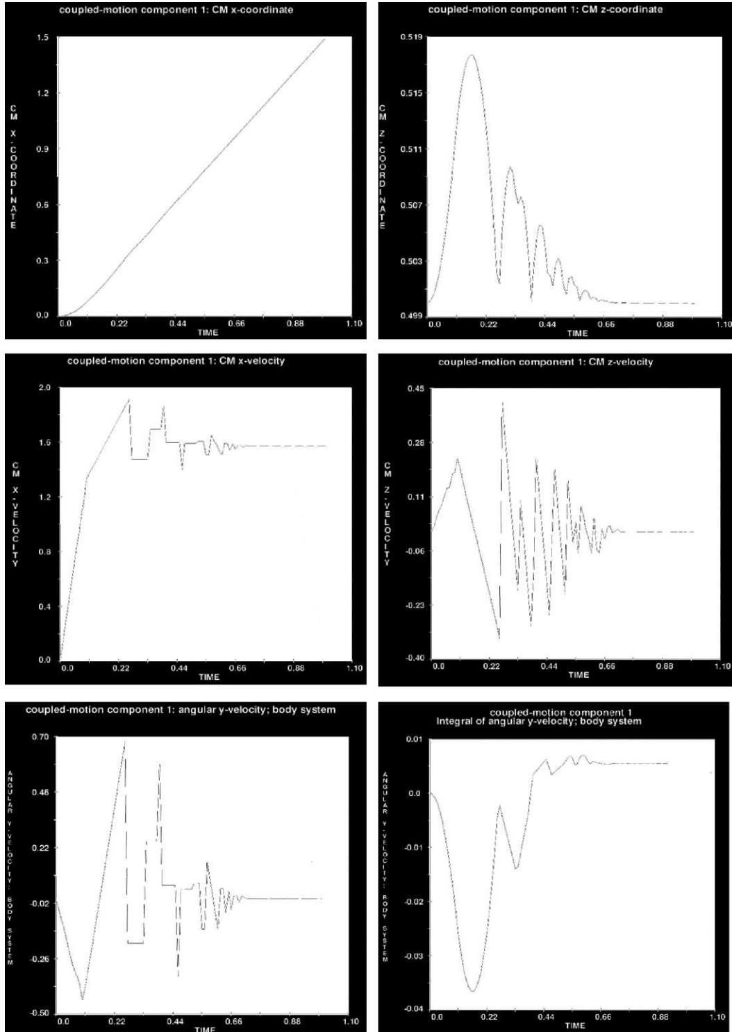
Figure B.4. The motions of the top block due to applied velocity on the base block
