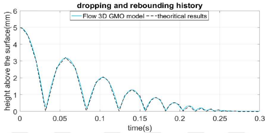
Figure 4.14. Dropping and rebounding validation
