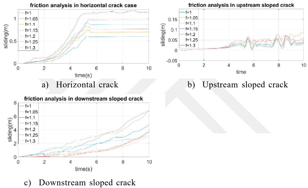
Figure 4.6. Friction coefficient effects on the motion of top Part
