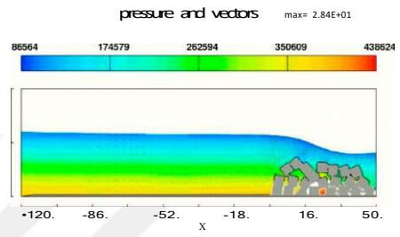
f) Semi-gradual failure (t=100s)
