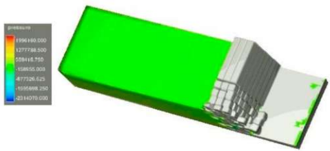
e) t\sim 11.6s (semi-gradual failure)
