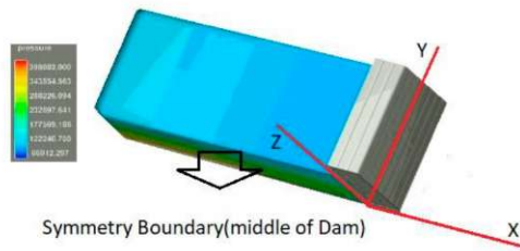
a) t=10s (semi-gradual failure)
