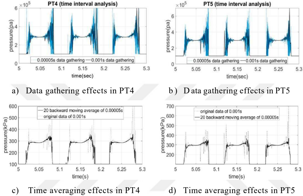
Figure 3.6. Time step and data gathering time interval size effects on captured pressure values
