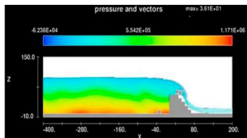
b) Gradual failure (t=74s)
