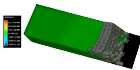
b) t=2s (sudden failure)
