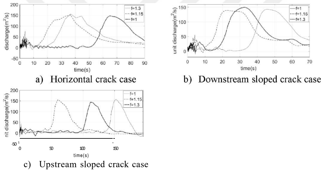
Figure 4.25. Friction effects on discharge hydrograph ( f > 1 )
