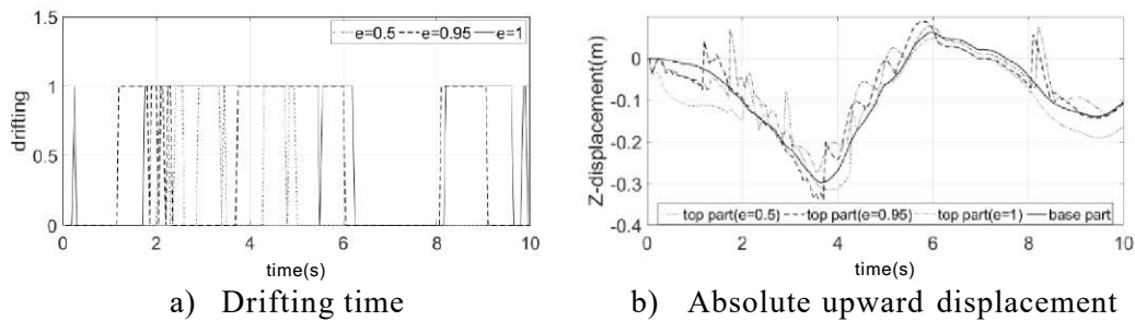
Figure 4.5 Restitution coefficient effects on upward displacement
