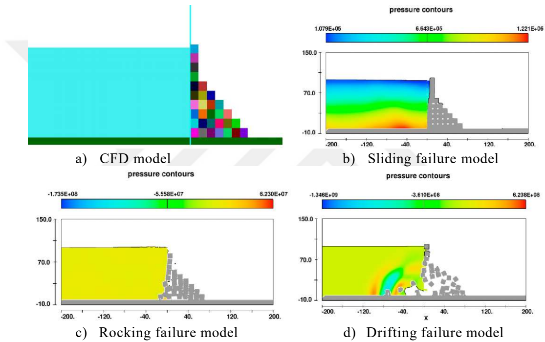
Figure 5.5. Sliding, rocking, and drifting mode of dam failure initiation
