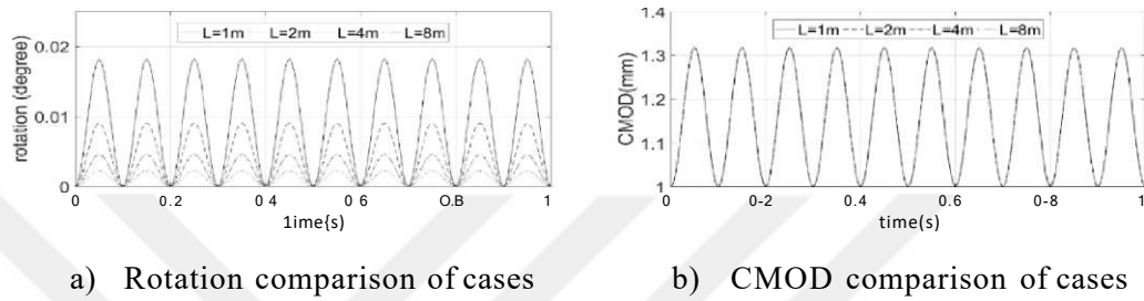
Figure 3.20. Constant CMOD- crack length effects
