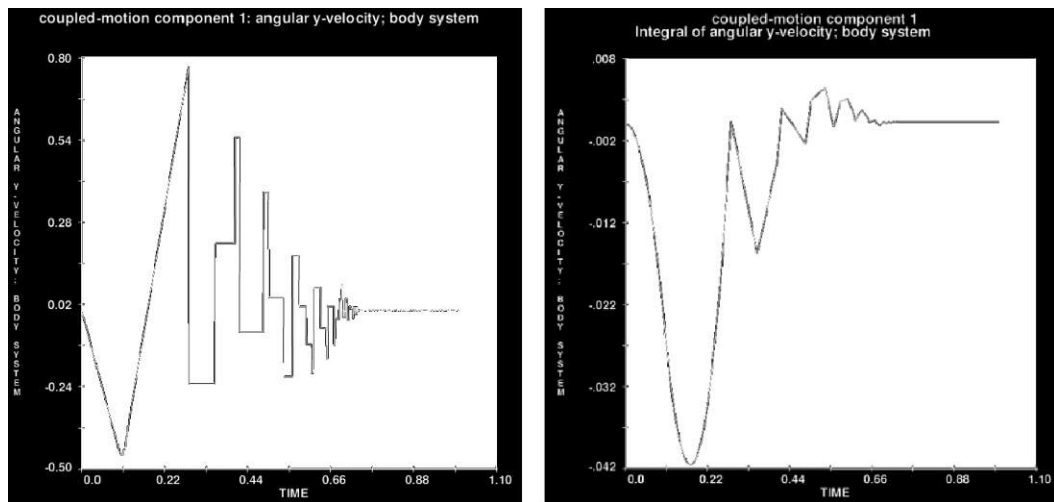
Figure B.1. The motions of the top block due to applied force on it- constant base
