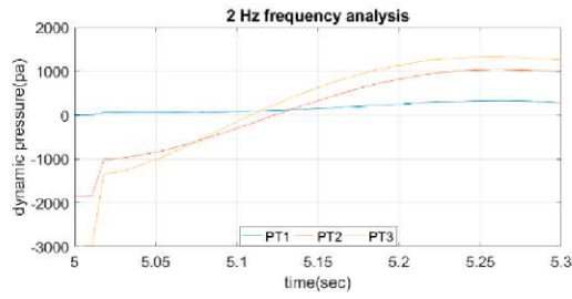
a) Dynamic pressure with 2Hz frequency
