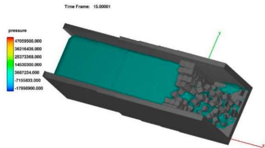
v) t=15s (3D view)
