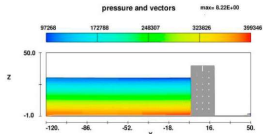
b) Semi-gradual failure (t=10s)
