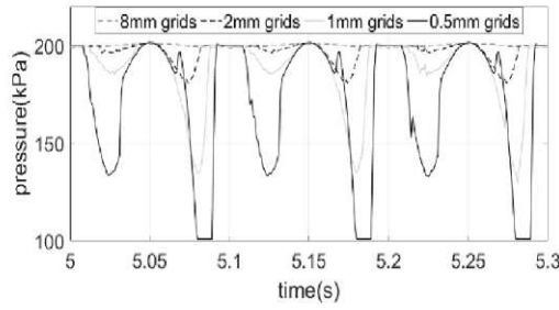
a) Grid size analysis in PT1
