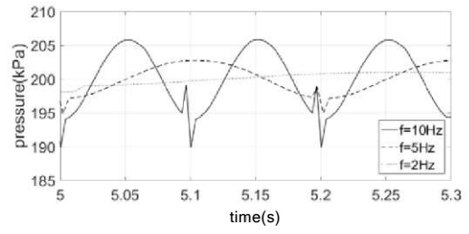
b) Pressure variation with time in PT2
