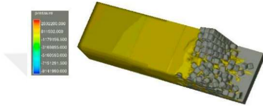
k) t = 15s (semi-gradual failure)
