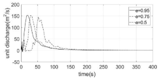
b) Downstream sloped crack case
