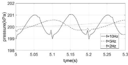
a) Pressure variation with time in PT1
