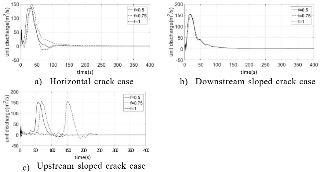
Figure 4.24. Friction effects on discharge hydrograph ( f < 1 )
