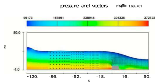
i) Sudden failure (t=400s)
