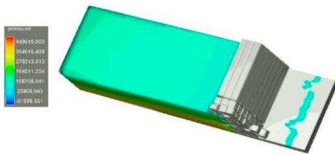
c) t\sim 10.8s (semi-gradual failure)
