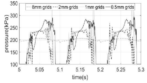
b) Grid size analysis in PT2
