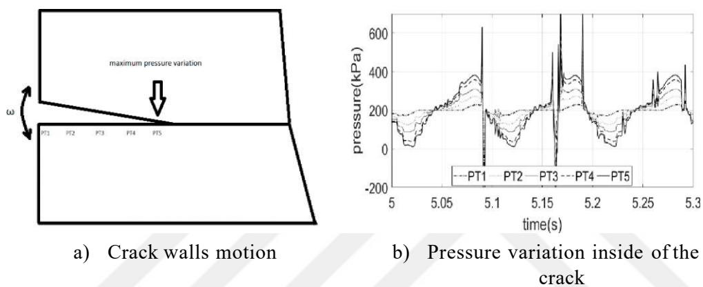
Figure 5.6. Inside crack pressure variation
