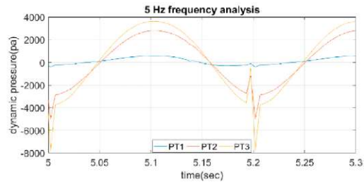
b) Dynamic pressure with 5Hz frequency
