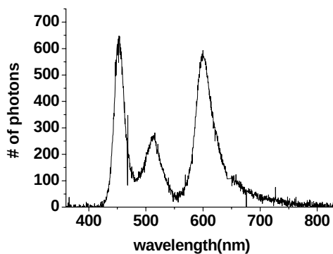
Figure 5.3.4. Electroluminescence spectrum of 75 µl cyan NC and 9.3 µl PMMA corresponding to a film concentration of 12.05 µmol/mL and 150 µl yellow NCs ( \lambda_{PL}=500 and 580 nm) and 18.75 µl PMMA corresponding to a film concentration of 12.05 µmol/mL hybridized on blue LED ( \lambda_{EL}=452 nm) measured at an injection current level of 5 mA at room temperature.
