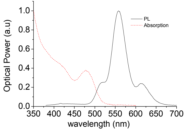
Figure 4.2.10. PL and absorption spectra of onion like CdSe/ZnS/CdSe ( \lambda_{PL}=520, 560 and 620 nm) nanoparticle in solution.
