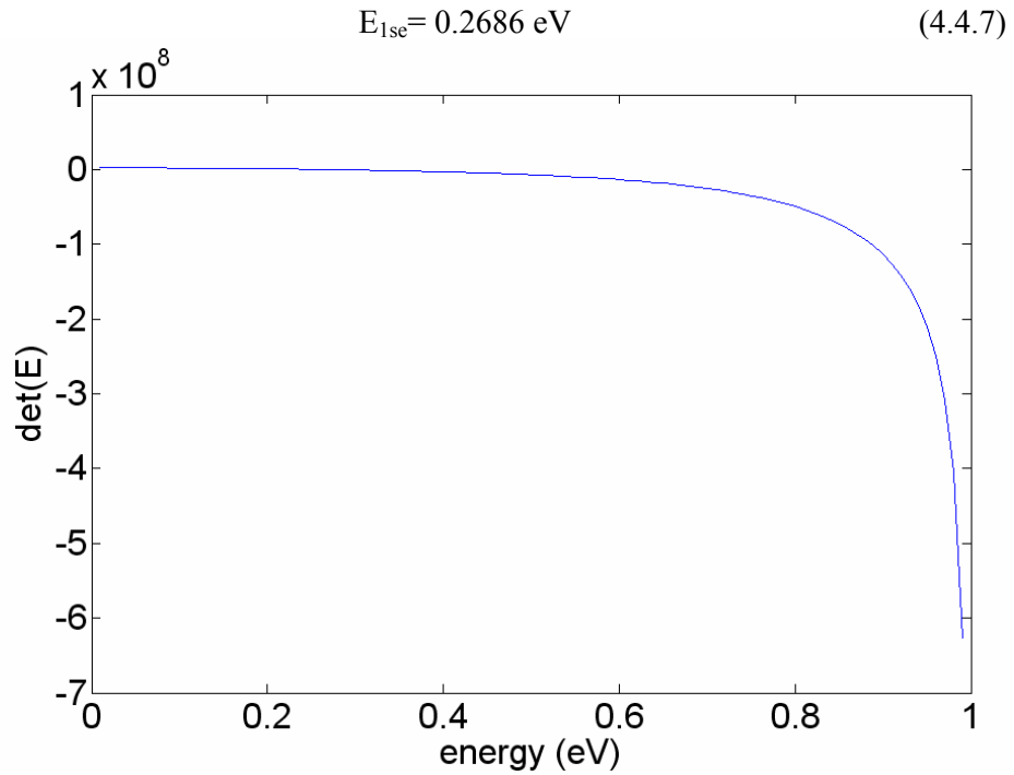
Figure 4.4.2. Determinant of 2x2 matrix vs. energy for electrons.
