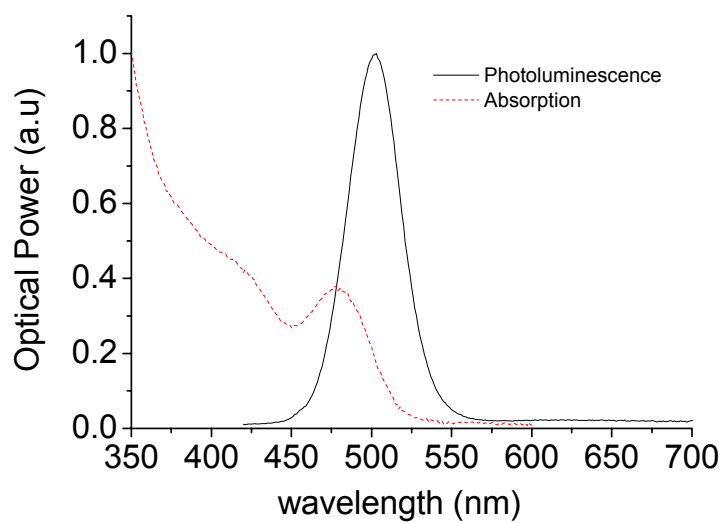
Figure 4.2.5. PL and absorption spectra of cyan CdSe ( \lambda_{PL}=502 nm) nanoparticle in solution.
