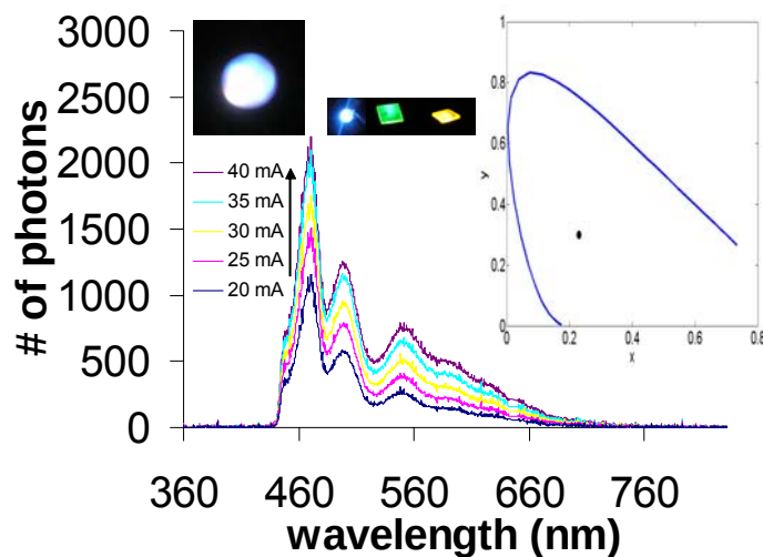
Figure 5.4.3.1. Electroluminescence spectra of blue polyfluorene ( \lambda_{\text{PL}} = 439 \text{ nm} ) and green and yellow CdSe/ZnS core-shell nanocrystals ( \lambda_{\text{PL}} = 540 and 580 \text{ nm} ) layer-by-layer hybridized on an InGaN/GaN n-UV LED ( \lambda_{\text{EL}} = 383 \text{ nm} ) at different levels of current injection (at room temperature) along with a picture of the generated white light (blue polymer and green and yellow nanocrystals); and the location of the corresponding operating point on the (x, y) coordinates.
