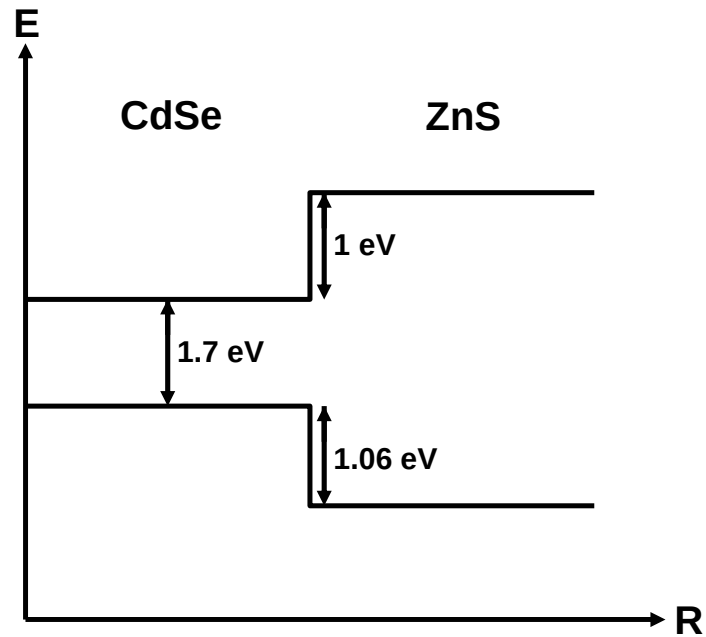
Figure 4.4.1. Energy diagram of CdSe/ZnS core-shell nanocrystals.
