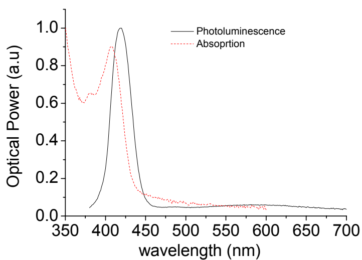
Figure 4.2.1. PL and absorption spectra of violet ( \lambda_{\text{PL}}=419 nm) CdS nanoparticle in solution.
