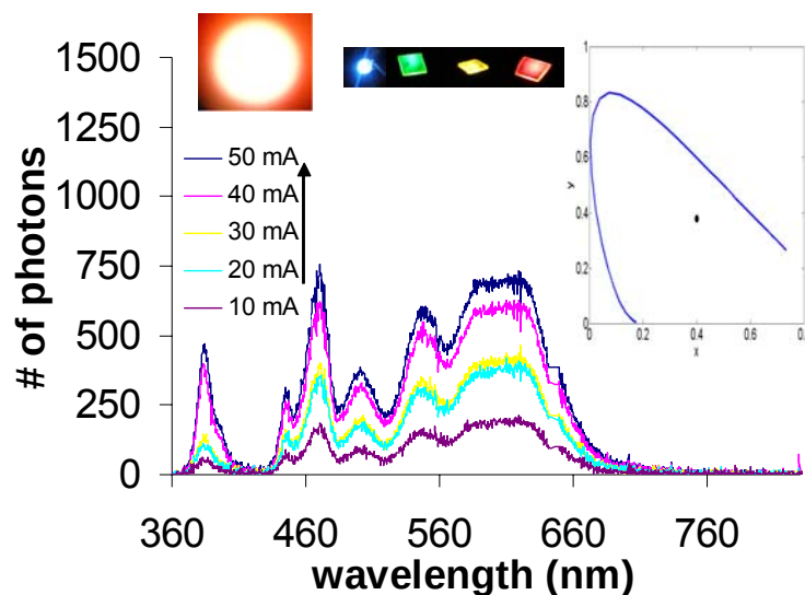
Figure 5.4.5.1. Electroluminescence spectra of blends of blue polyfluorene ( \lambda_{PL} = 439 nm) and yellow, green and red CdSe/ZnS core-shell nanocrystals ( \lambda_{PL} = 580, 540 and 620 nm) hybridized on a InGaN/GaN n-UV LED at different levels of current injection at room temperature along with a picture of the generated white light, blue conjugated polymer and green, yellow and red nanocrystals, and the location of the corresponding operating point on the (x, y) coordinates.
