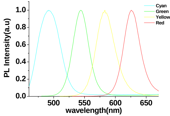
Figure 5.1.3.1. Photoluminescence spectra of our CdSe-ZnS core-shell nanocrystals in UV-curable resin.
