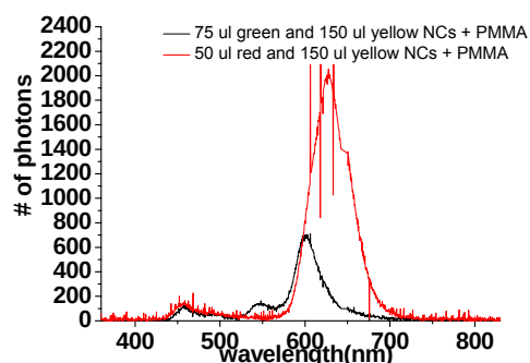
Figure 5.3.3. Electroluminescence spectrum of 75 µl green NC and 9.3 µl PMMA corresponding to a film concentration of 5.59 µmol/mL and 150 µl yellow NCs ( \lambda_{PL}=540 nm and 580 nm) and 18.75 µl PMMA corresponding to a film concentration of 12.05 µmol/mL hybridized with blue LED ( \lambda_{EL}=452 nm) at an injection current level of 5 mA and the electroluminescence spectrum of 50 µl red NC and 6.2 µl PMMA corresponding to a film concentration of 0.88 µmol/mL and 150 µl yellow NCs ( \lambda_{PL}=620 nm and 580 nm) and 18.75 µl PMMA corresponding to a film concentration of 12.05 µmol/mL hybridized on blue LED ( \lambda_{EL}=452 nm) measured at an injection current level of 5 mA at room temperature.
