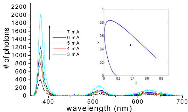
Figure 5.2.5.1. Electroluminescence spectra of dichromatic combinations of cyan ( \lambda_{PL}=504 nm) and red ( \lambda_{PL}=615 nm) nanocrystals hybridized on an n-UV LED for various current levels at room temperature.
